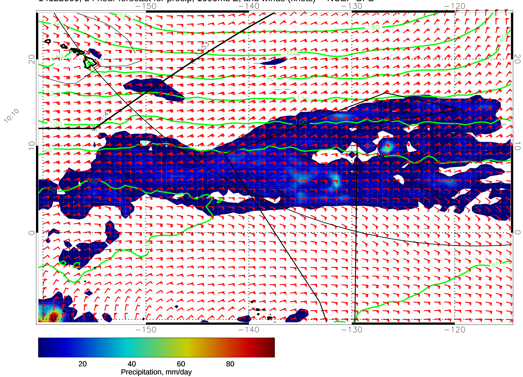
14122000, 24 hour forecast for precip, 1000mb Z, and winds (knots) -- NCEP GFS
