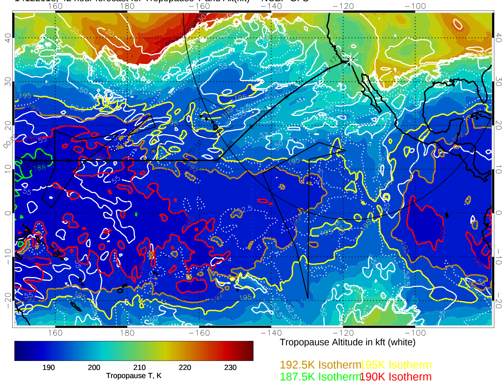
14122018, 42 hour forecast for Tropopause T and Alt(kft) -- NCEP GFS
