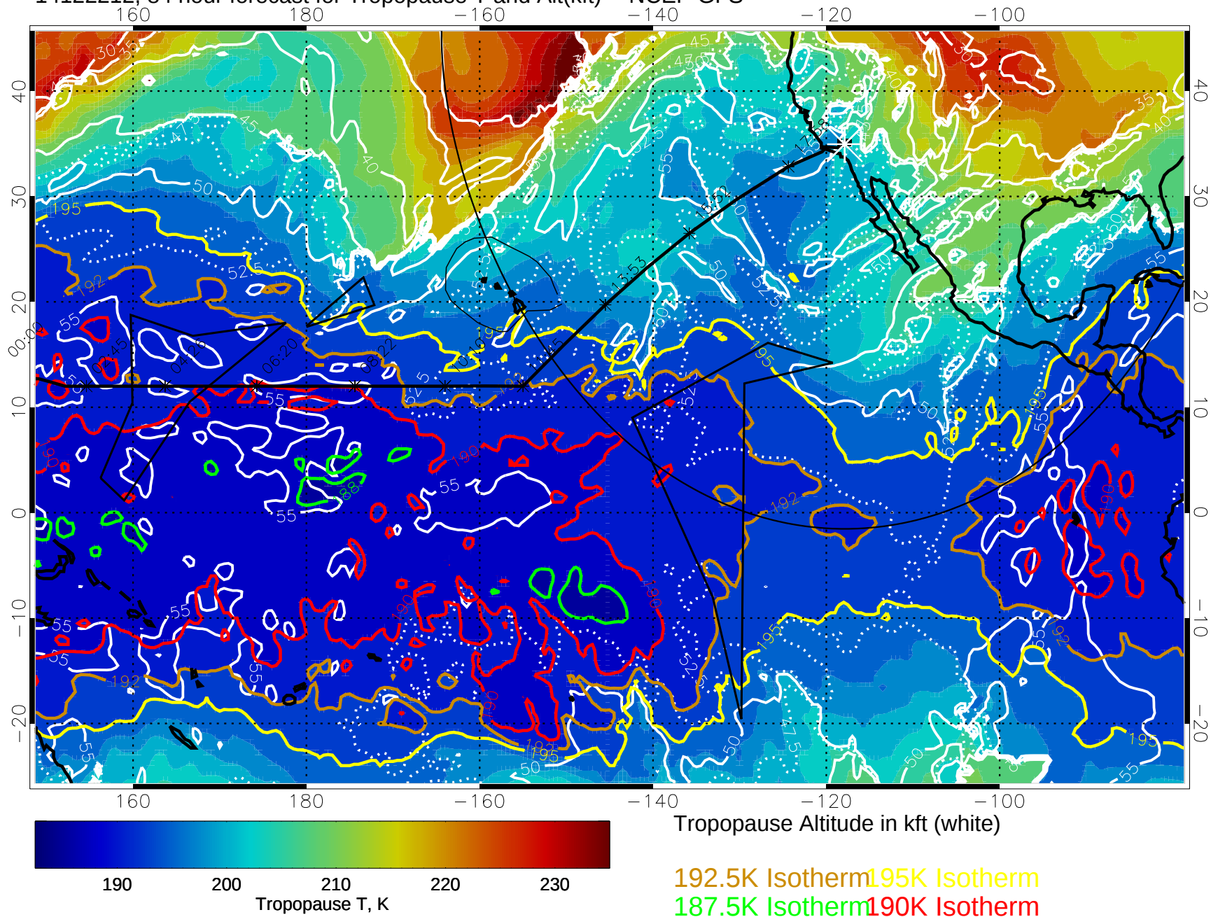
14122212, 84 hour forecast for Tropopause T and Alt(kft) -- NCEP GFS
