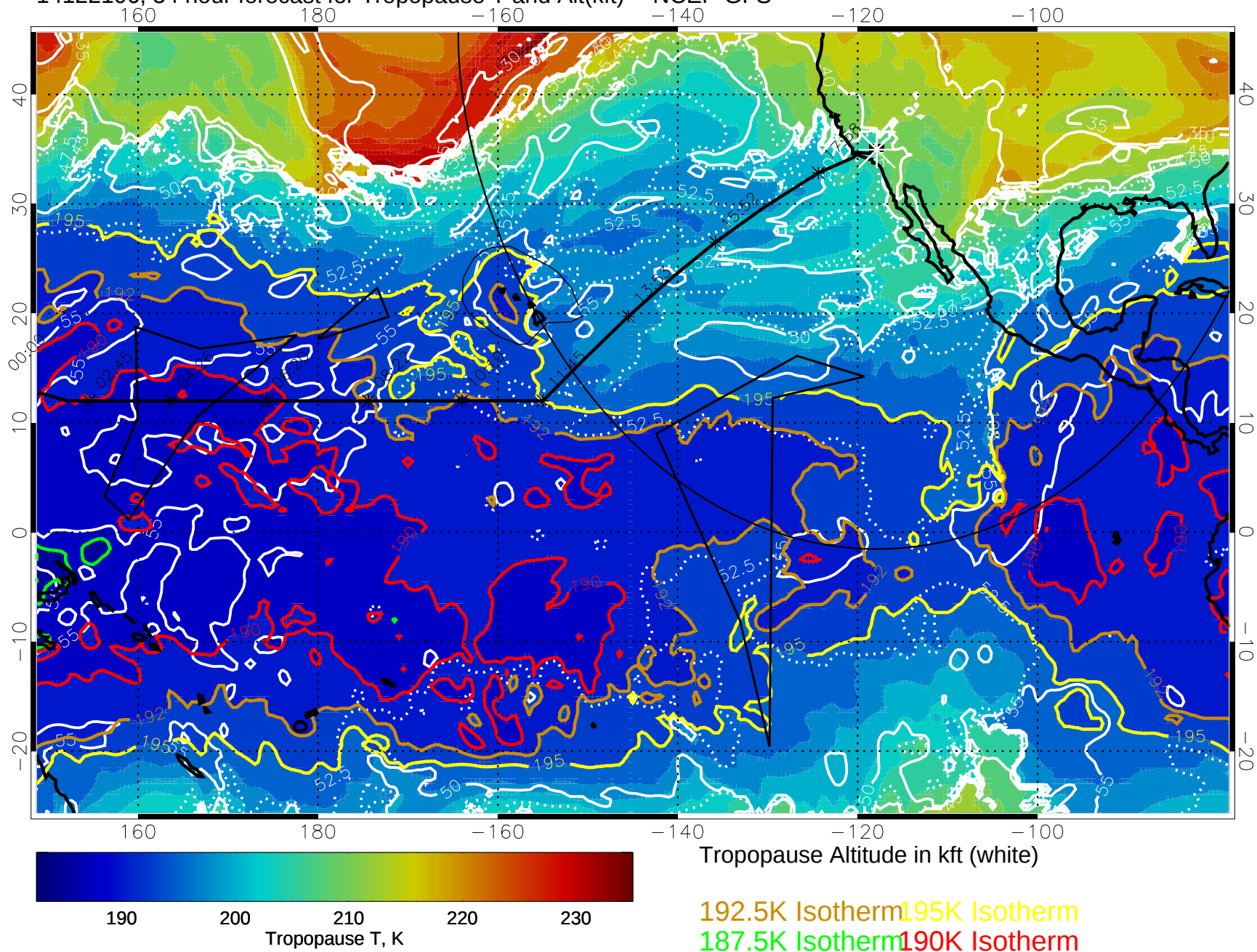
14122106, 54 hour forecast for Tropopause T and Alt(kft) -- NCEP GFS
