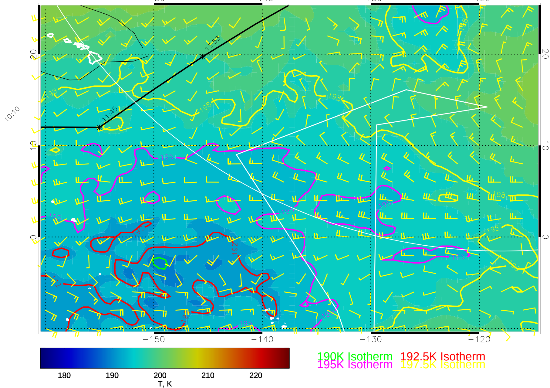
14122306, 102 hour forecast for 70mb T and winds (knots) -- NCEP GFS
