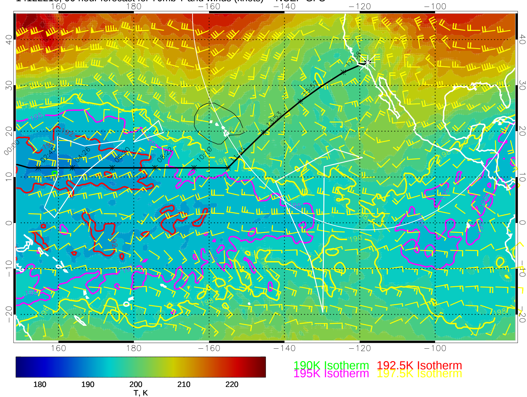
14122218, 90 hour forecast for 70mb T and winds (knots) -- NCEP GFS
