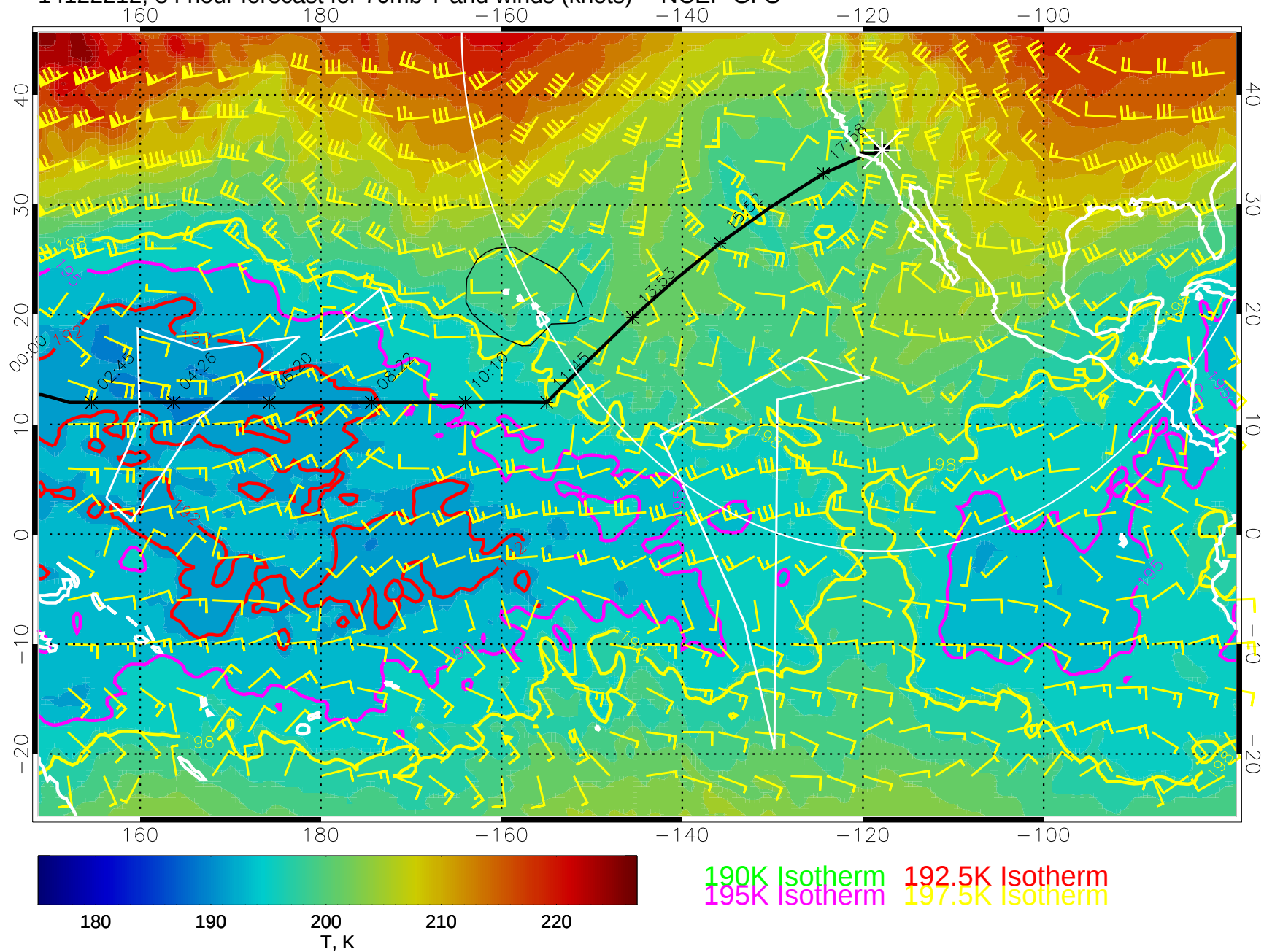
14122212, 84 hour forecast for 70mb T and winds (knots) -- NCEP GFS
