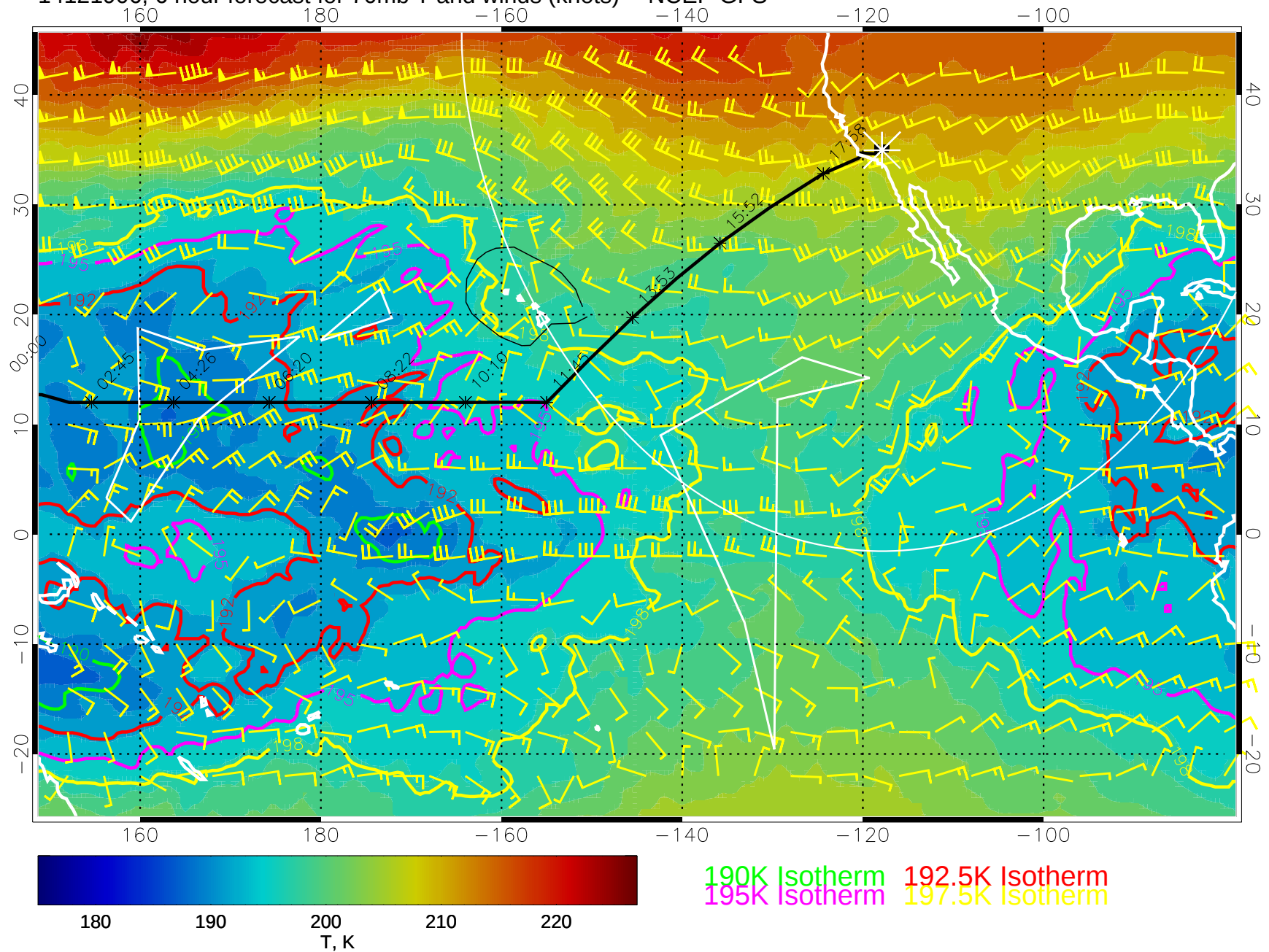
14121906, 6 hour forecast for 70mb T and winds (knots) -- NCEP GFS
