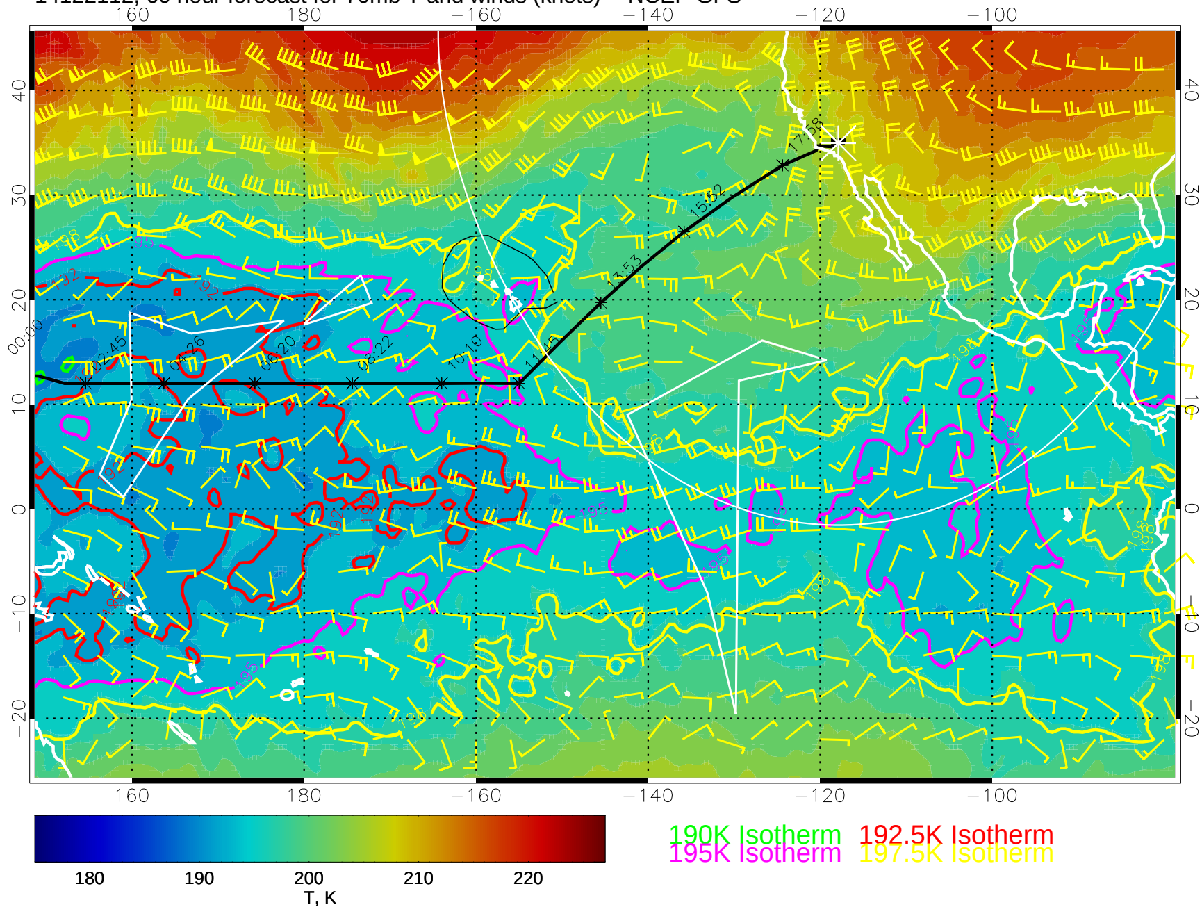
14122112, 60 hour forecast for 70mb T and winds (knots) -- NCEP GFS
