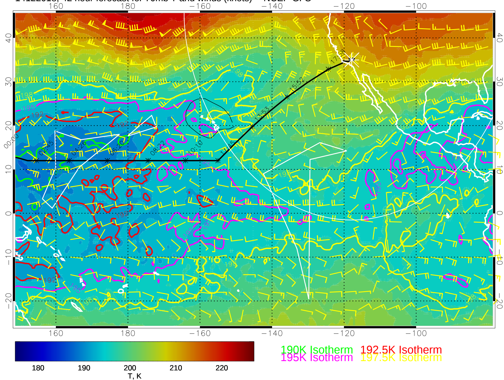
14122018, 42 hour forecast for 70mb T and winds (knots) -- NCEP GFS
