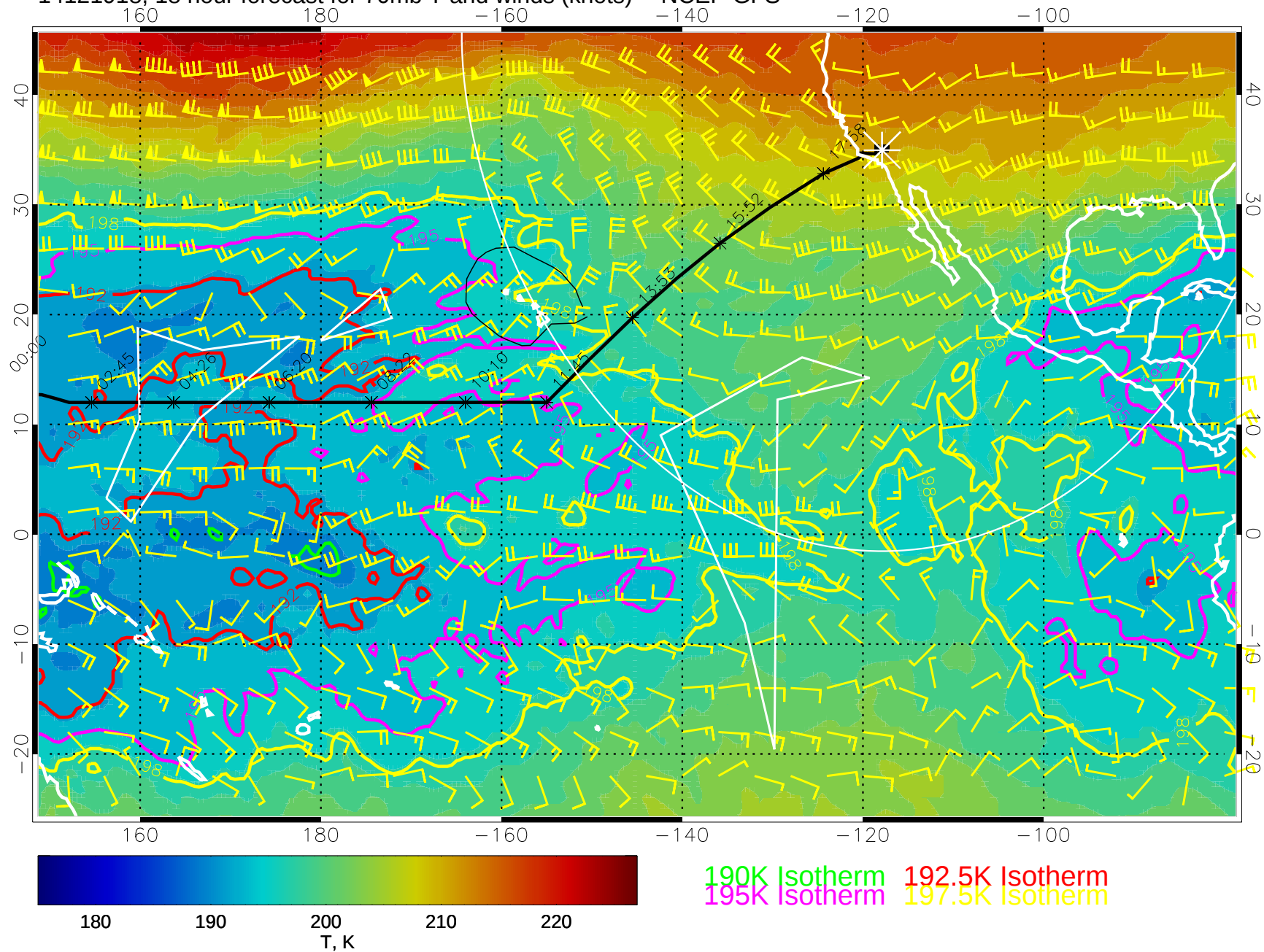
14121918, 18 hour forecast for 70mb T and winds (knots) -- NCEP GFS
