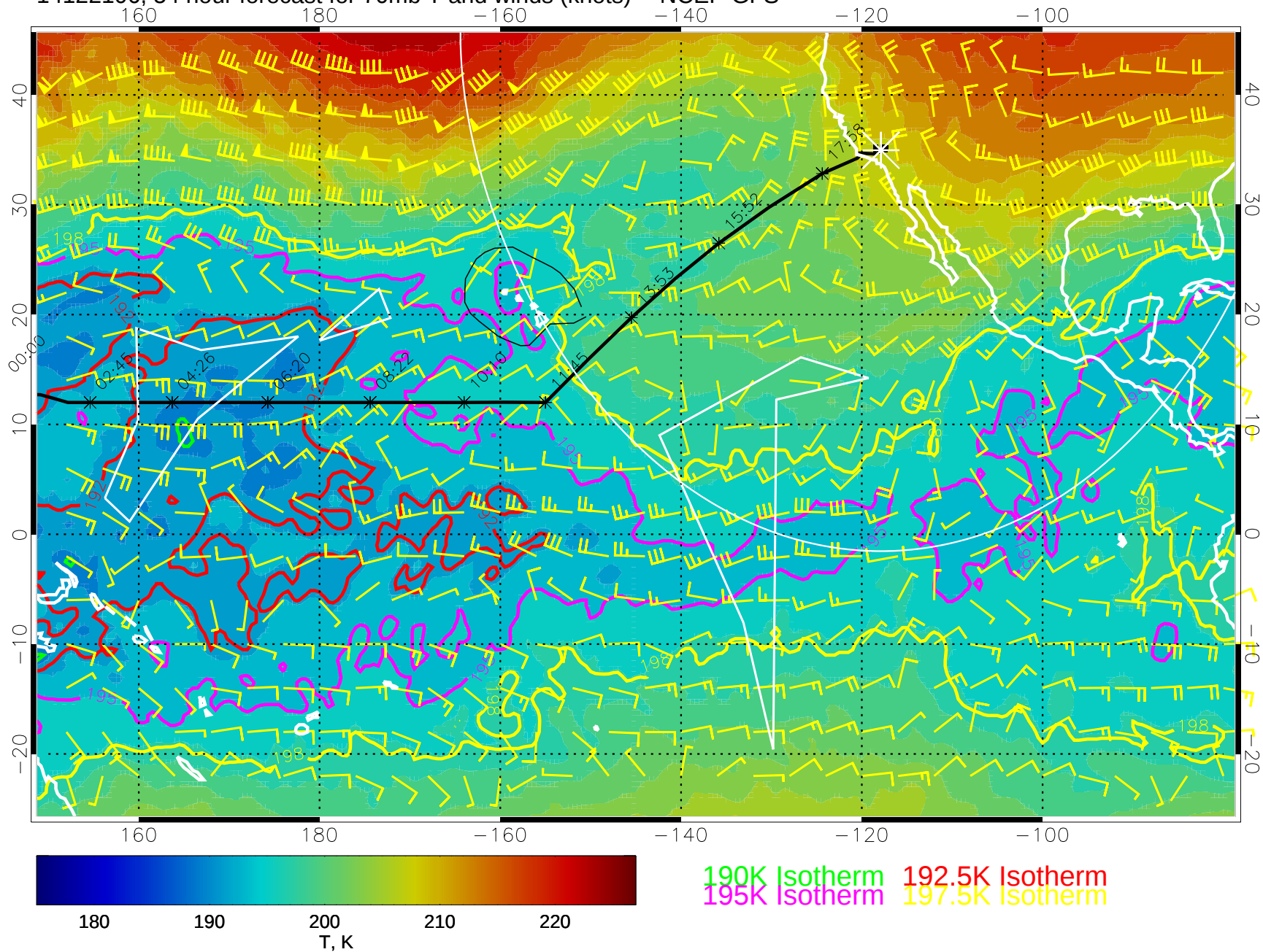
14122106, 54 hour forecast for 70mb T and winds (knots) -- NCEP GFS
