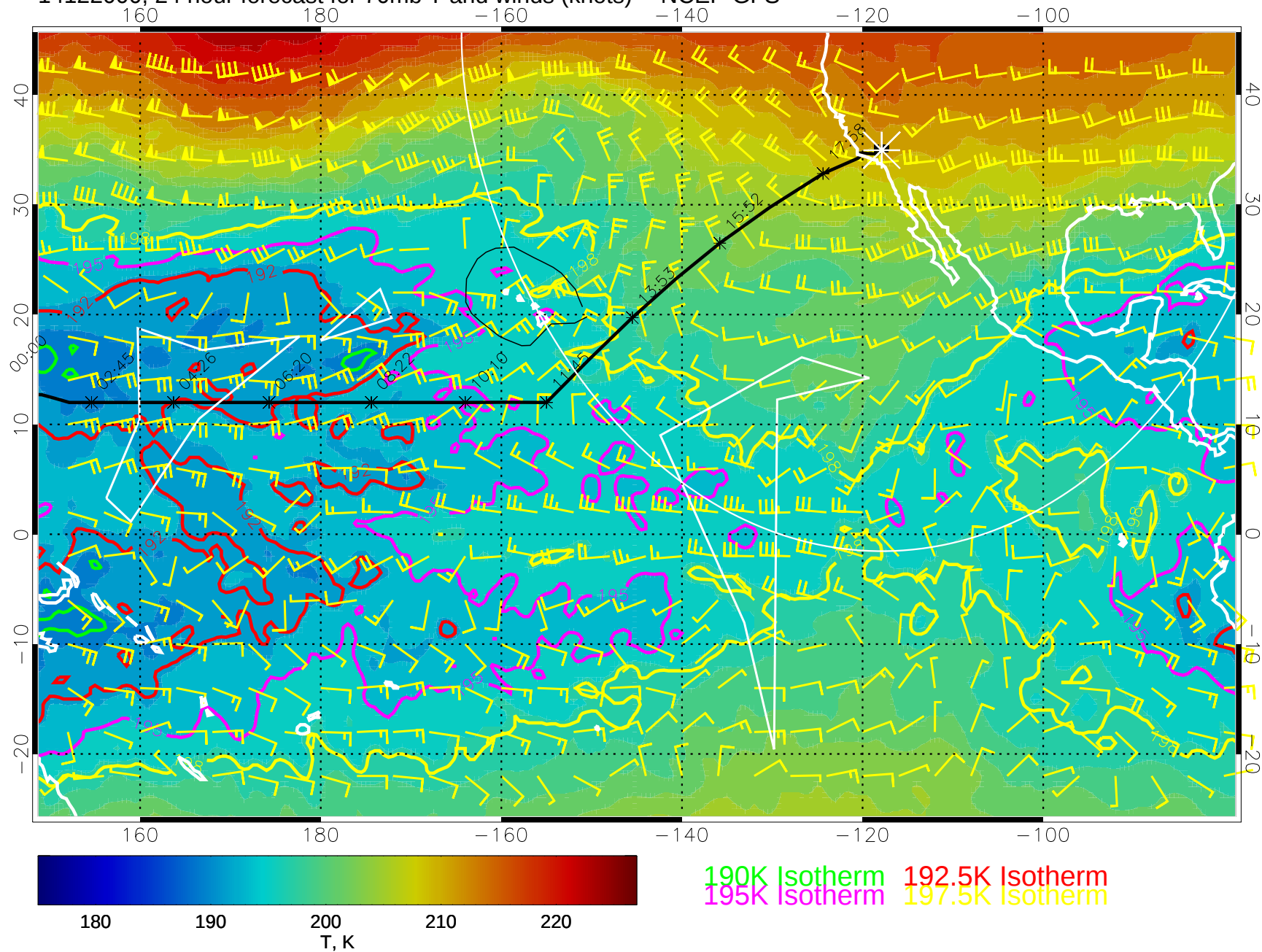
14122000, 24 hour forecast for 70mb T and winds (knots) -- NCEP GFS
