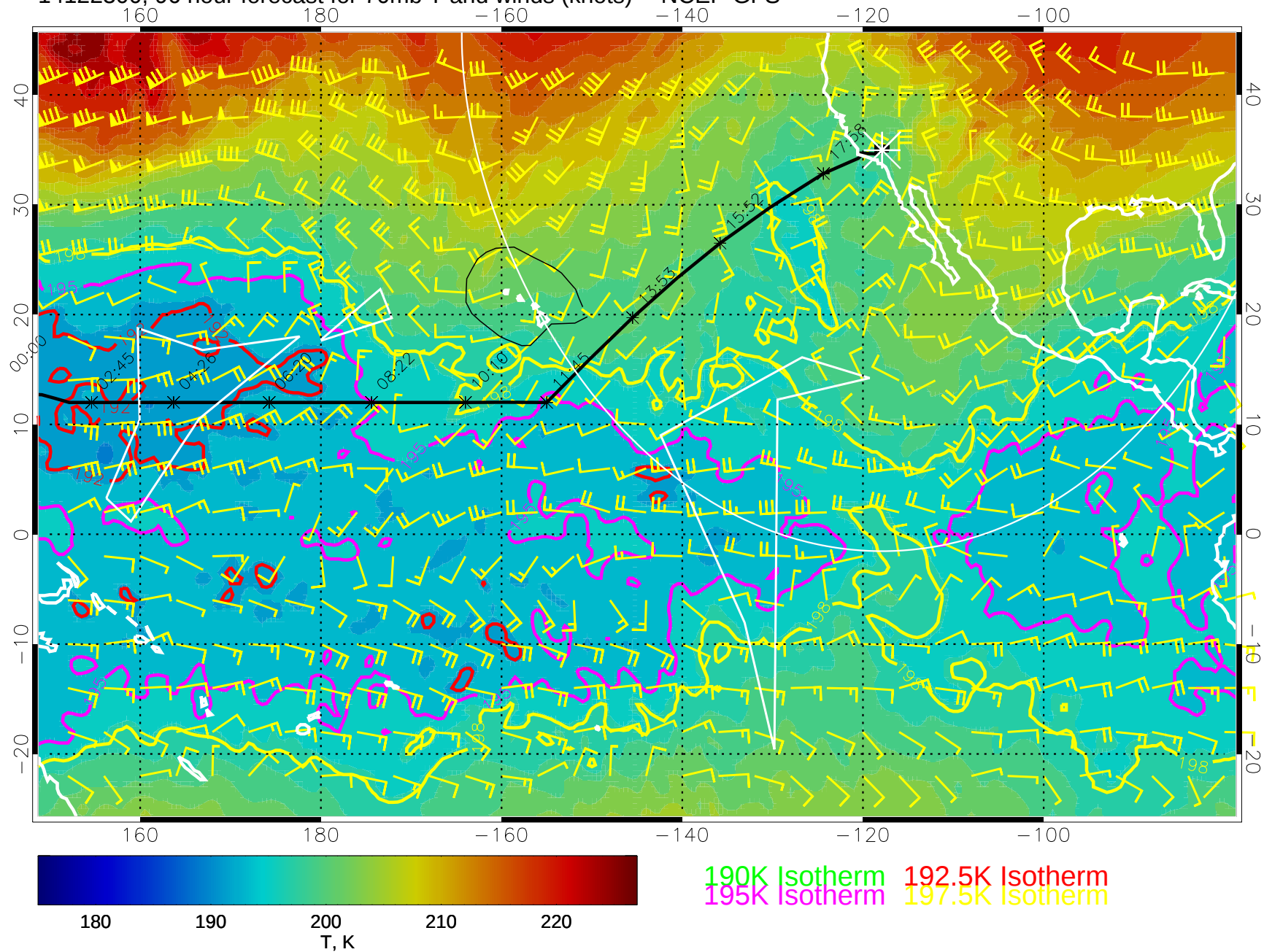
14122300, 96 hour forecast for 70mb T and winds (knots) -- NCEP GFS
