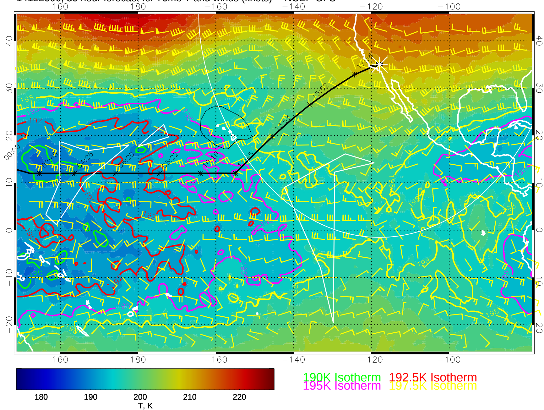
14122006, 30 hour forecast for 70mb T and winds (knots) -- NCEP GFS
