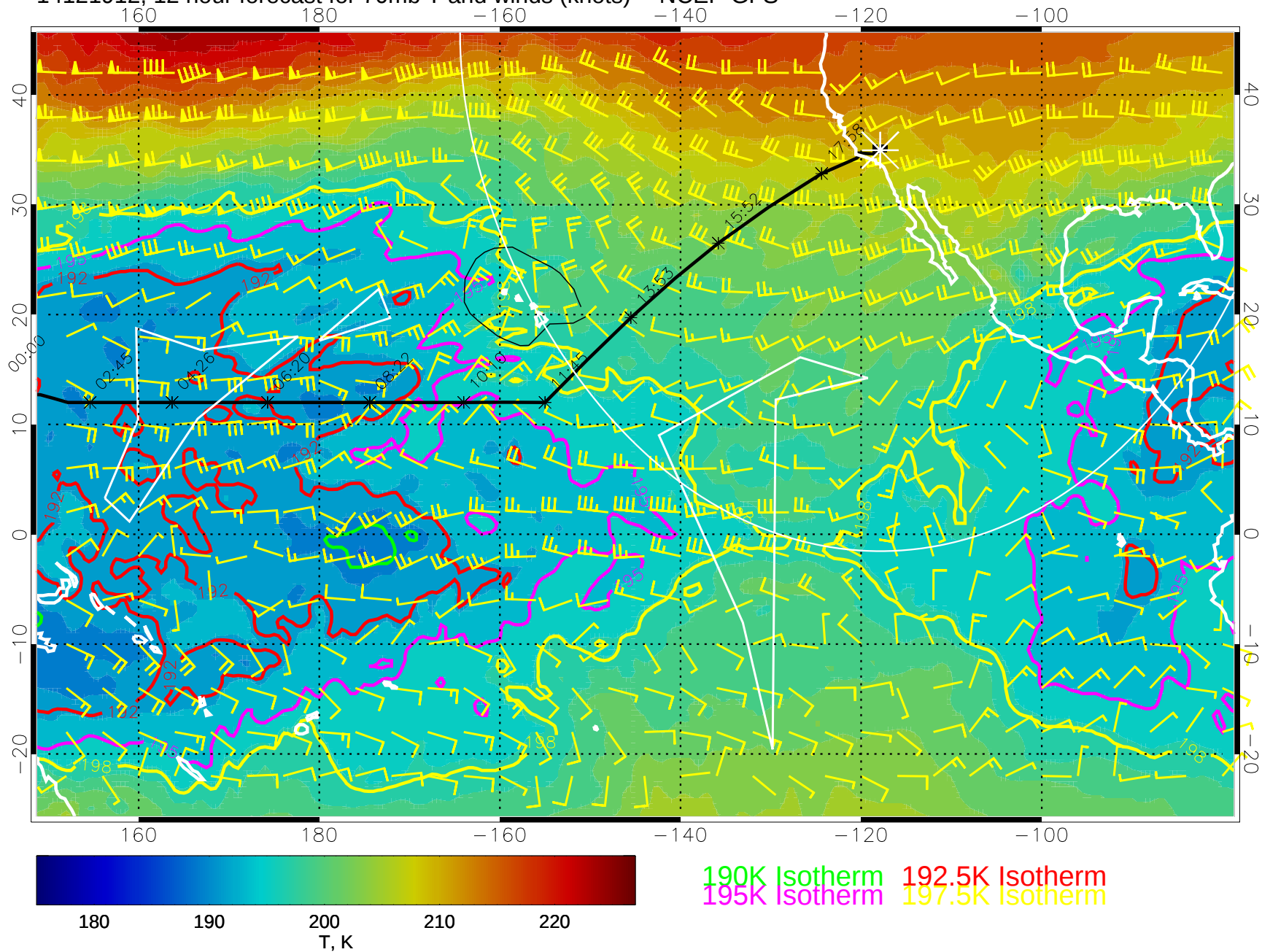
14121912, 12 hour forecast for 70mb T and winds (knots) -- NCEP GFS
