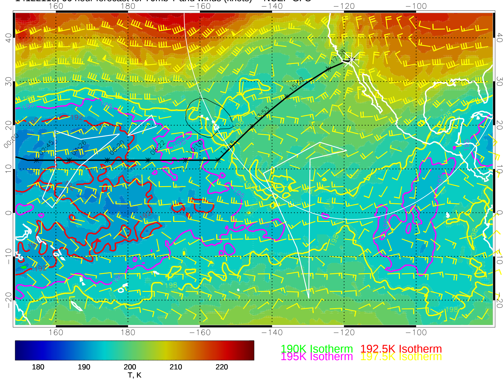
14122118, 66 hour forecast for 70mb T and winds (knots) -- NCEP GFS
