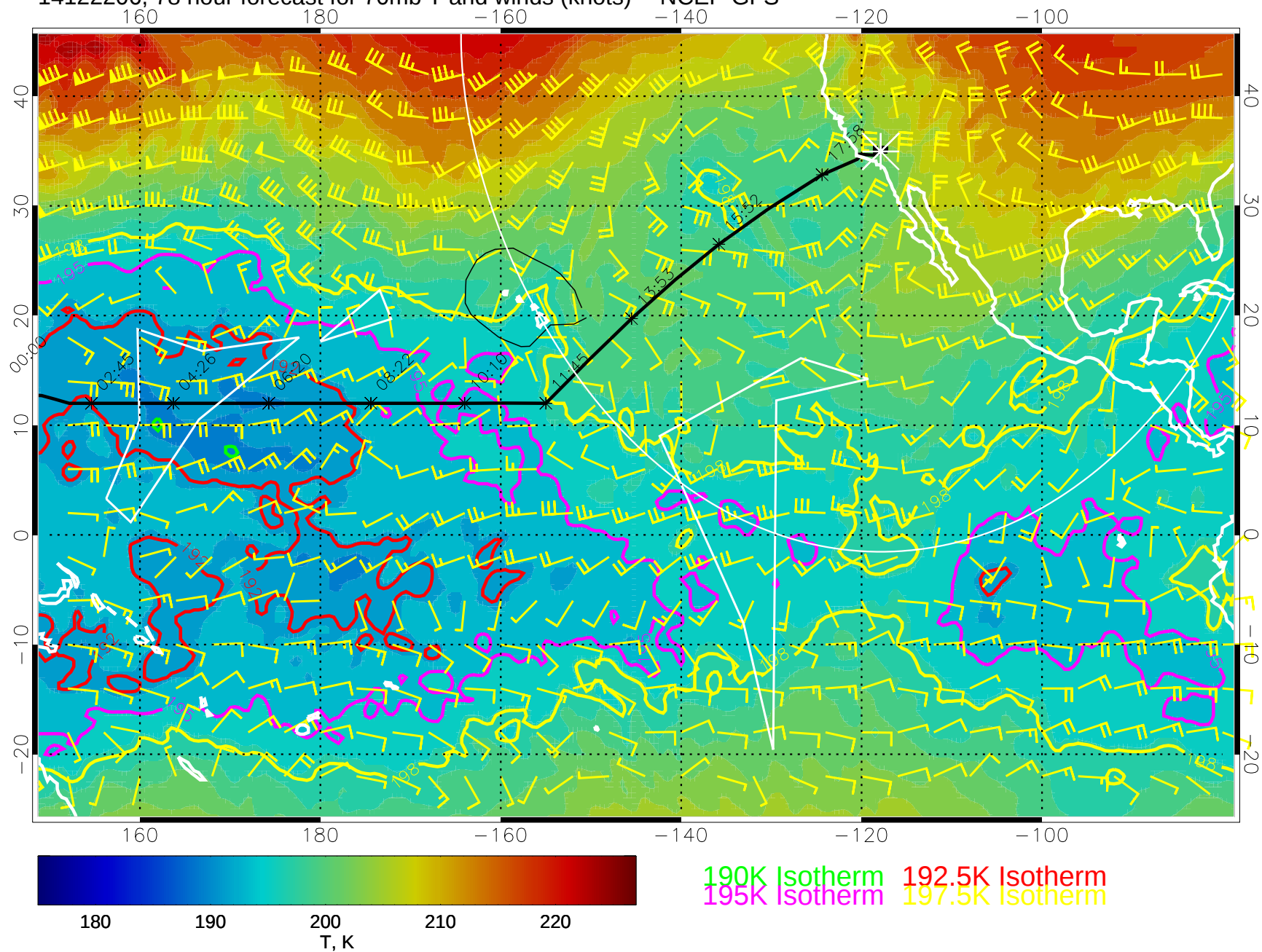
14122206, 78 hour forecast for 70mb T and winds (knots) -- NCEP GFS
