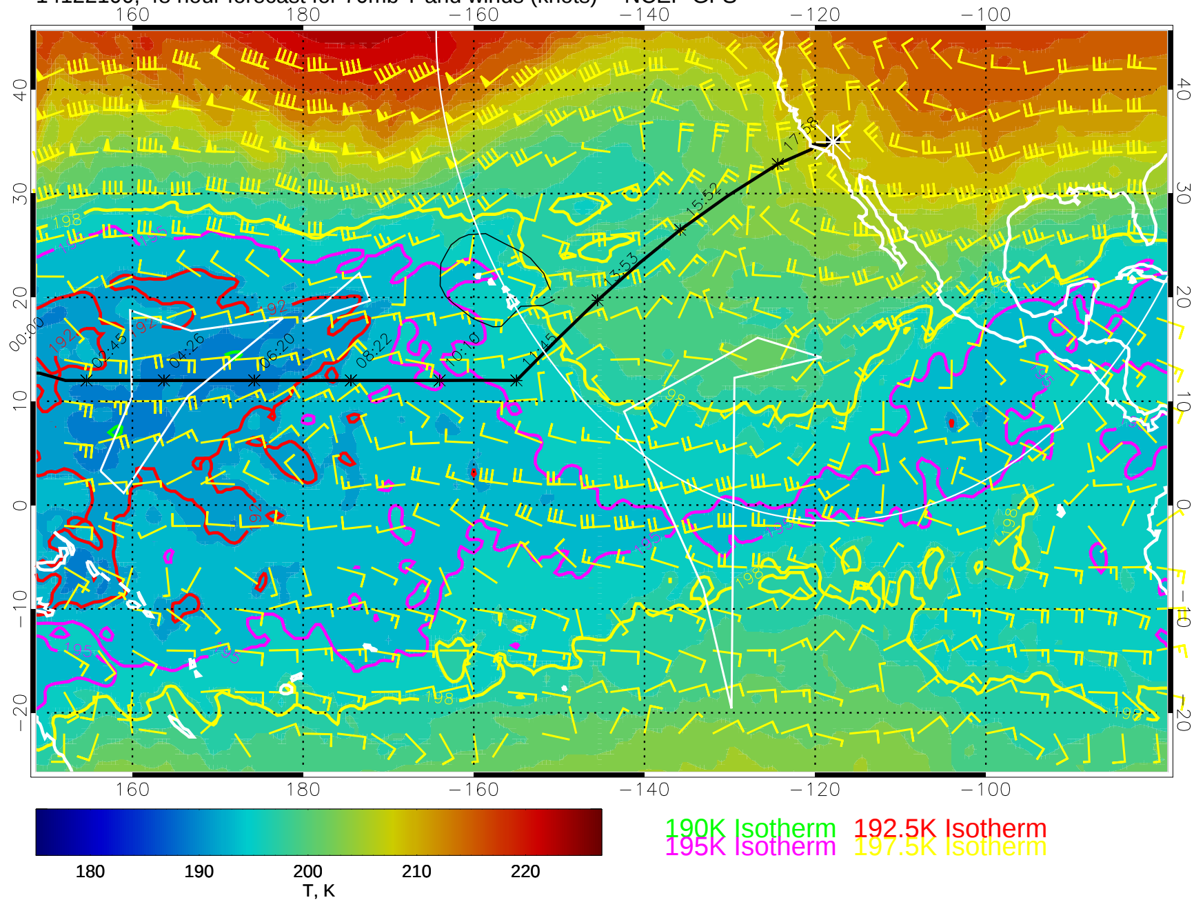
14122100, 48 hour forecast for 70mb T and winds (knots) -- NCEP GFS
