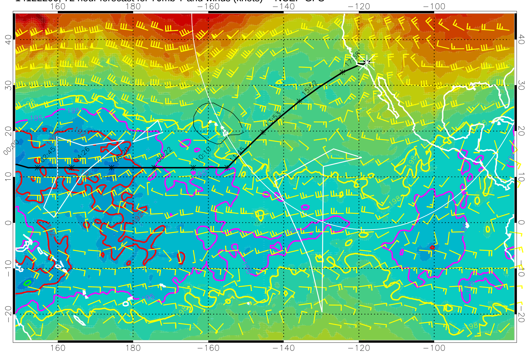
14122200, 72 hour forecast for 70mb T and winds (knots) -- NCEP GFS
