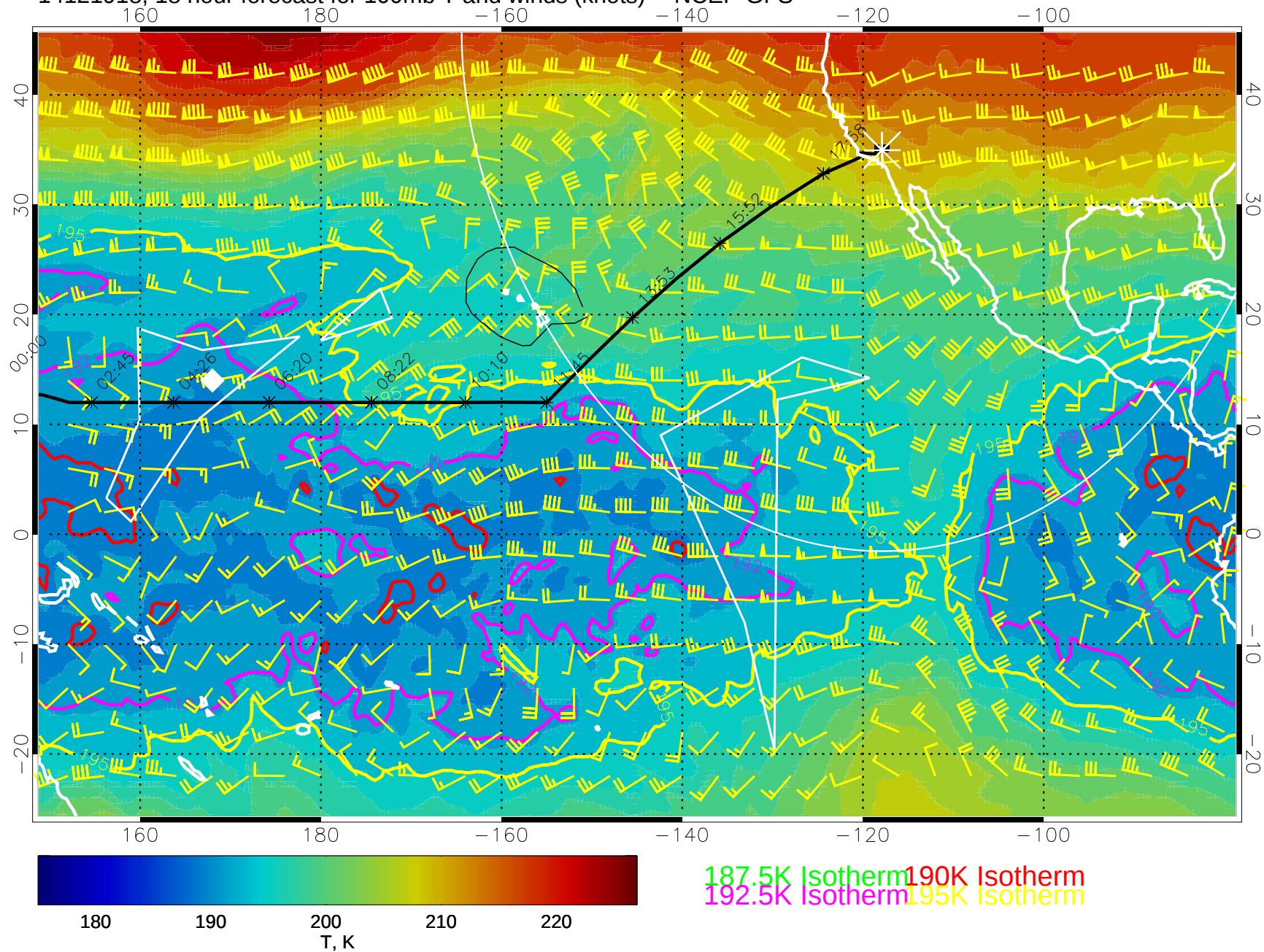
14121918, 18 hour forecast for 100mb T and winds (knots) -- NCEP GFS
