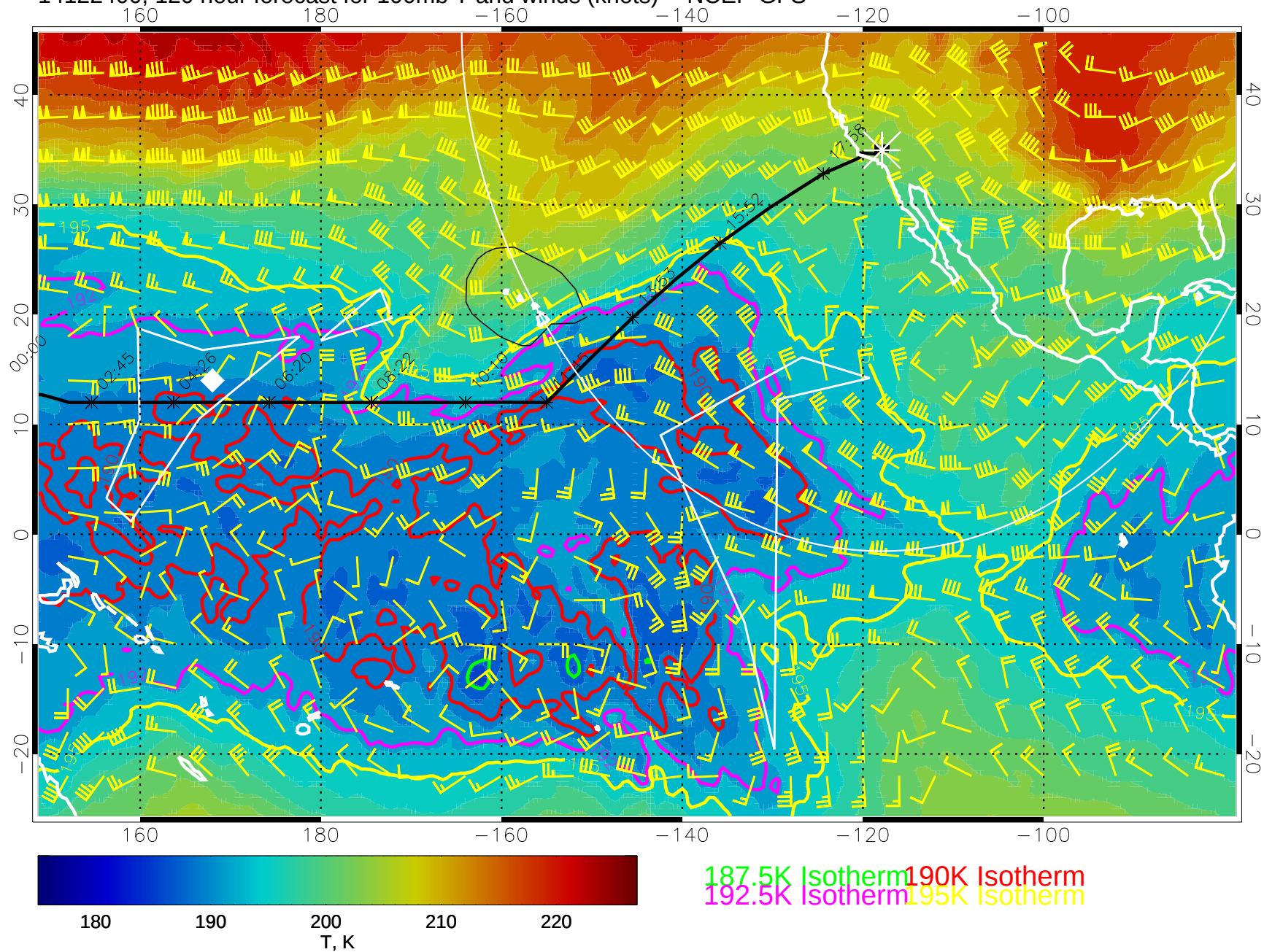
14122400, 120 hour forecast for 100mb T and winds (knots) -- NCEP GFS
