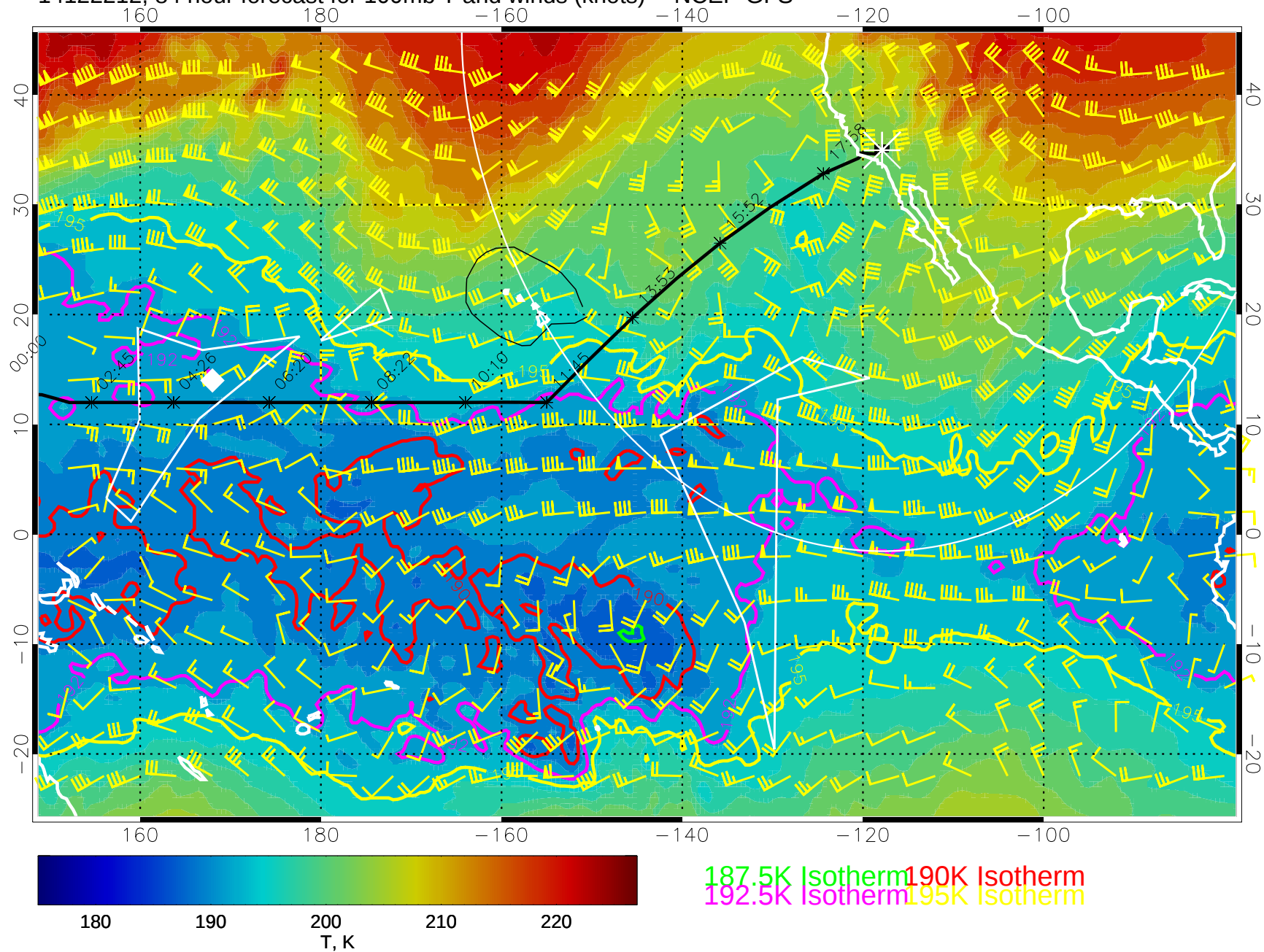
14122212, 84 hour forecast for 100mb T and winds (knots) -- NCEP GFS
