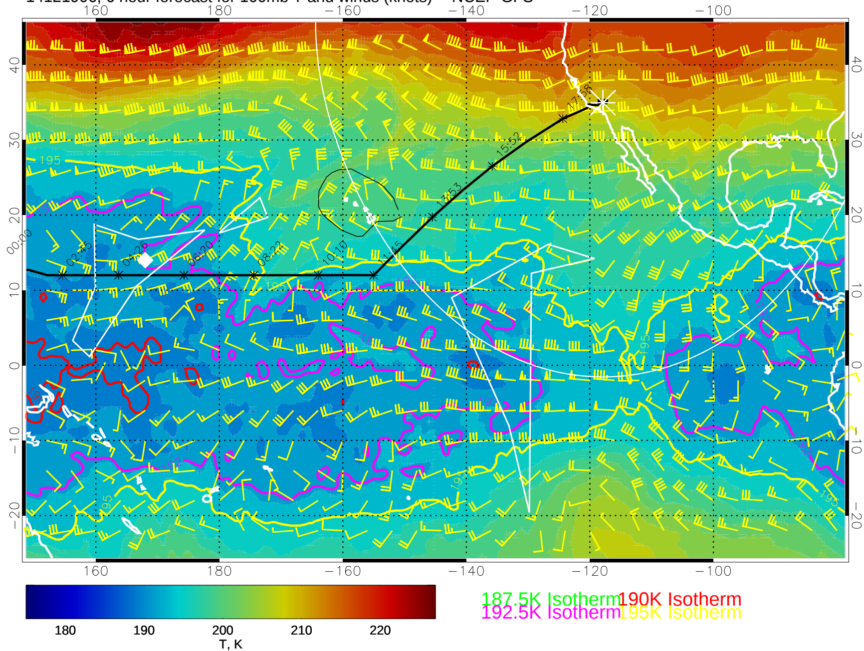
14121906, 6 hour forecast for 100mb T and winds (knots) -- NCEP GFS
