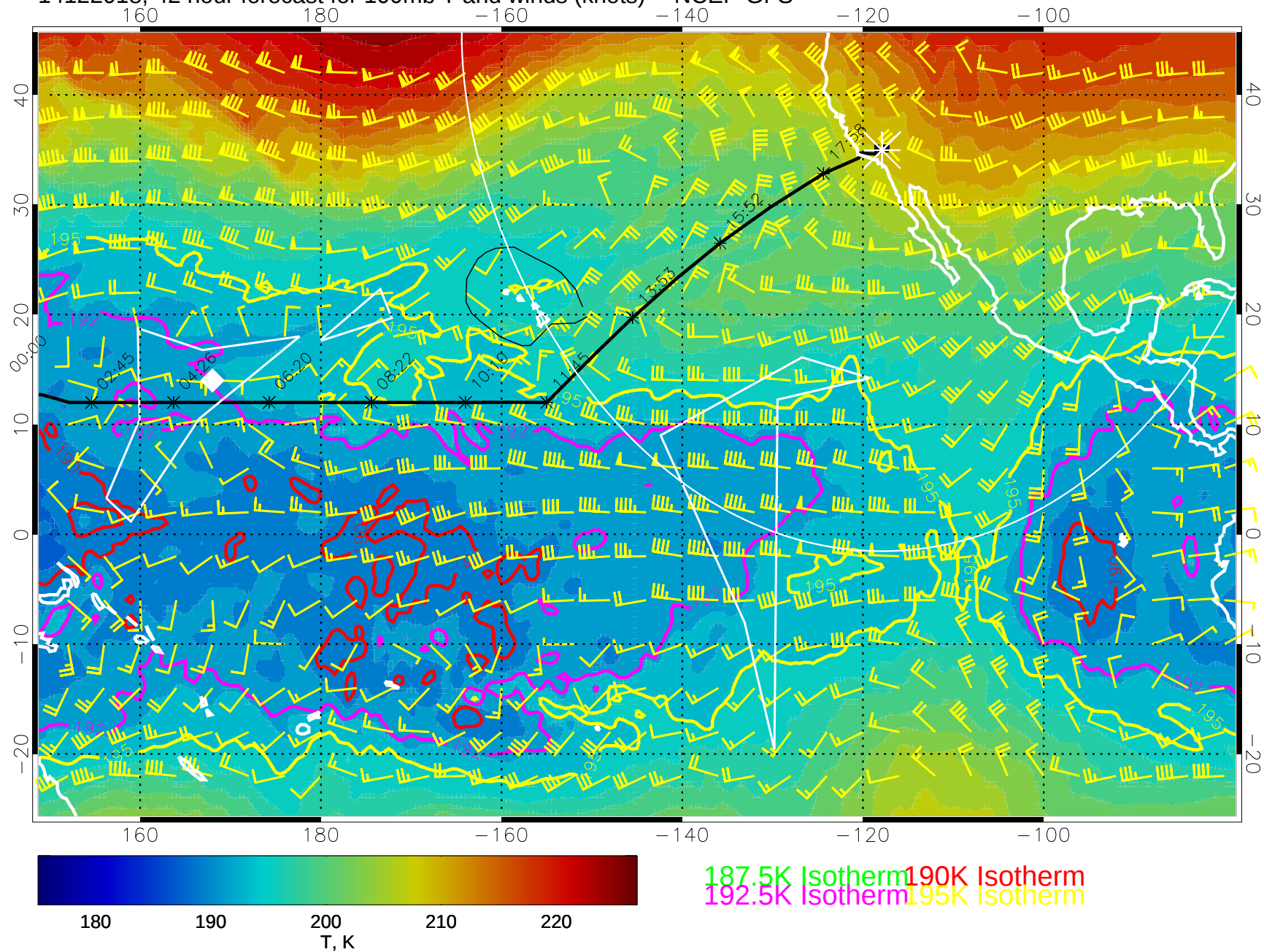
14122018, 42 hour forecast for 100mb T and winds (knots) -- NCEP GFS
