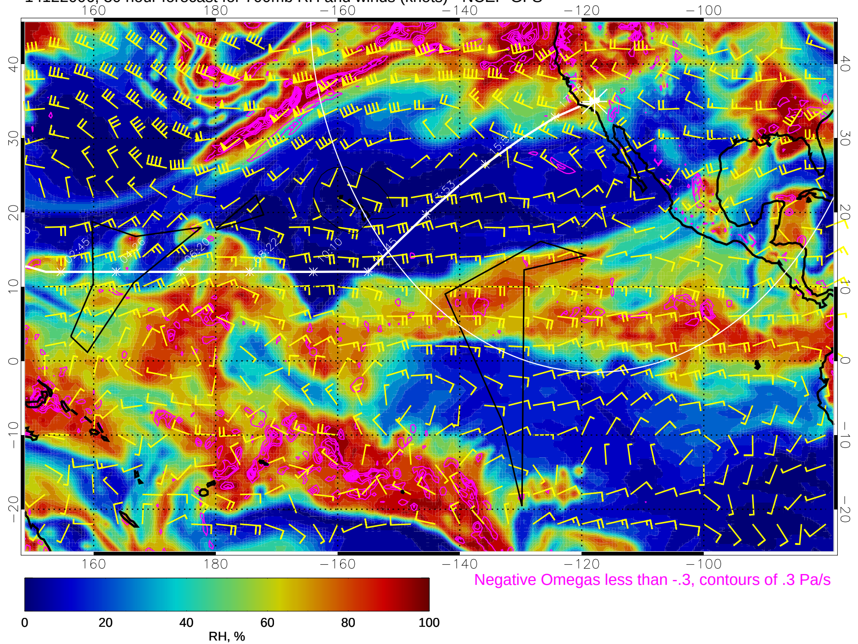
14122006, 30 hour forecast for 700mb RH and winds (knots) - NCEP GFS
