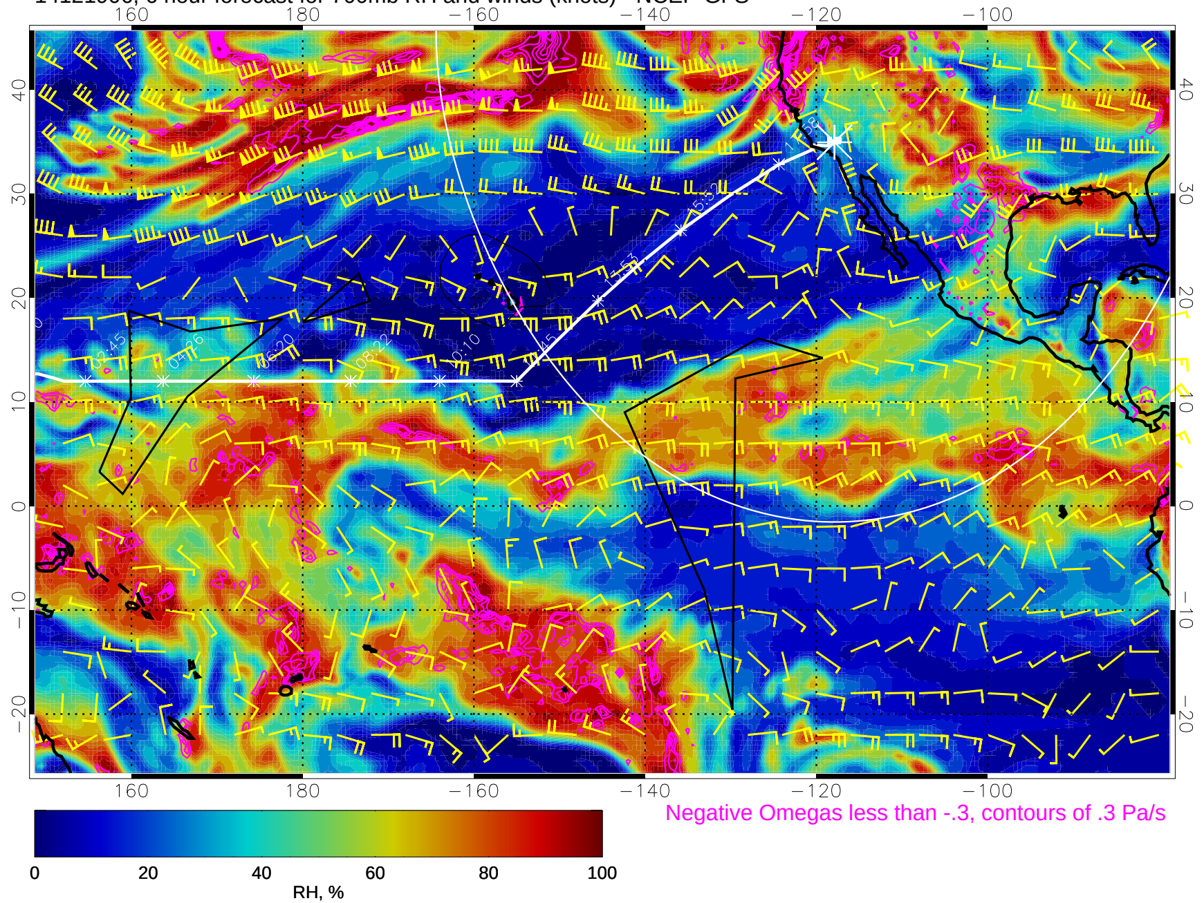
14121906, 6 hour forecast for 700mb RH and winds (knots) - NCEP GFS
