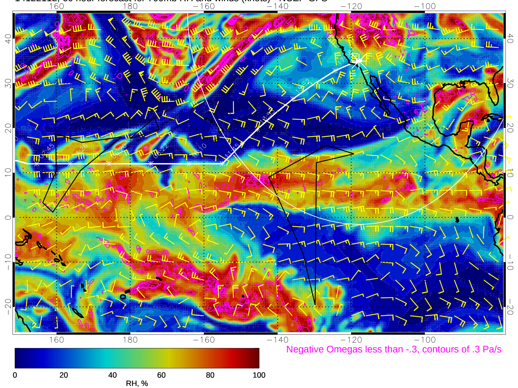
14122112, 60 hour forecast for 700mb RH and winds (knots) - NCEP GFS
