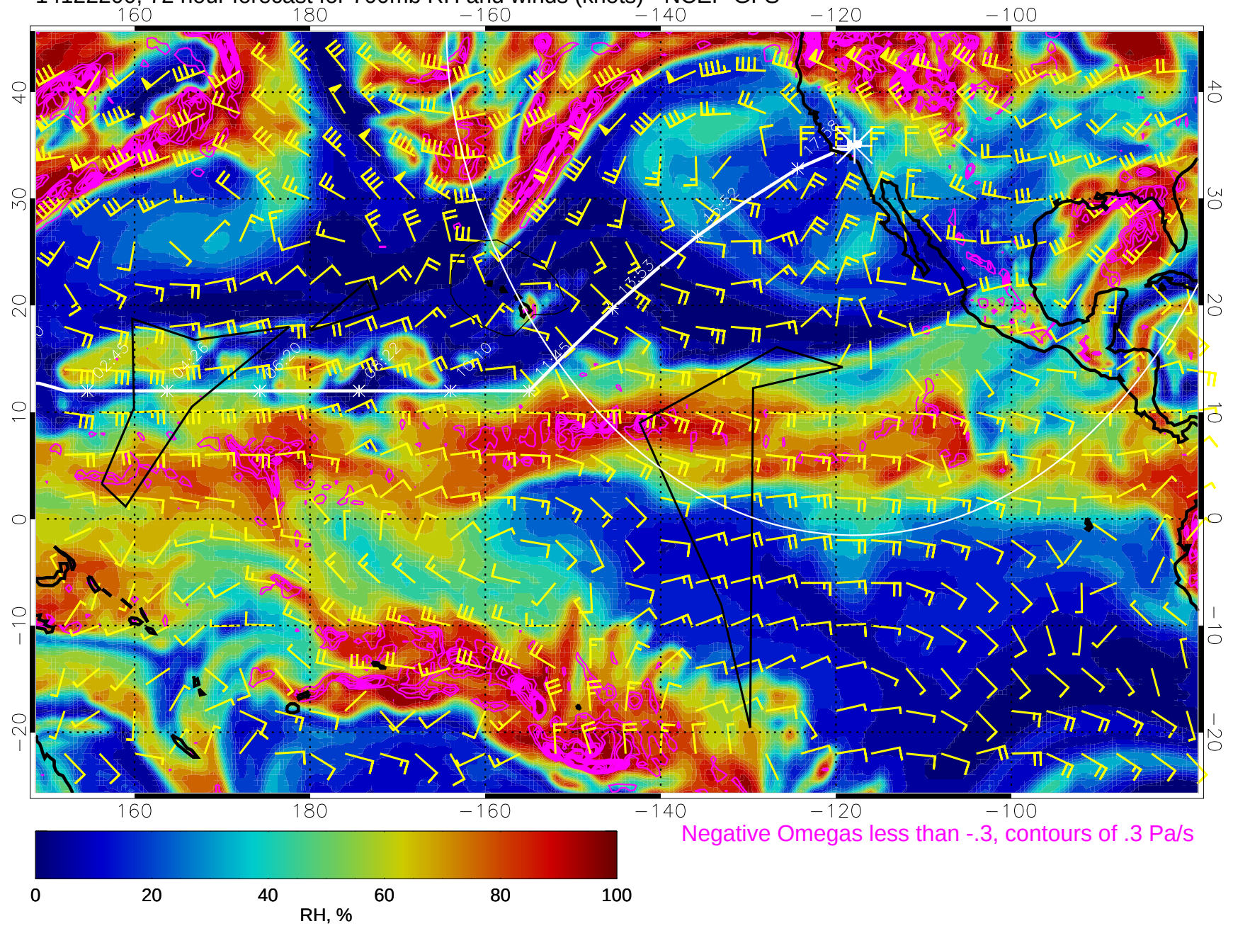
14122200, 72 hour forecast for 700mb RH and winds (knots) - NCEP GFS
