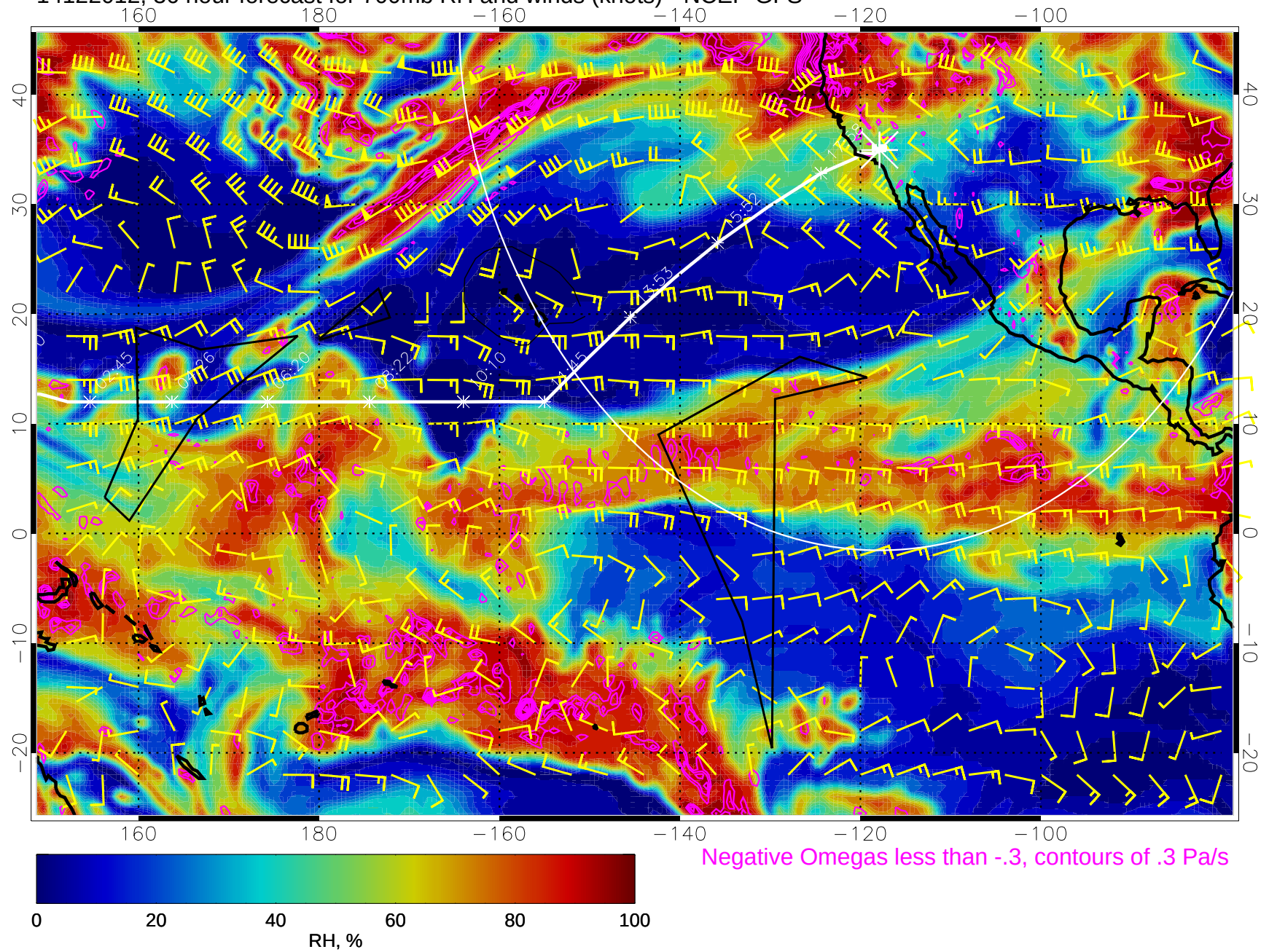
14122012, 36 hour forecast for 700mb RH and winds (knots) - NCEP GFS
