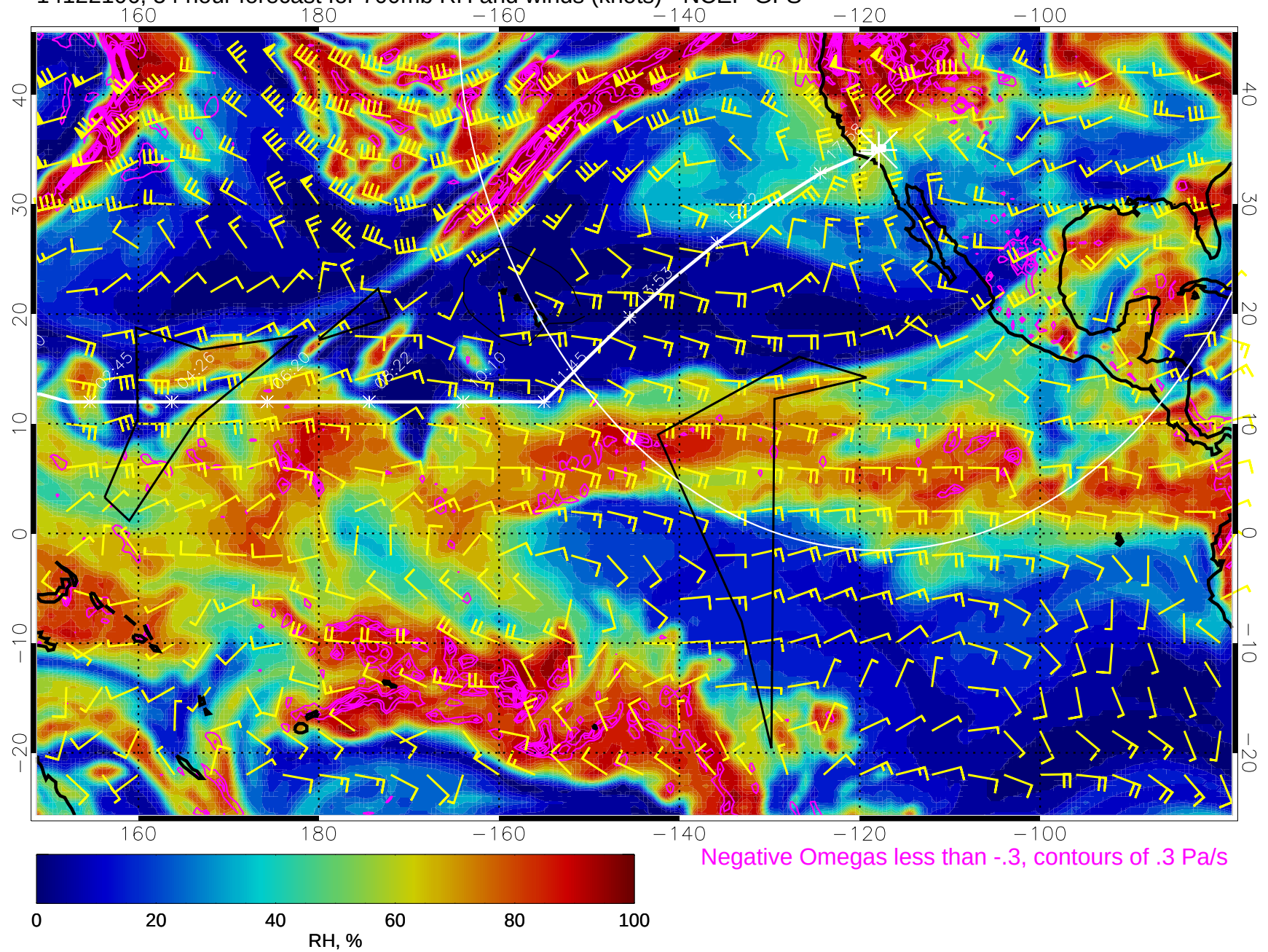
14122106, 54 hour forecast for 700mb RH and winds (knots) - NCEP GFS
