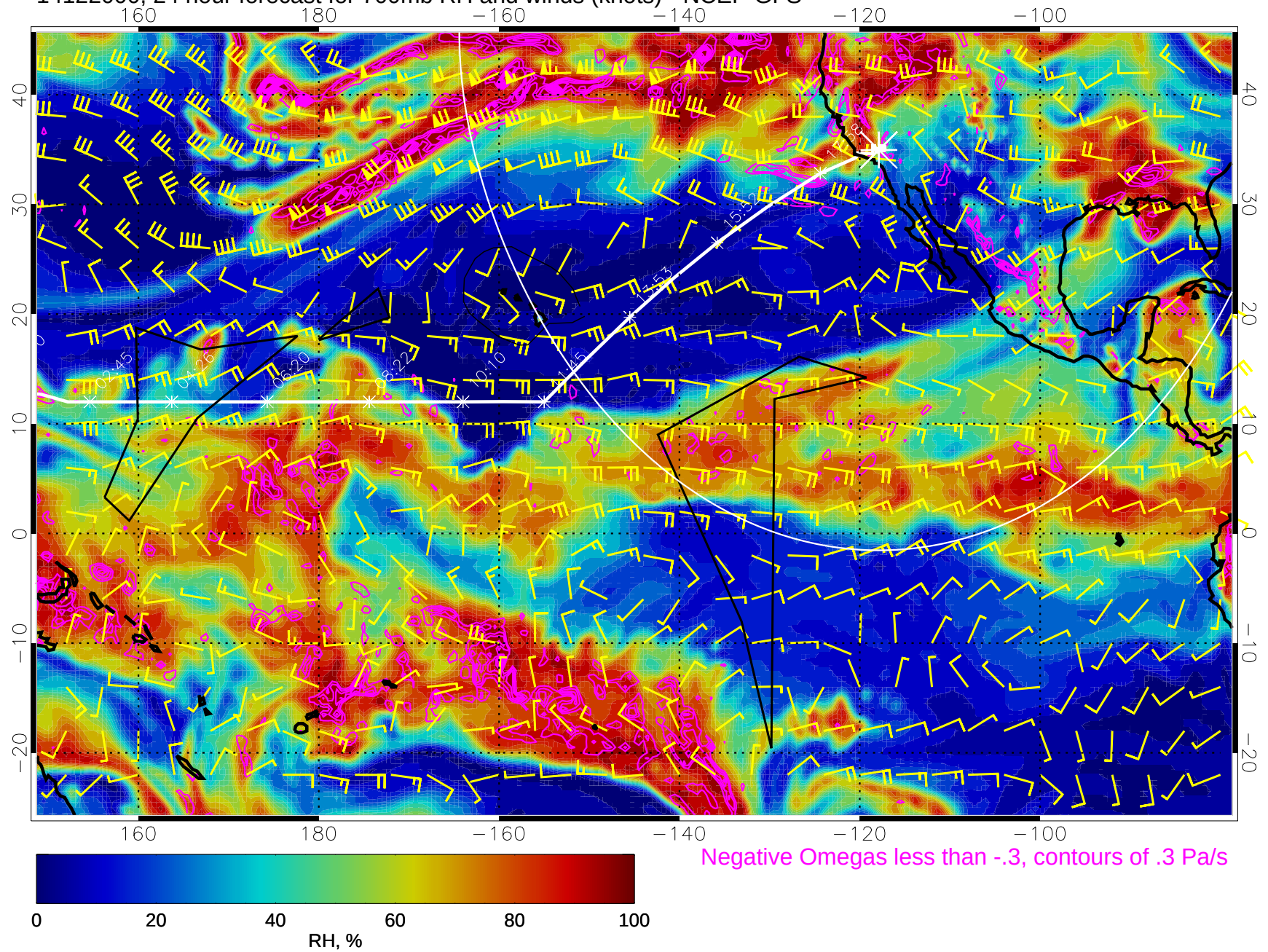
14122000, 24 hour forecast for 700mb RH and winds (knots) - NCEP GFS
