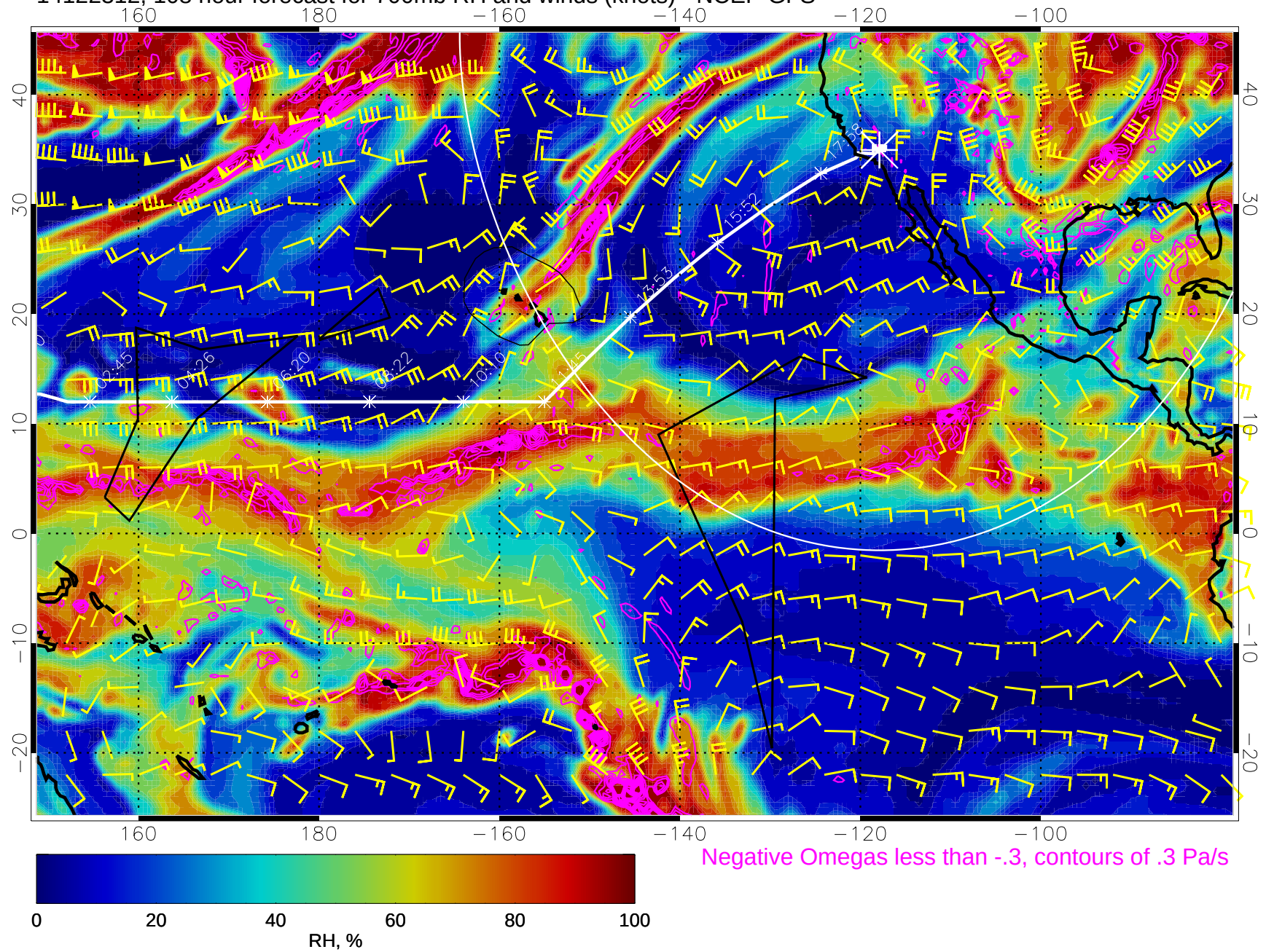
14122312, 108 hour forecast for 700mb RH and winds (knots) - NCEP GFS
