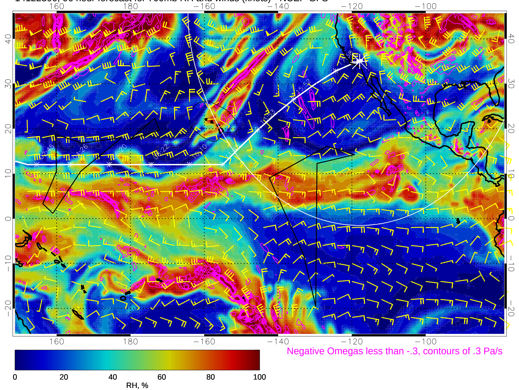
14122300, 96 hour forecast for 700mb RH and winds (knots) - NCEP GFS
