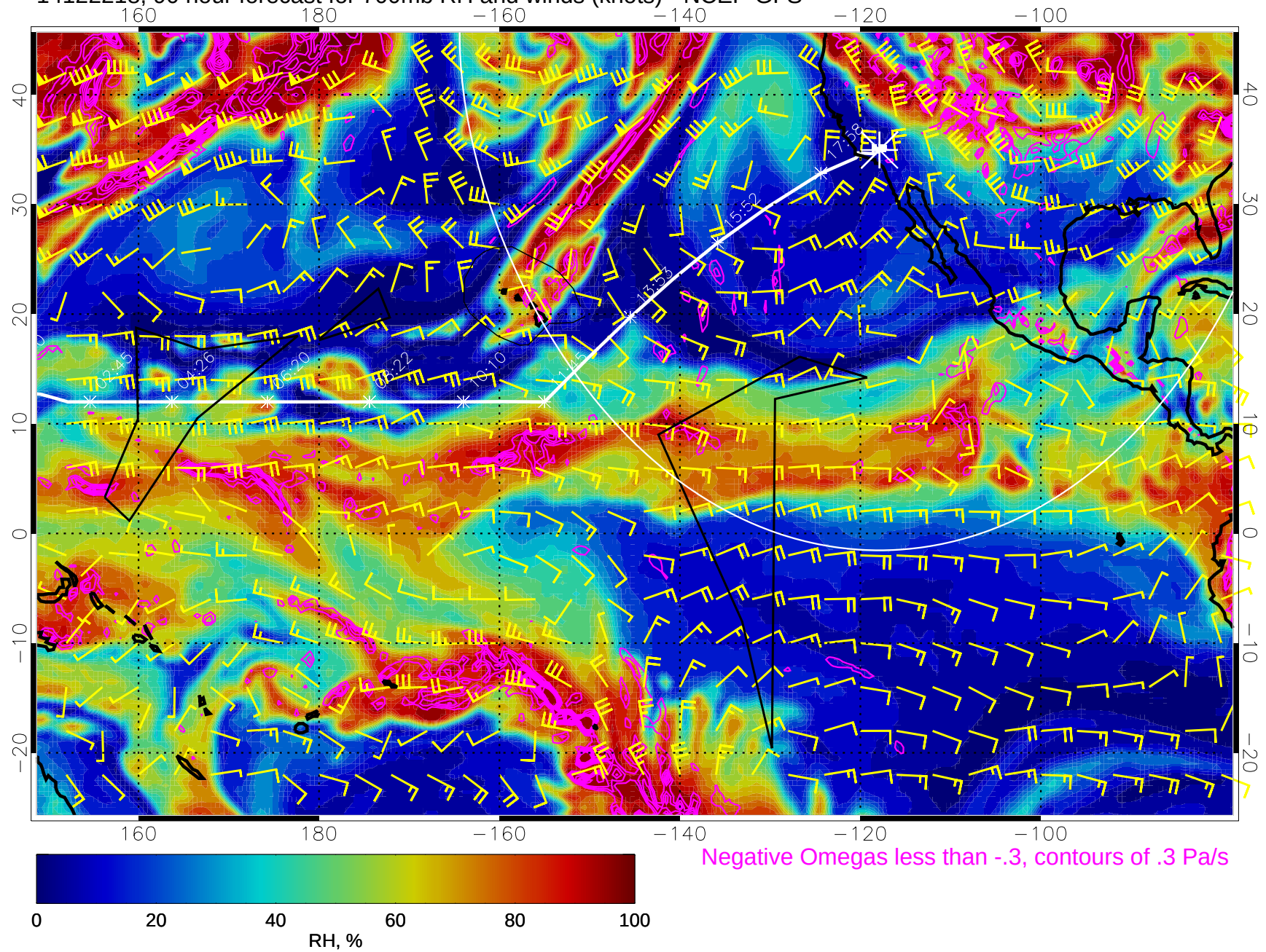
14122218, 90 hour forecast for 700mb RH and winds (knots) - NCEP GFS
