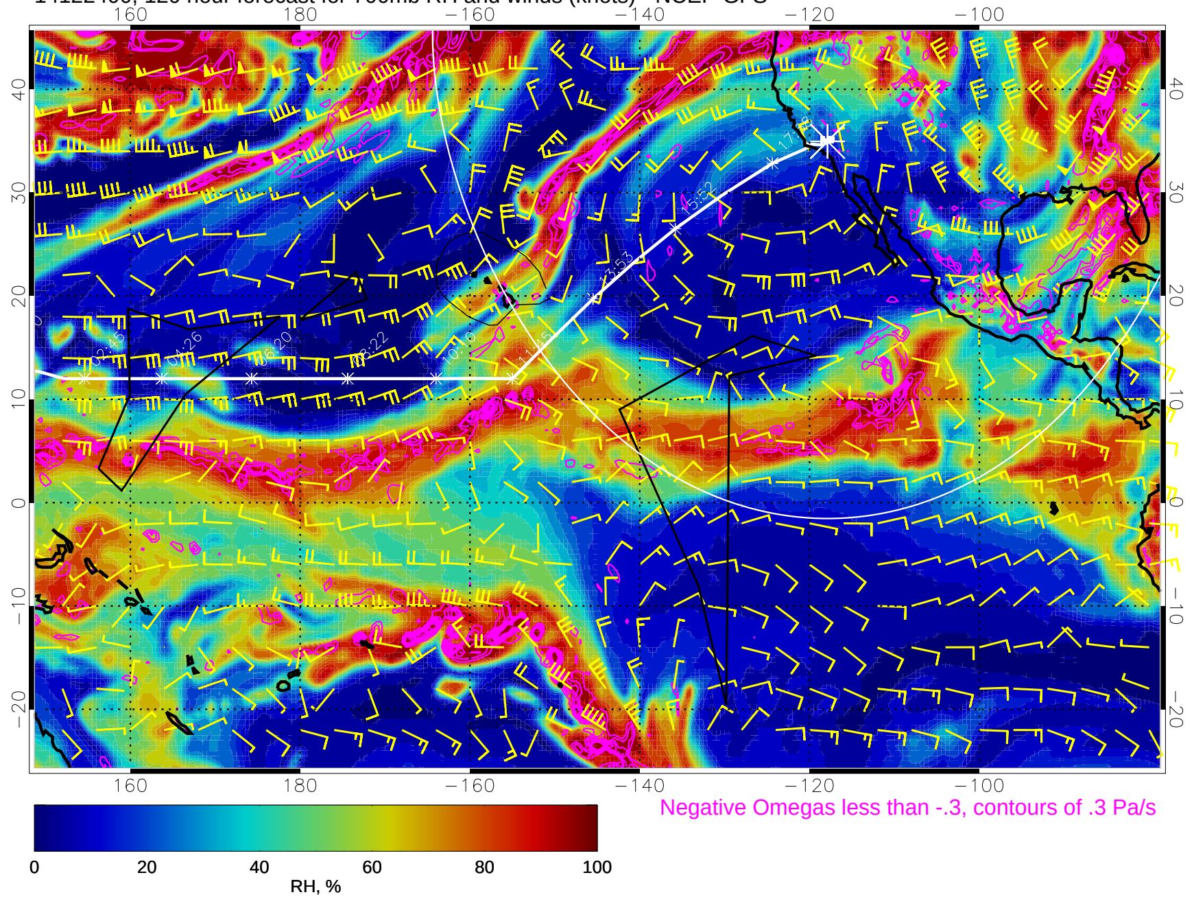
14122400, 120 hour forecast for 700mb RH and winds (knots) - NCEP GFS
