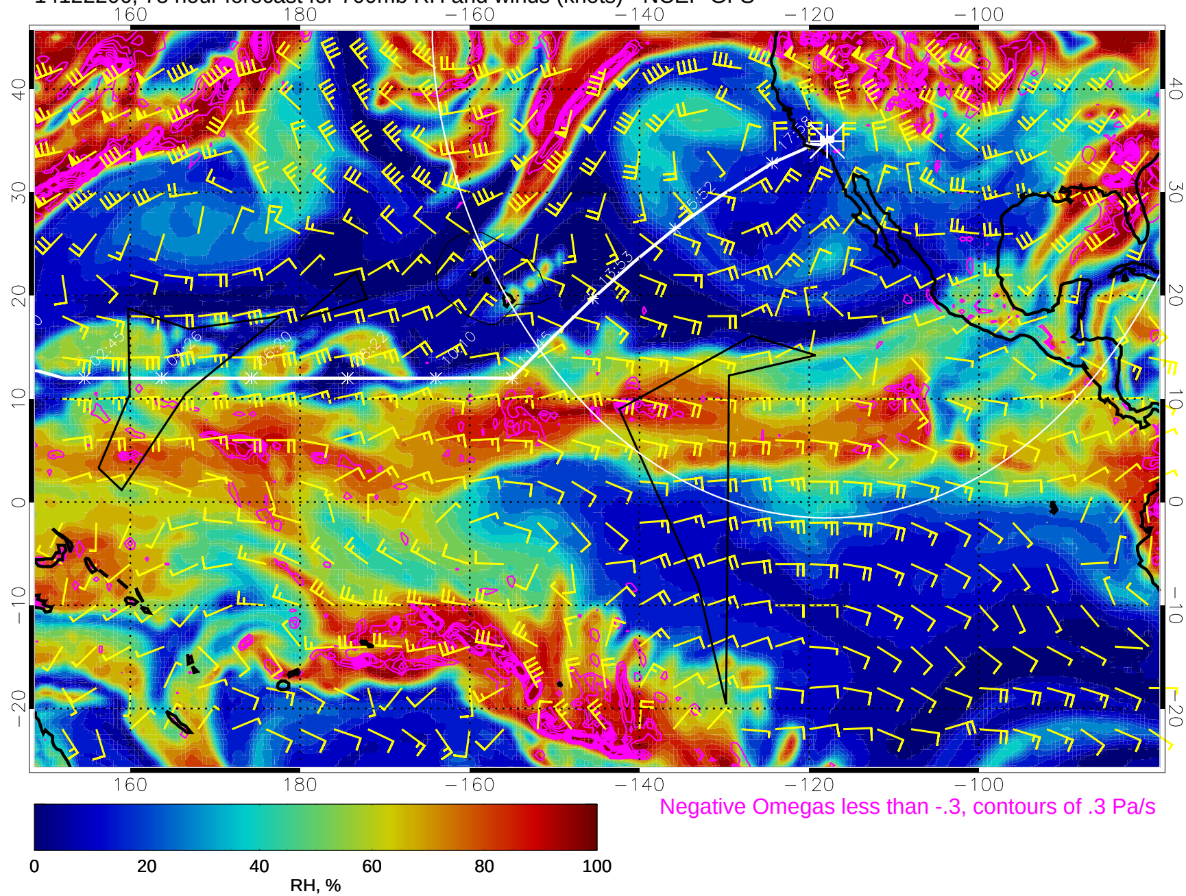
14122206, 78 hour forecast for 700mb RH and winds (knots) - NCEP GFS
