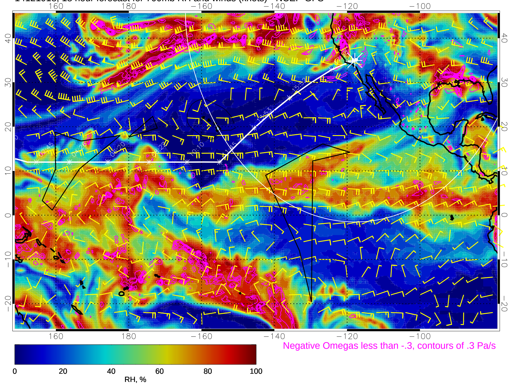
14121918, 18 hour forecast for 700mb RH and winds (knots) - NCEP GFS
