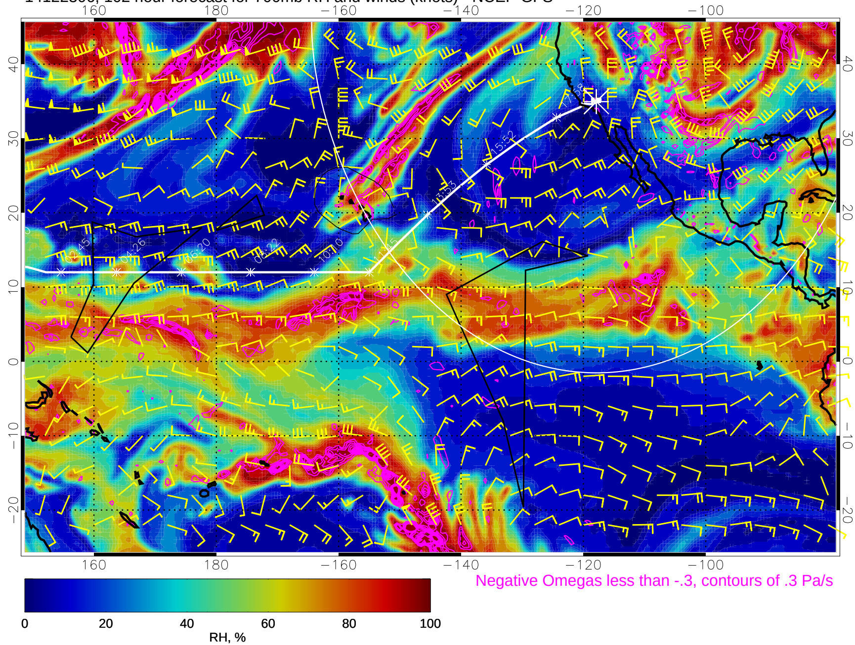
14122306, 102 hour forecast for 700mb RH and winds (knots) - NCEP GFS
