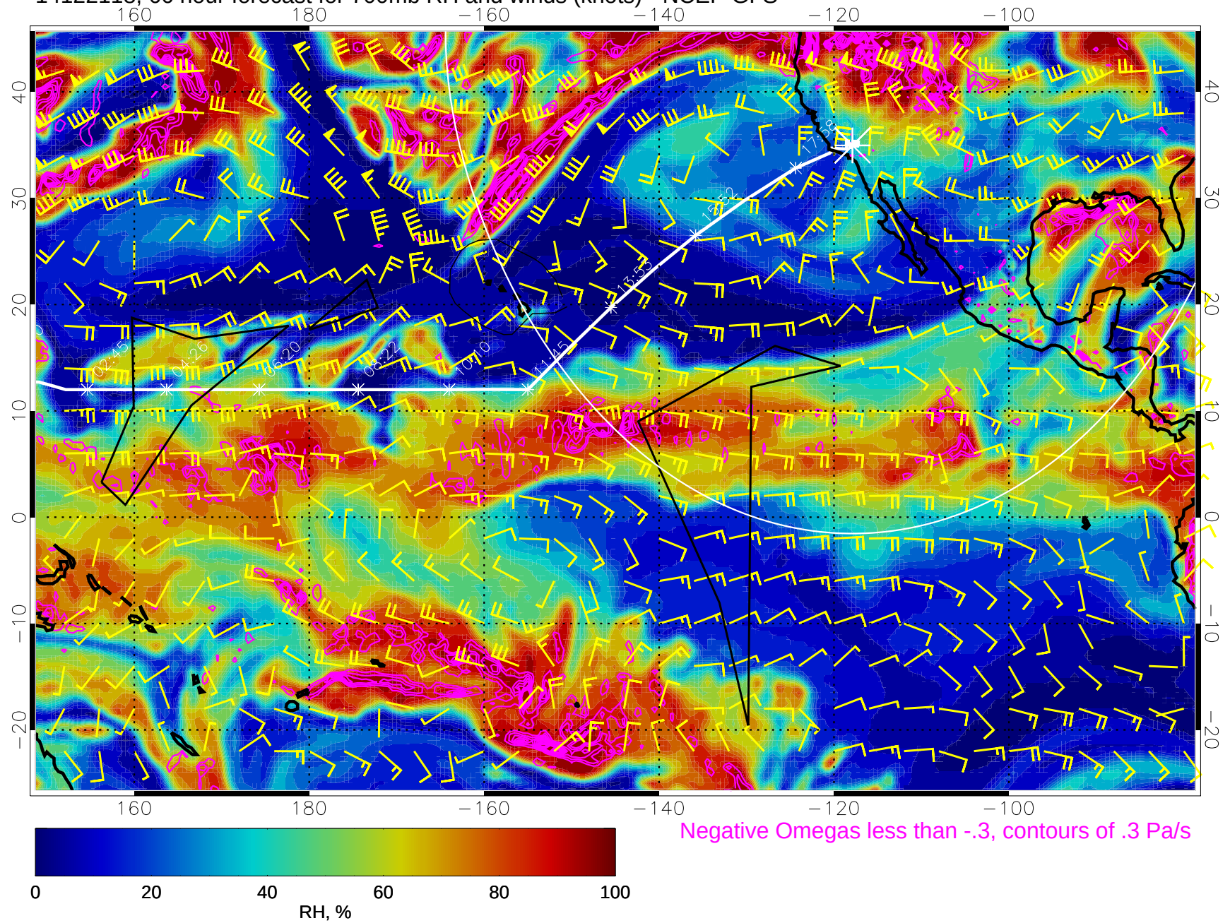
14122118, 66 hour forecast for 700mb RH and winds (knots) - NCEP GFS
