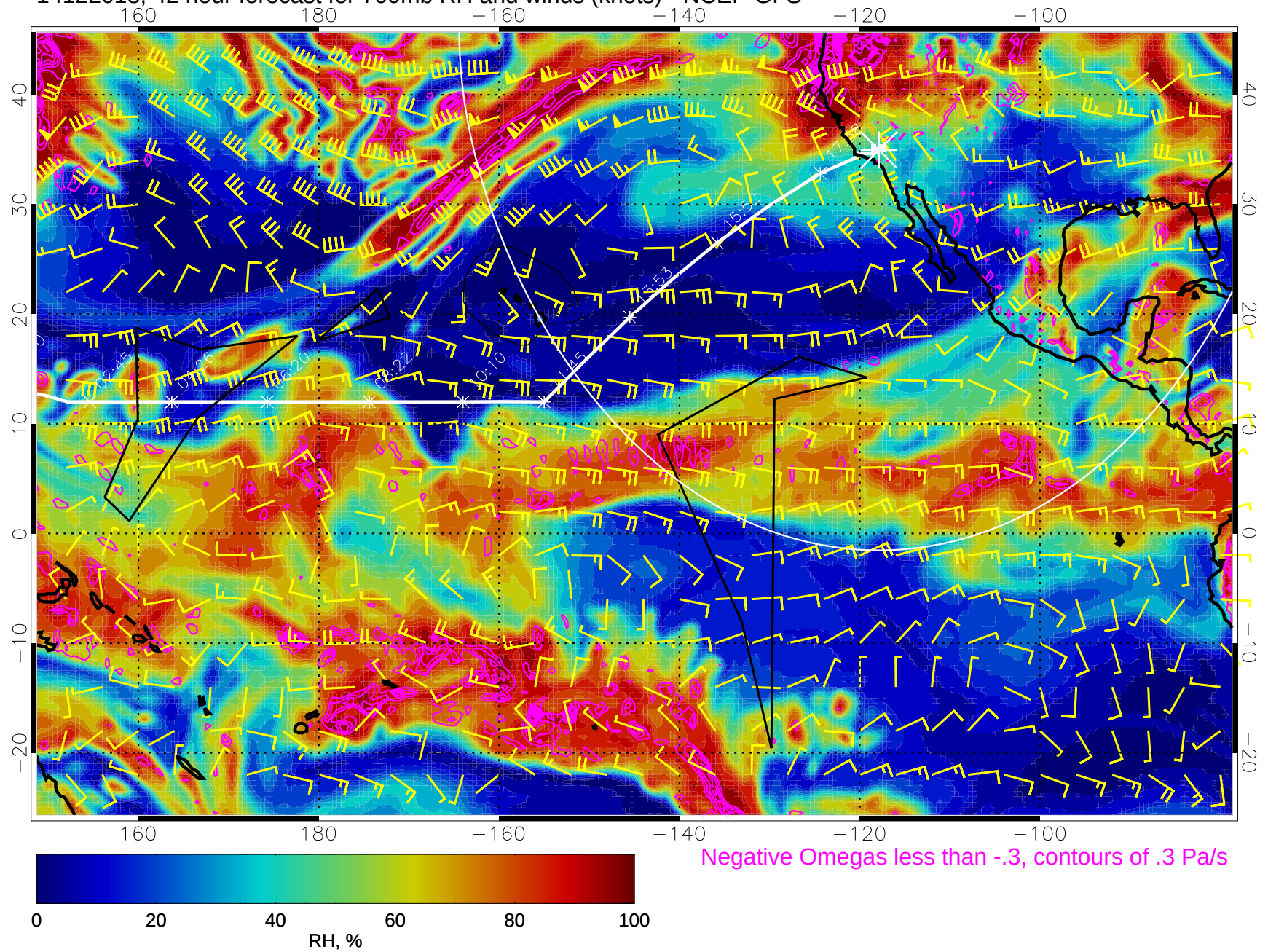
14122018, 42 hour forecast for 700mb RH and winds (knots) - NCEP GFS
