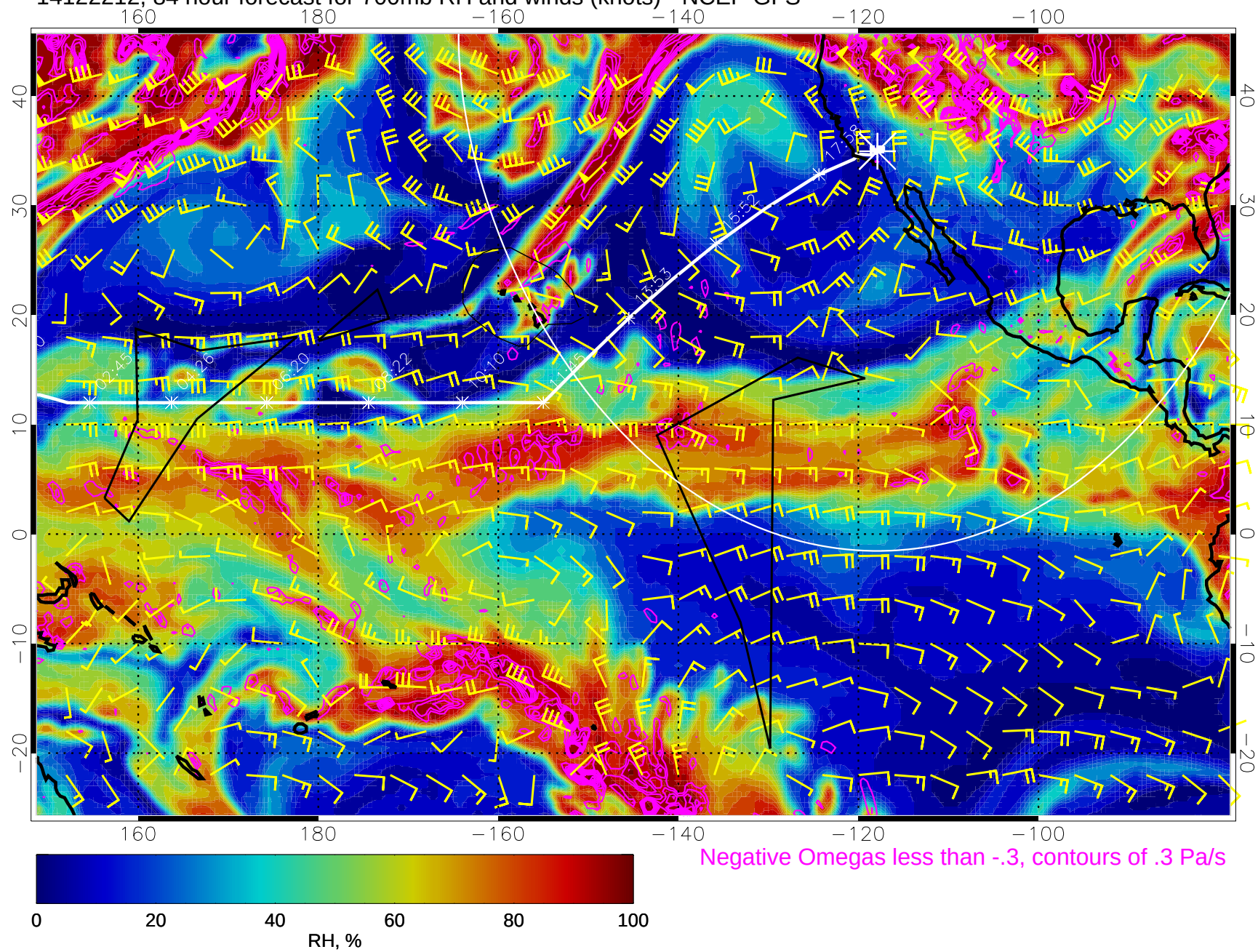
14122212, 84 hour forecast for 700mb RH and winds (knots) - NCEP GFS
