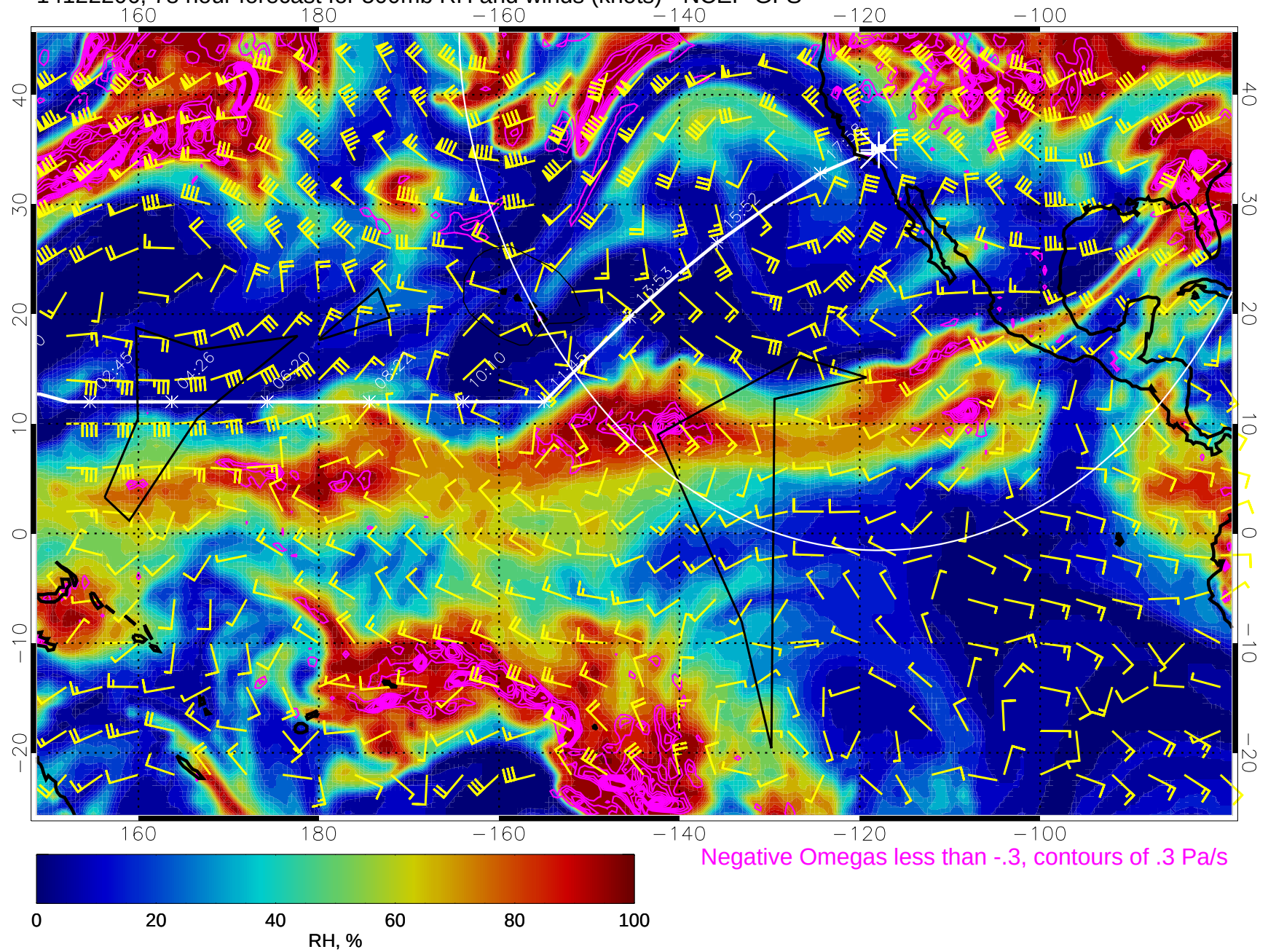
14122206, 78 hour forecast for 500mb RH and winds (knots) - NCEP GFS
