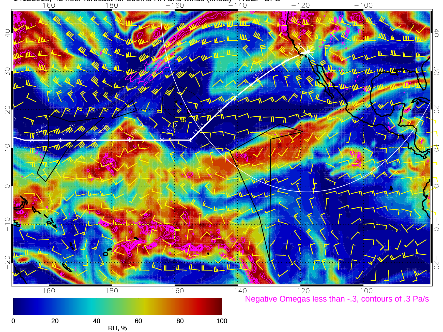
14122018, 42 hour forecast for 500mb RH and winds (knots) - NCEP GFS
