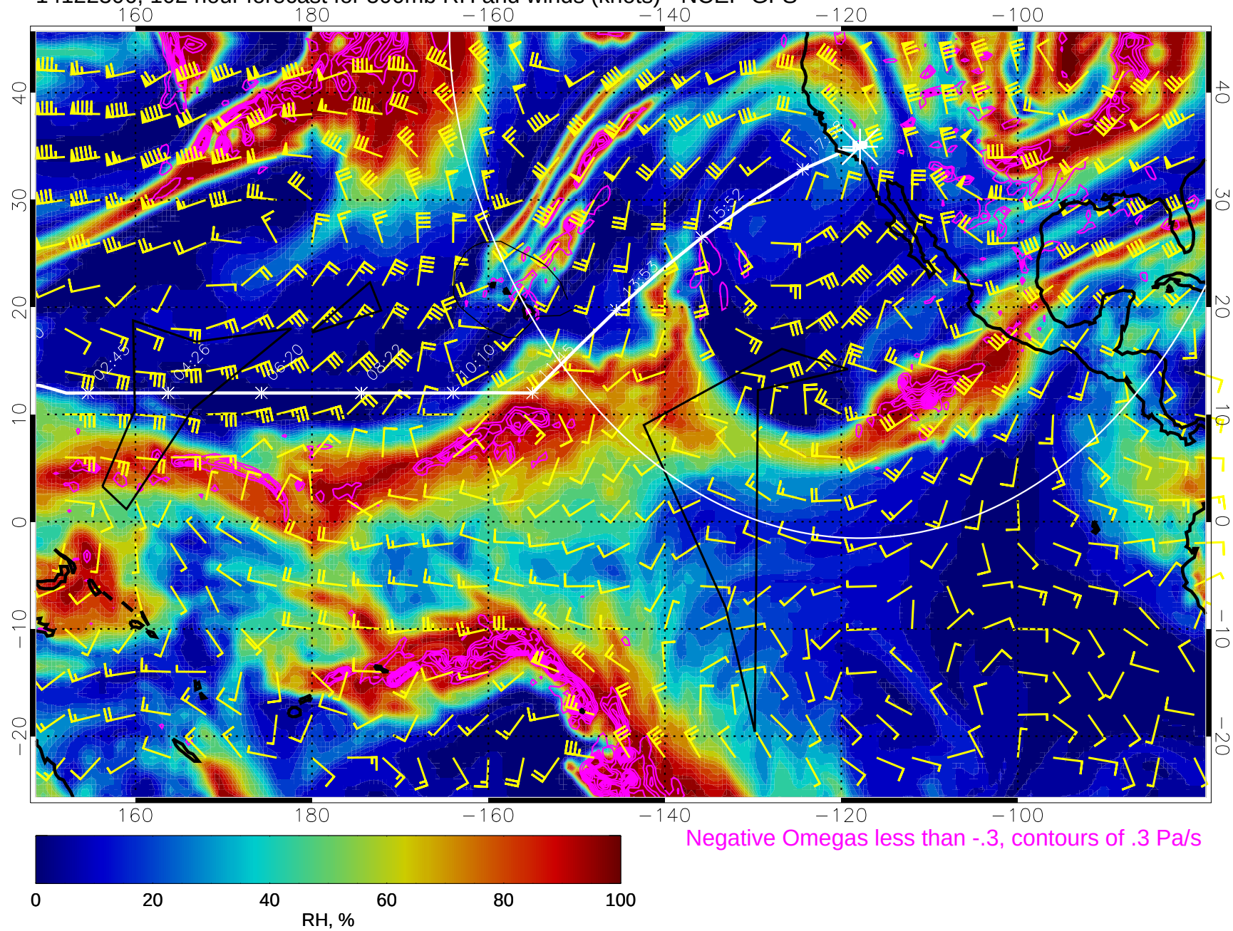
14122306, 102 hour forecast for 500mb RH and winds (knots) - NCEP GFS
