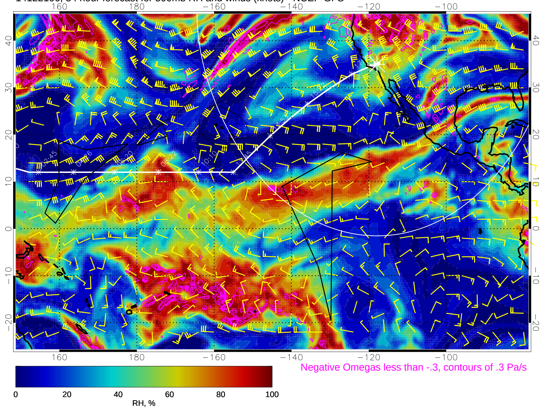
14122106, 54 hour forecast for 500mb RH and winds (knots) - NCEP GFS
