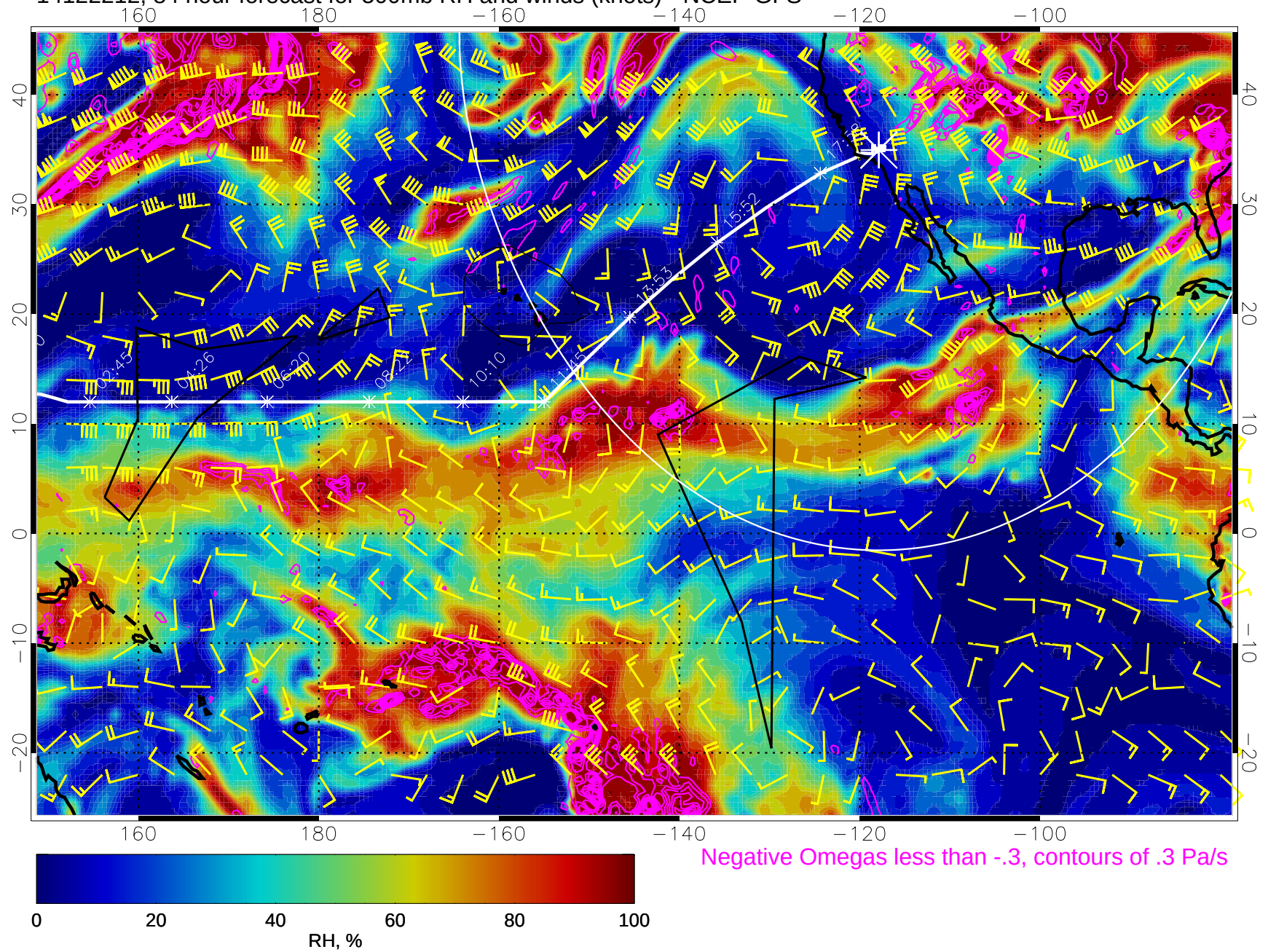
14122212, 84 hour forecast for 500mb RH and winds (knots) - NCEP GFS
