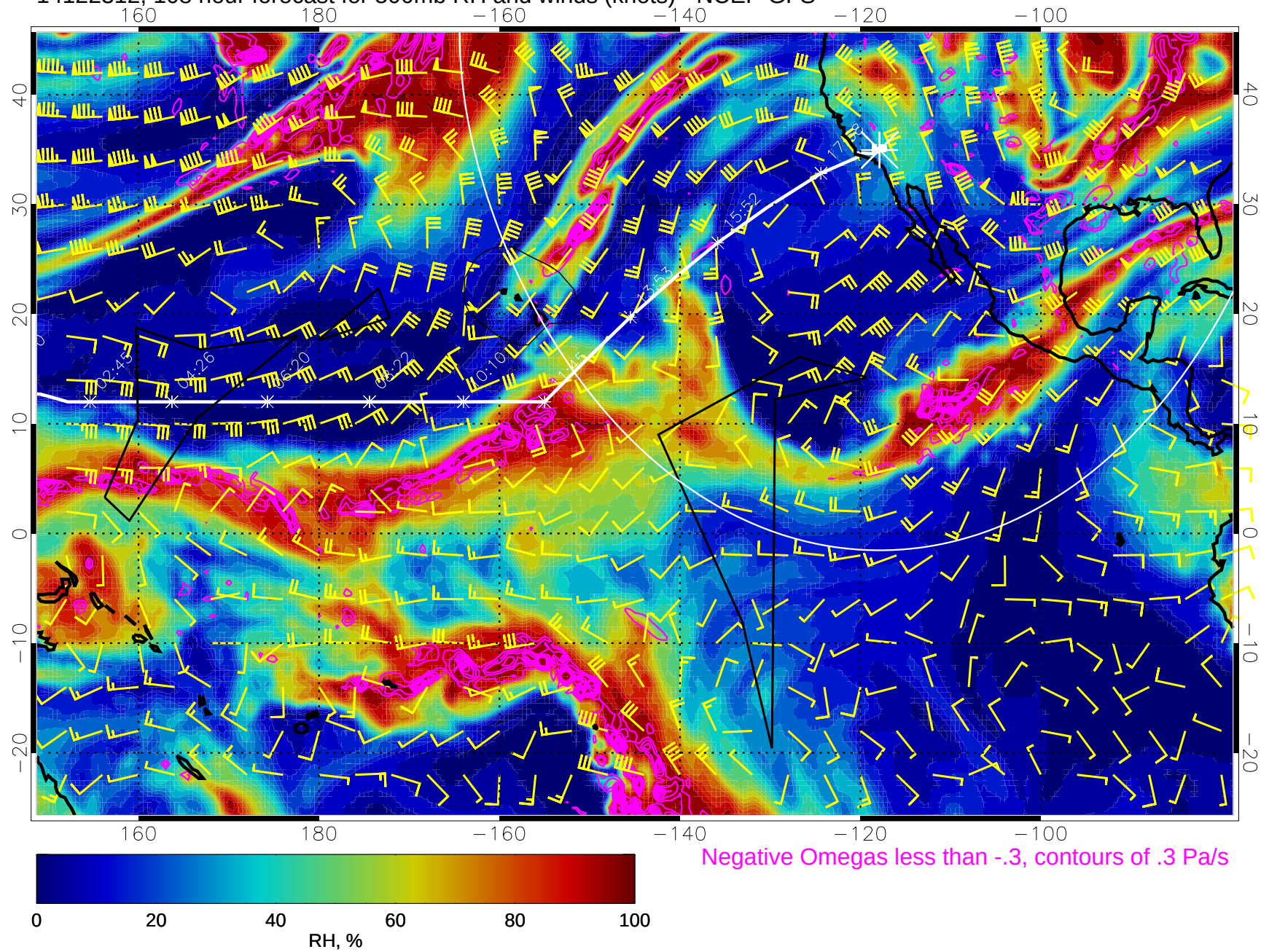
14122312, 108 hour forecast for 500mb RH and winds (knots) - NCEP GFS
