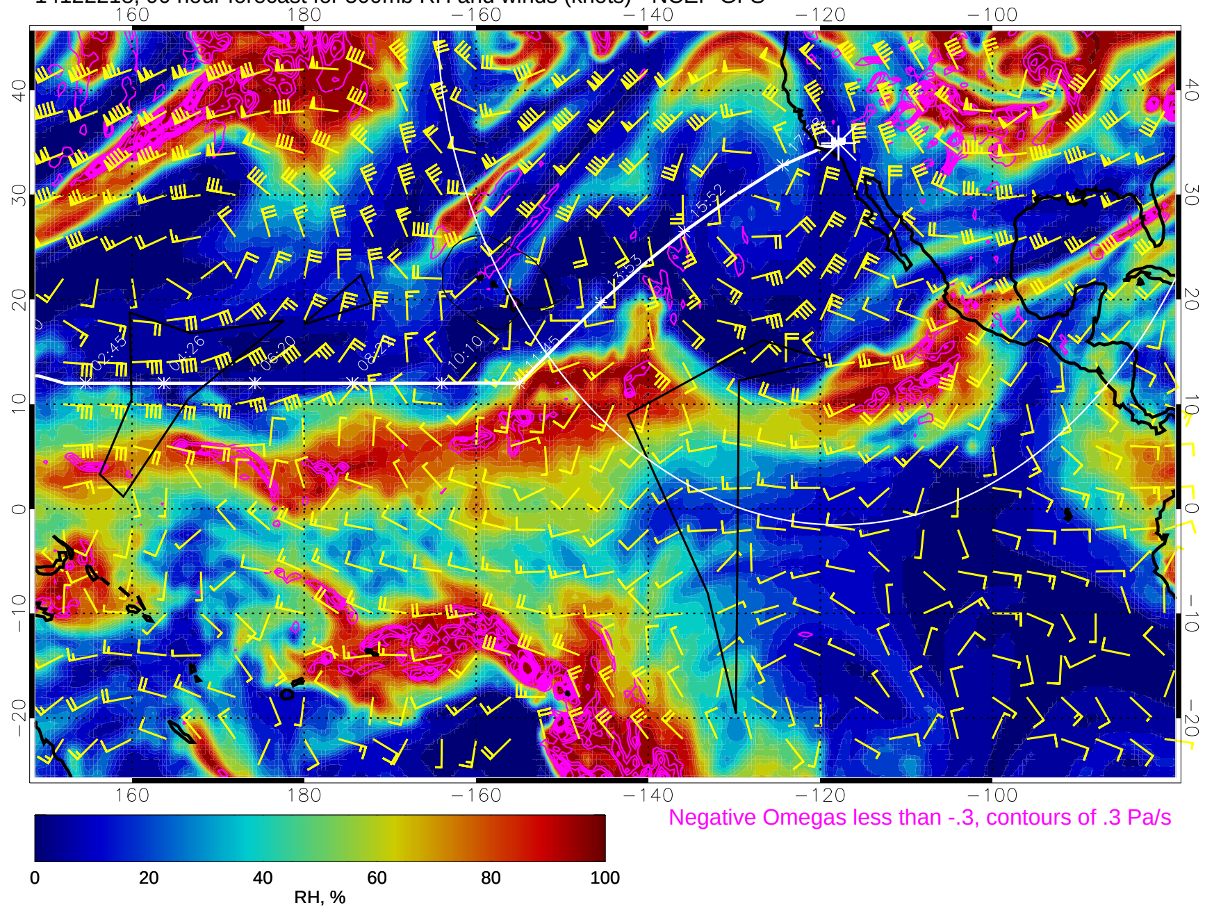
14122218, 90 hour forecast for 500mb RH and winds (knots) - NCEP GFS
