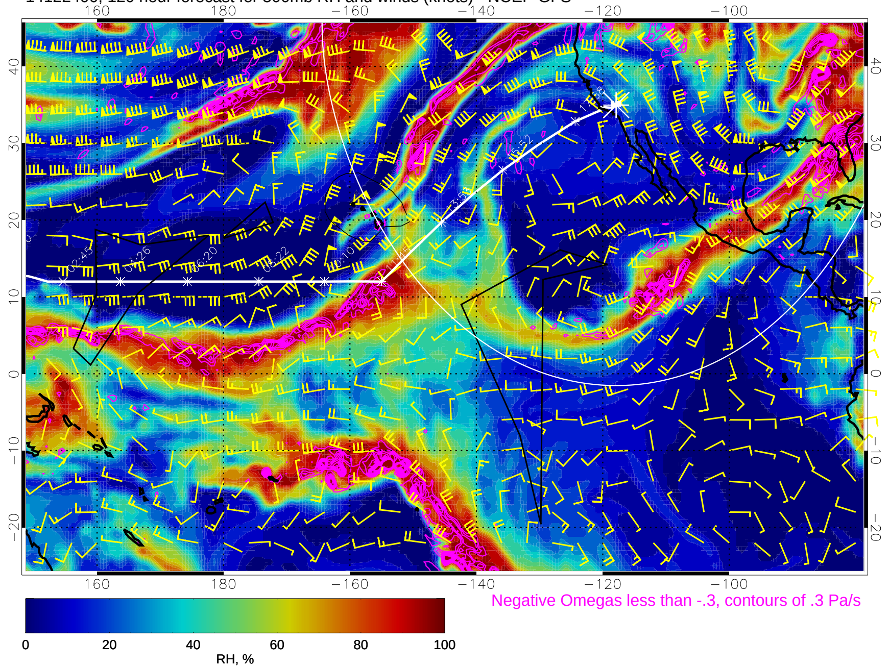
14122400, 120 hour forecast for 500mb RH and winds (knots) - NCEP GFS
