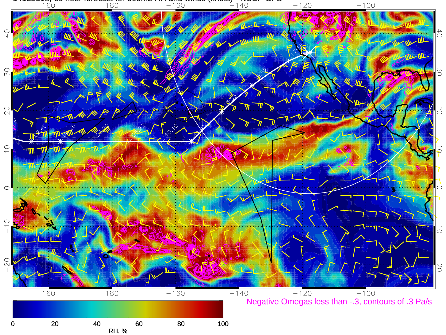
14122118, 66 hour forecast for 500mb RH and winds (knots) - NCEP GFS
