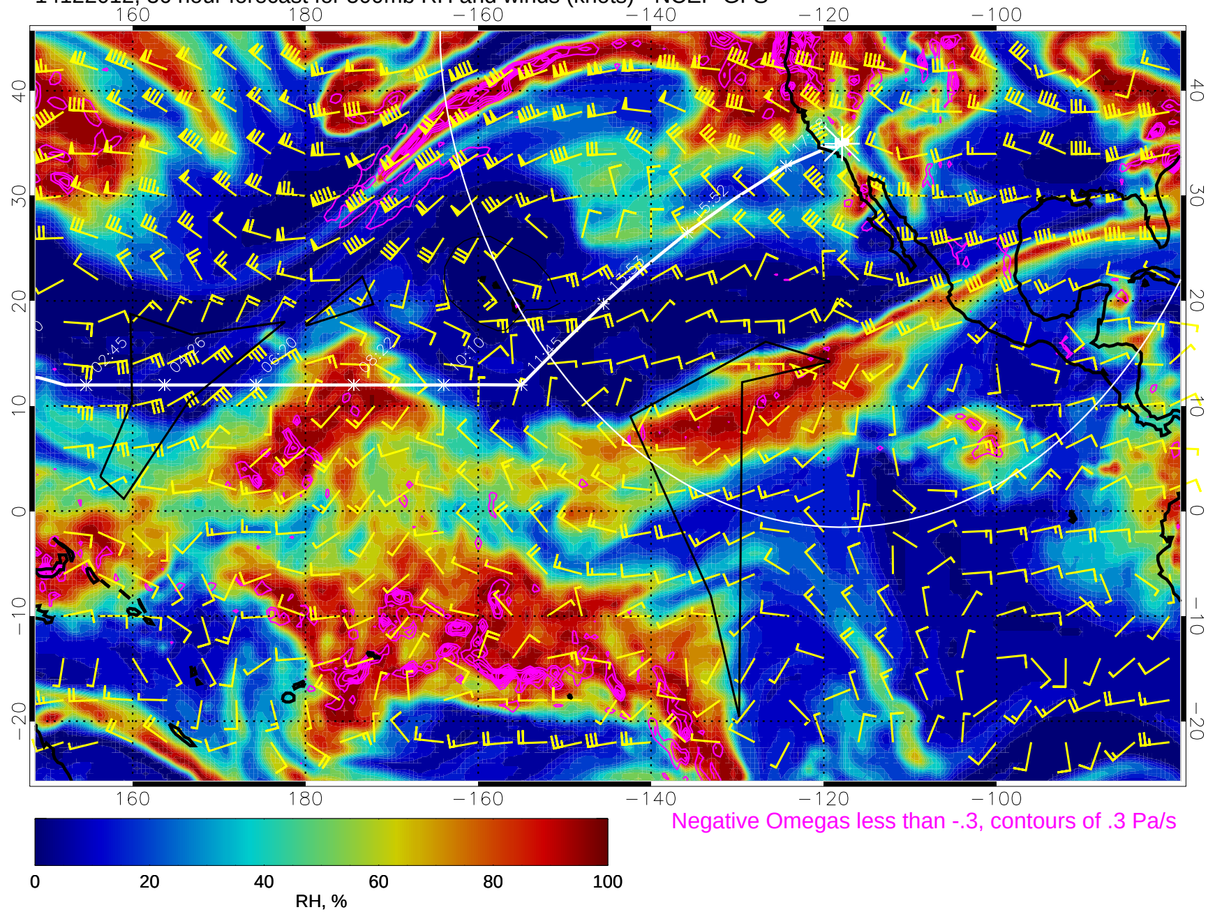
14122012, 36 hour forecast for 500mb RH and winds (knots) - NCEP GFS
