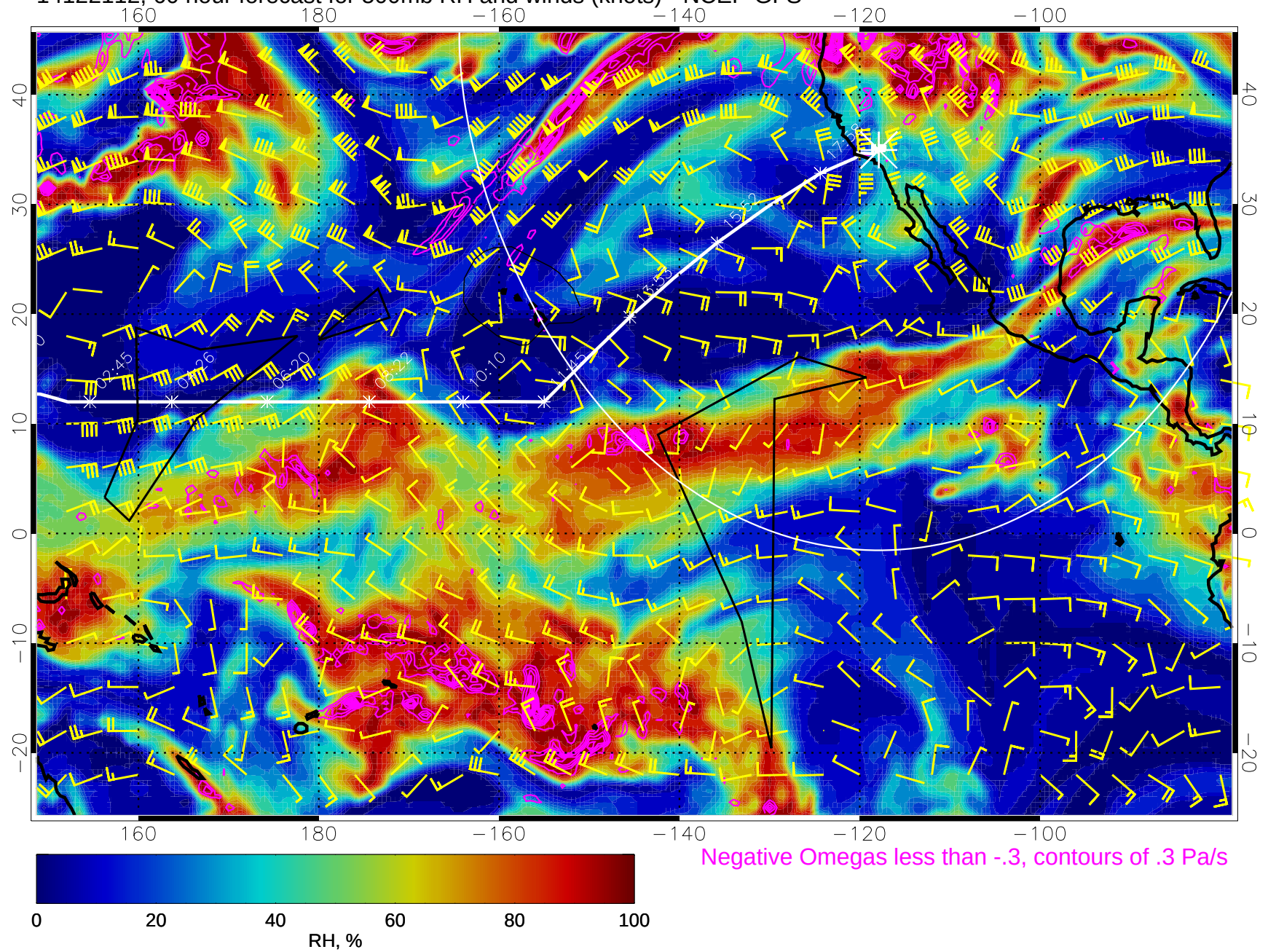
14122112, 60 hour forecast for 500mb RH and winds (knots) - NCEP GFS
