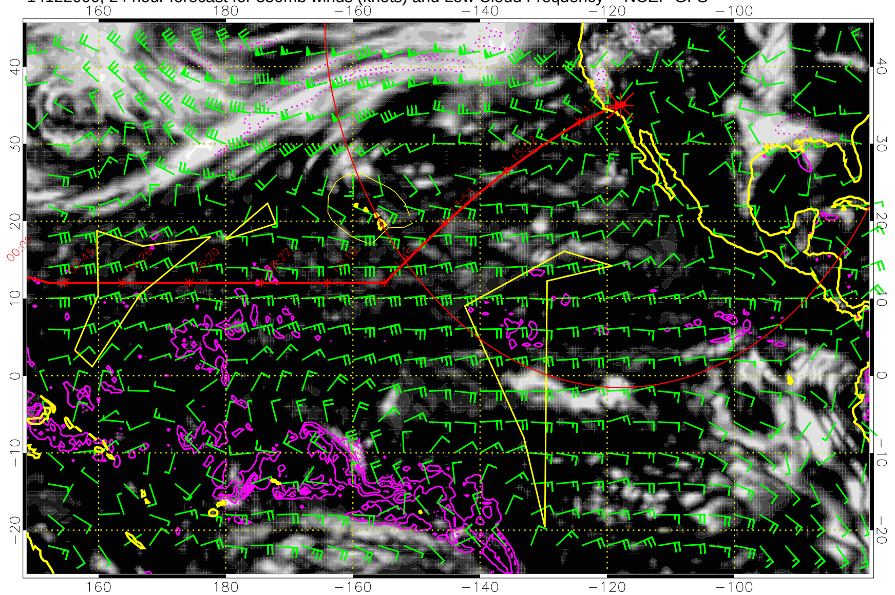
14122000, 24 hour forecast for 850mb winds (knots) and Low Cloud Frequency -- NCEP GFS
