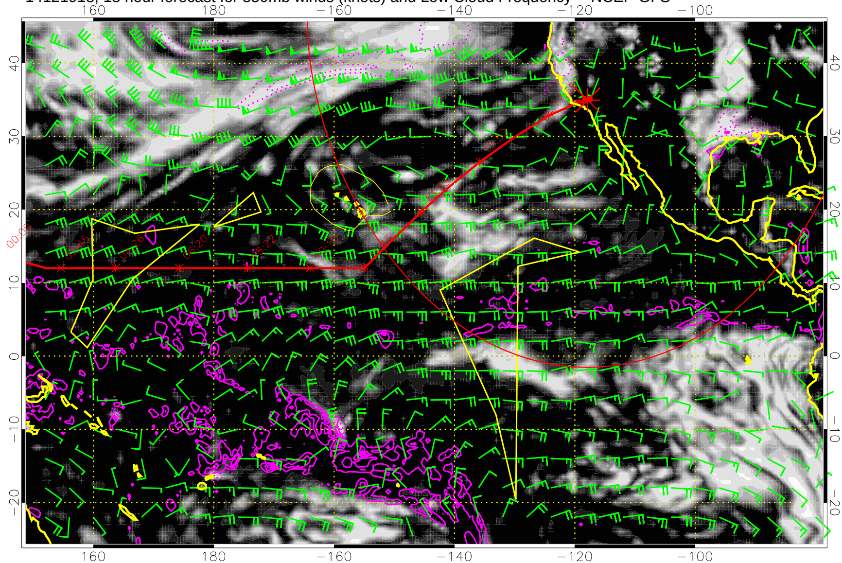
14121918, 18 hour forecast for 850mb winds (knots) and Low Cloud Frequency -- NCEP GFS
