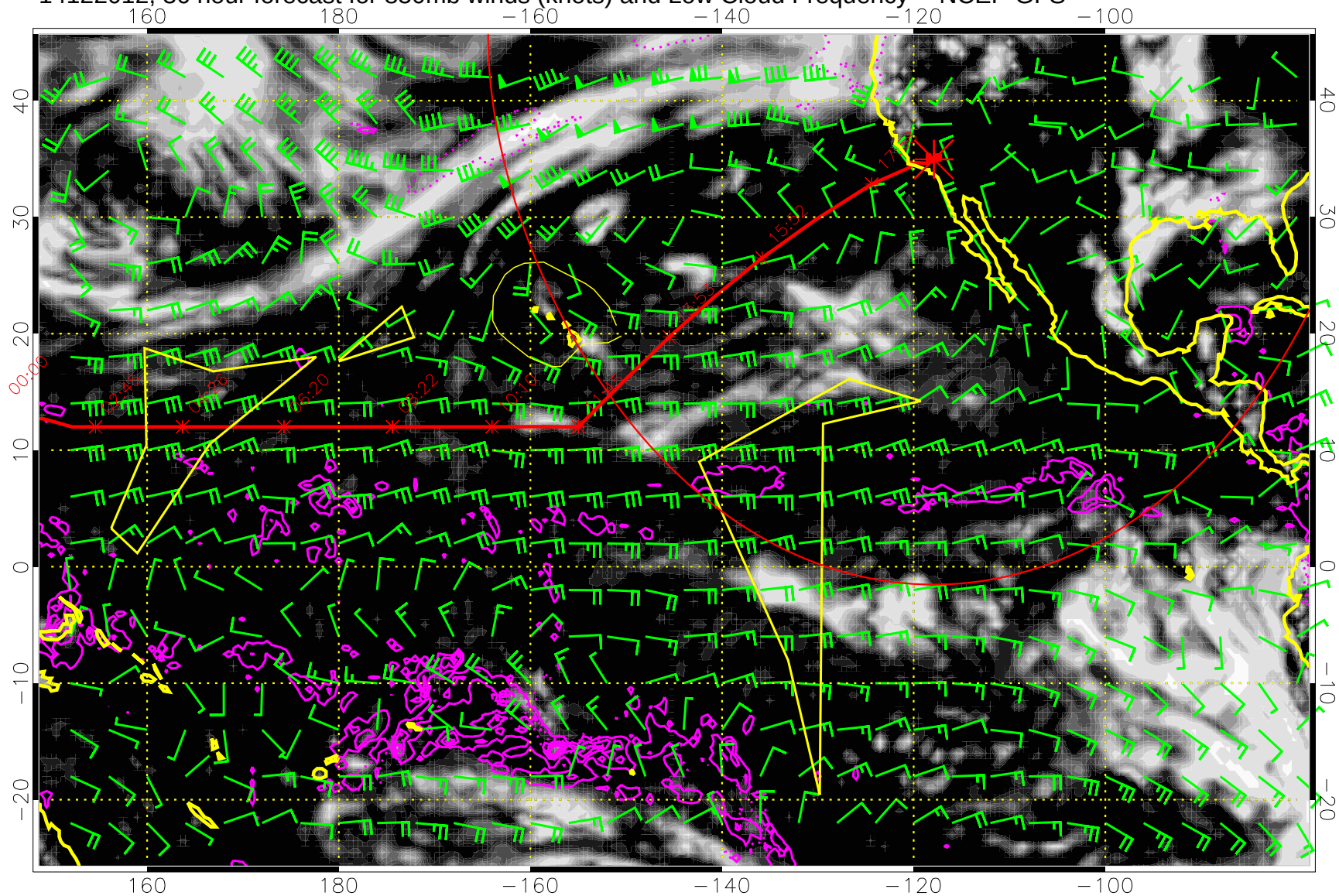
14122012, 36 hour forecast for 850mb winds (knots) and Low Cloud Frequency -- NCEP GFS
