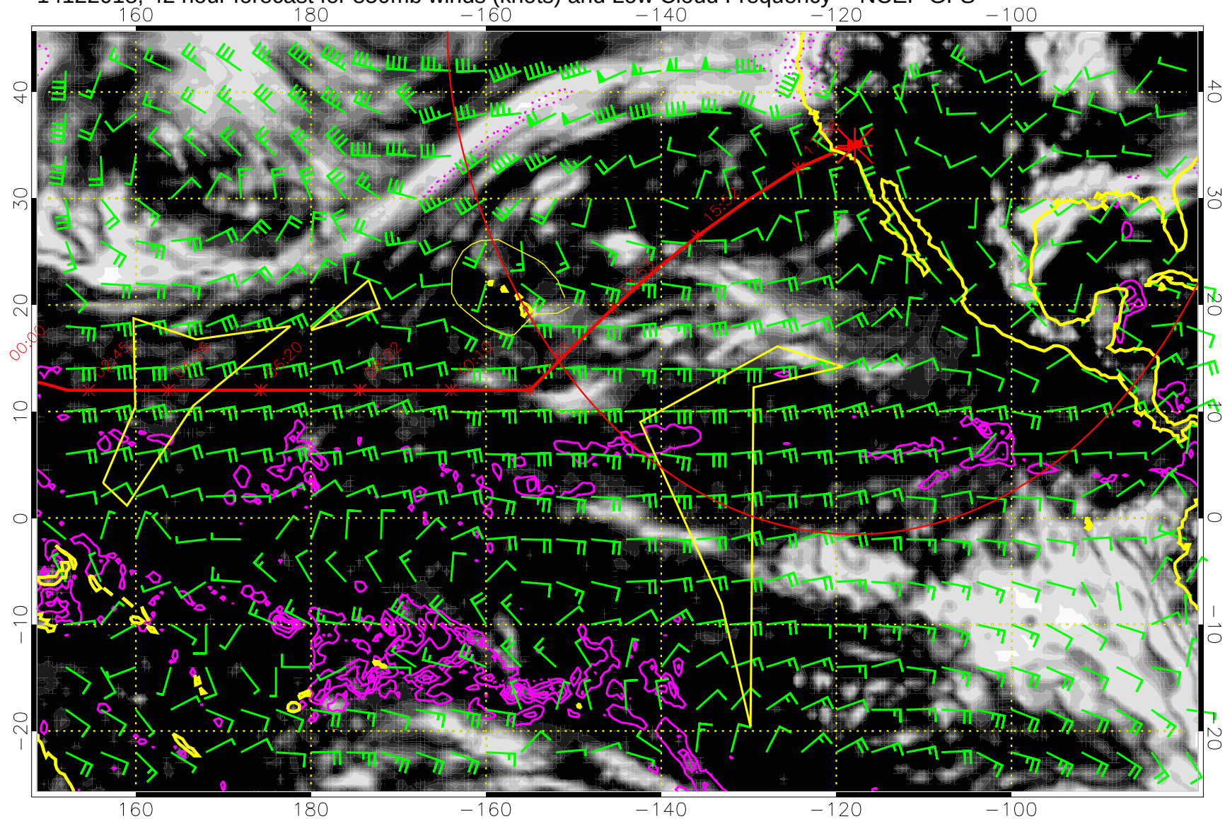
14122018, 42 hour forecast for 850mb winds (knots) and Low Cloud Frequency -- NCEP GFS
