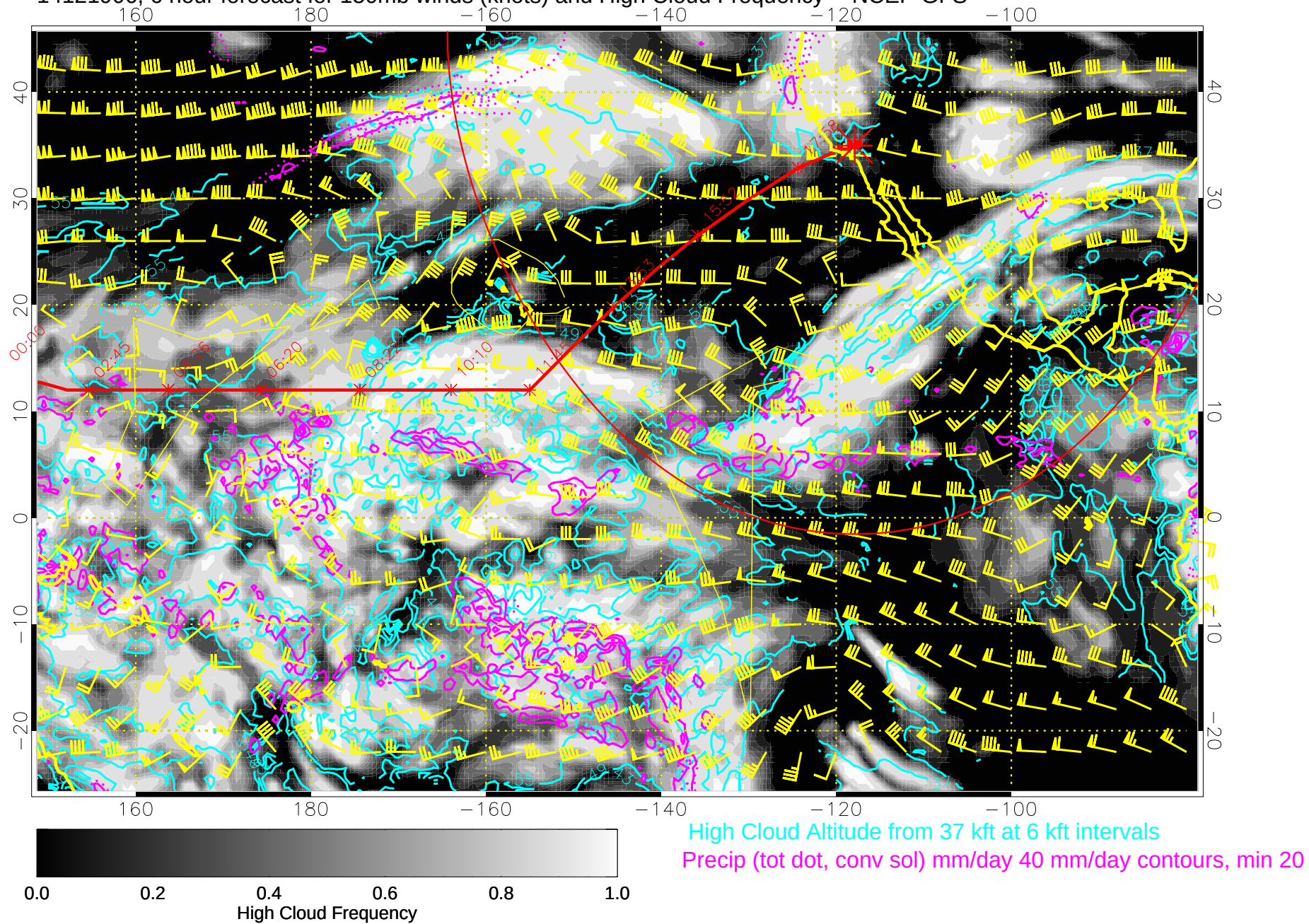
14121906, 6 hour forecast for 150mb winds (knots) and High Cloud Frequency -- NCEP GFS
