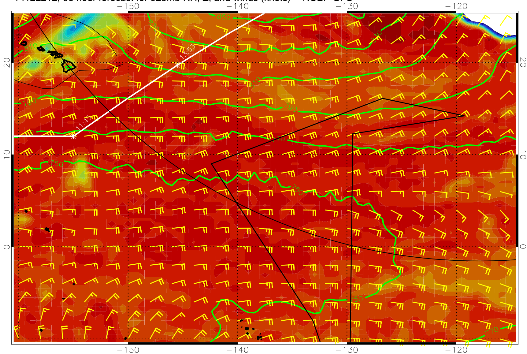
14122212, 96 hour forecast for 925mb RH, Z, and winds (knots) -- NCEP GFS
