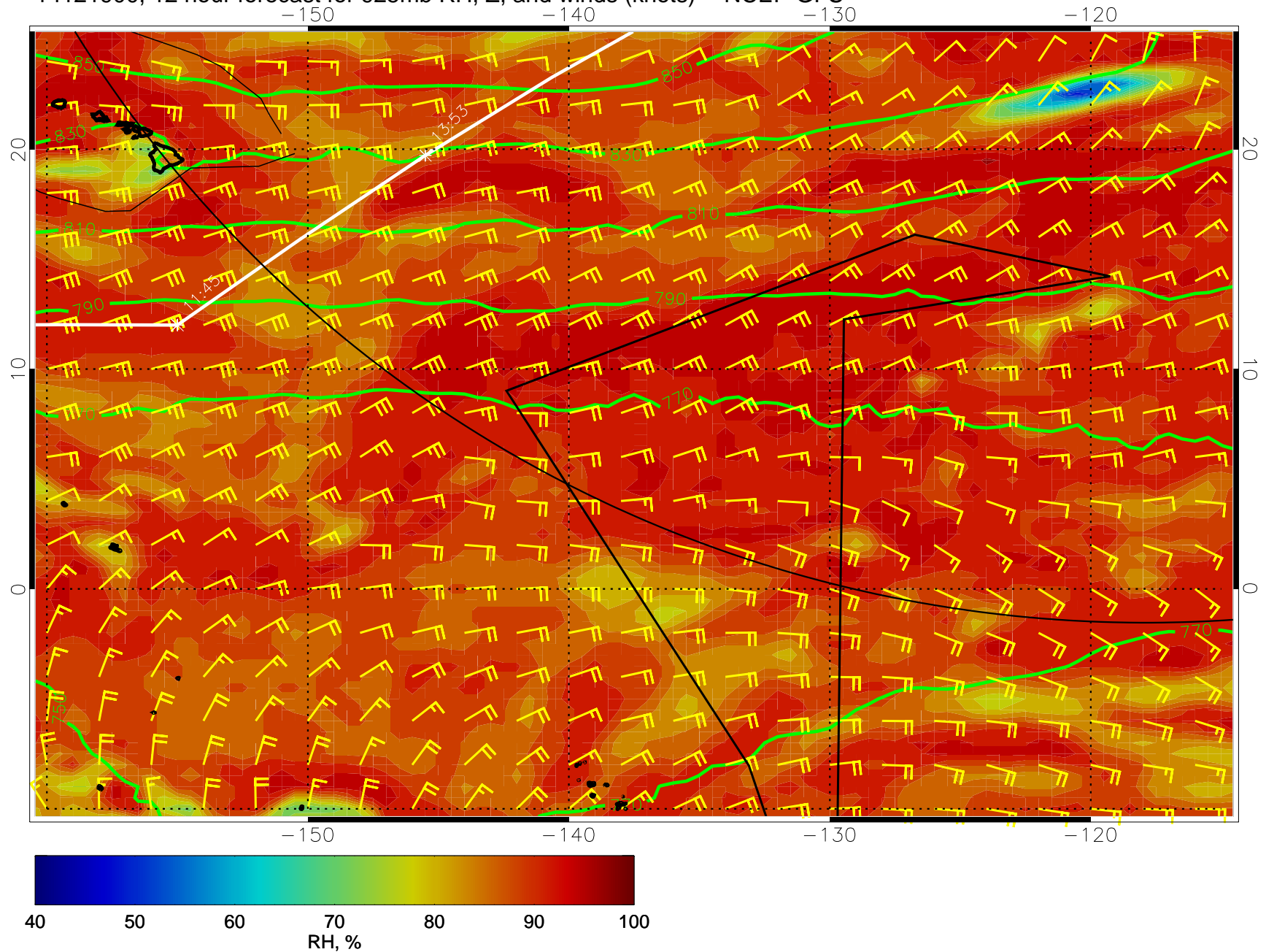
14121900, 12 hour forecast for 925mb RH, Z, and winds (knots) -- NCEP GFS
