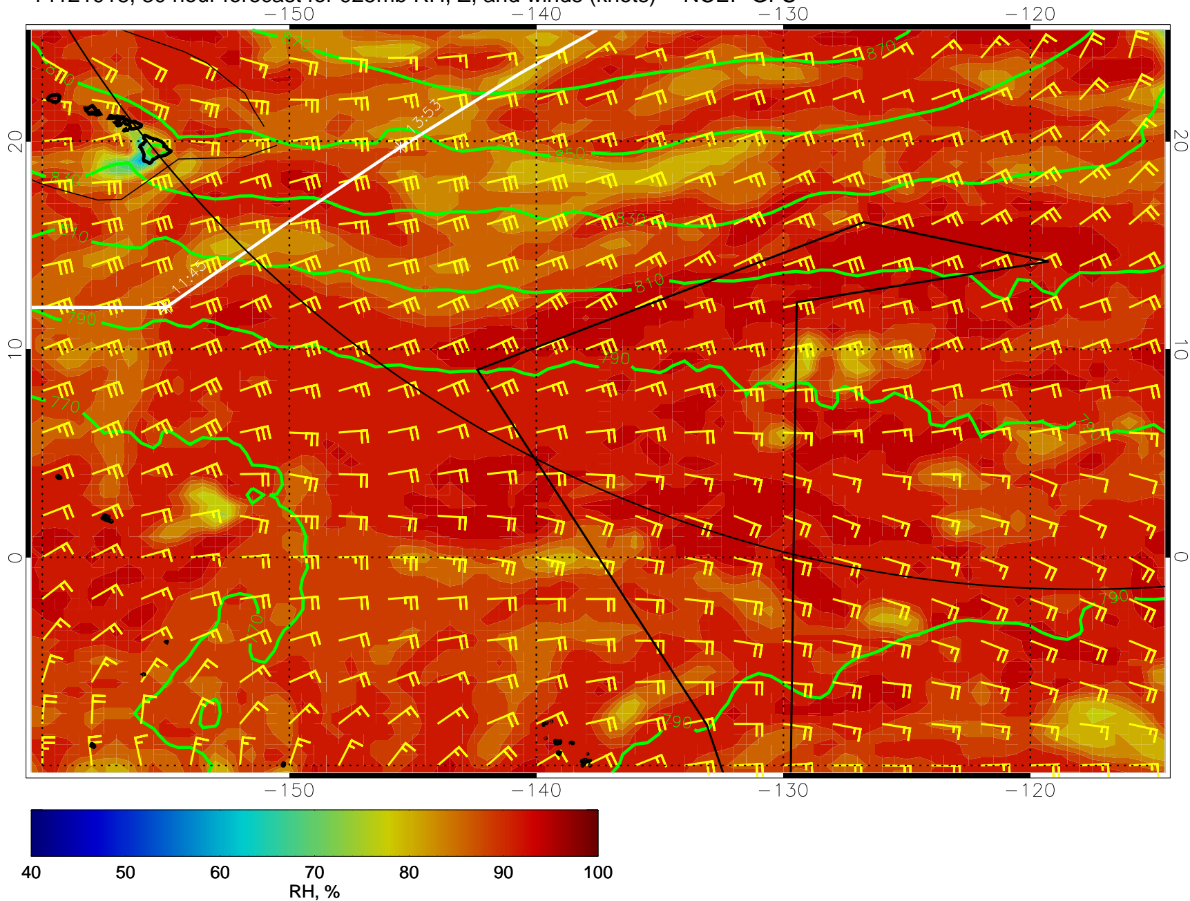
14121918, 30 hour forecast for 925mb RH, Z, and winds (knots) -- NCEP GFS
