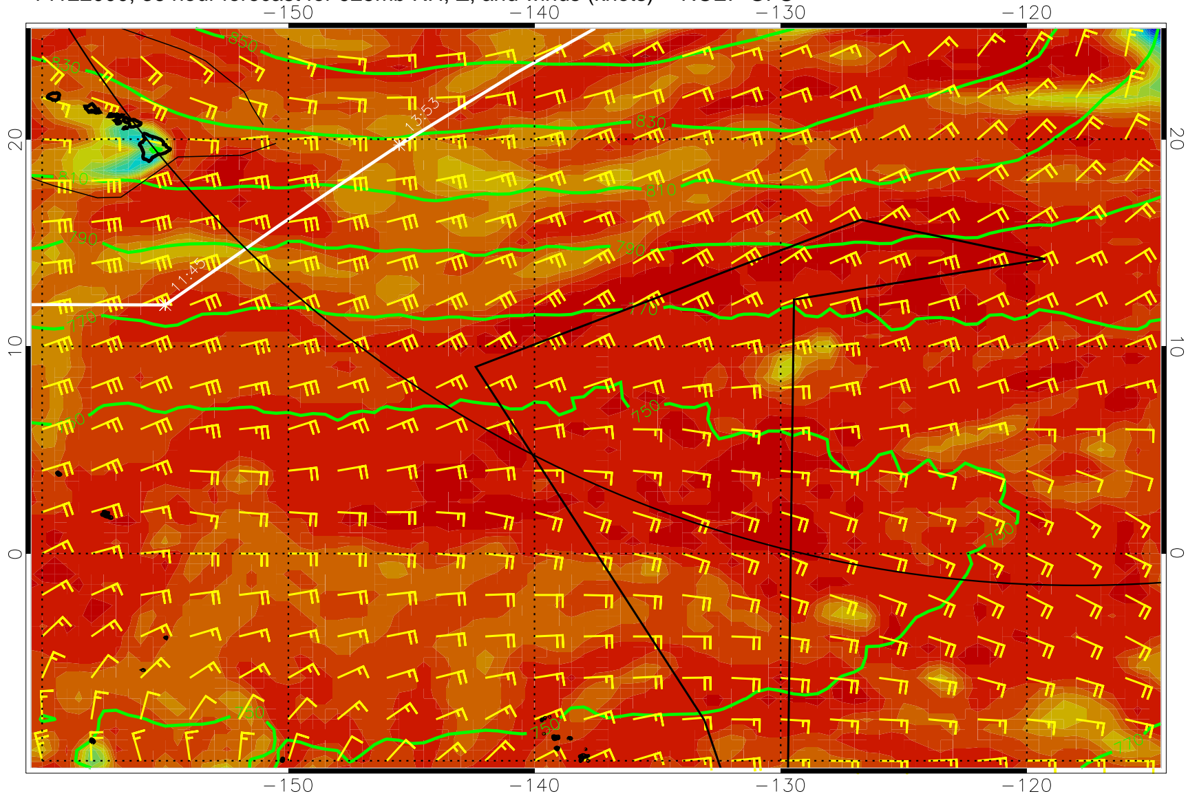
14122000, 36 hour forecast for 925mb RH, Z, and winds (knots) -- NCEP GFS
