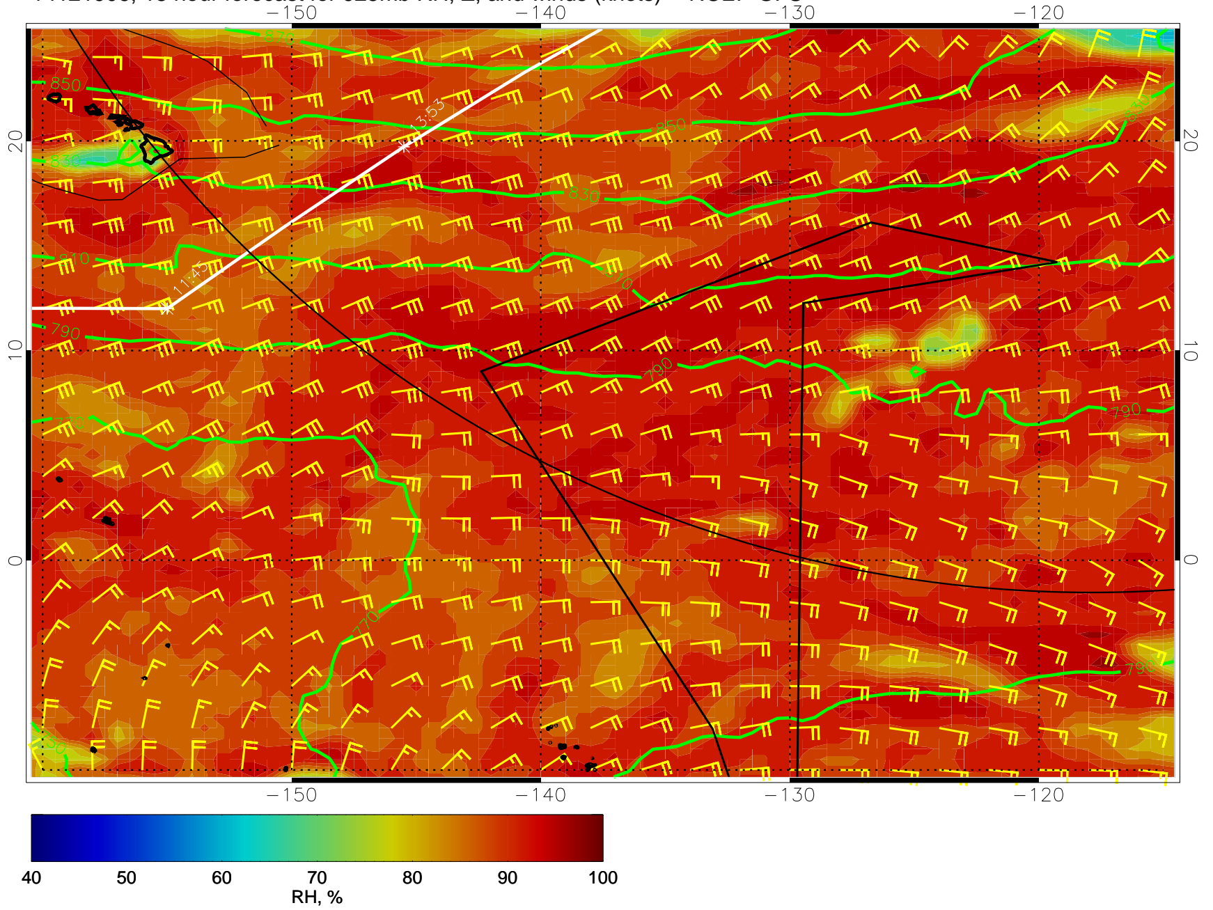
14121906, 18 hour forecast for 925mb RH, Z, and winds (knots) -- NCEP GFS
