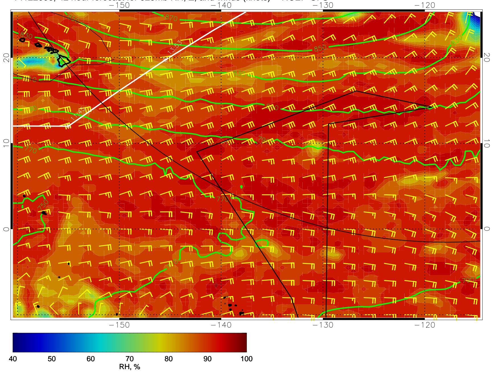
14122006, 42 hour forecast for 925mb RH, Z, and winds (knots) -- NCEP GFS
