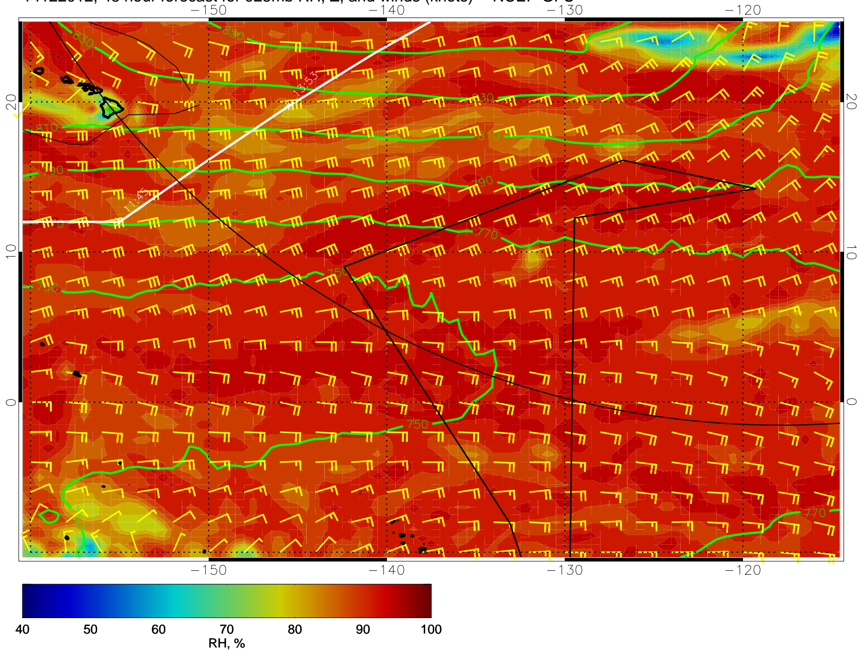
14122012, 48 hour forecast for 925mb RH, Z, and winds (knots) -- NCEP GFS
