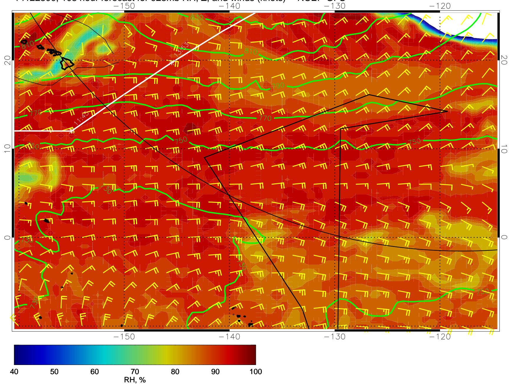
14122300, 108 hour forecast for 925mb RH, Z, and winds (knots) -- NCEP GFS
