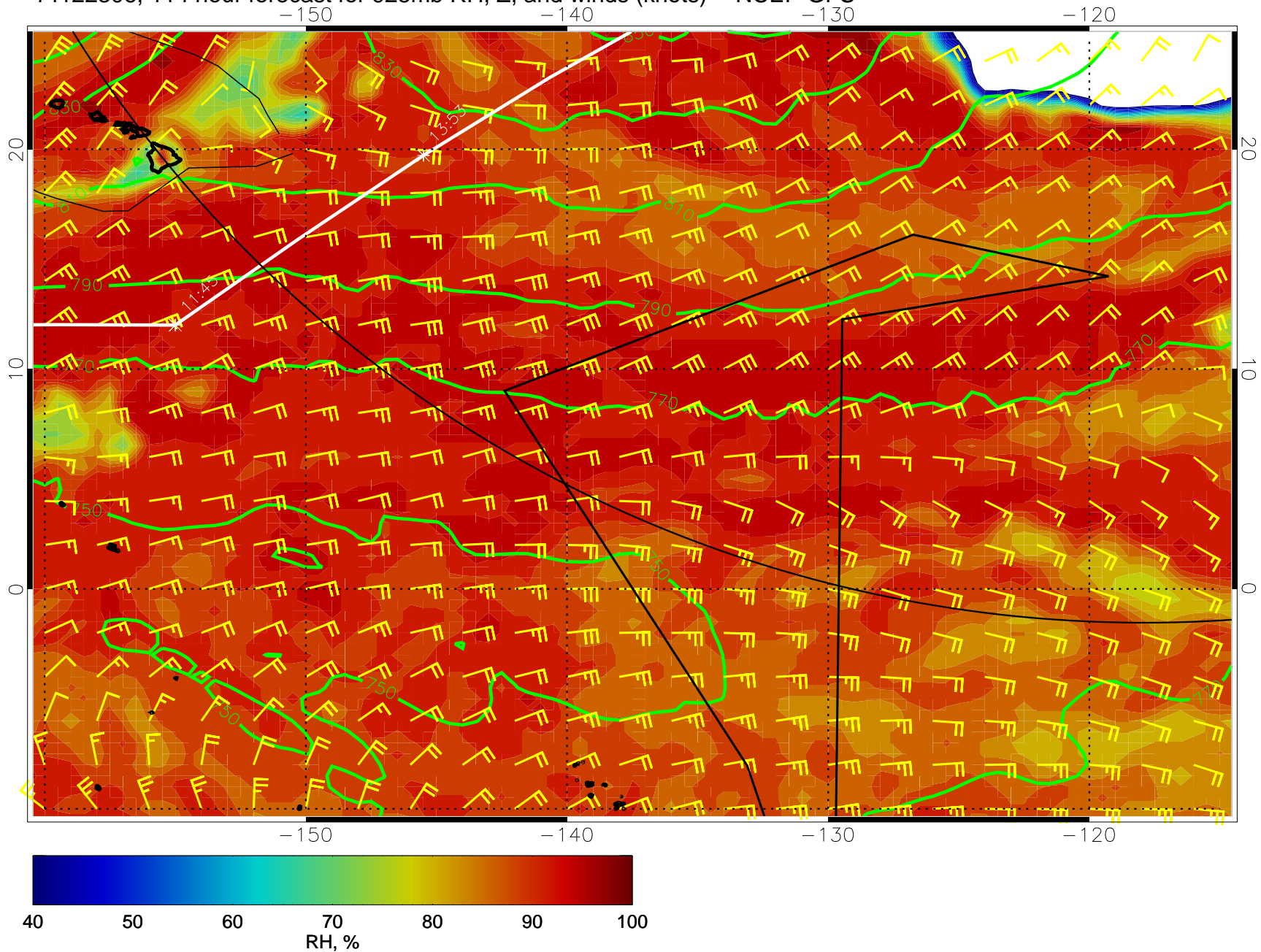
14122306, 114 hour forecast for 925mb RH, Z, and winds (knots) -- NCEP GFS
