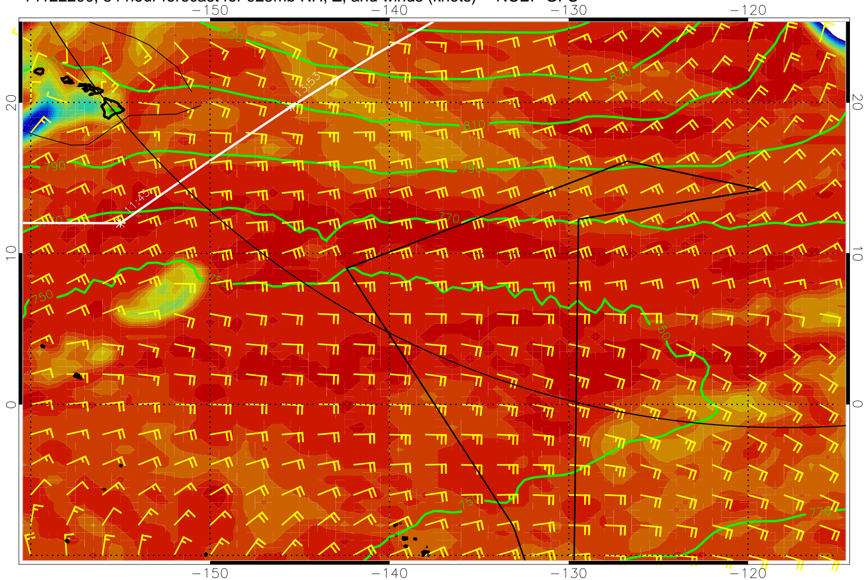
14122200, 84 hour forecast for 925mb RH, Z, and winds (knots) -- NCEP GFS
