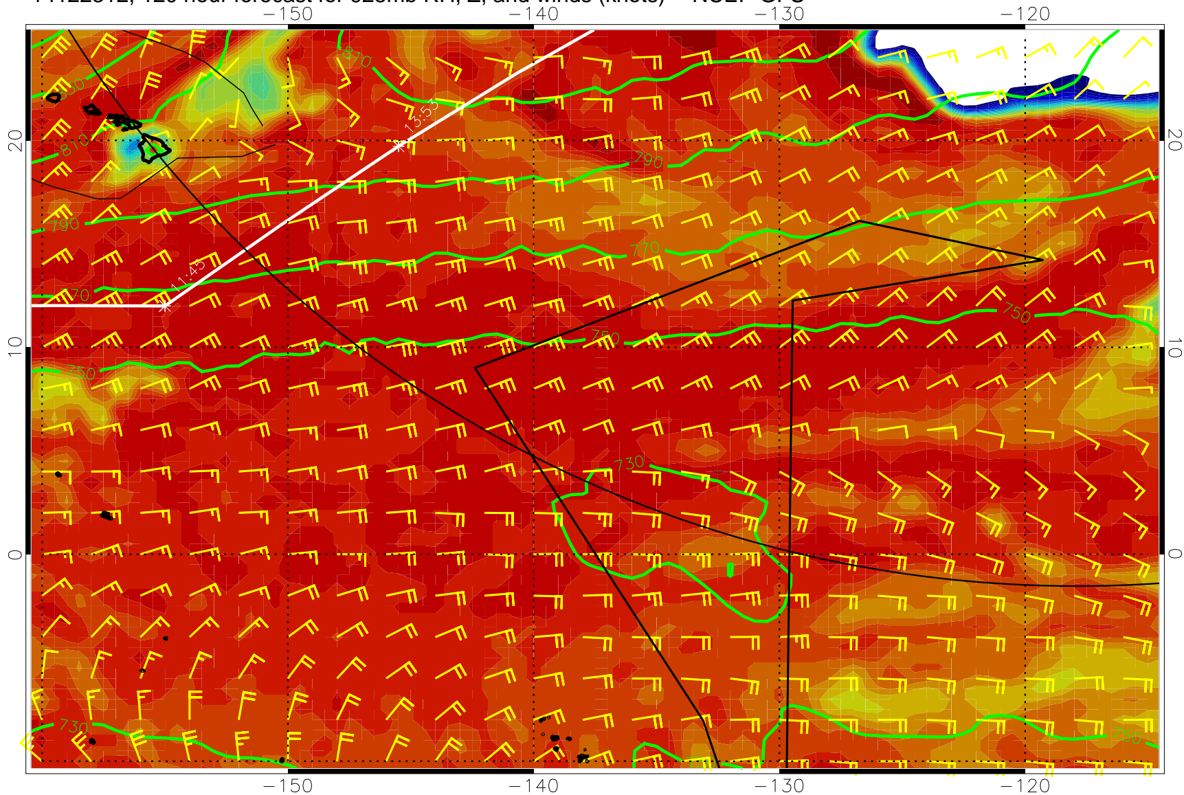
14122312, 120 hour forecast for 925mb RH, Z, and winds (knots) -- NCEP GFS
