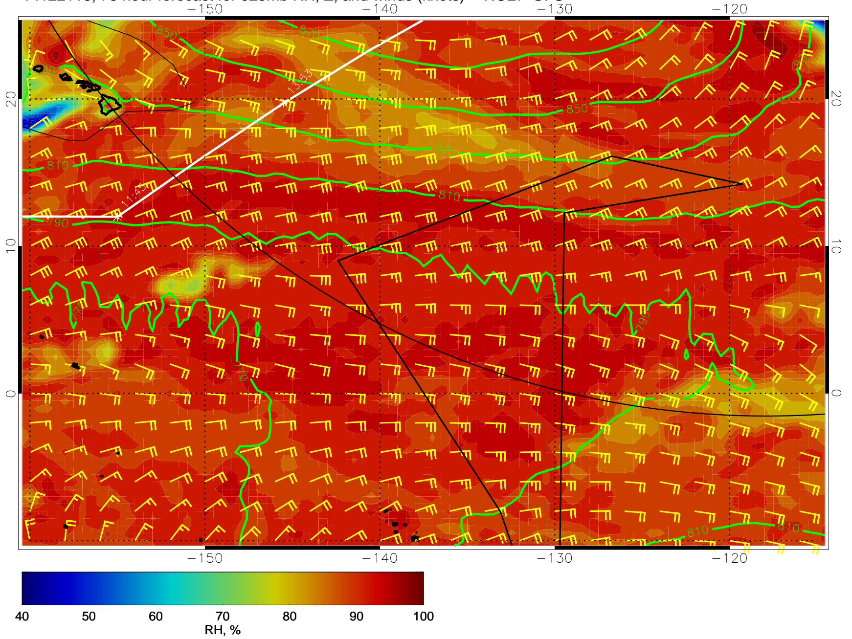
14122118, 78 hour forecast for 925mb RH, Z, and winds (knots) -- NCEP GFS
