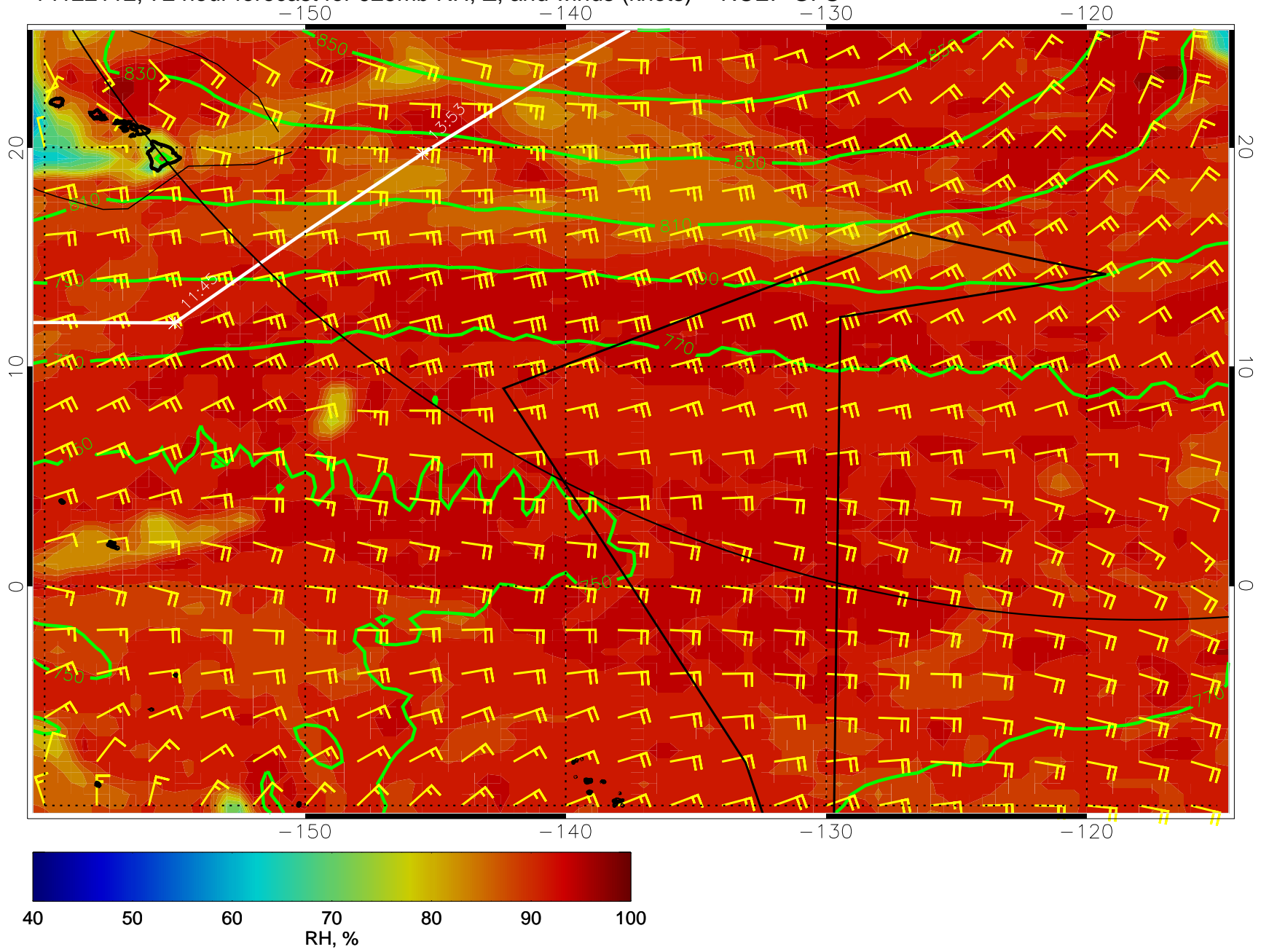
14122112, 72 hour forecast for 925mb RH, Z, and winds (knots) -- NCEP GFS
