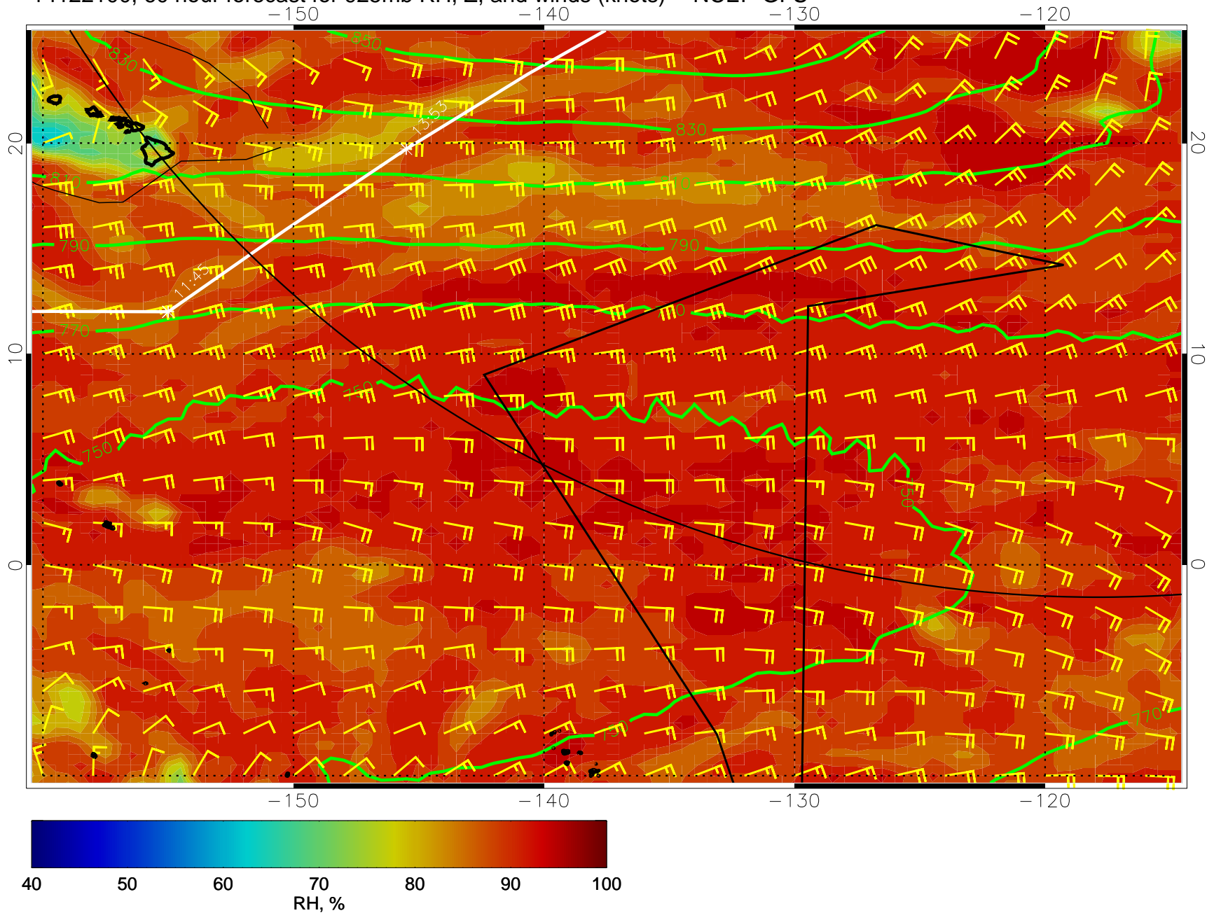
14122100, 60 hour forecast for 925mb RH, Z, and winds (knots) -- NCEP GFS
