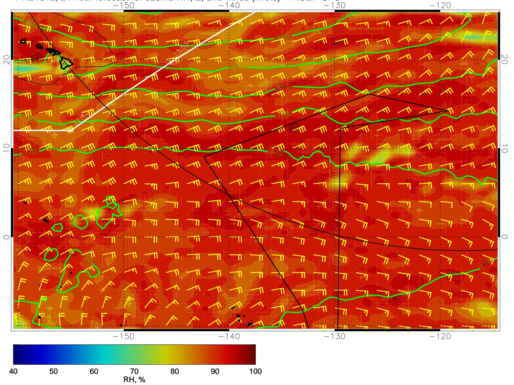
14121912, 24 hour forecast for 925mb RH, Z, and winds (knots) -- NCEP GFS
