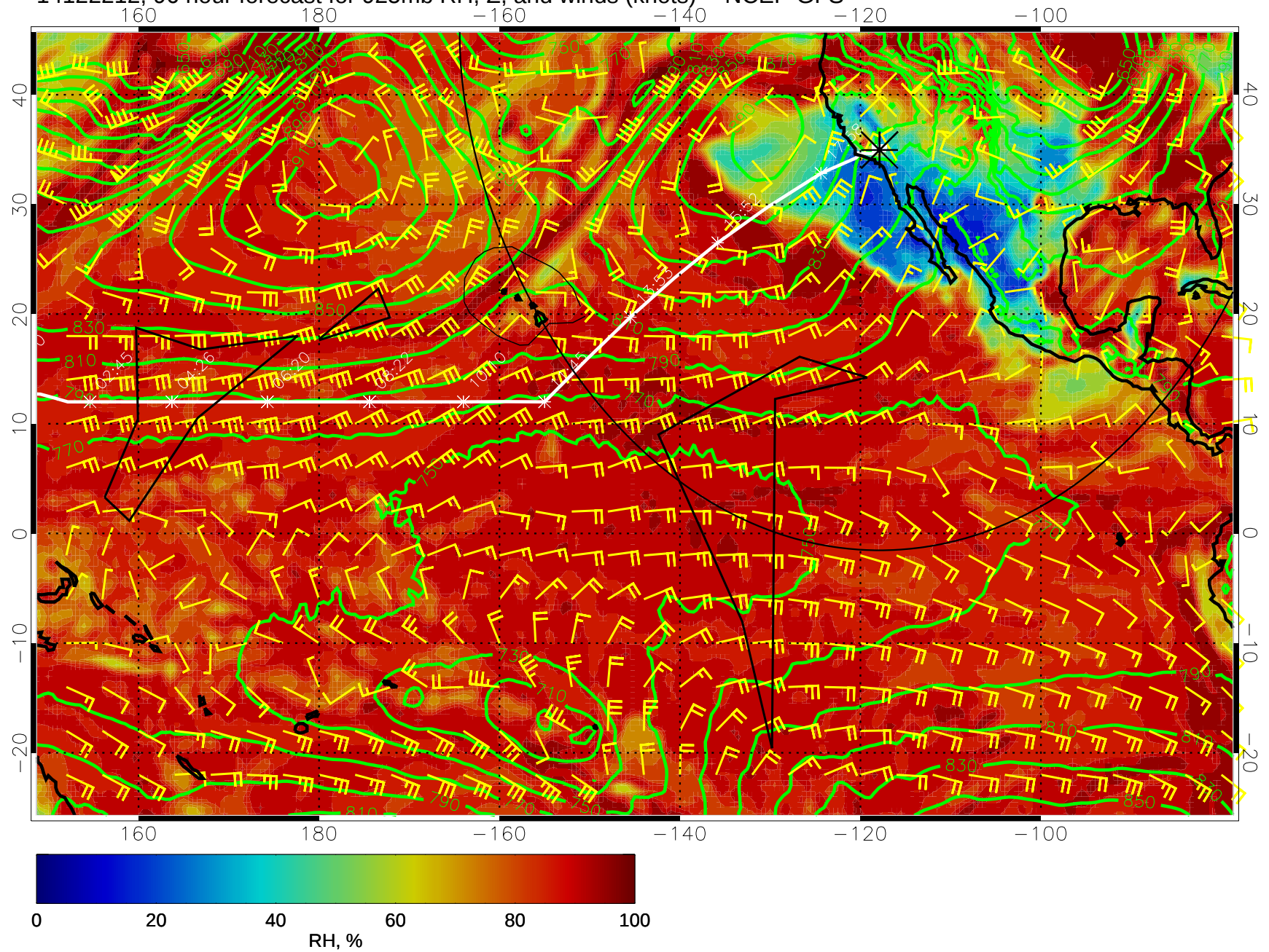
14122212, 96 hour forecast for 925mb RH, Z, and winds (knots) -- NCEP GFS
