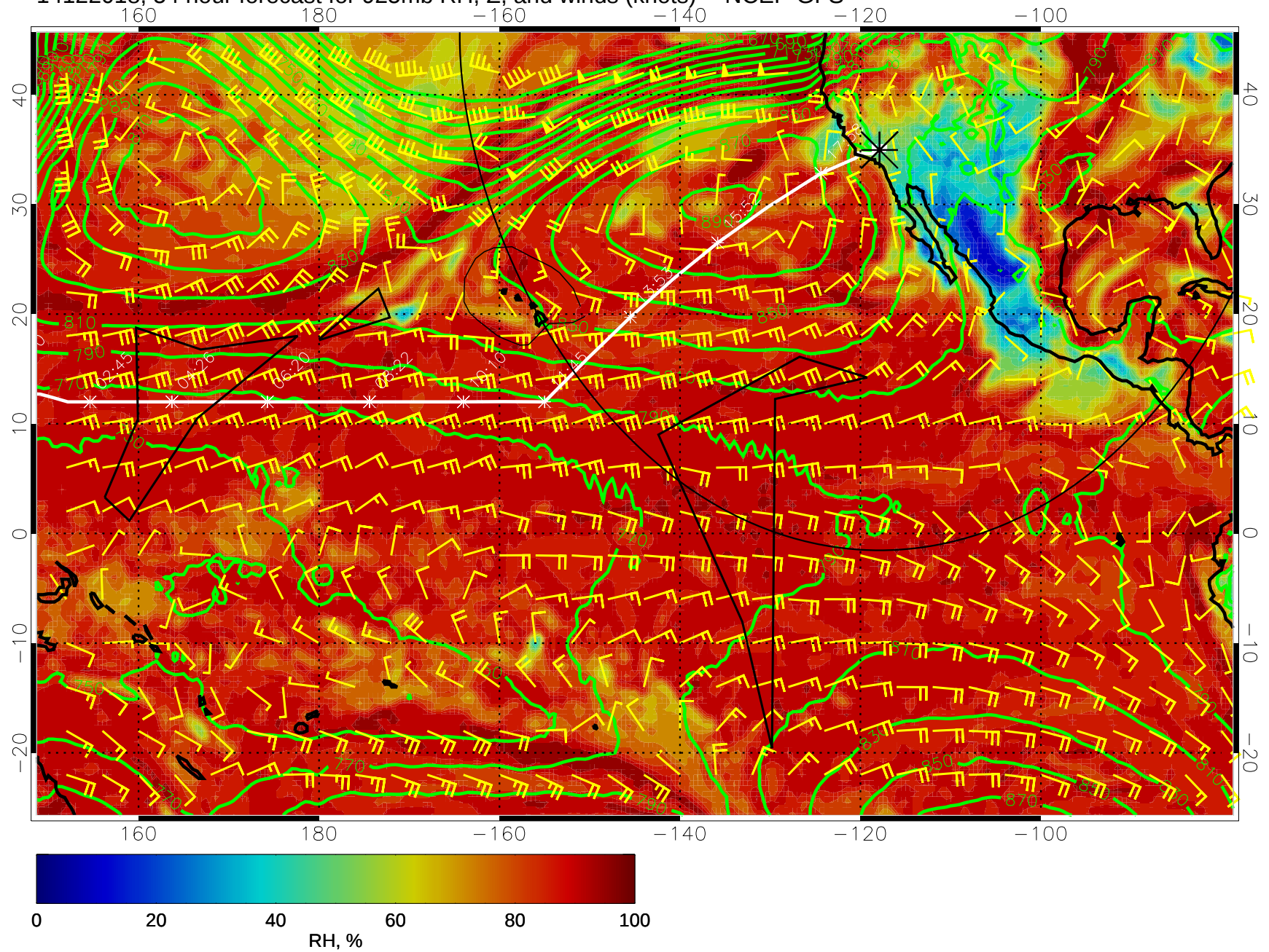
14122018, 54 hour forecast for 925mb RH, Z, and winds (knots) -- NCEP GFS
