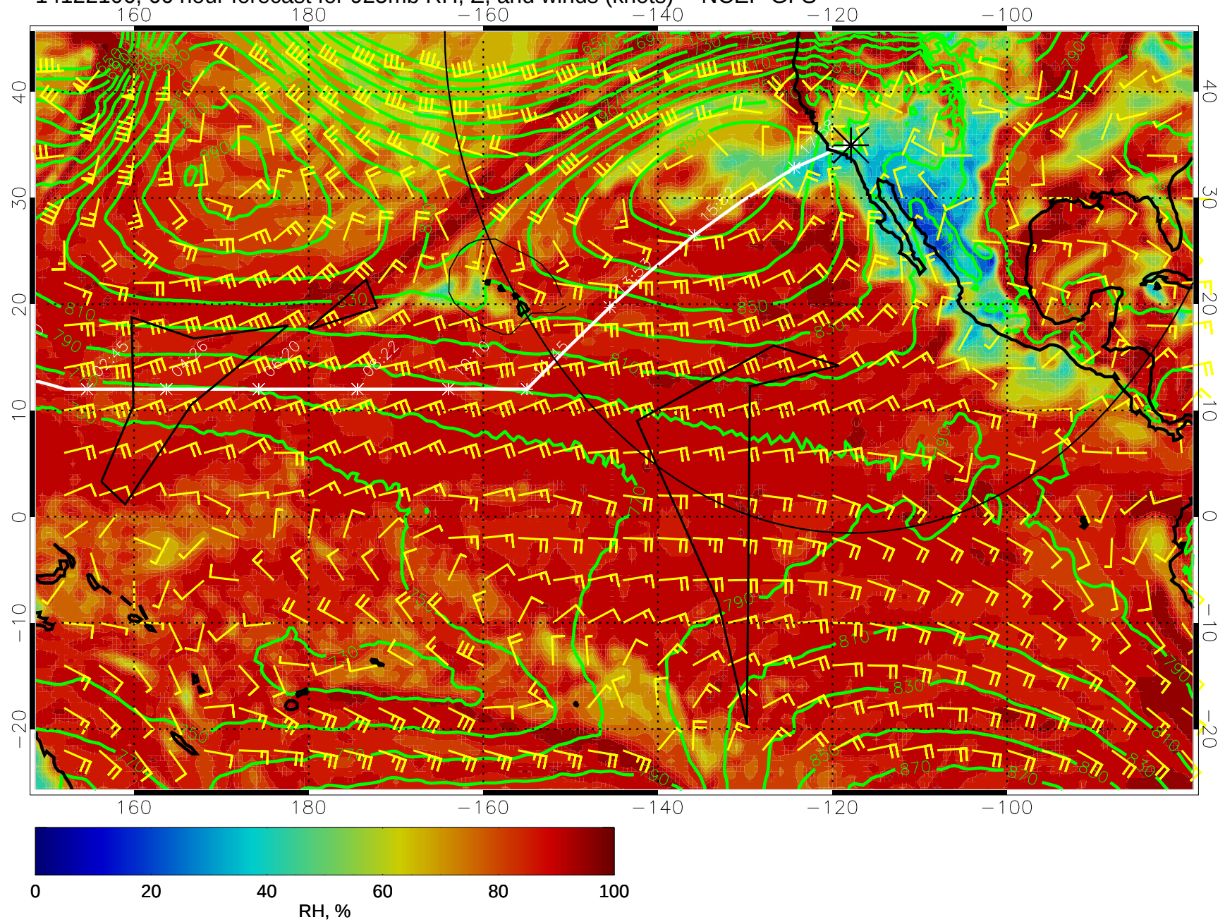
14122106, 66 hour forecast for 925mb RH, Z, and winds (knots) -- NCEP GFS
