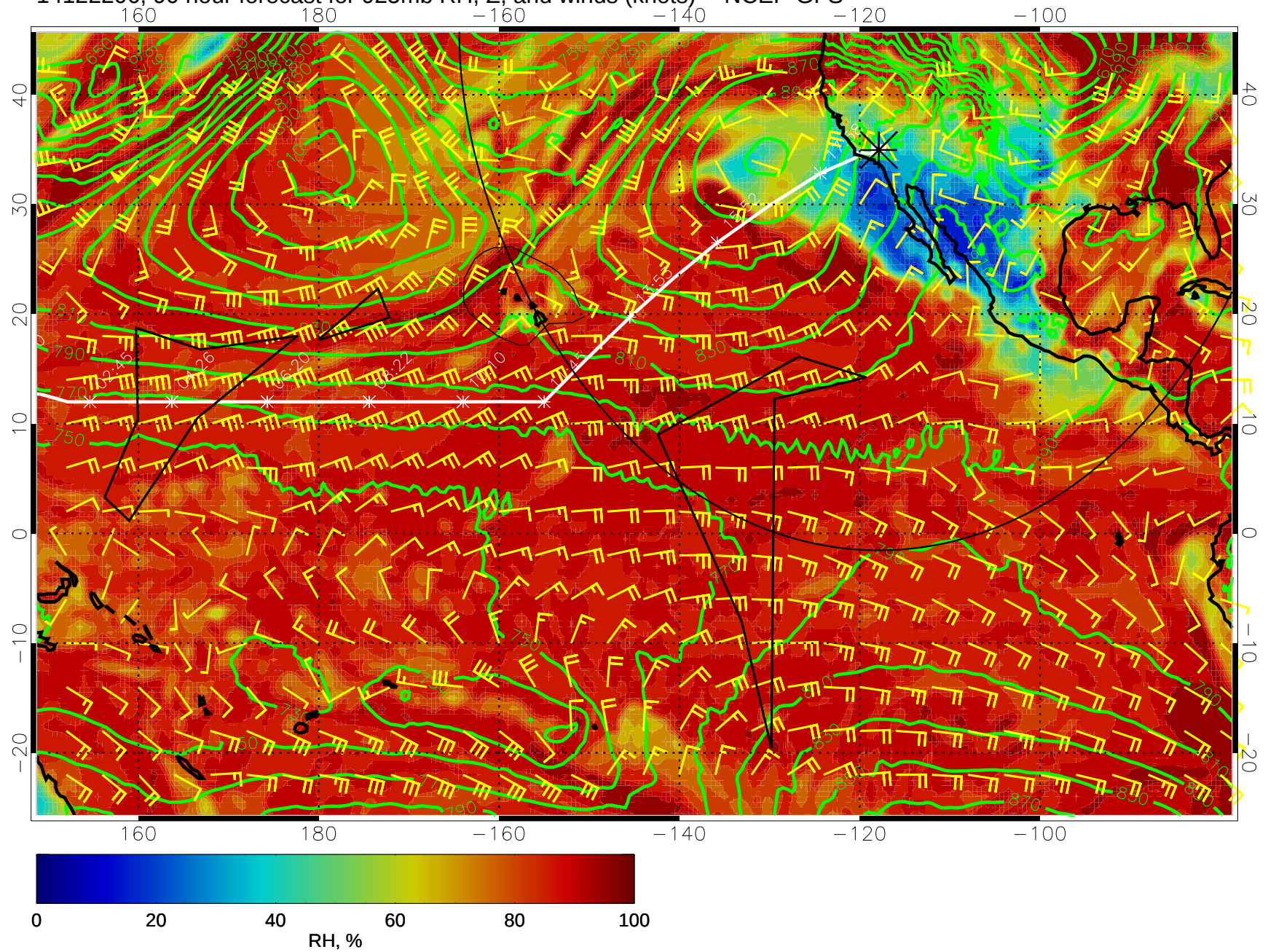
14122206, 90 hour forecast for 925mb RH, Z, and winds (knots) -- NCEP GFS
