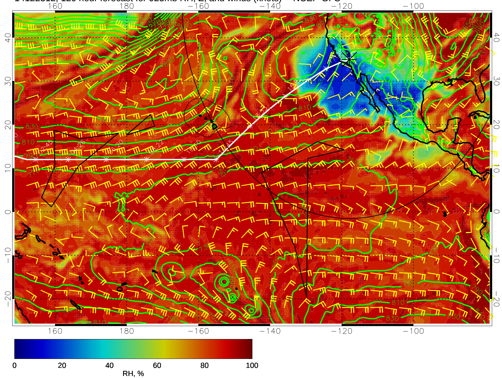
14122312, 120 hour forecast for 925mb RH, Z, and winds (knots) -- NCEP GFS
