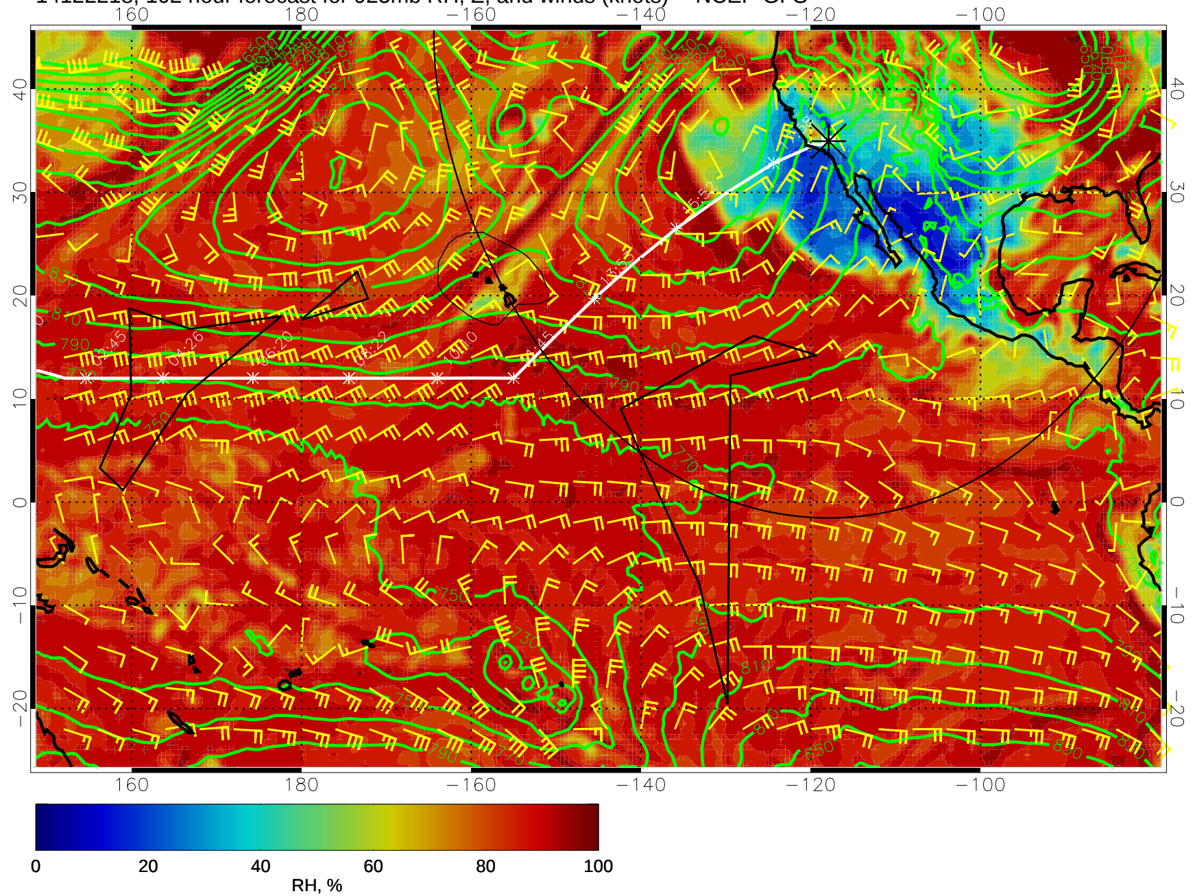
14122218, 102 hour forecast for 925mb RH, Z, and winds (knots) -- NCEP GFS
