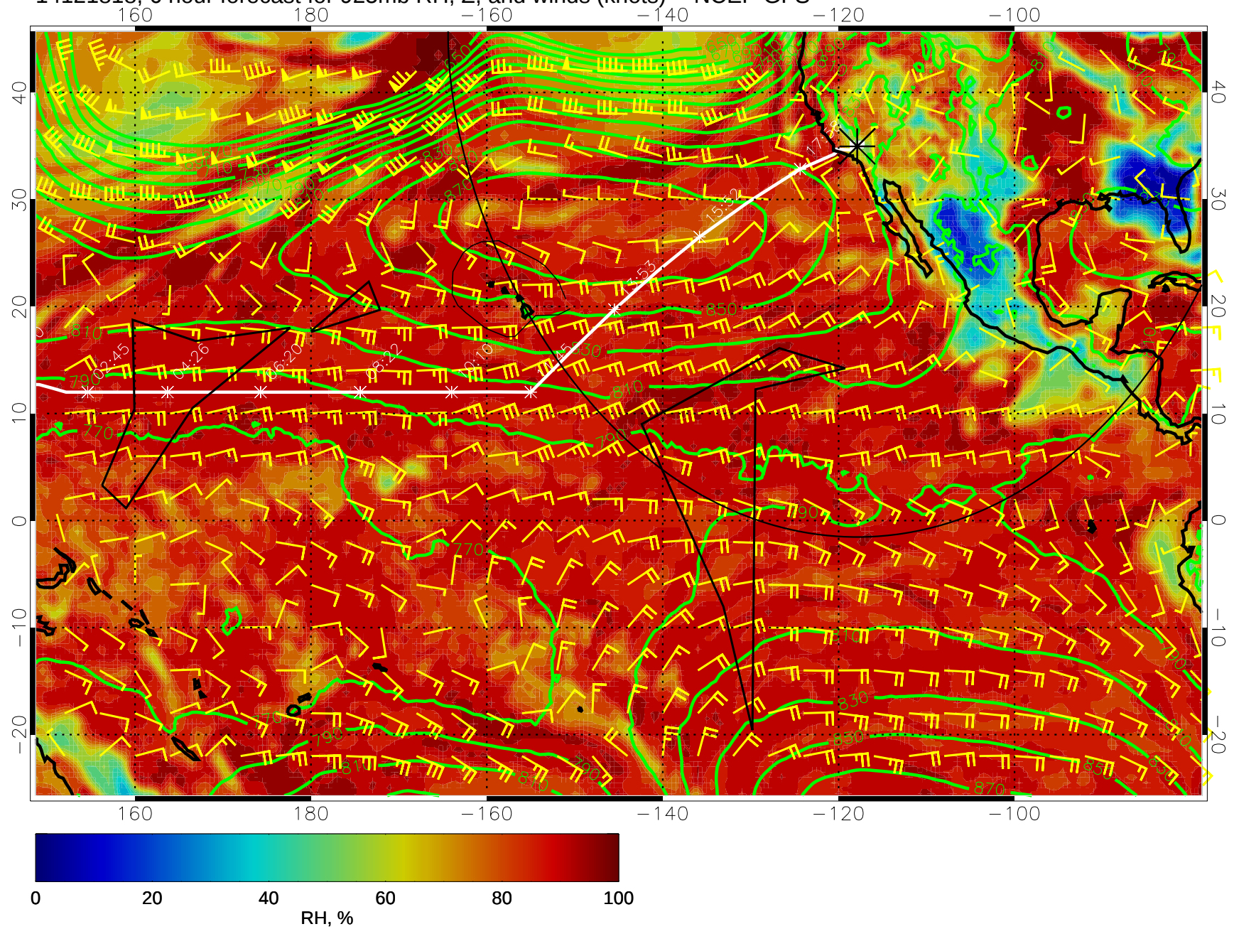
14121818, 6 hour forecast for 925mb RH, Z, and winds (knots) -- NCEP GFS
