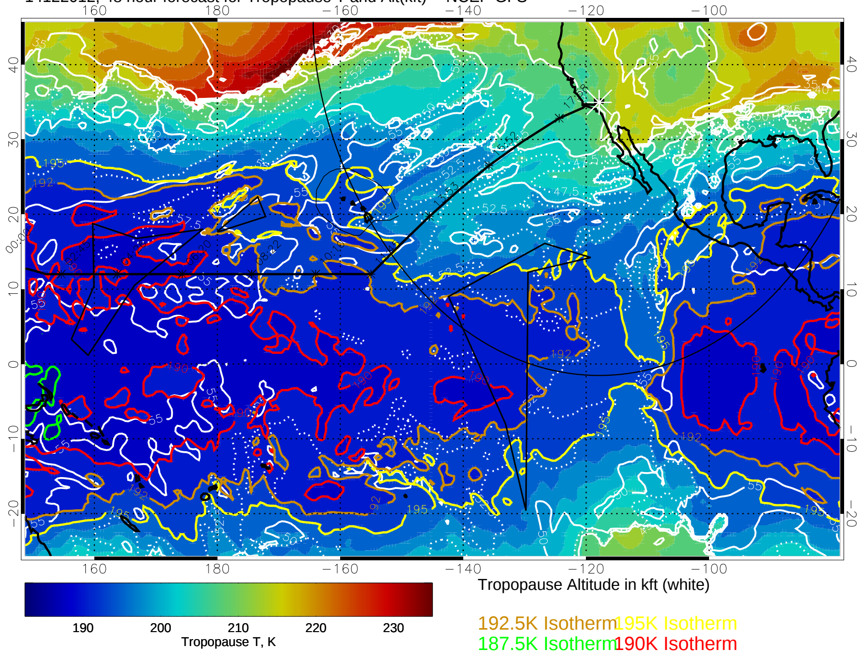
14122012, 48 hour forecast for Tropopause T and Alt(kft) -- NCEP GFS
