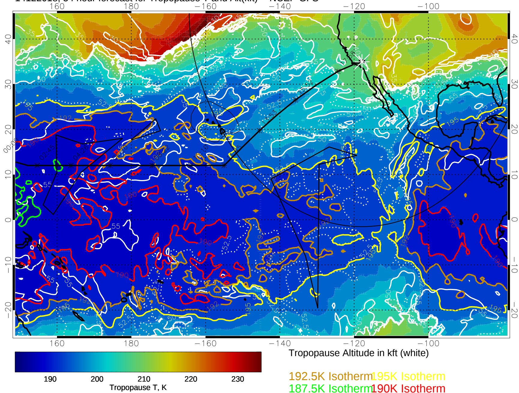
14122018, 54 hour forecast for Tropopause T and Alt(kft) -- NCEP GFS
