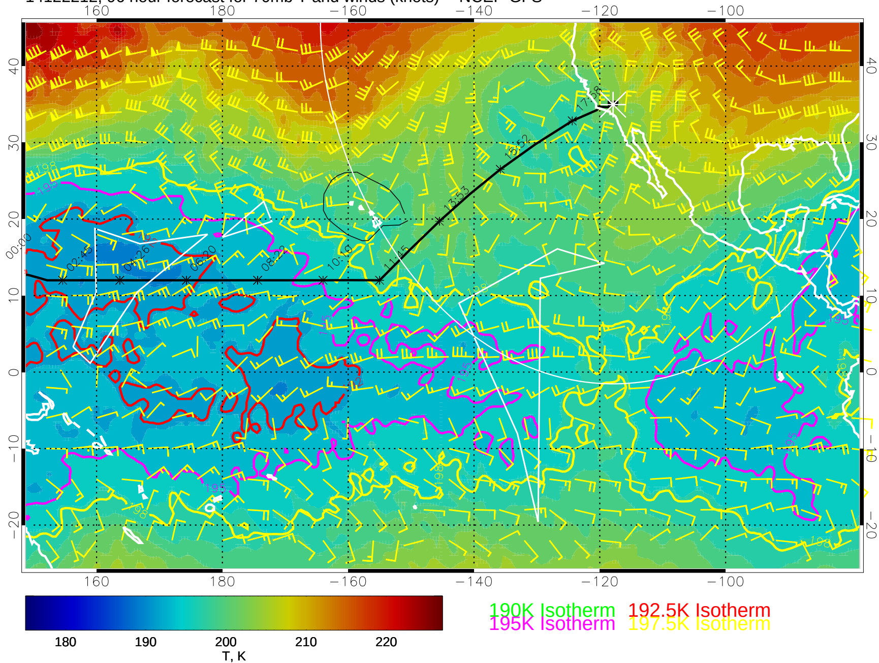
14122212, 96 hour forecast for 70mb T and winds (knots) -- NCEP GFS
