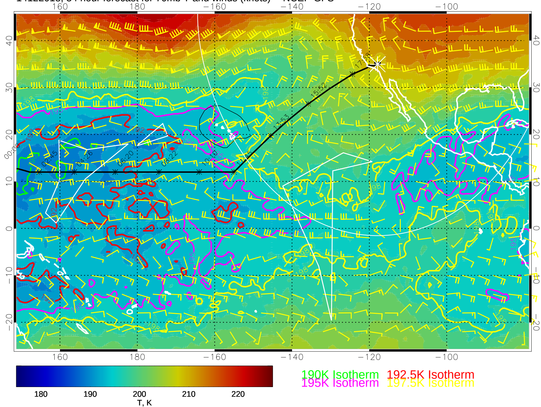
14122018, 54 hour forecast for 70mb T and winds (knots) -- NCEP GFS
