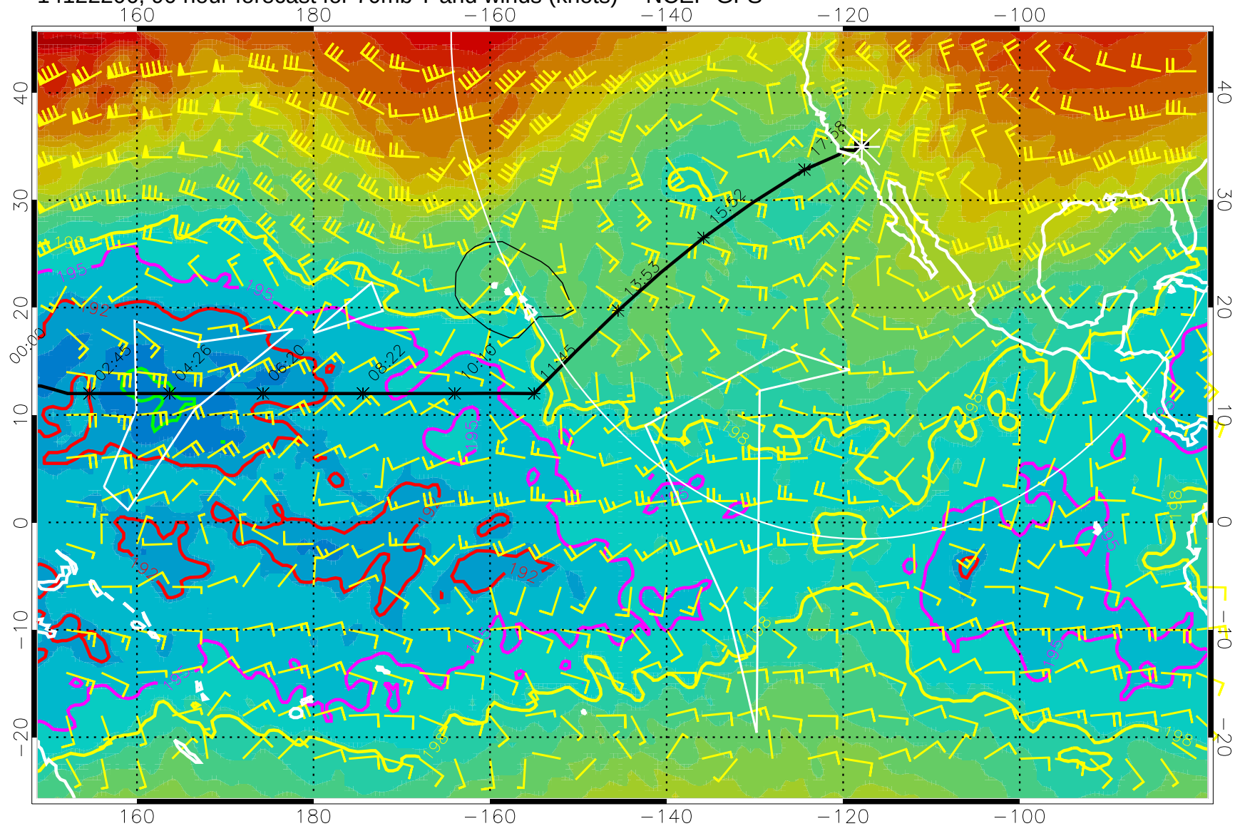
14122206, 90 hour forecast for 70mb T and winds (knots) -- NCEP GFS
