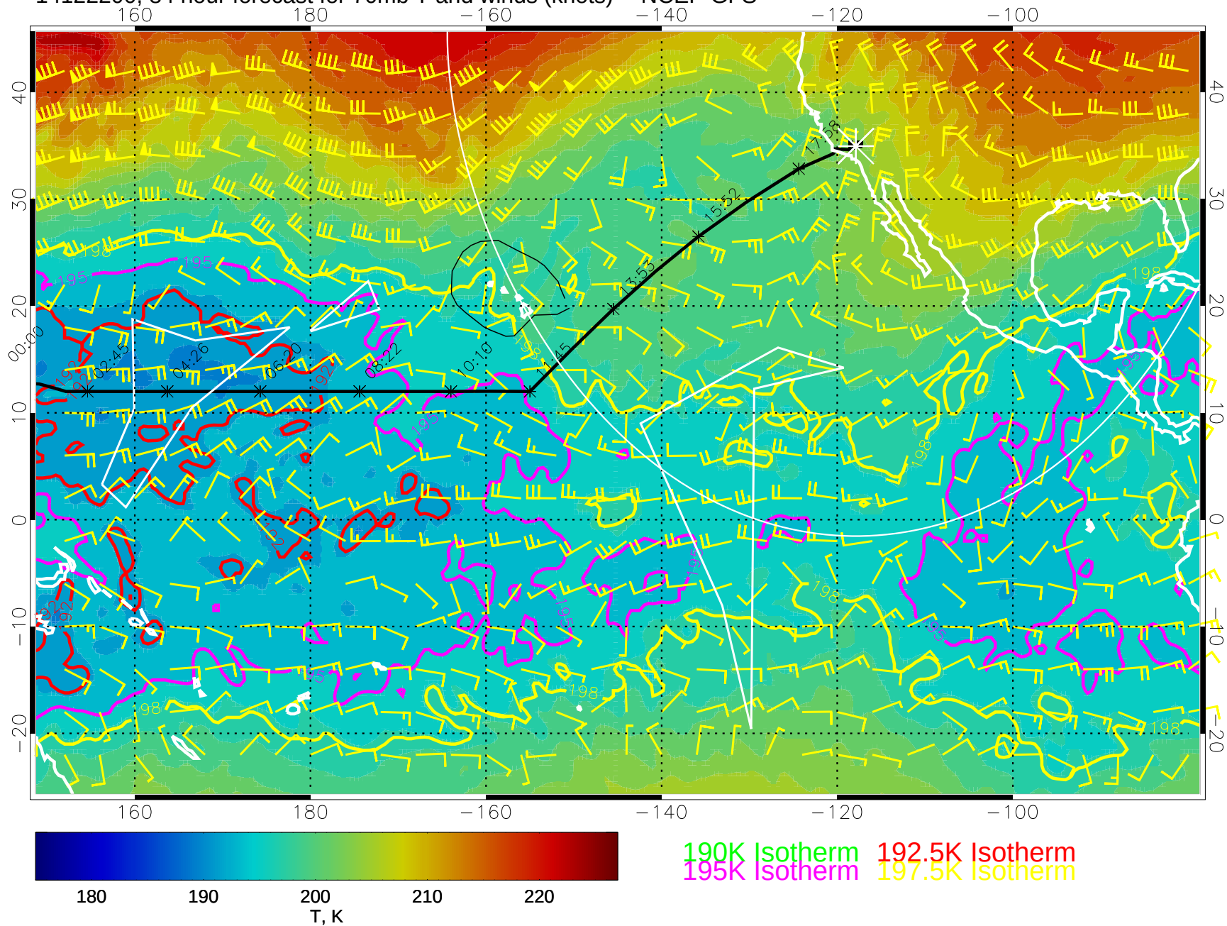
14122200, 84 hour forecast for 70mb T and winds (knots) -- NCEP GFS
