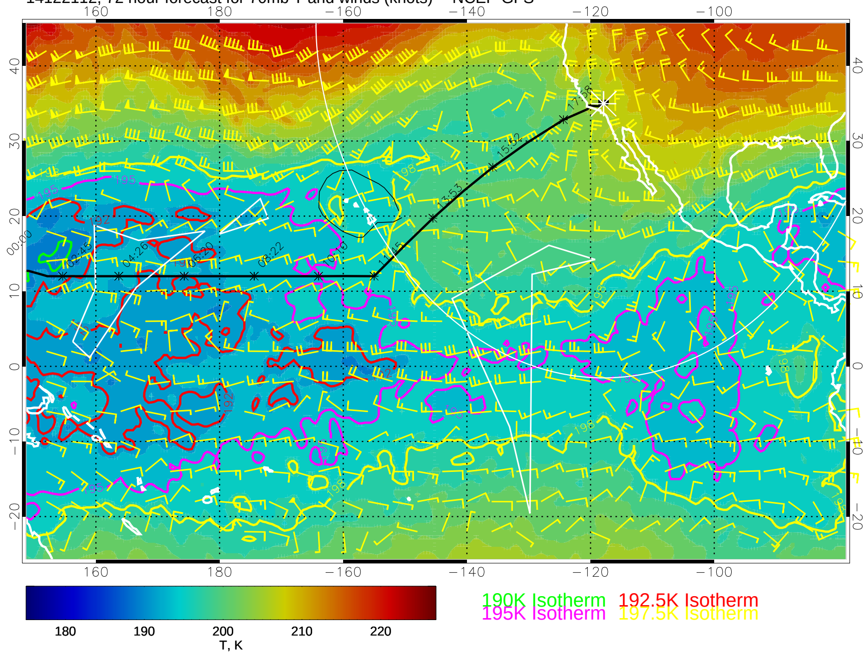
14122112, 72 hour forecast for 70mb T and winds (knots) -- NCEP GFS
