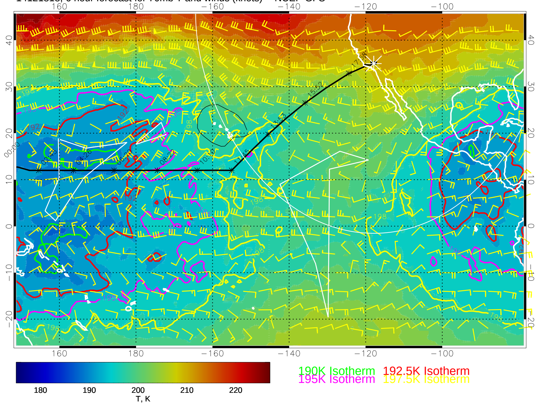
14121818, 6 hour forecast for 70mb T and winds (knots) -- NCEP GFS
