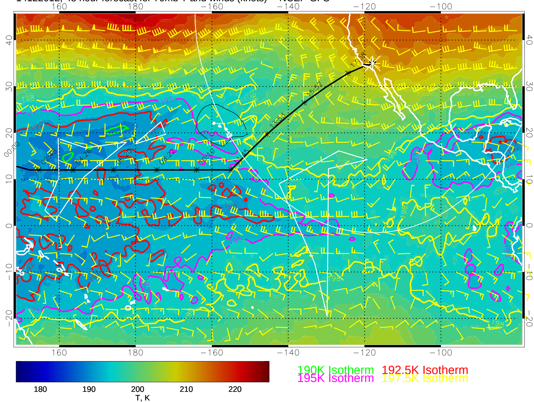
14122012, 48 hour forecast for 70mb T and winds (knots) -- NCEP GFS
