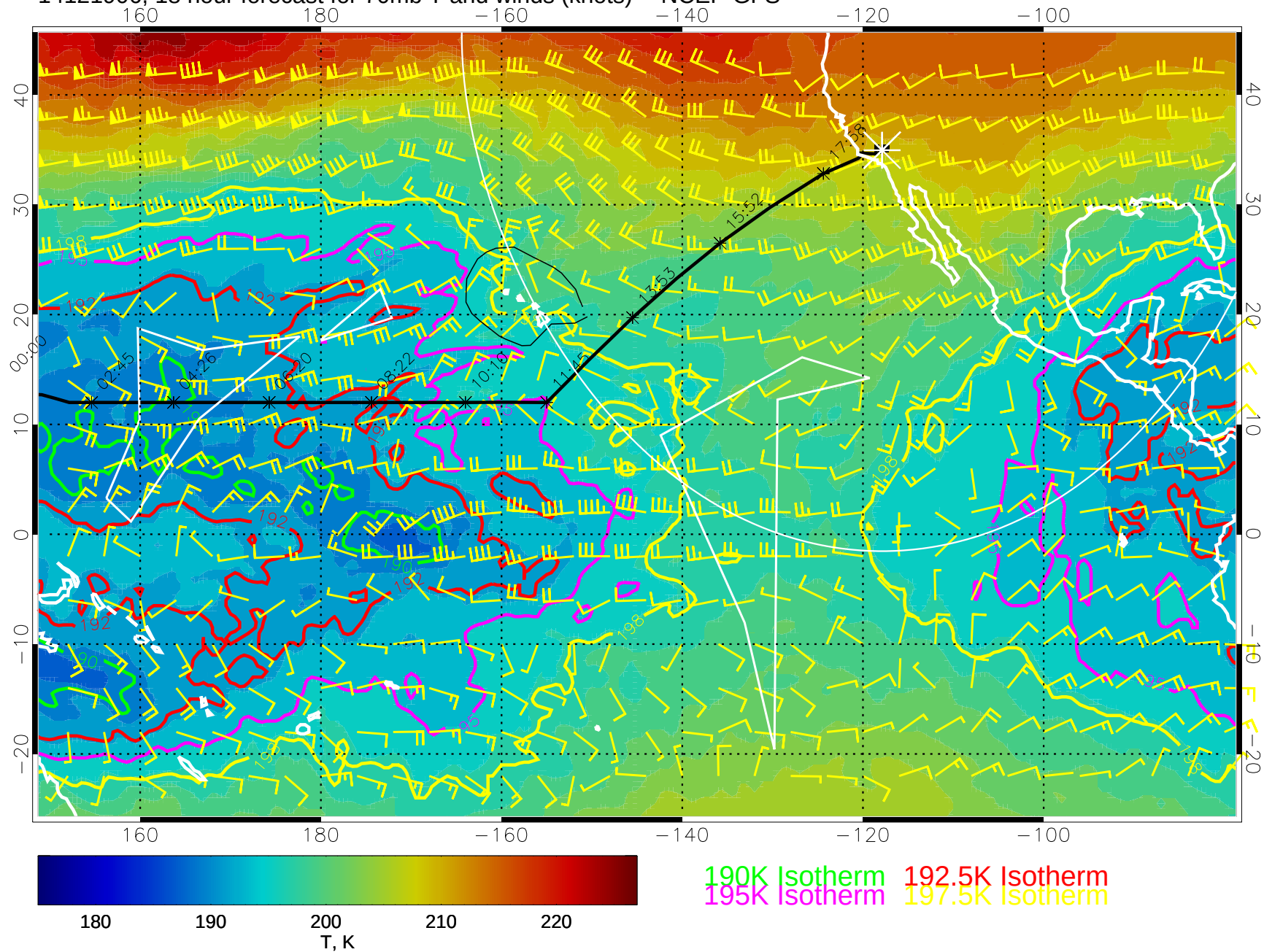
14121906, 18 hour forecast for 70mb T and winds (knots) -- NCEP GFS
