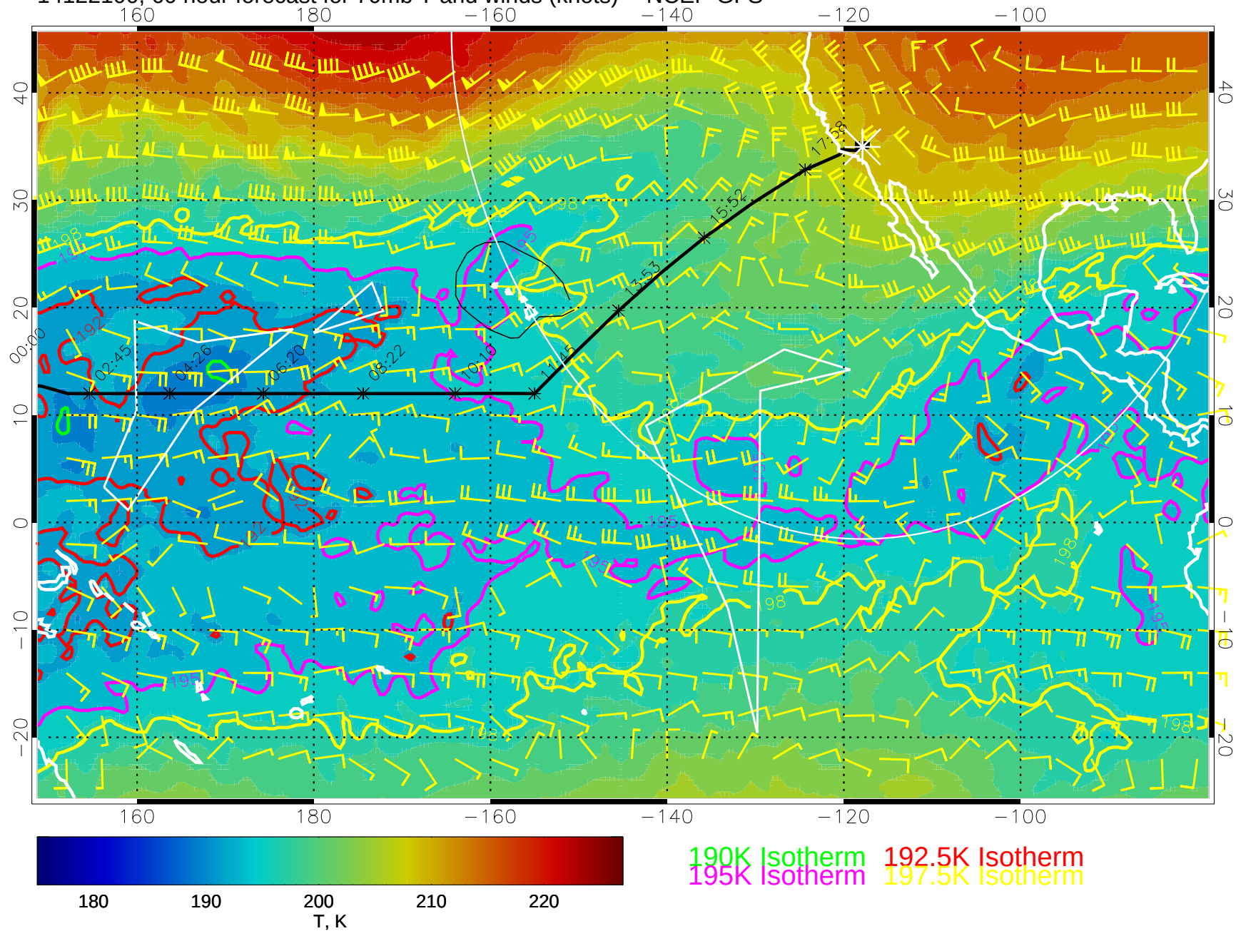
14122100, 60 hour forecast for 70mb T and winds (knots) -- NCEP GFS
