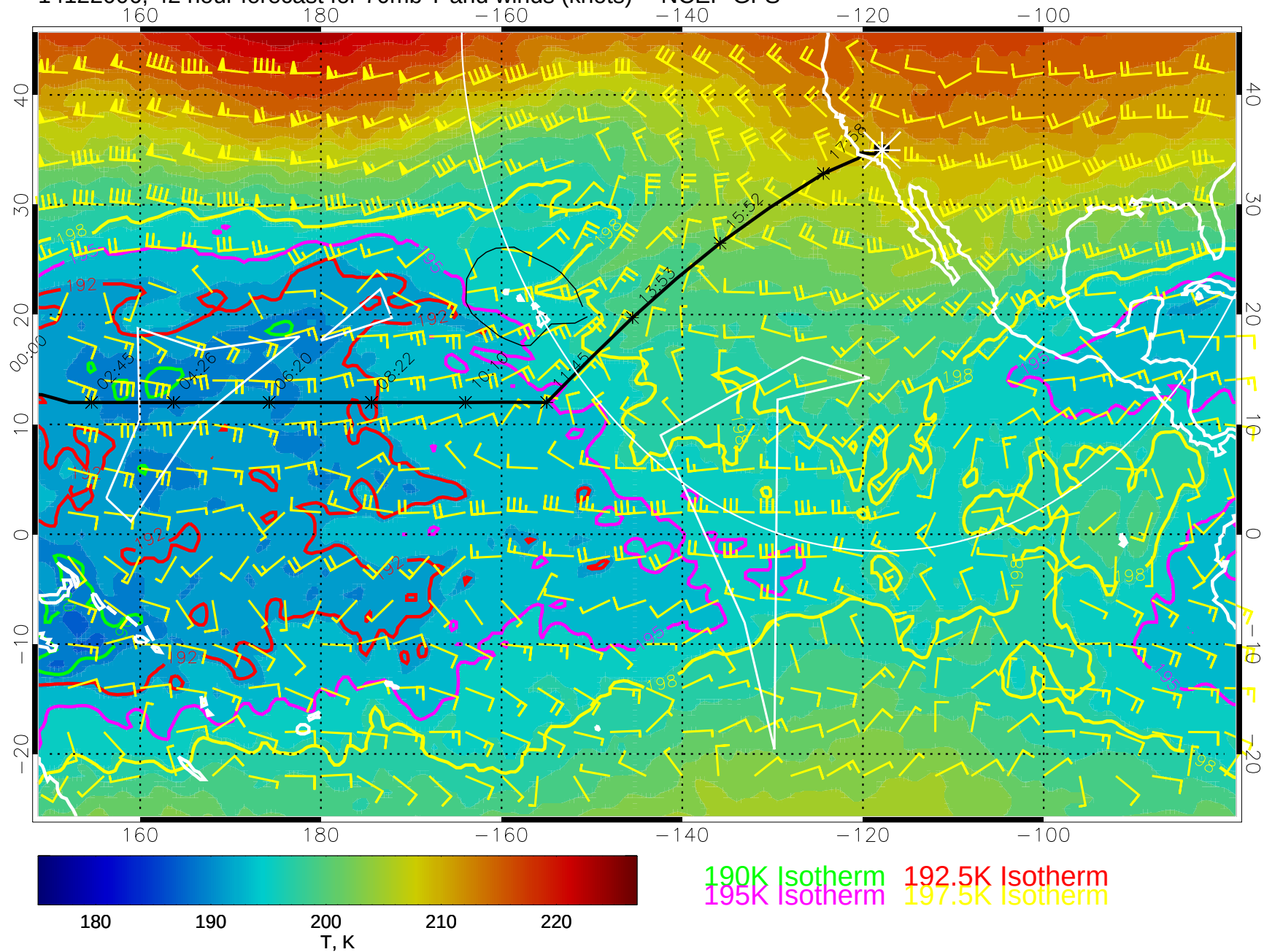
14122006, 42 hour forecast for 70mb T and winds (knots) -- NCEP GFS
