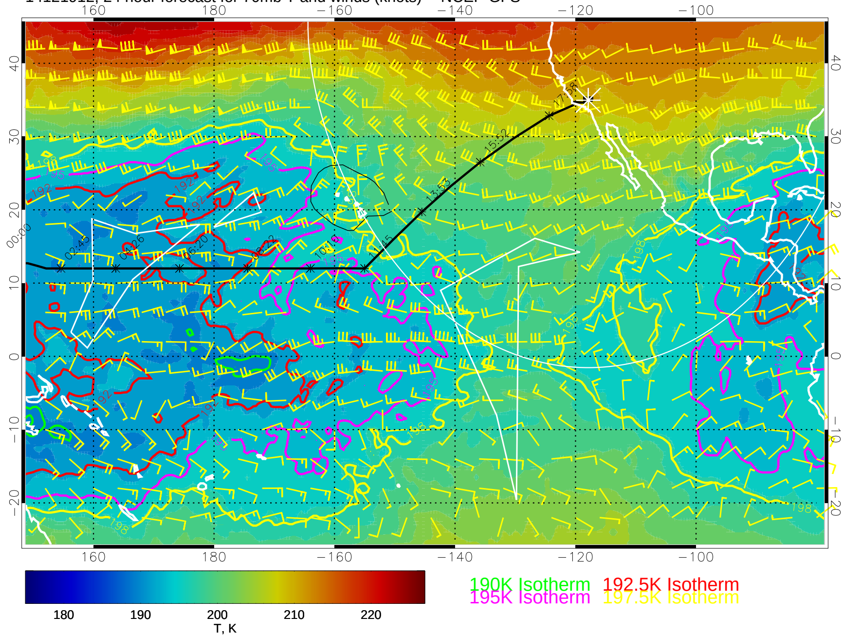
14121912, 24 hour forecast for 70mb T and winds (knots) -- NCEP GFS
