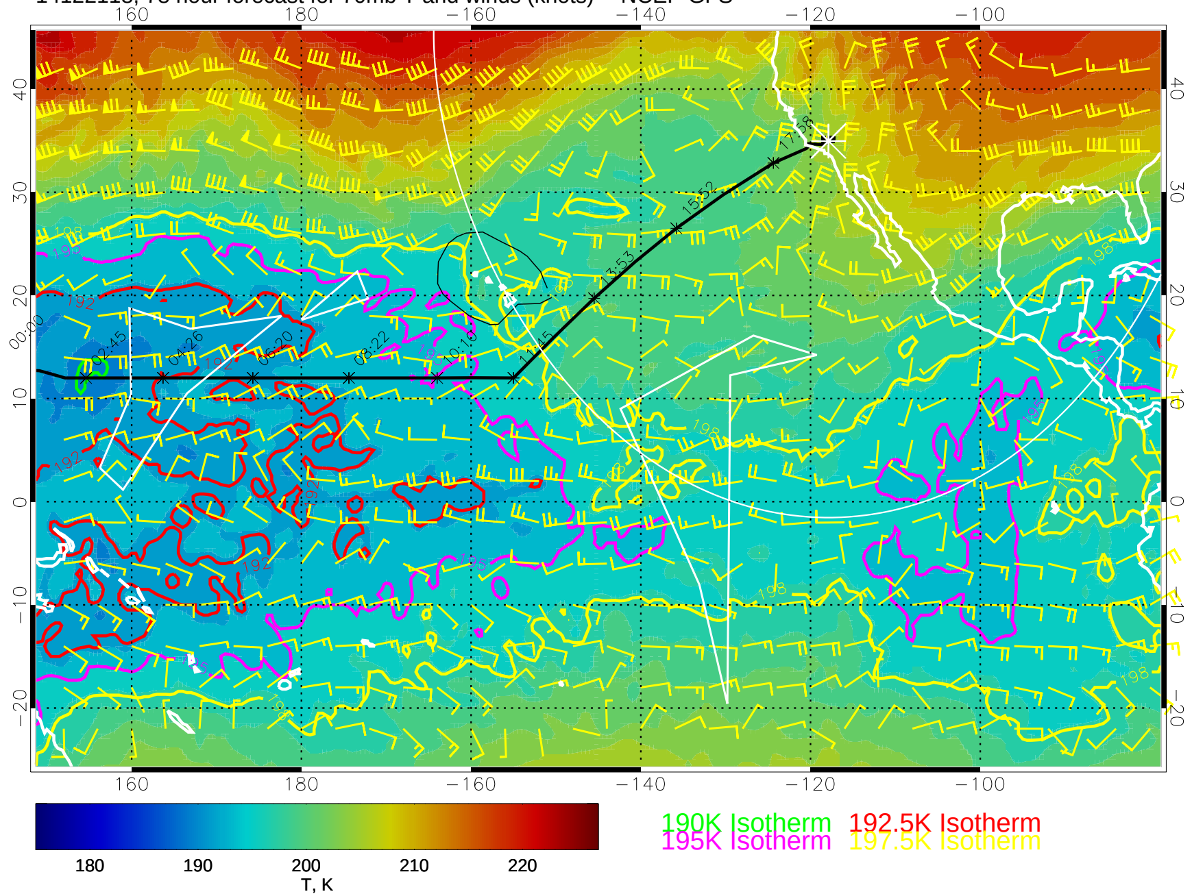
14122118, 78 hour forecast for 70mb T and winds (knots) -- NCEP GFS
