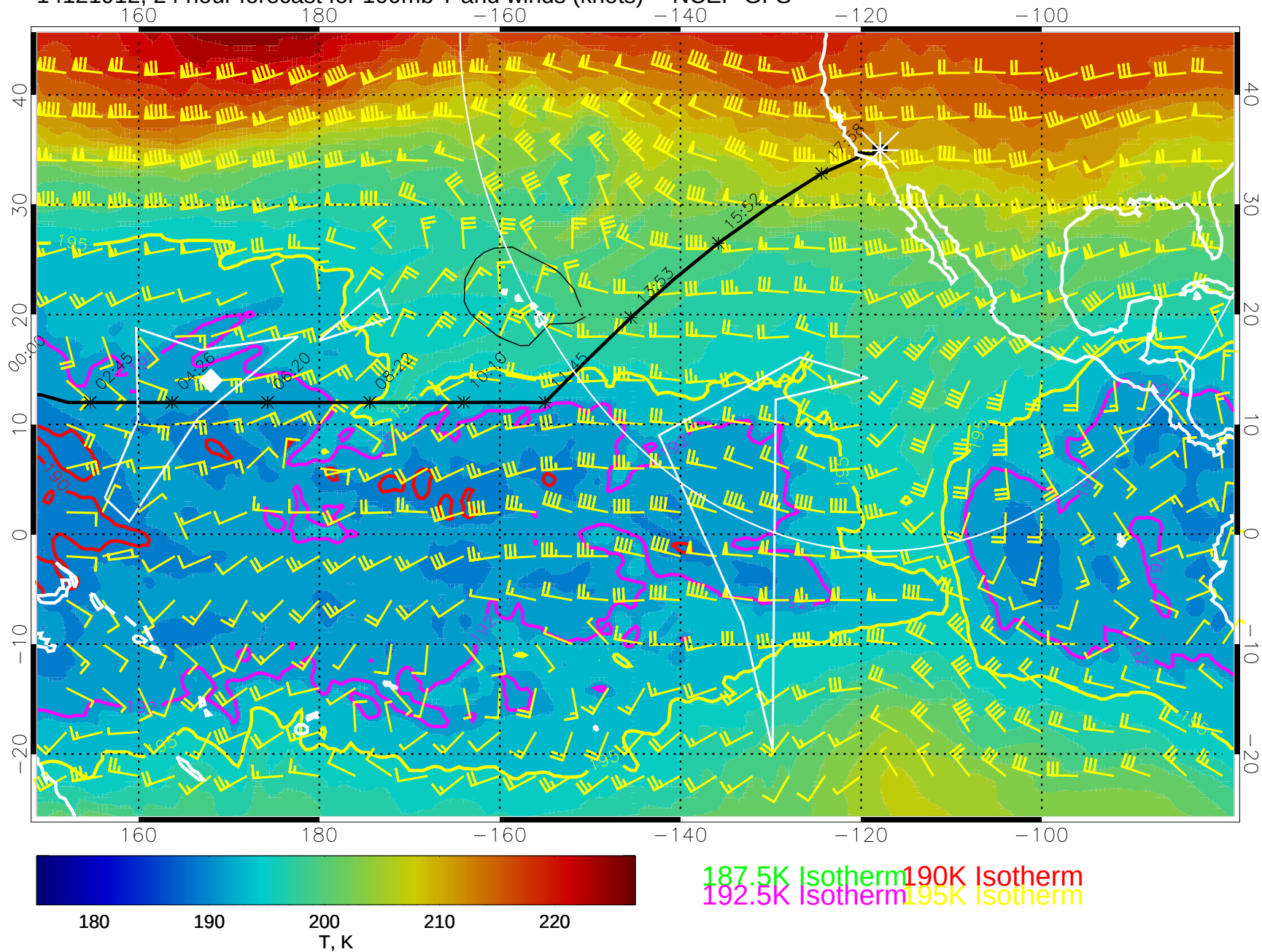
14121912, 24 hour forecast for 100mb T and winds (knots) -- NCEP GFS
