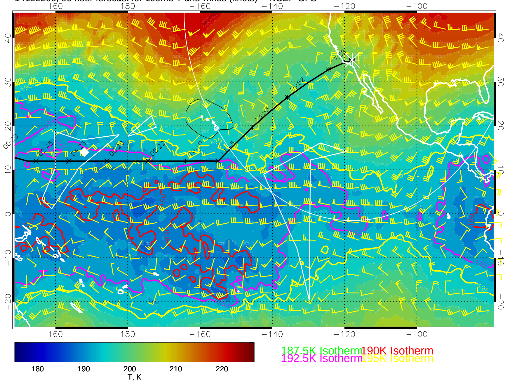
14122206, 90 hour forecast for 100mb T and winds (knots) -- NCEP GFS
