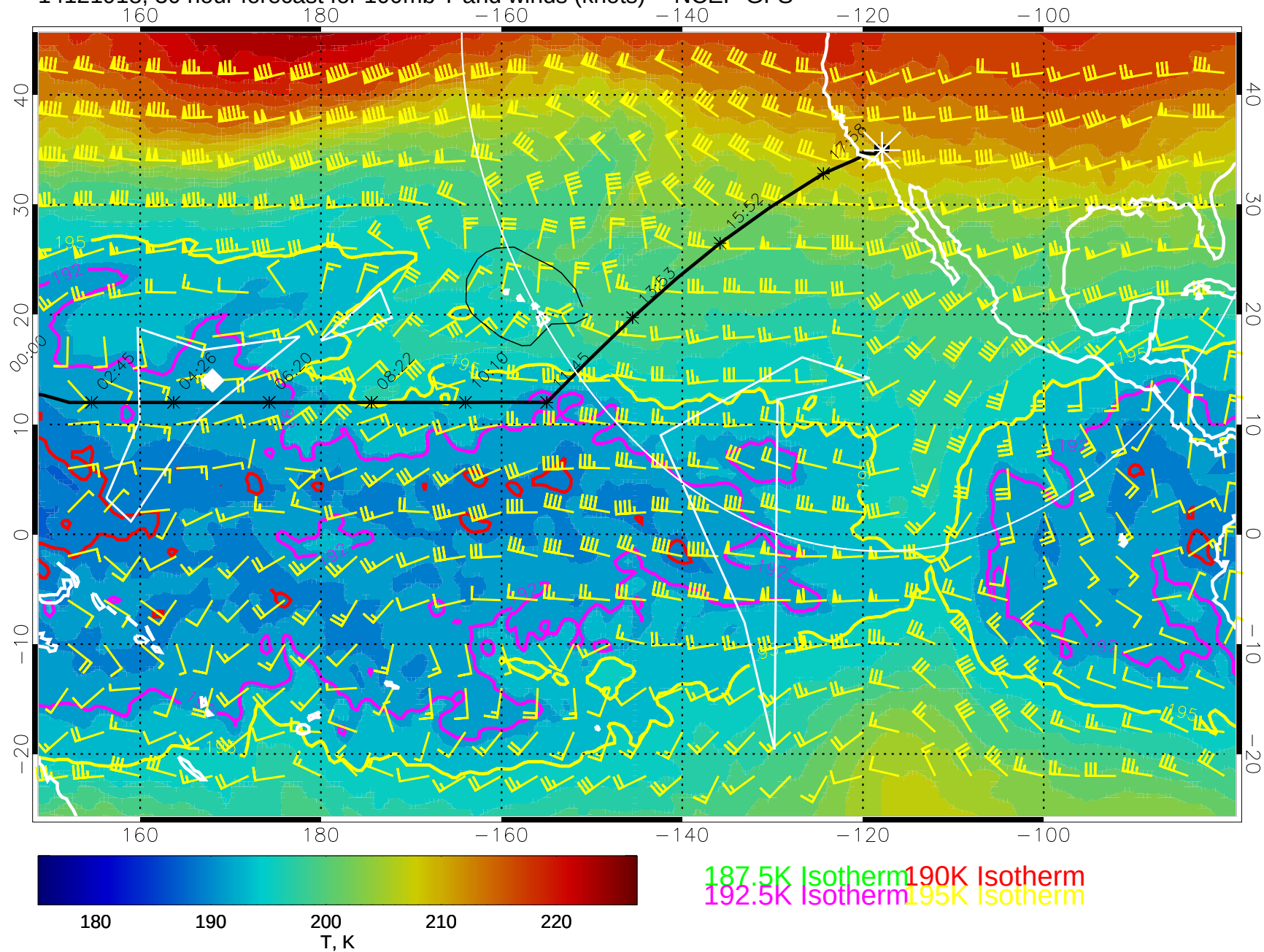
14121918, 30 hour forecast for 100mb T and winds (knots) -- NCEP GFS
