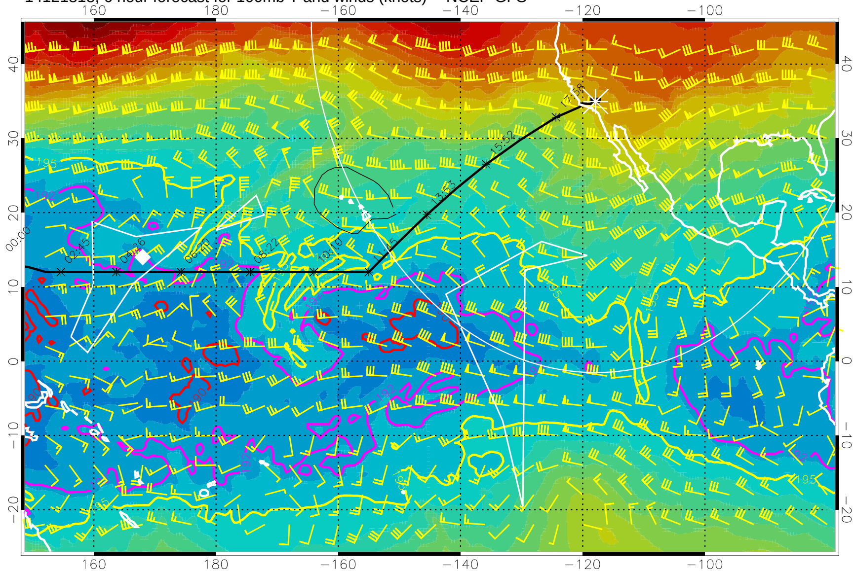
14121818, 6 hour forecast for 100mb T and winds (knots) -- NCEP GFS
