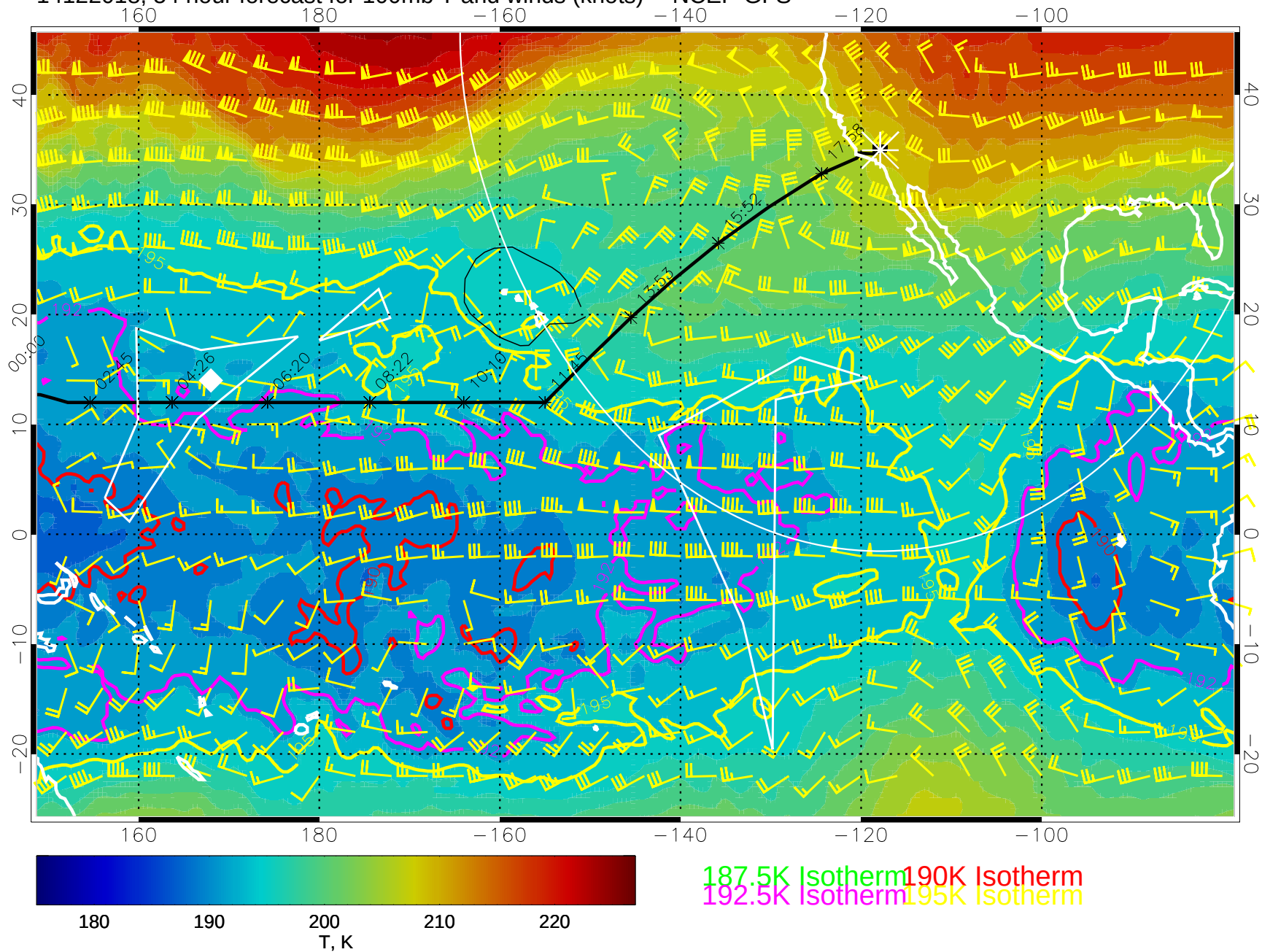
14122018, 54 hour forecast for 100mb T and winds (knots) -- NCEP GFS
