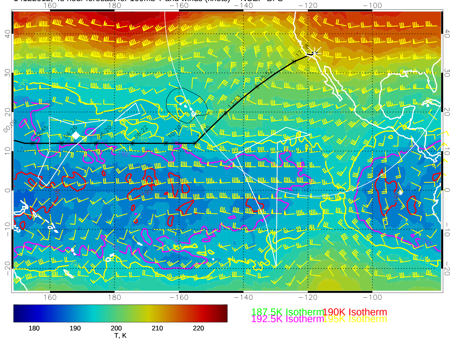
14122012, 48 hour forecast for 100mb T and winds (knots) -- NCEP GFS
