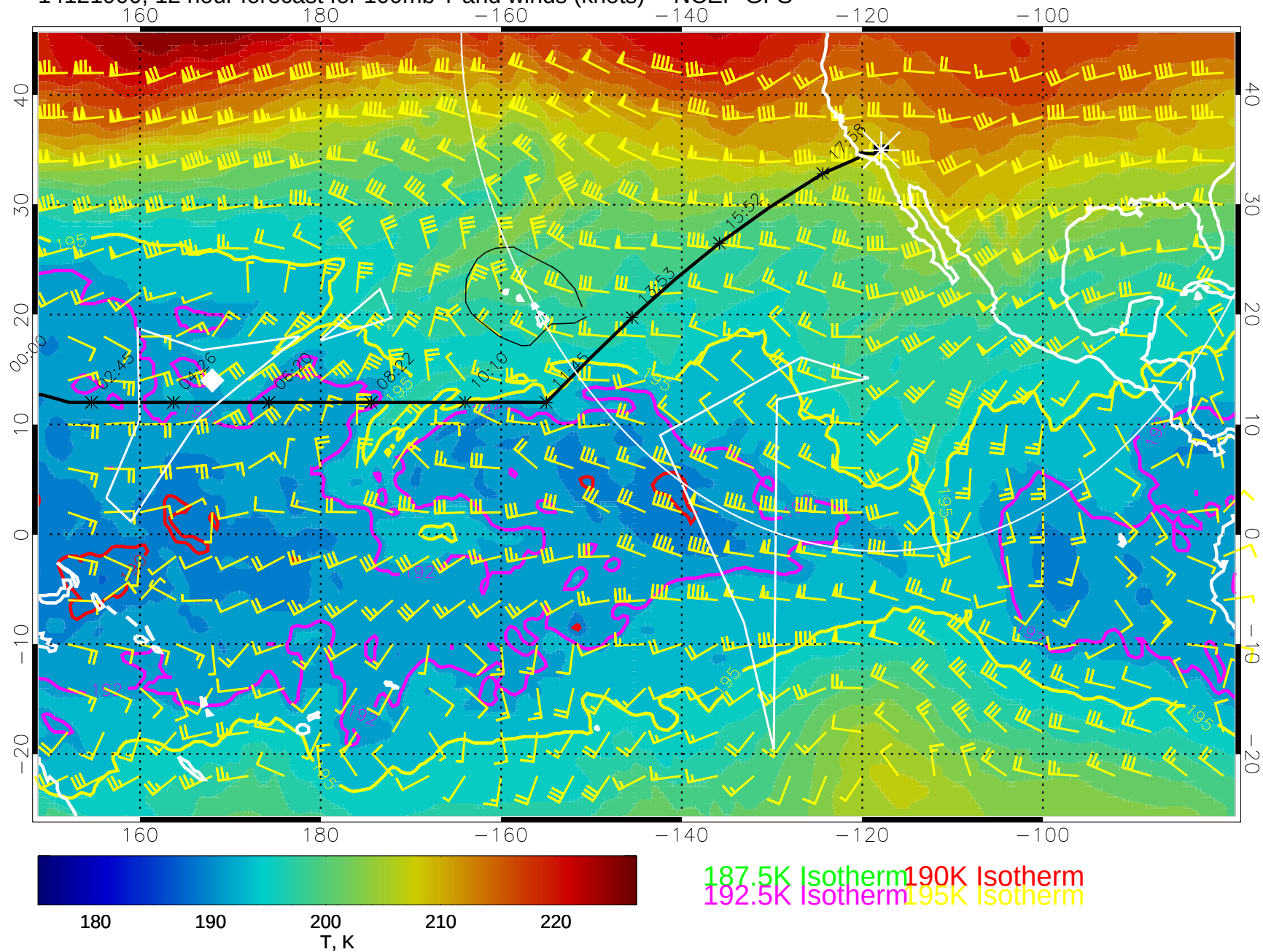
14121900, 12 hour forecast for 100mb T and winds (knots) -- NCEP GFS
