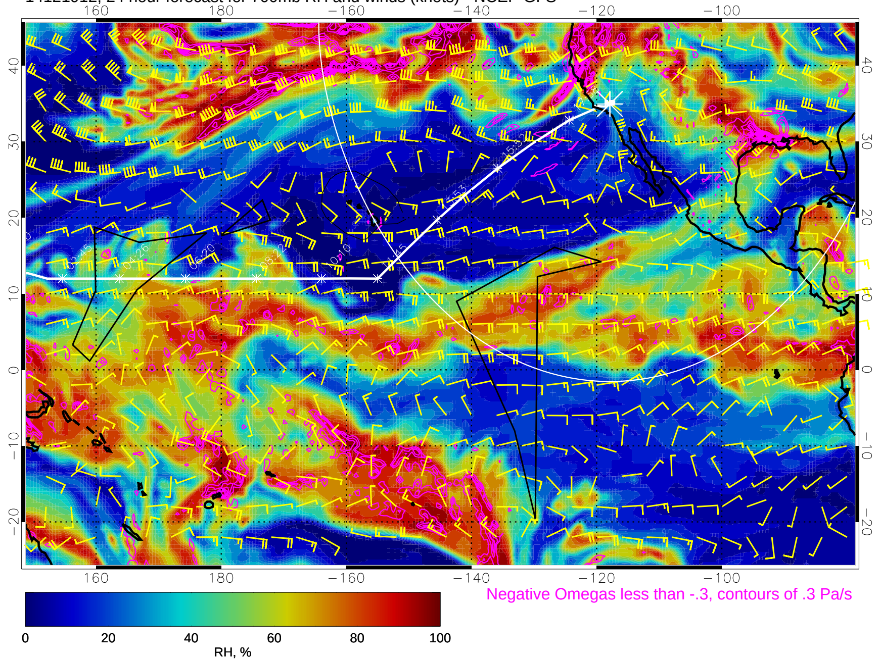
14121912, 24 hour forecast for 700mb RH and winds (knots) - NCEP GFS
