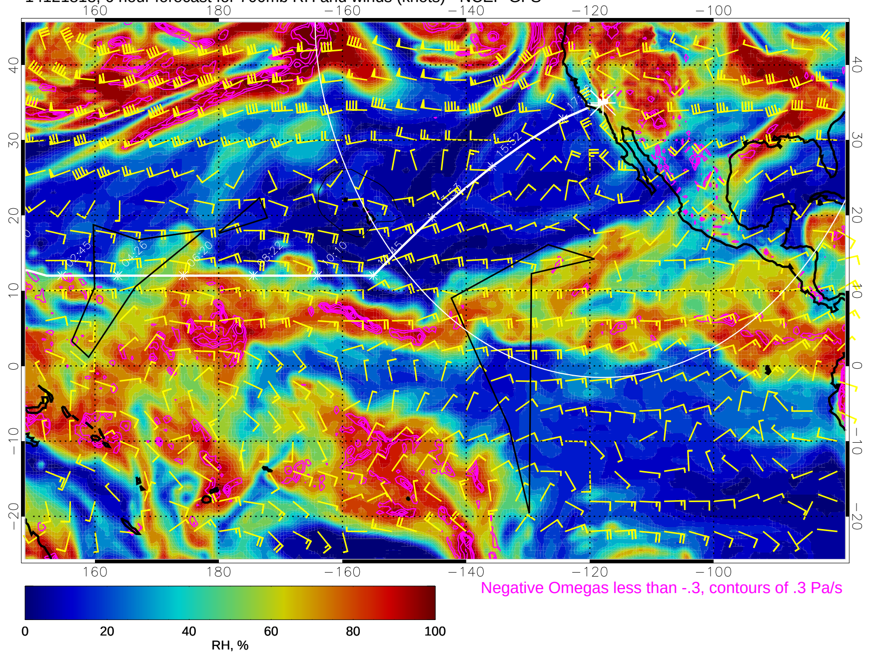
14121818, 6 hour forecast for 700mb RH and winds (knots) - NCEP GFS
