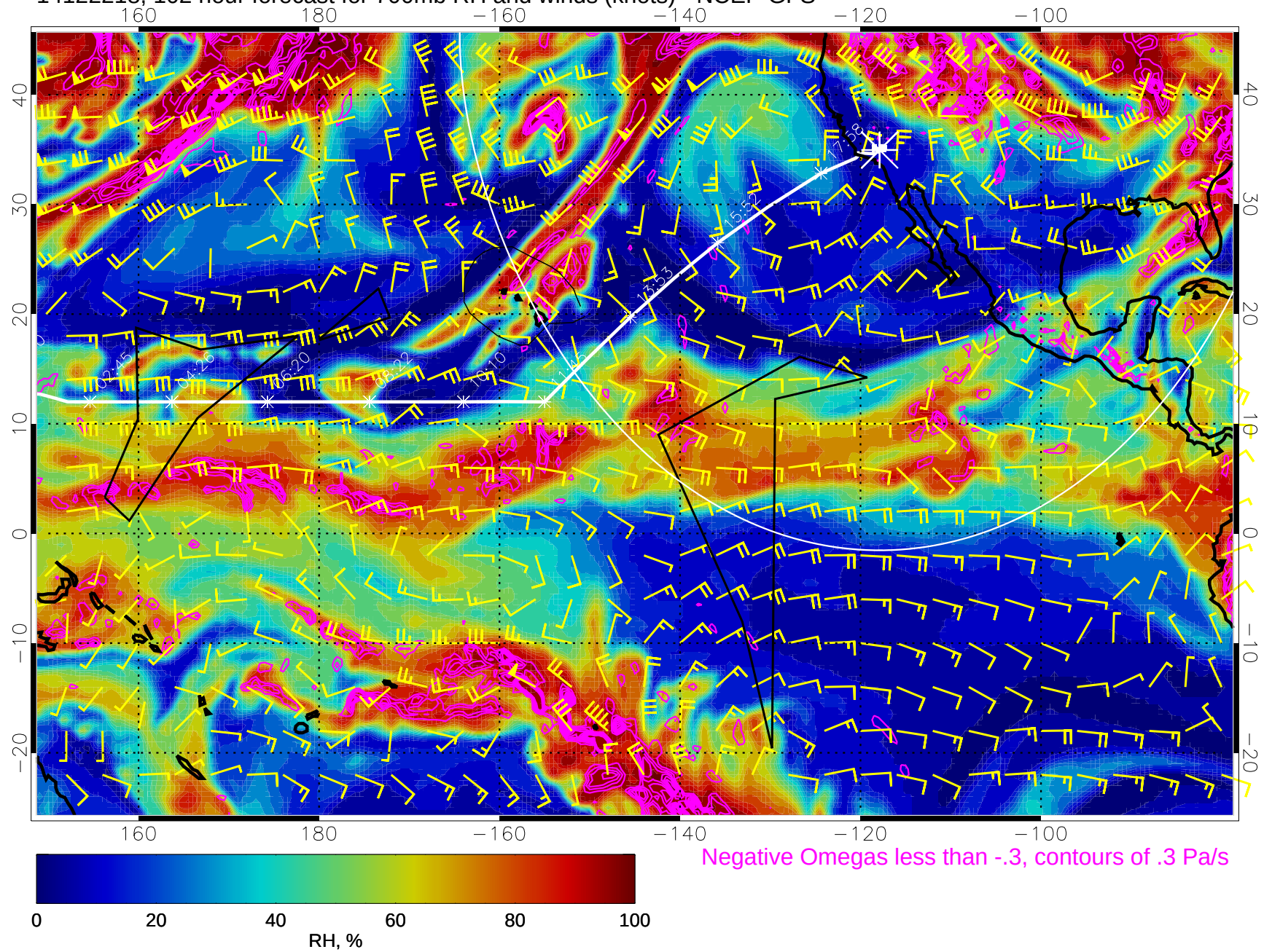
14122218, 102 hour forecast for 700mb RH and winds (knots) - NCEP GFS
