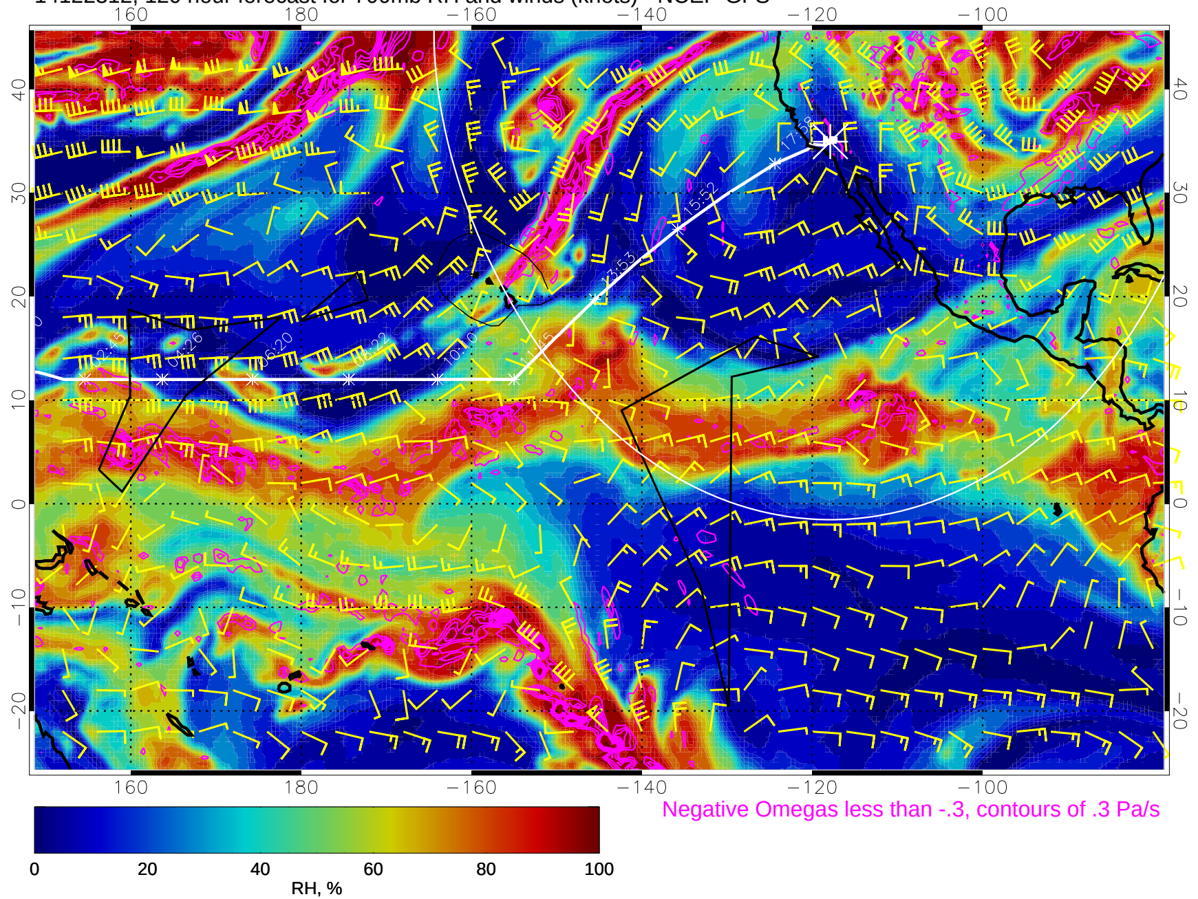
14122312, 120 hour forecast for 700mb RH and winds (knots) - NCEP GFS
