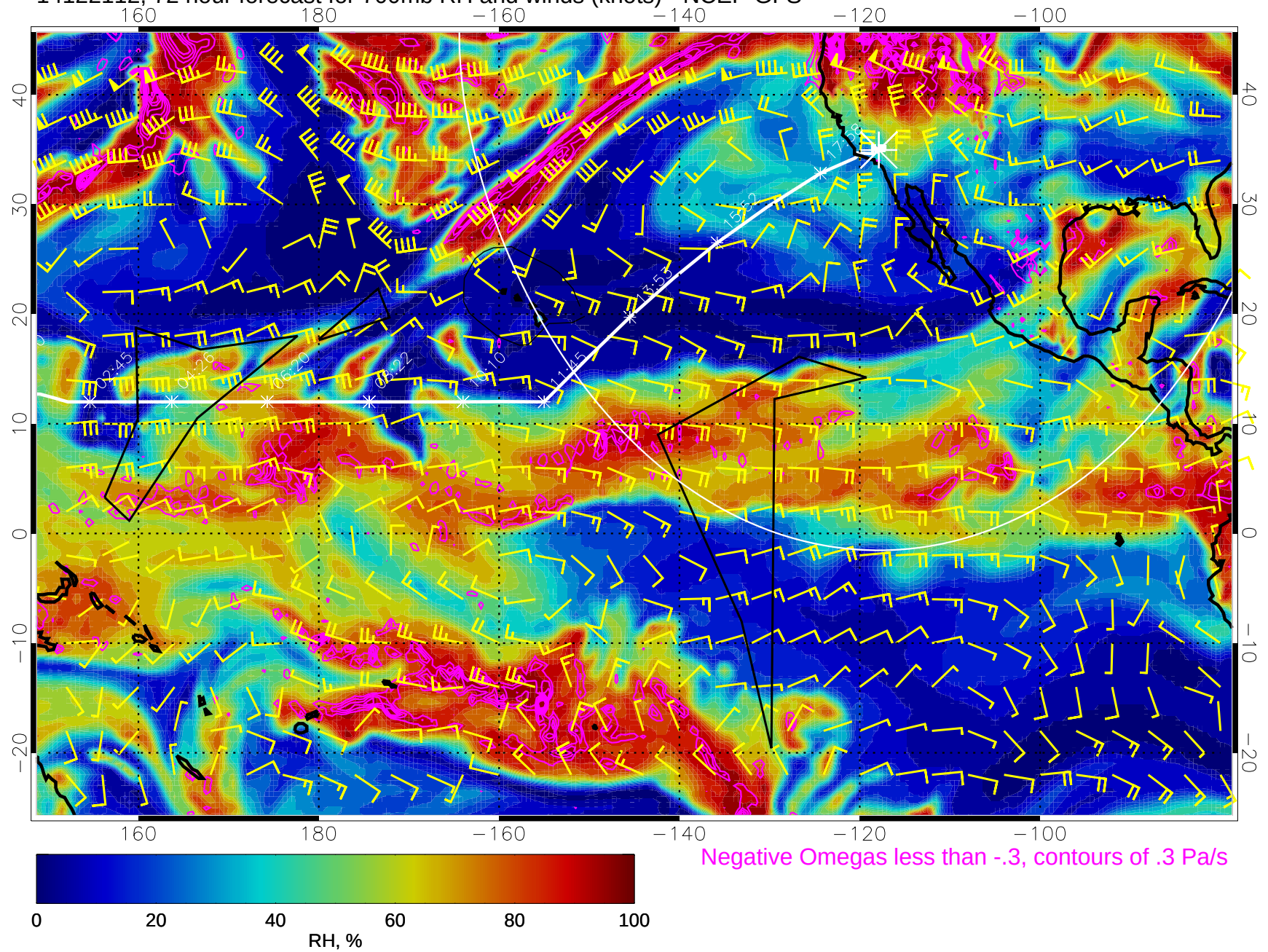
14122112, 72 hour forecast for 700mb RH and winds (knots) - NCEP GFS
