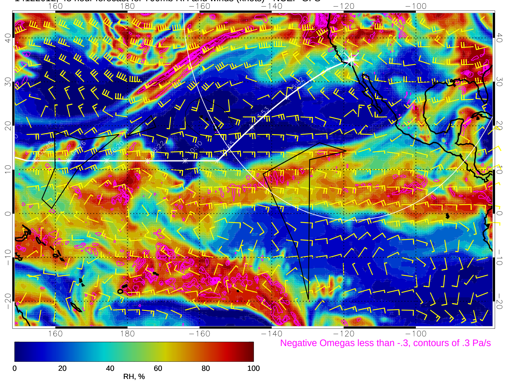
14122012, 48 hour forecast for 700mb RH and winds (knots) - NCEP GFS
