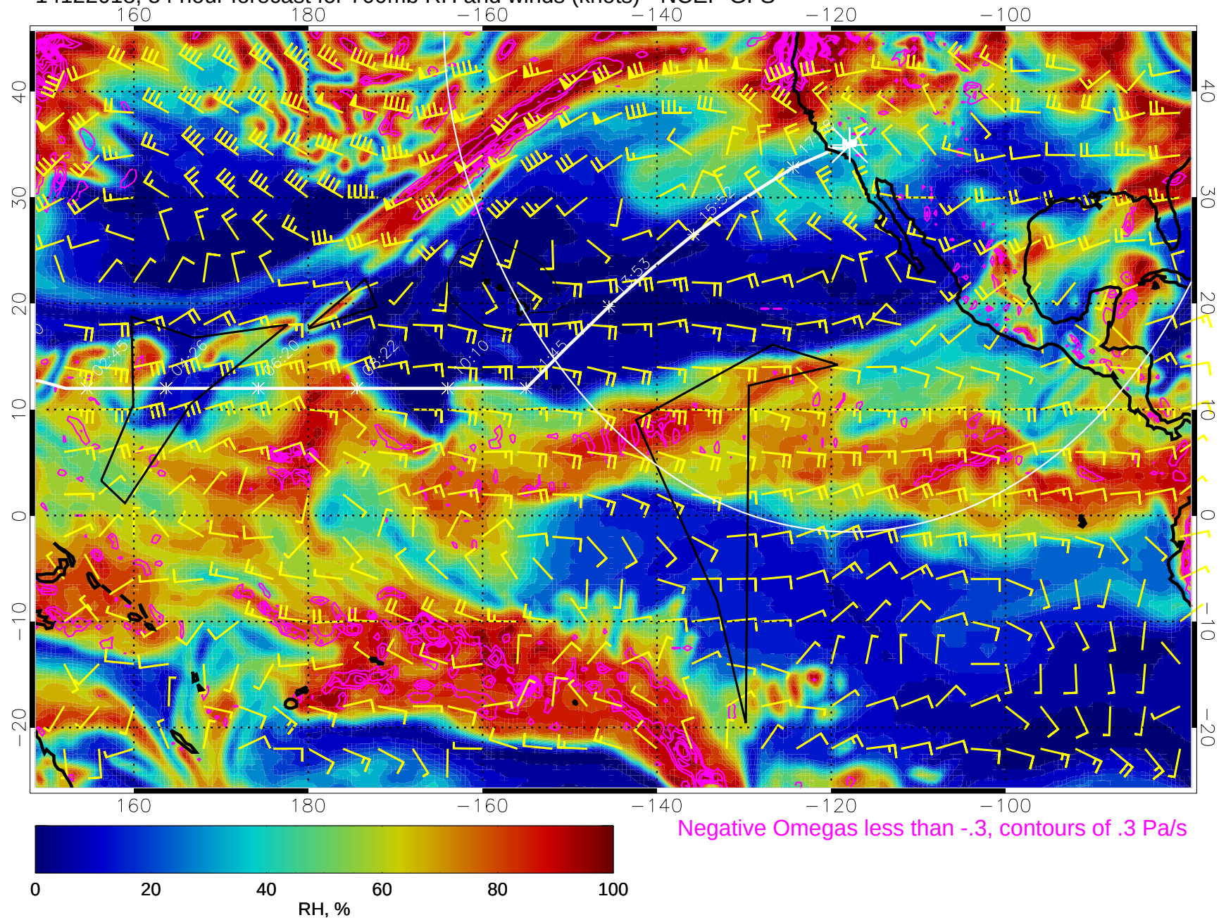
14122018, 54 hour forecast for 700mb RH and winds (knots) - NCEP GFS
