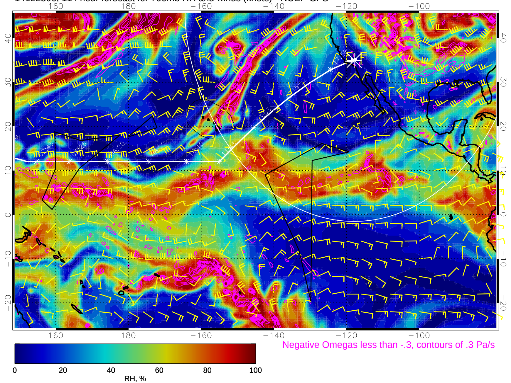
14122306, 114 hour forecast for 700mb RH and winds (knots) - NCEP GFS
