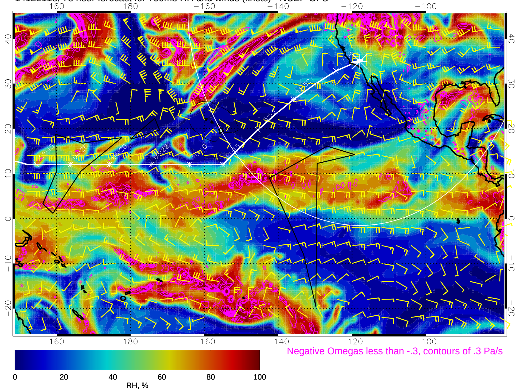
14122118, 78 hour forecast for 700mb RH and winds (knots) - NCEP GFS
