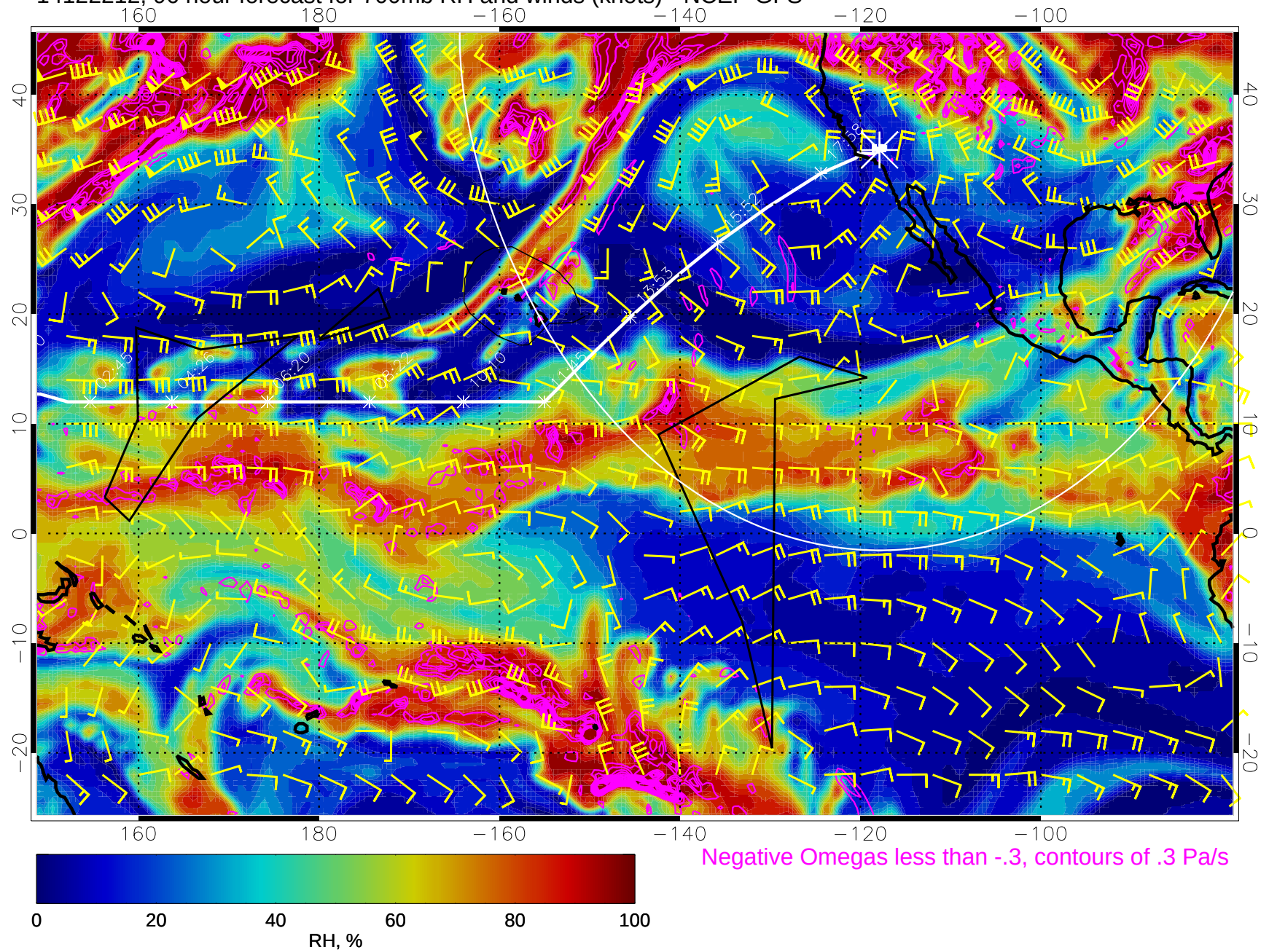
14122212, 96 hour forecast for 700mb RH and winds (knots) - NCEP GFS
