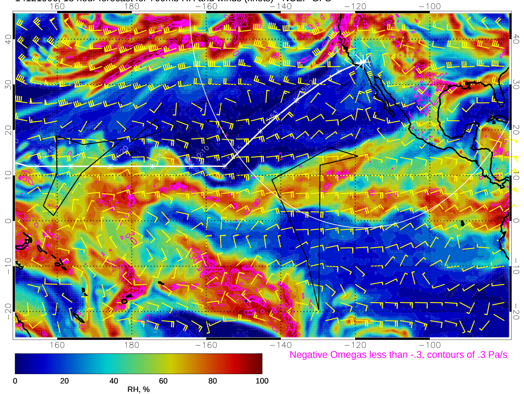
14121906, 18 hour forecast for 700mb RH and winds (knots) - NCEP GFS
