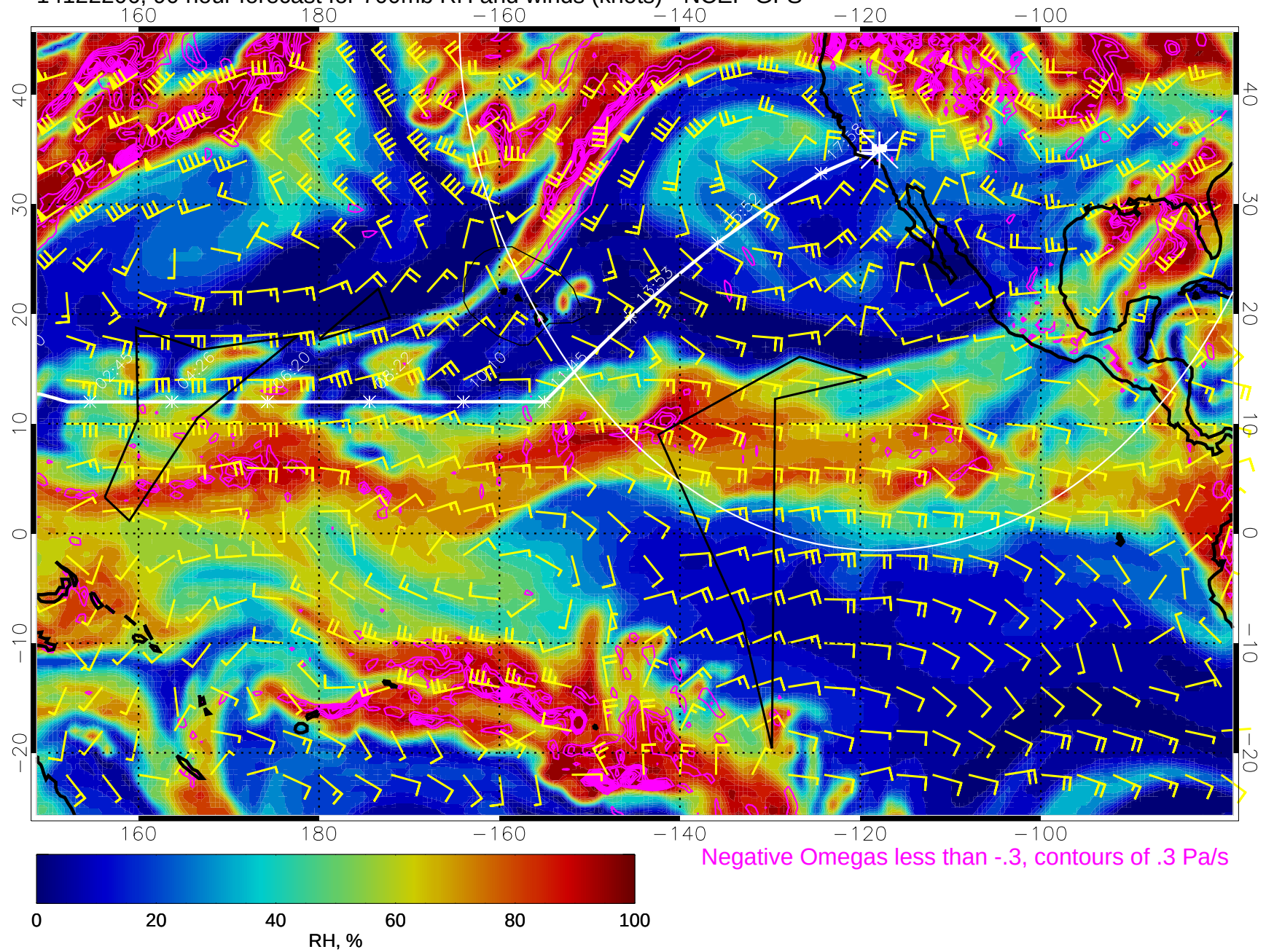
14122206, 90 hour forecast for 700mb RH and winds (knots) - NCEP GFS
