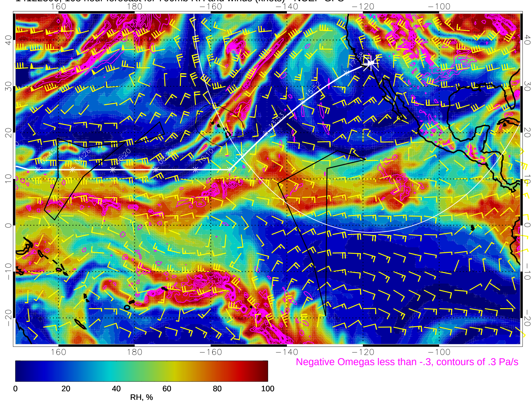
14122300, 108 hour forecast for 700mb RH and winds (knots) - NCEP GFS
