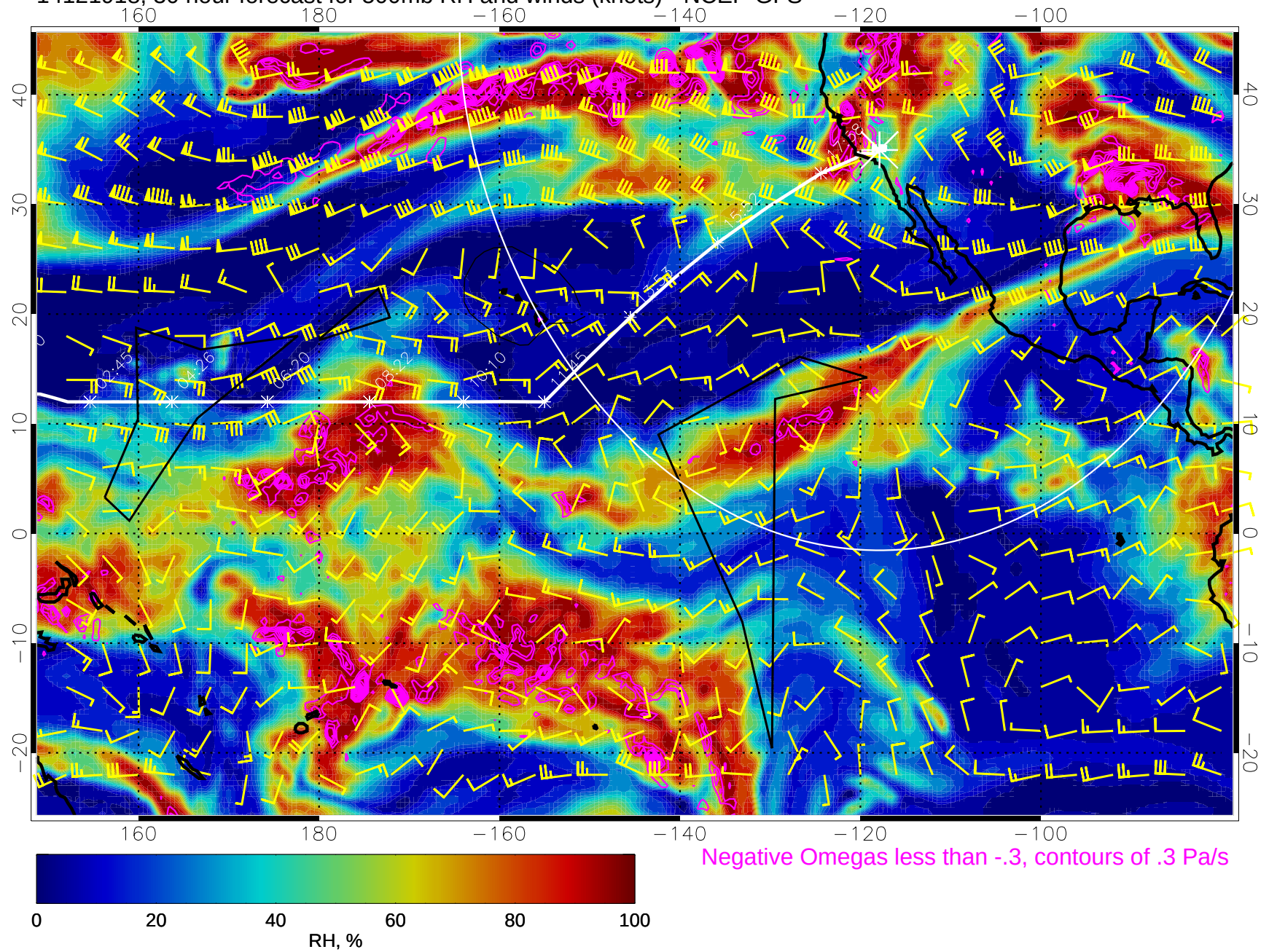
14121918, 30 hour forecast for 500mb RH and winds (knots) - NCEP GFS
