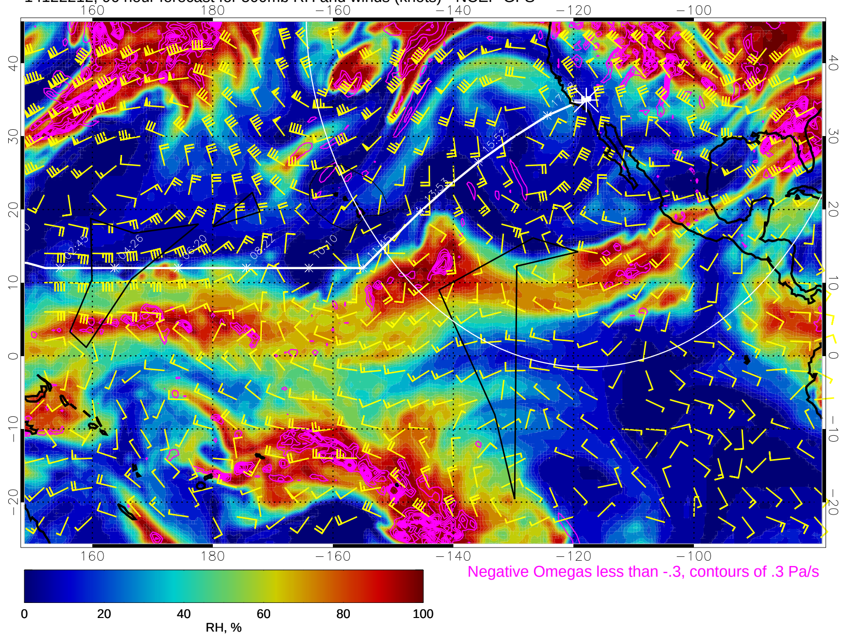
14122212, 96 hour forecast for 500mb RH and winds (knots) - NCEP GFS
