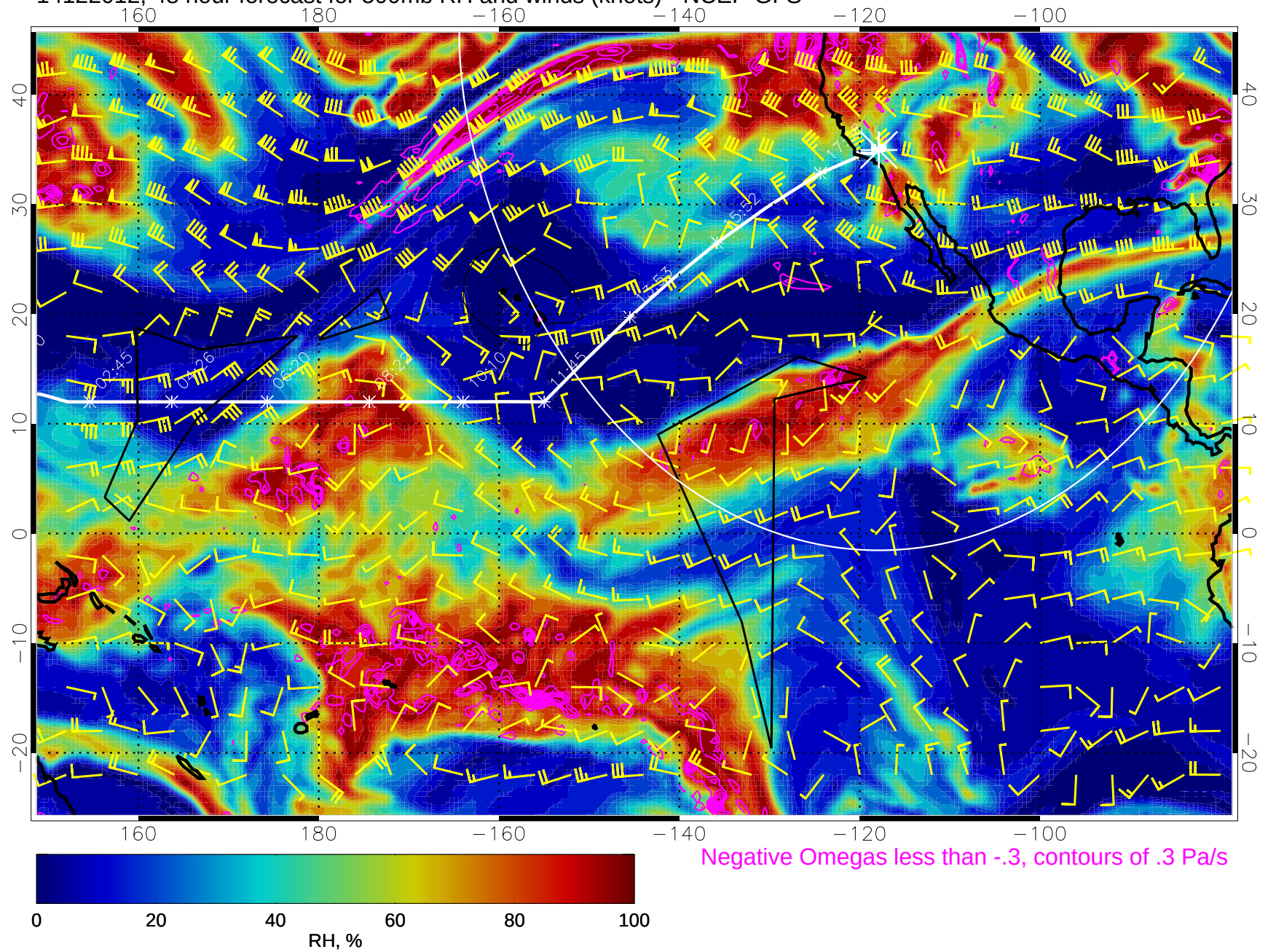
14122012, 48 hour forecast for 500mb RH and winds (knots) - NCEP GFS
