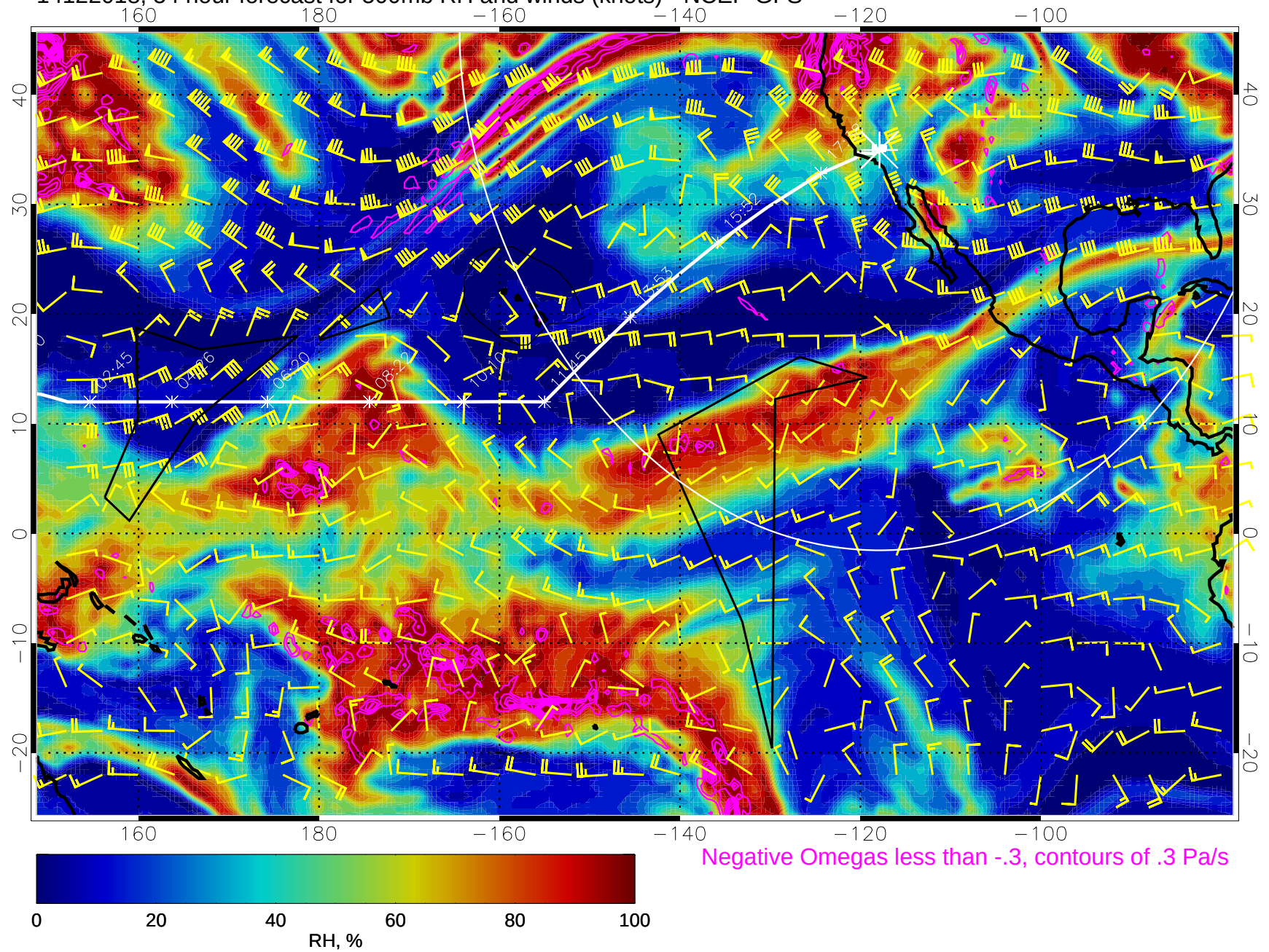
14122018, 54 hour forecast for 500mb RH and winds (knots) - NCEP GFS
