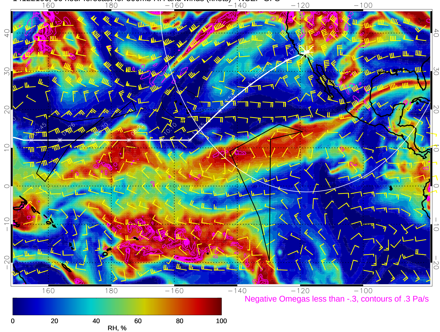
14122106, 66 hour forecast for 500mb RH and winds (knots) - NCEP GFS
