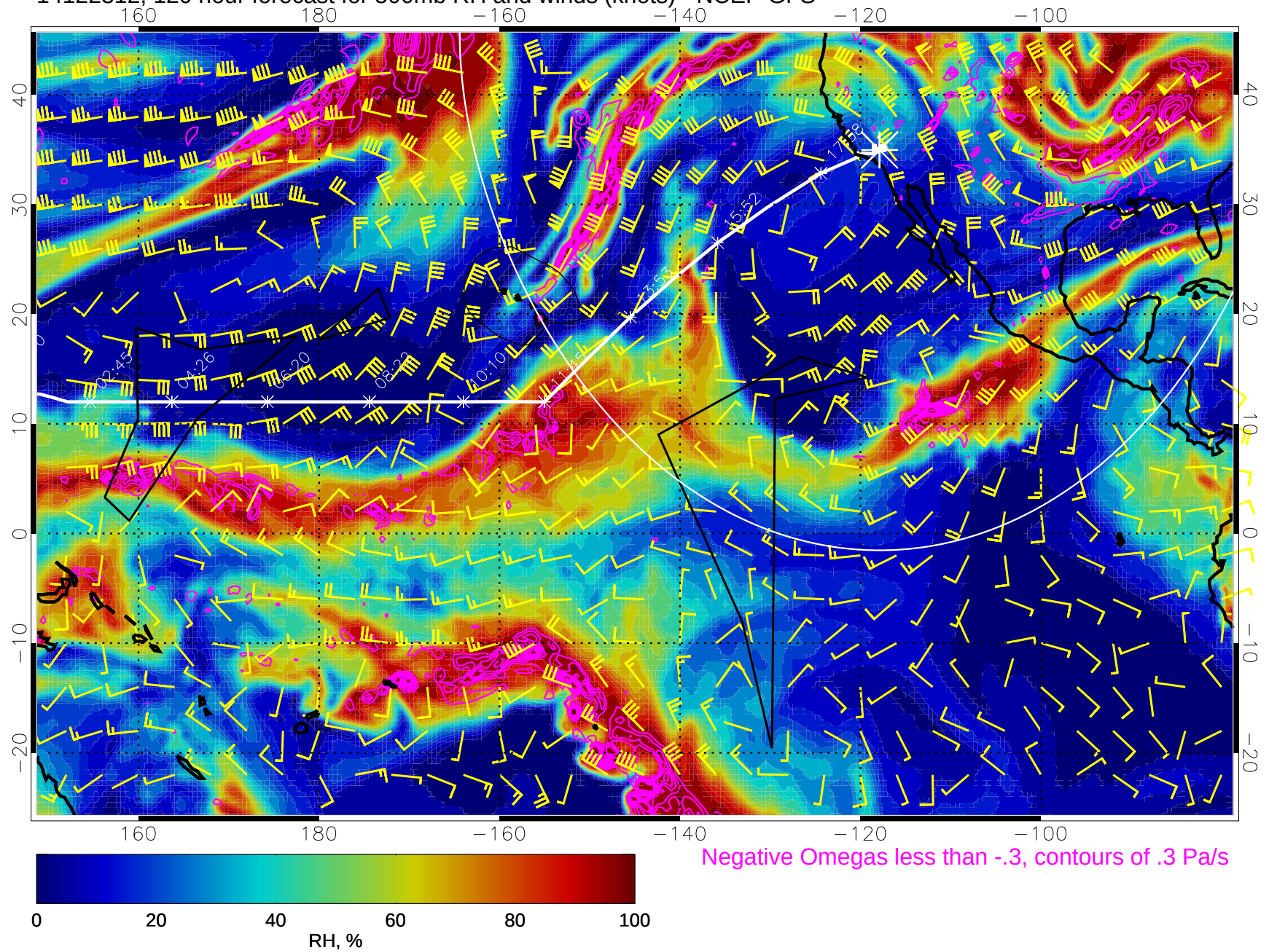
14122312, 120 hour forecast for 500mb RH and winds (knots) - NCEP GFS
