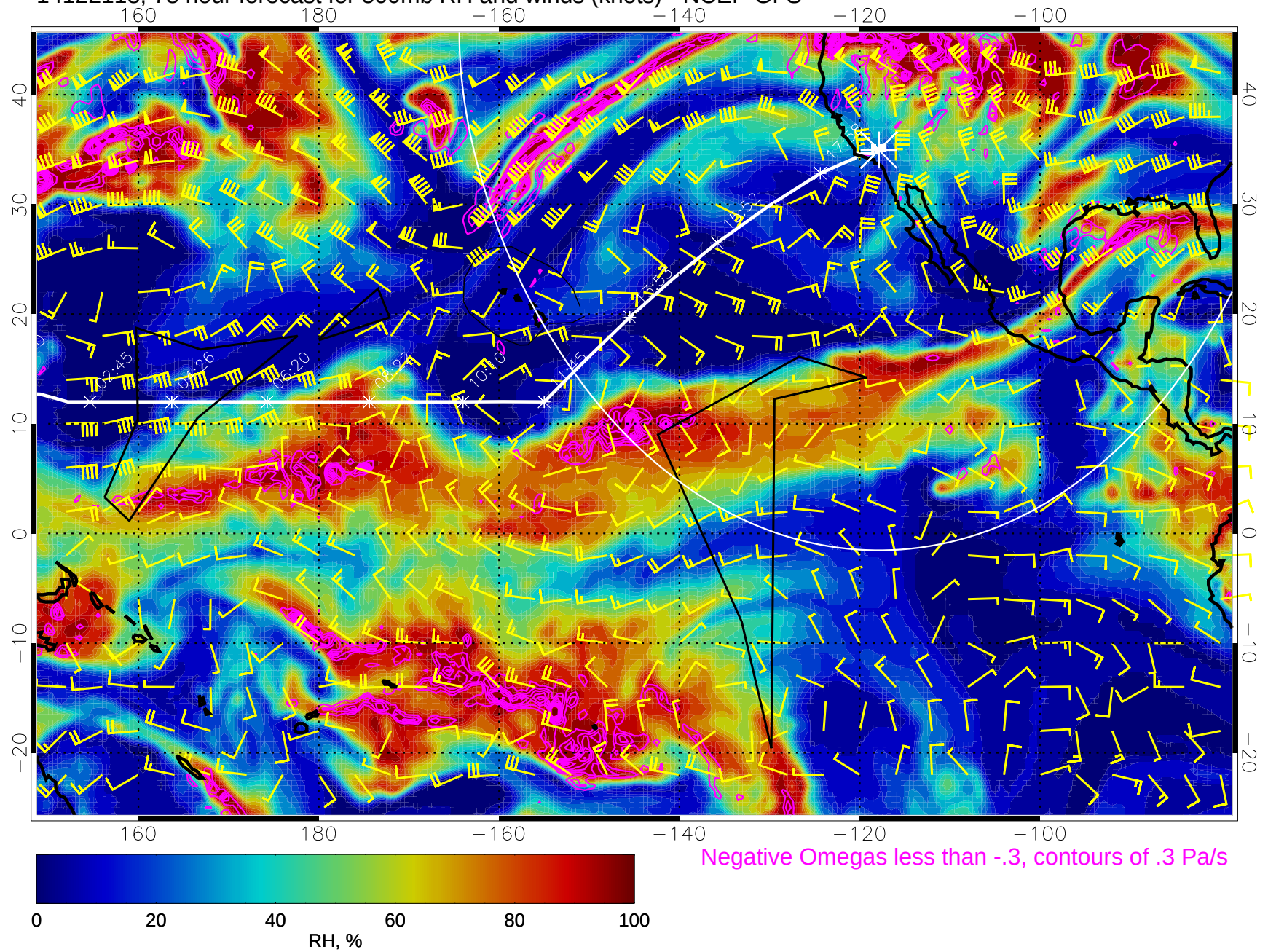
14122118, 78 hour forecast for 500mb RH and winds (knots) - NCEP GFS
