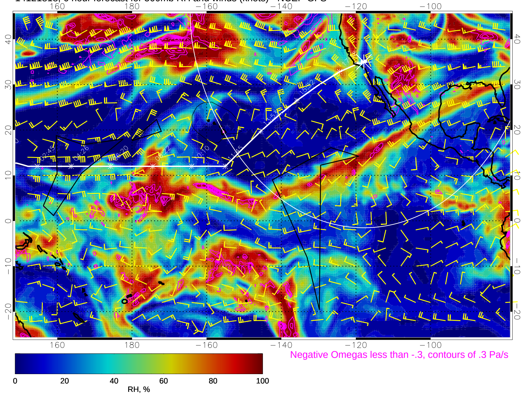
14121818, 6 hour forecast for 500mb RH and winds (knots) - NCEP GFS
