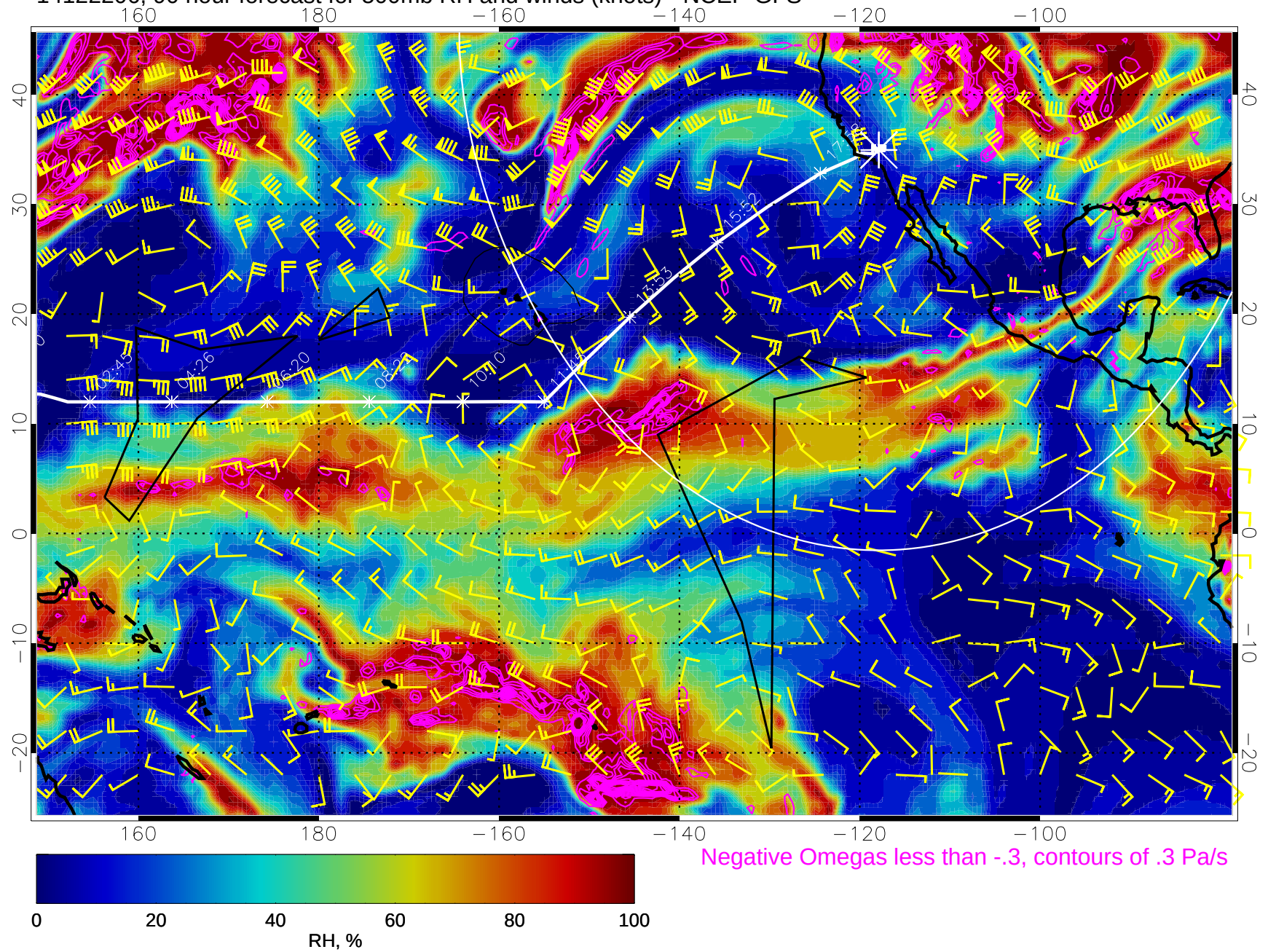
14122206, 90 hour forecast for 500mb RH and winds (knots) - NCEP GFS
