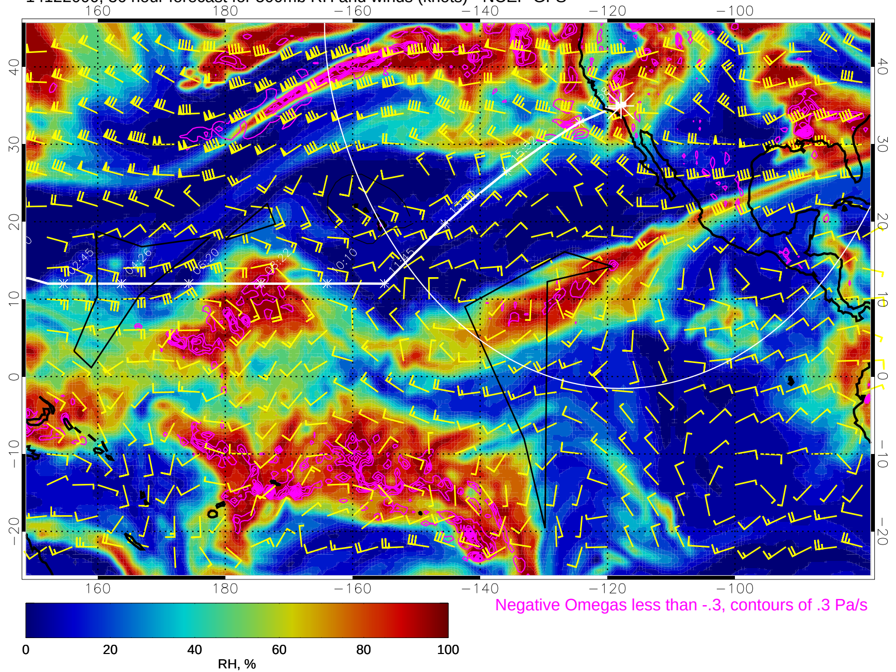
14122000, 36 hour forecast for 500mb RH and winds (knots) - NCEP GFS
