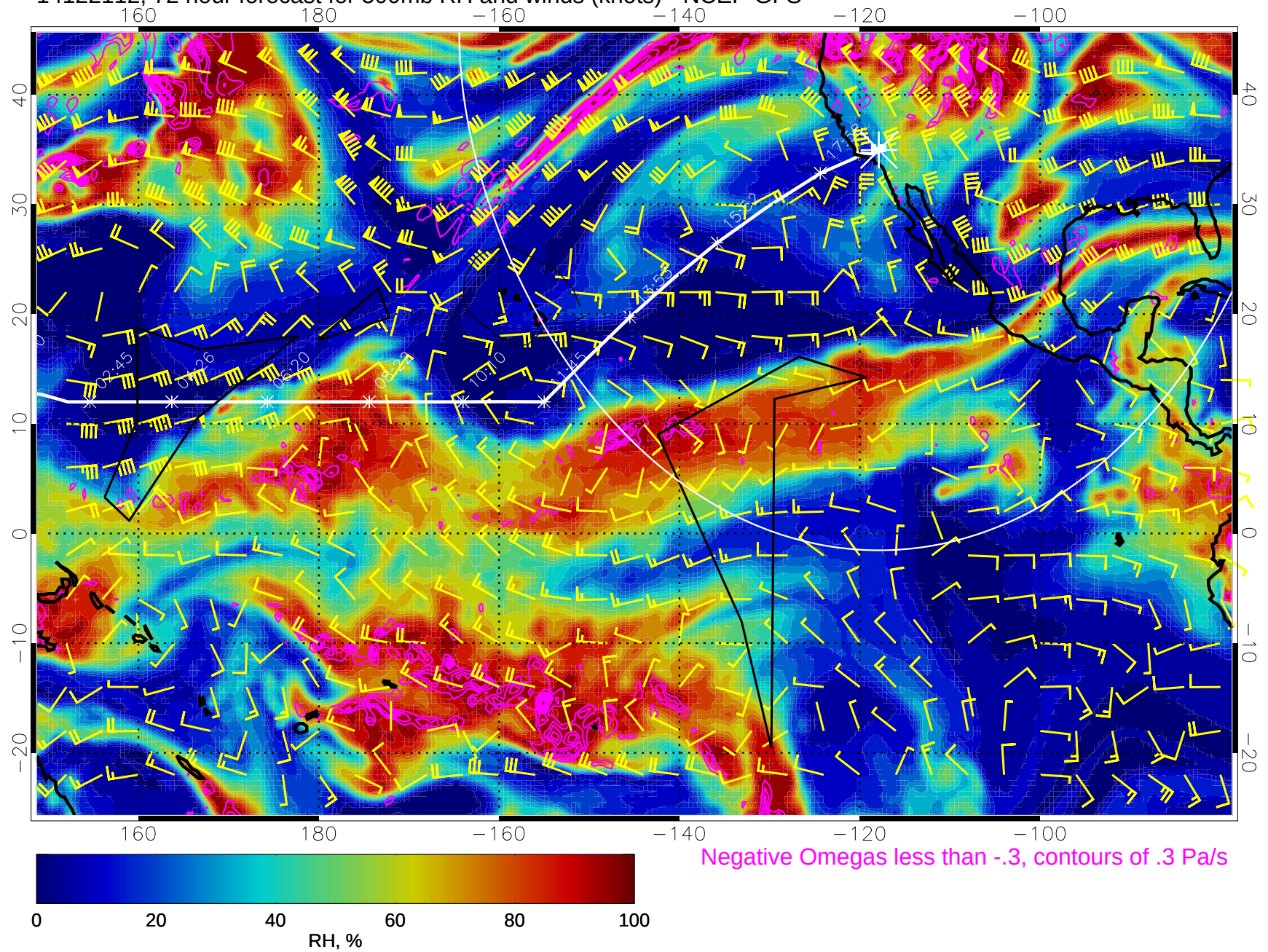
14122112, 72 hour forecast for 500mb RH and winds (knots) - NCEP GFS
