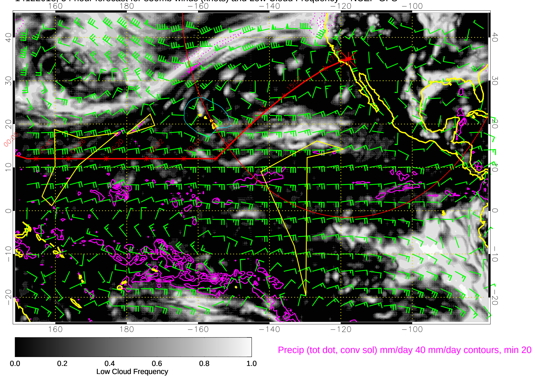
14122018, 54 hour forecast for 850mb winds (knots) and Low Cloud Frequency -- NCEP GFS
