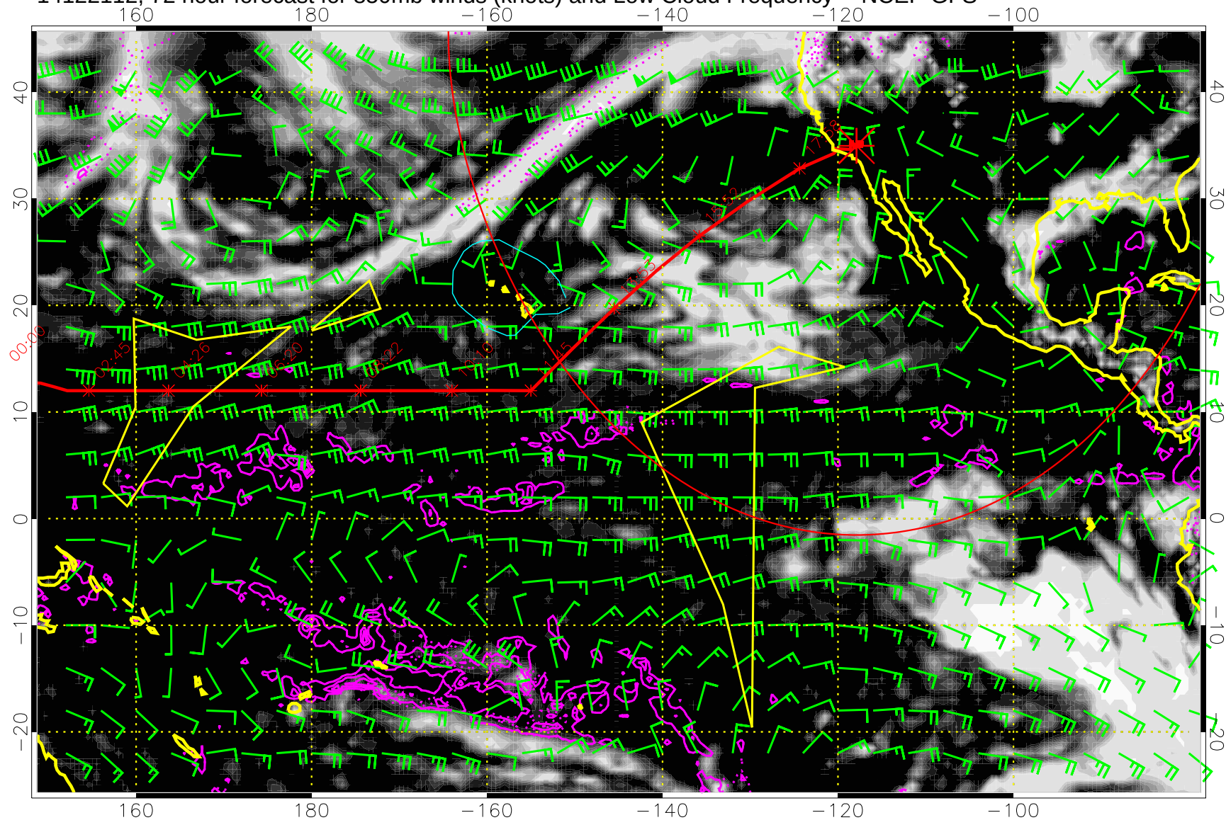
14122112, 72 hour forecast for 850mb winds (knots) and Low Cloud Frequency -- NCEP GFS
