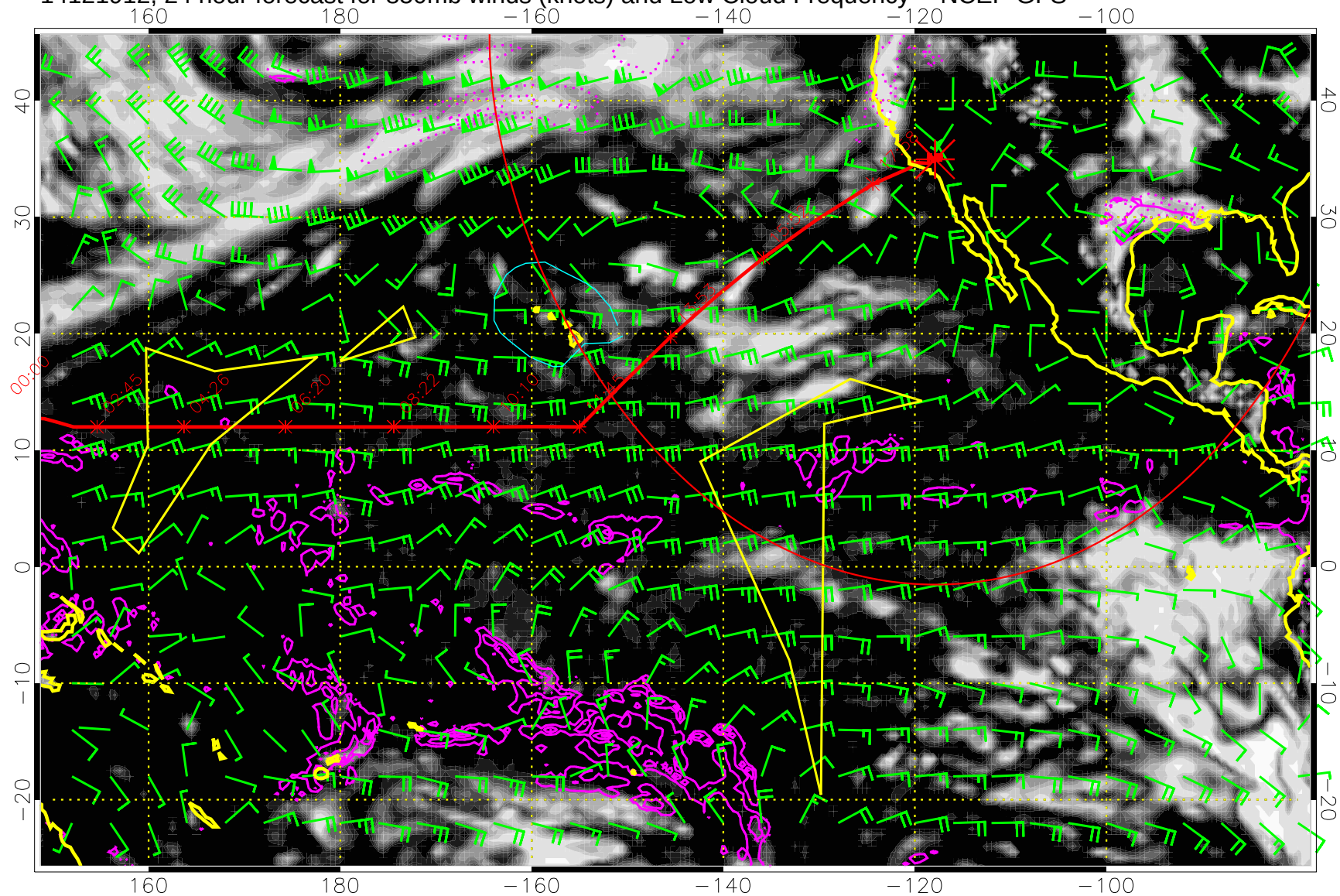
14121912, 24 hour forecast for 850mb winds (knots) and Low Cloud Frequency -- NCEP GFS
