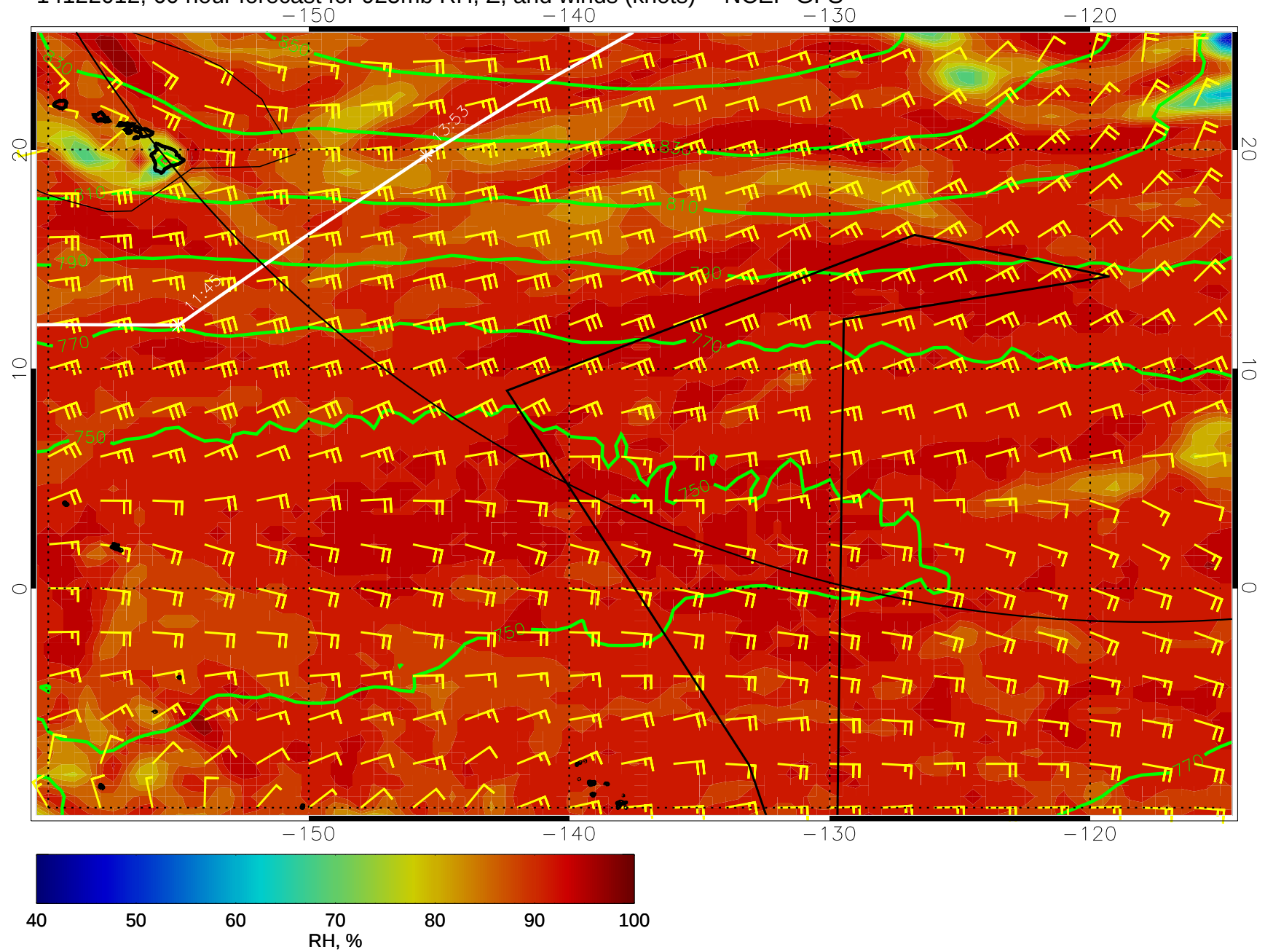
14122012, 60 hour forecast for 925mb RH, Z, and winds (knots) -- NCEP GFS
