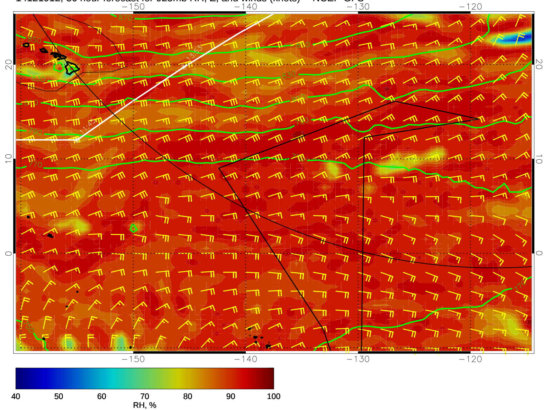
14121912, 36 hour forecast for 925mb RH, Z, and winds (knots) -- NCEP GFS
