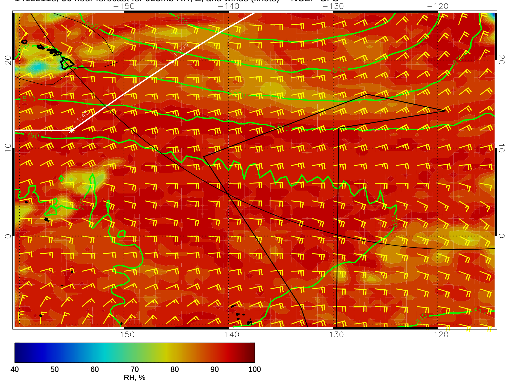
14122118, 90 hour forecast for 925mb RH, Z, and winds (knots) -- NCEP GFS
