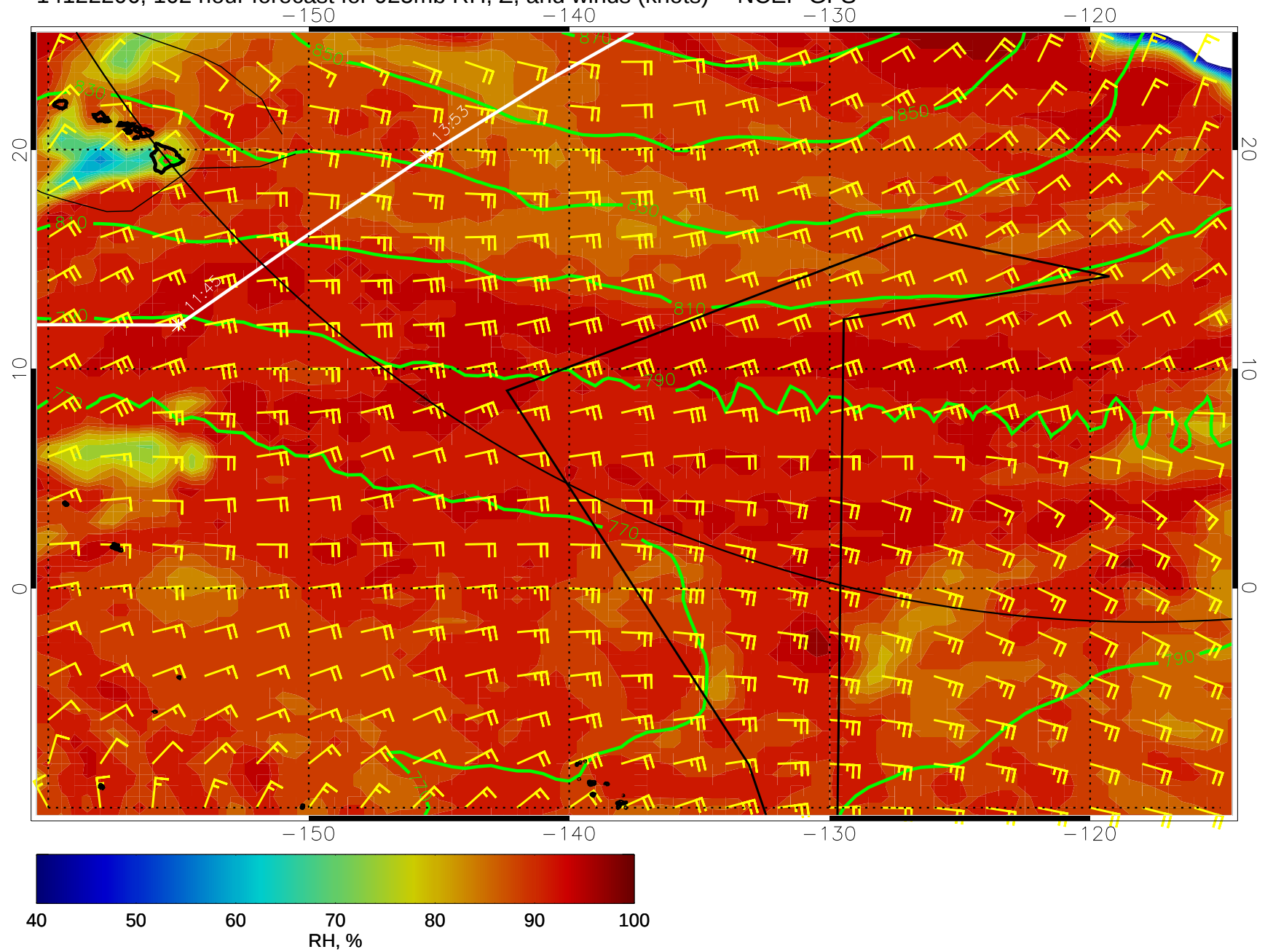
14122206, 102 hour forecast for 925mb RH, Z, and winds (knots) -- NCEP GFS
