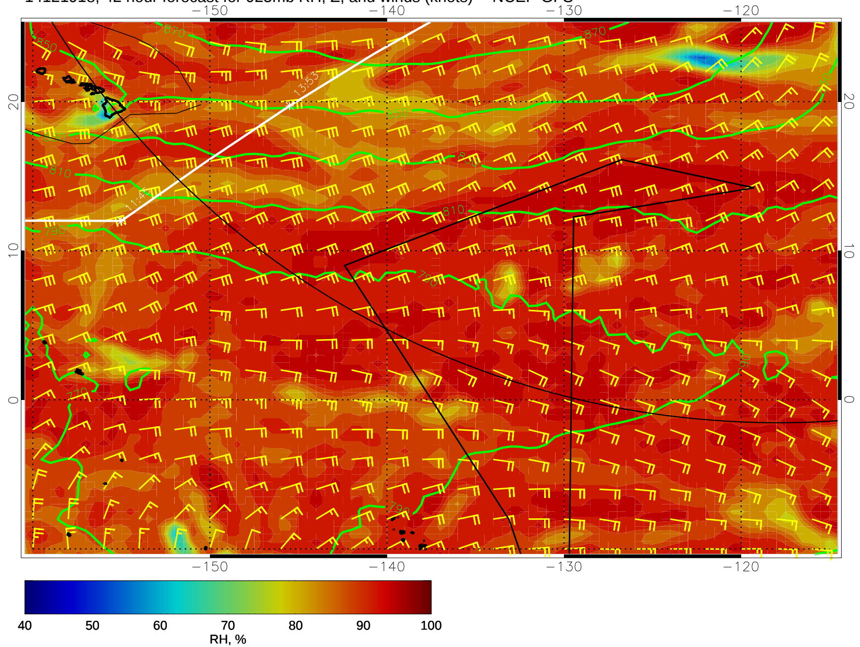
14121918, 42 hour forecast for 925mb RH, Z, and winds (knots) -- NCEP GFS
