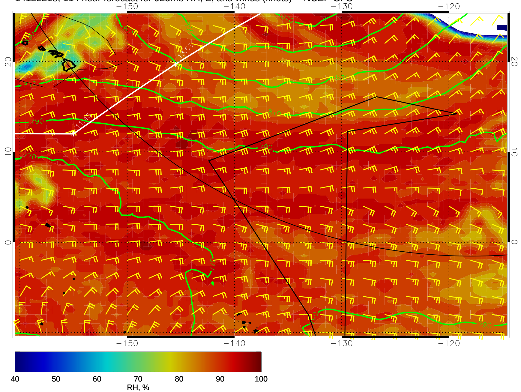
14122218, 114 hour forecast for 925mb RH, Z, and winds (knots) -- NCEP GFS
