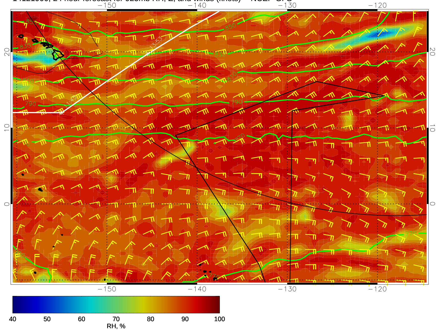
14121900, 24 hour forecast for 925mb RH, Z, and winds (knots) -- NCEP GFS
