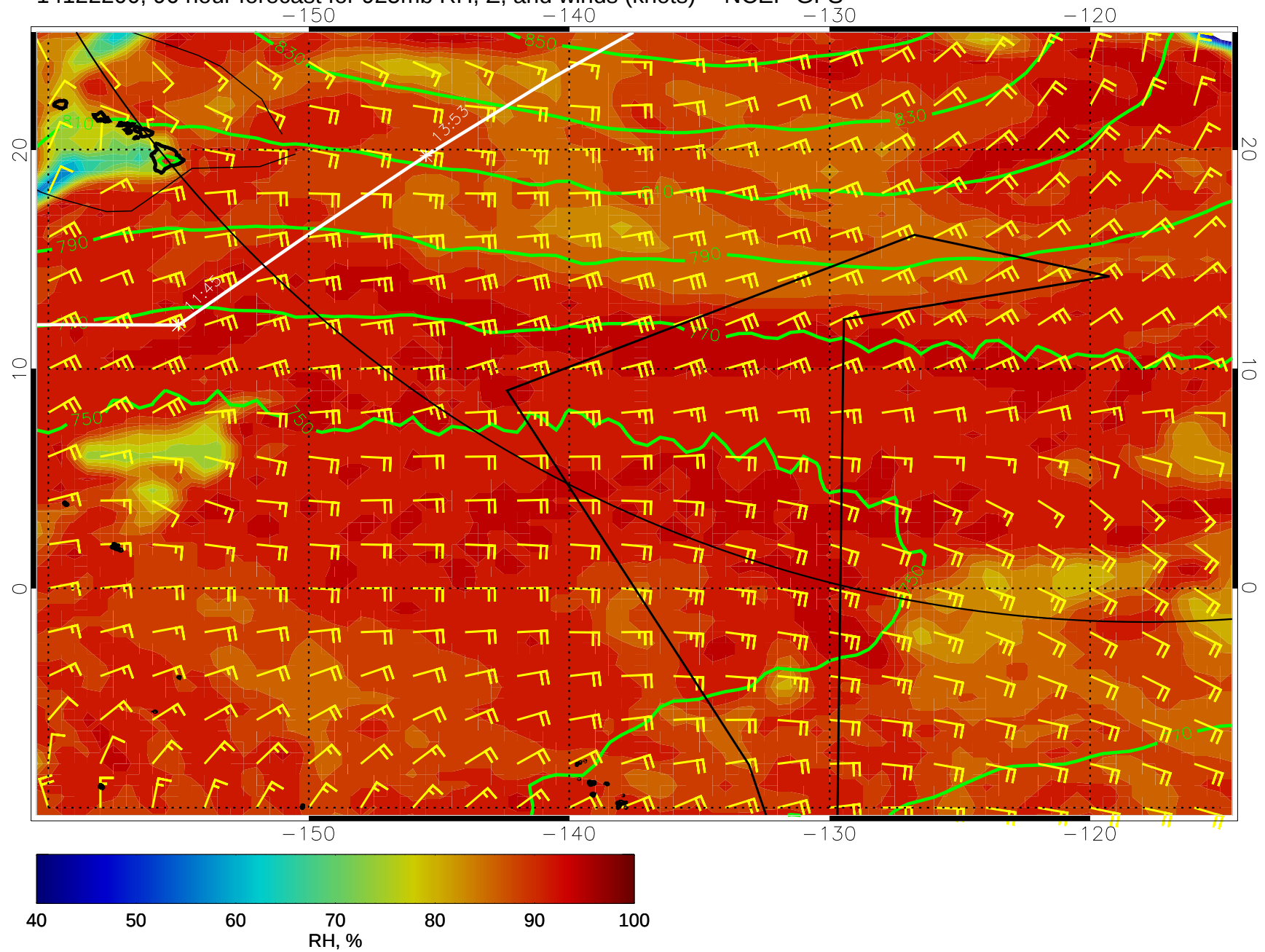
14122200, 96 hour forecast for 925mb RH, Z, and winds (knots) -- NCEP GFS
