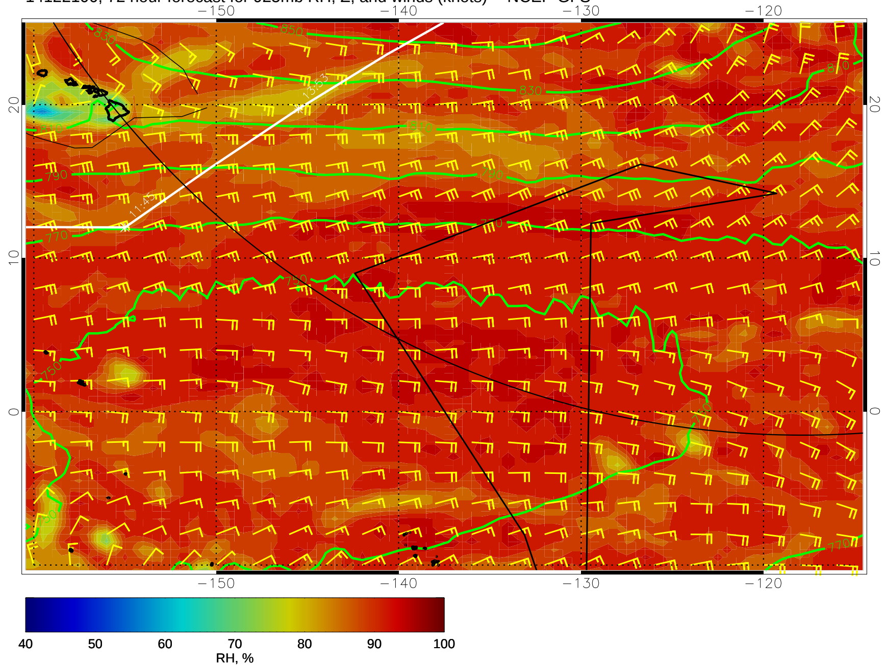
14122100, 72 hour forecast for 925mb RH, Z, and winds (knots) -- NCEP GFS
