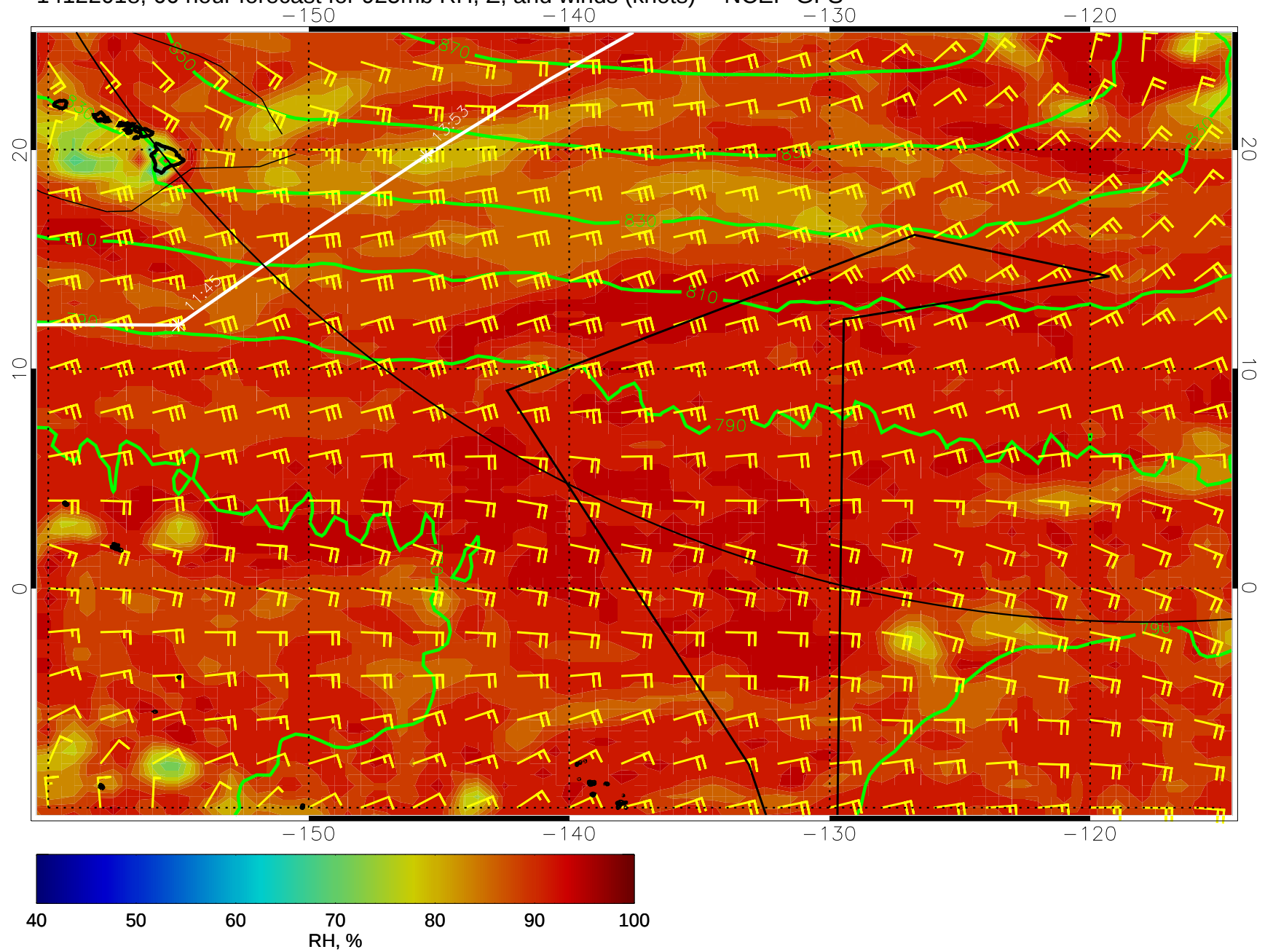
14122018, 66 hour forecast for 925mb RH, Z, and winds (knots) -- NCEP GFS
