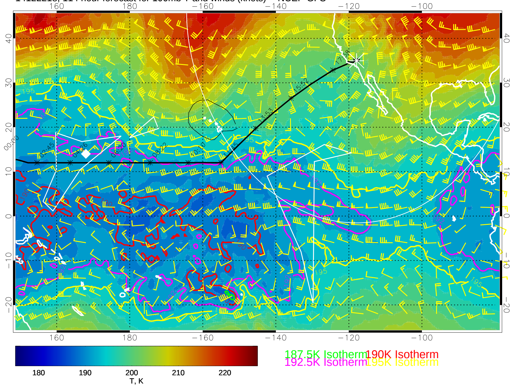
14122218, 114 hour forecast for 100mb T and winds (knots) -- NCEP GFS
