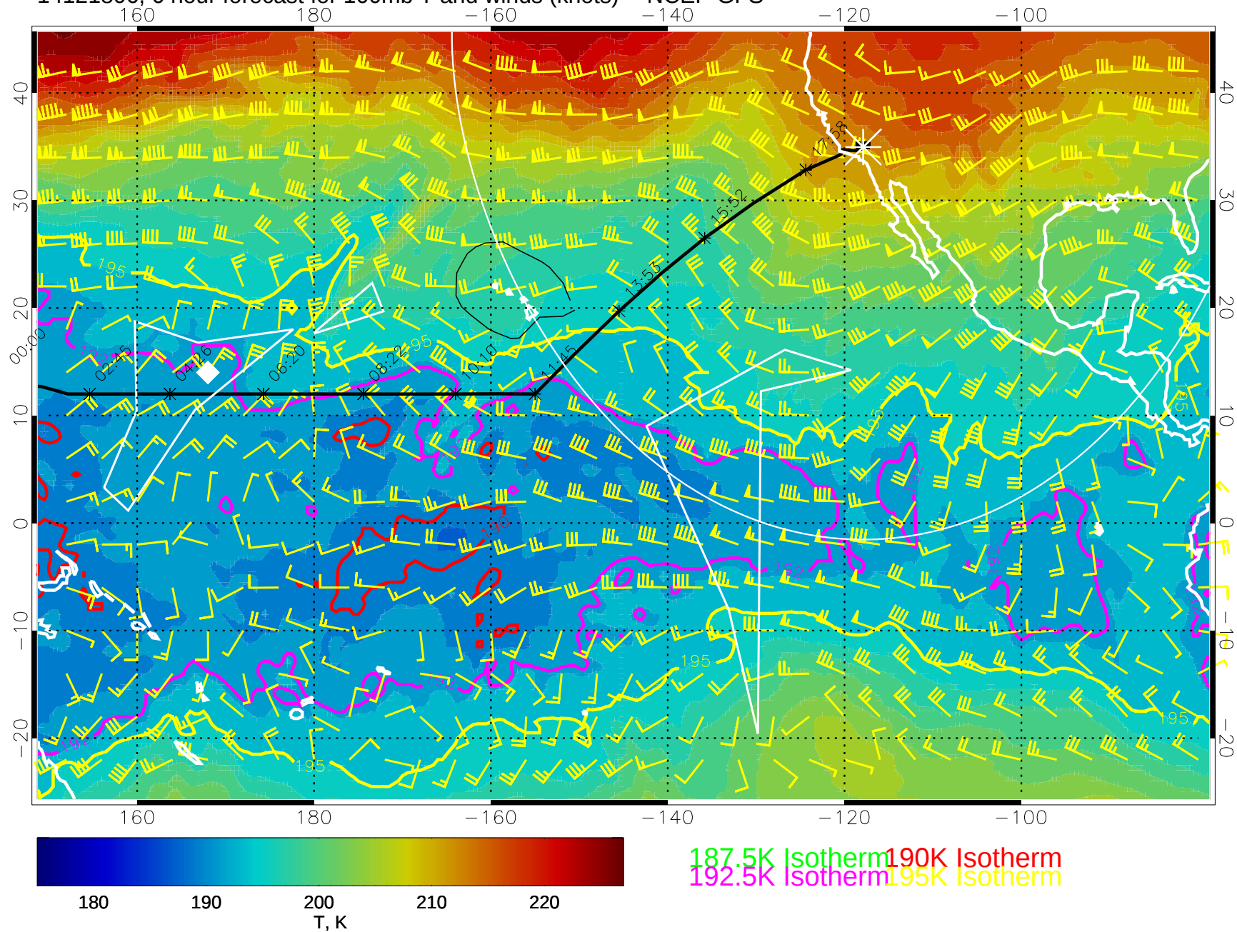
14121806, 6 hour forecast for 100mb T and winds (knots) -- NCEP GFS
