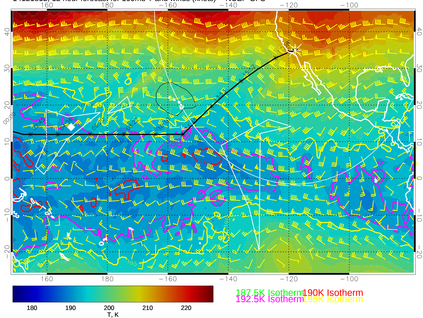
14121812, 12 hour forecast for 100mb T and winds (knots) -- NCEP GFS
