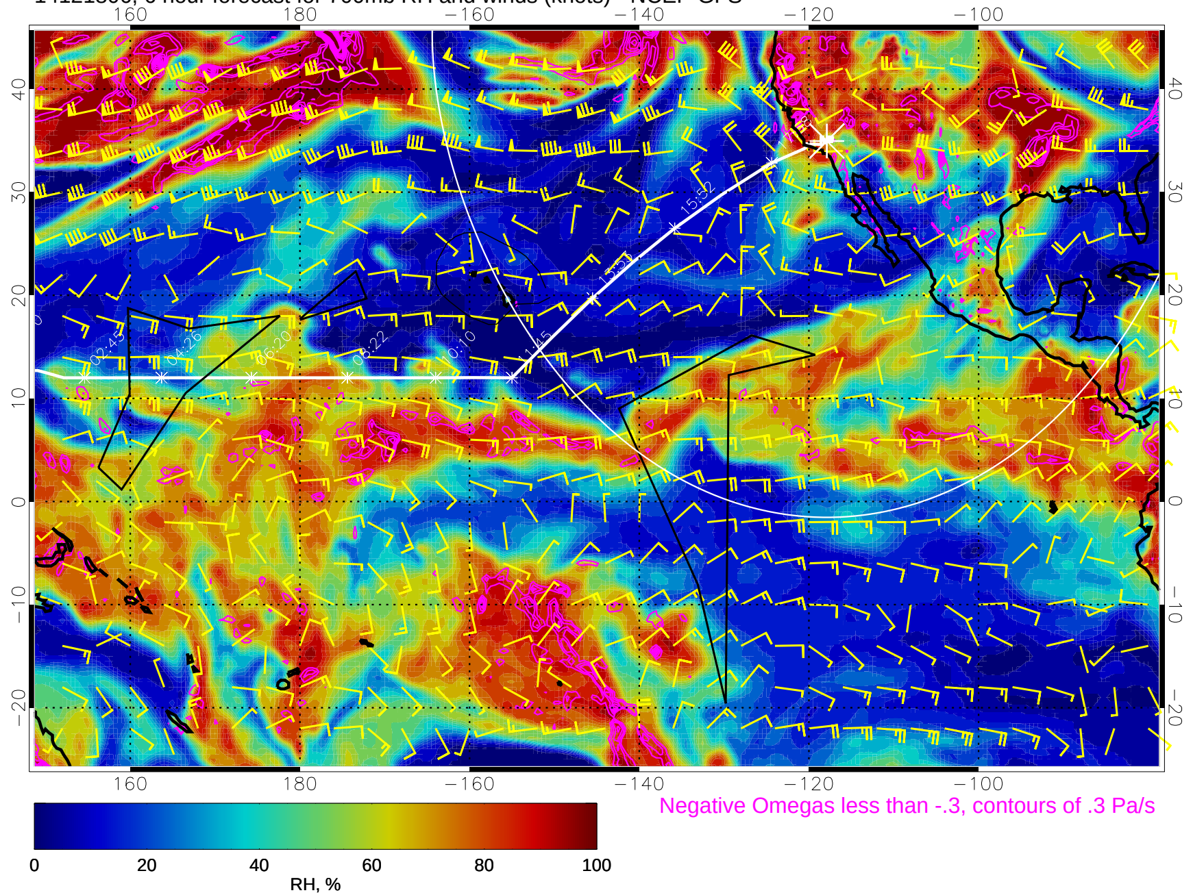
14121806, 6 hour forecast for 700mb RH and winds (knots) - NCEP GFS
