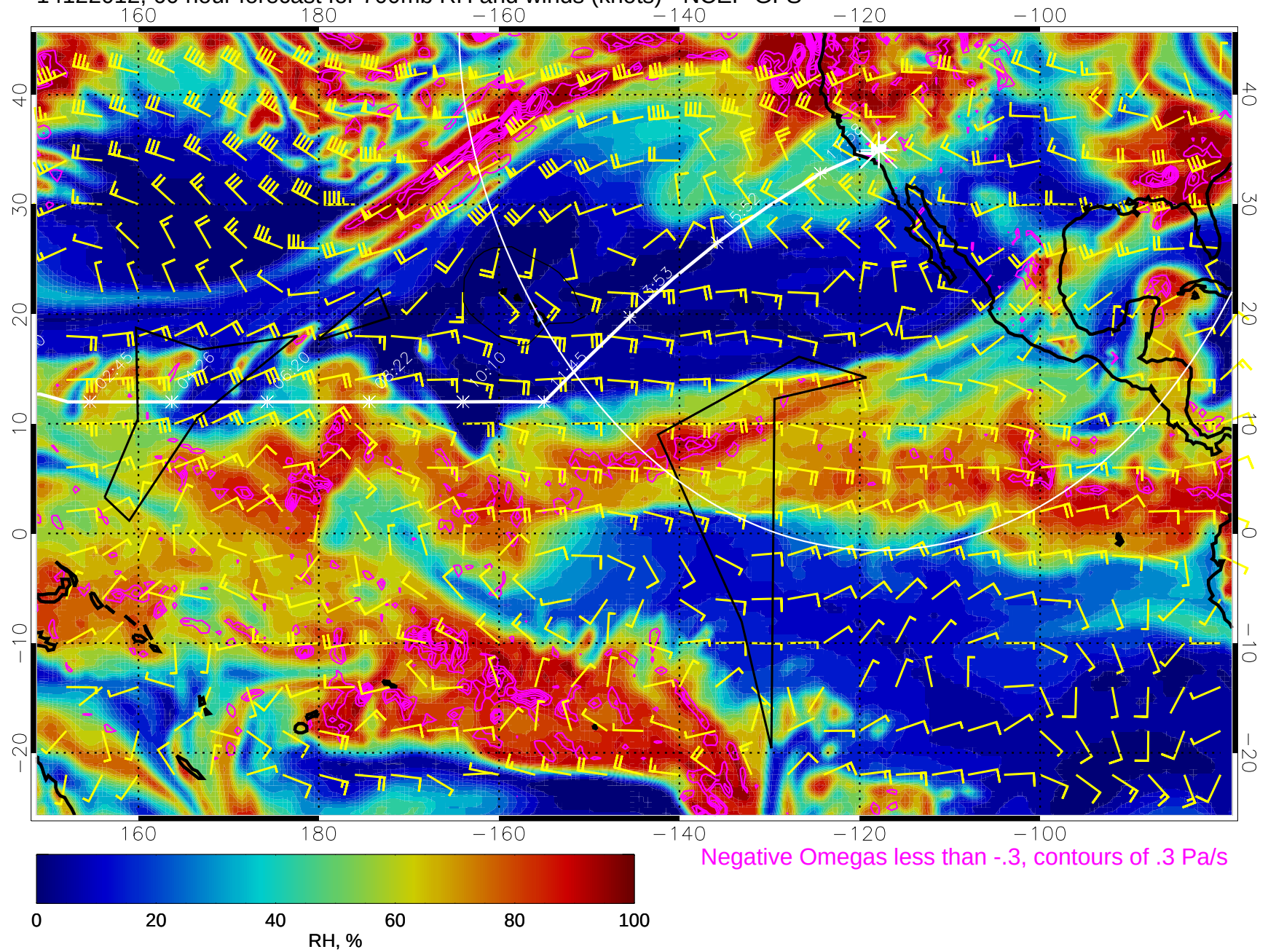
14122012, 60 hour forecast for 700mb RH and winds (knots) - NCEP GFS
