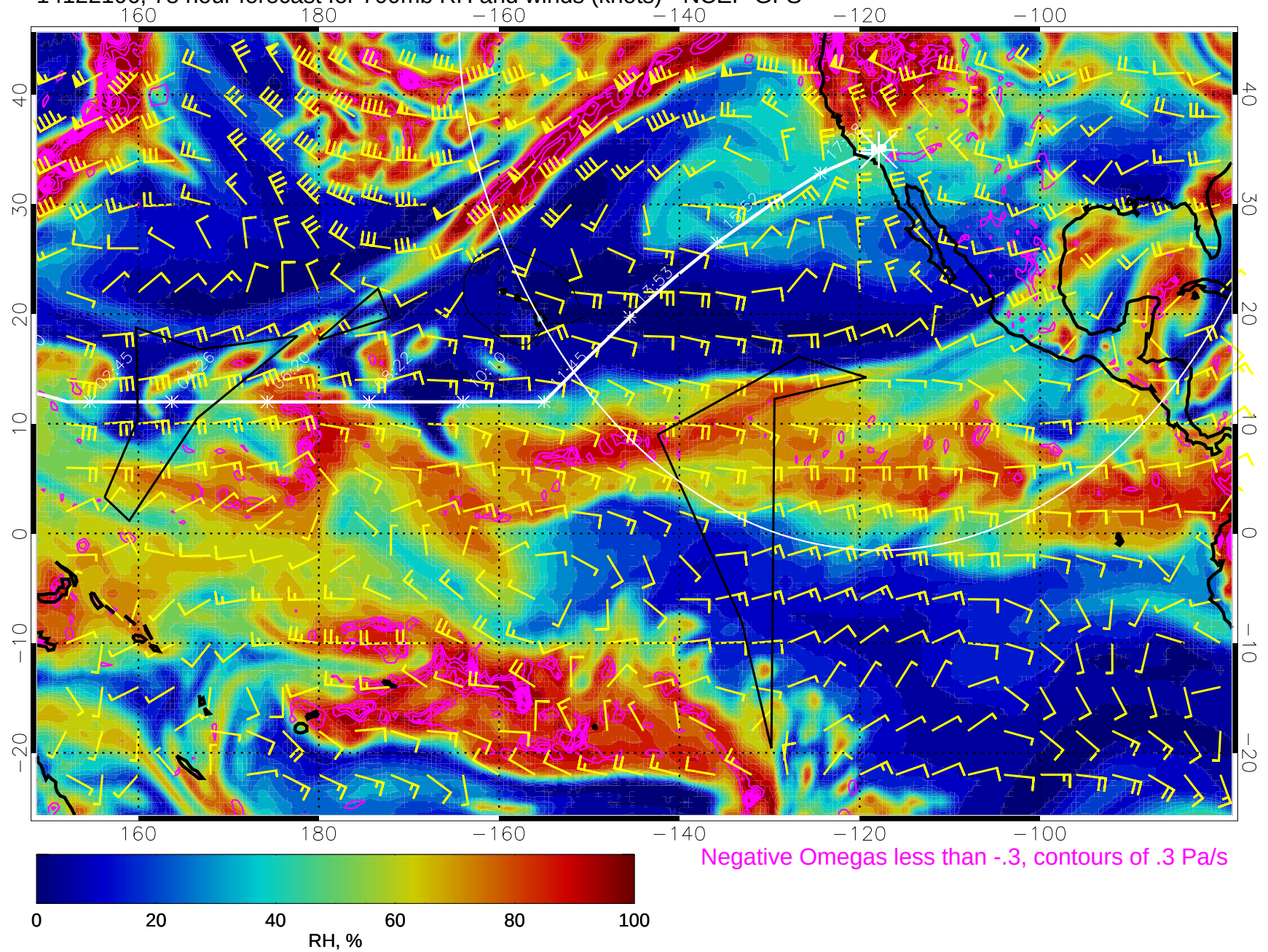
14122106, 78 hour forecast for 700mb RH and winds (knots) - NCEP GFS
