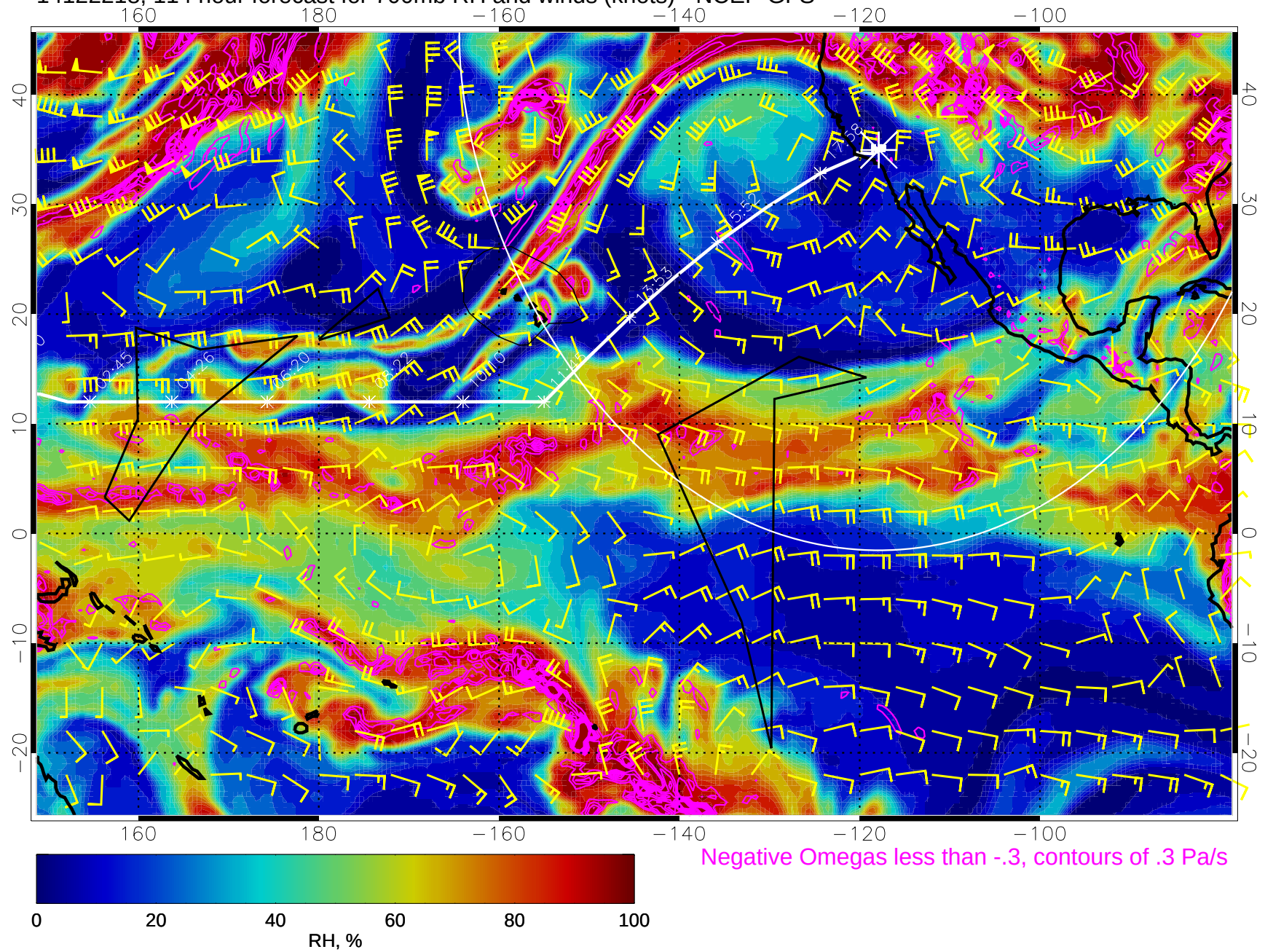
14122218, 114 hour forecast for 700mb RH and winds (knots) - NCEP GFS
