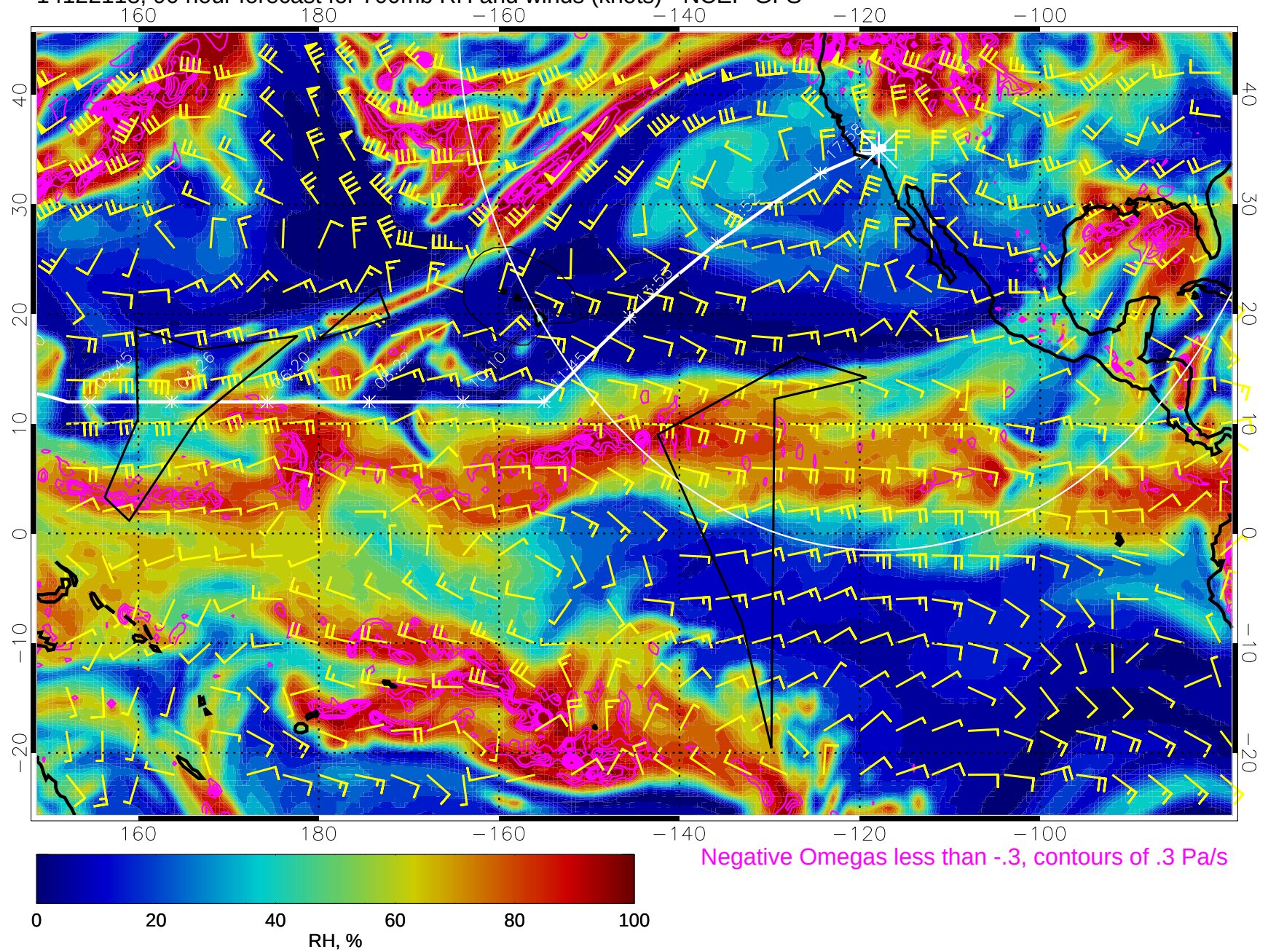
14122118, 90 hour forecast for 700mb RH and winds (knots) - NCEP GFS
