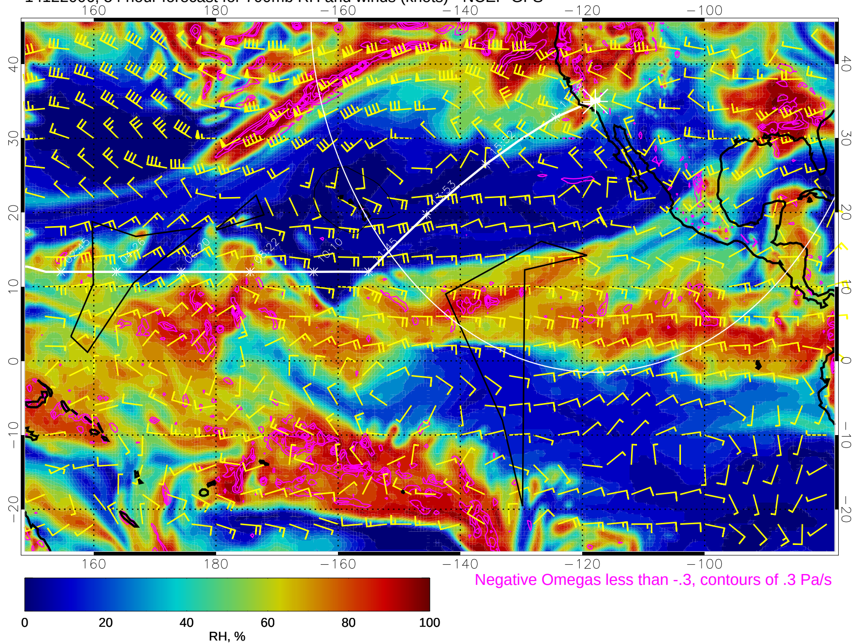
14122006, 54 hour forecast for 700mb RH and winds (knots) - NCEP GFS
