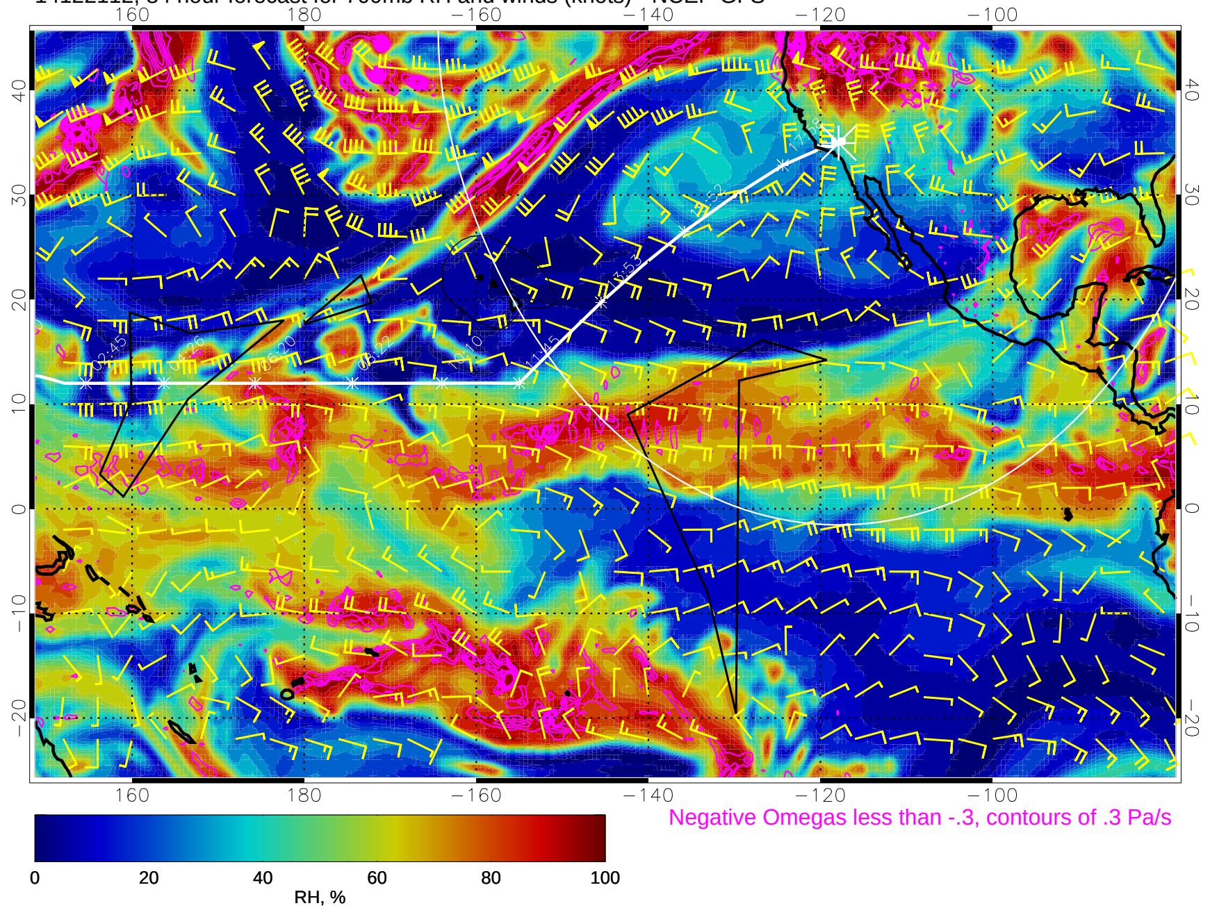
14122112, 84 hour forecast for 700mb RH and winds (knots) - NCEP GFS
