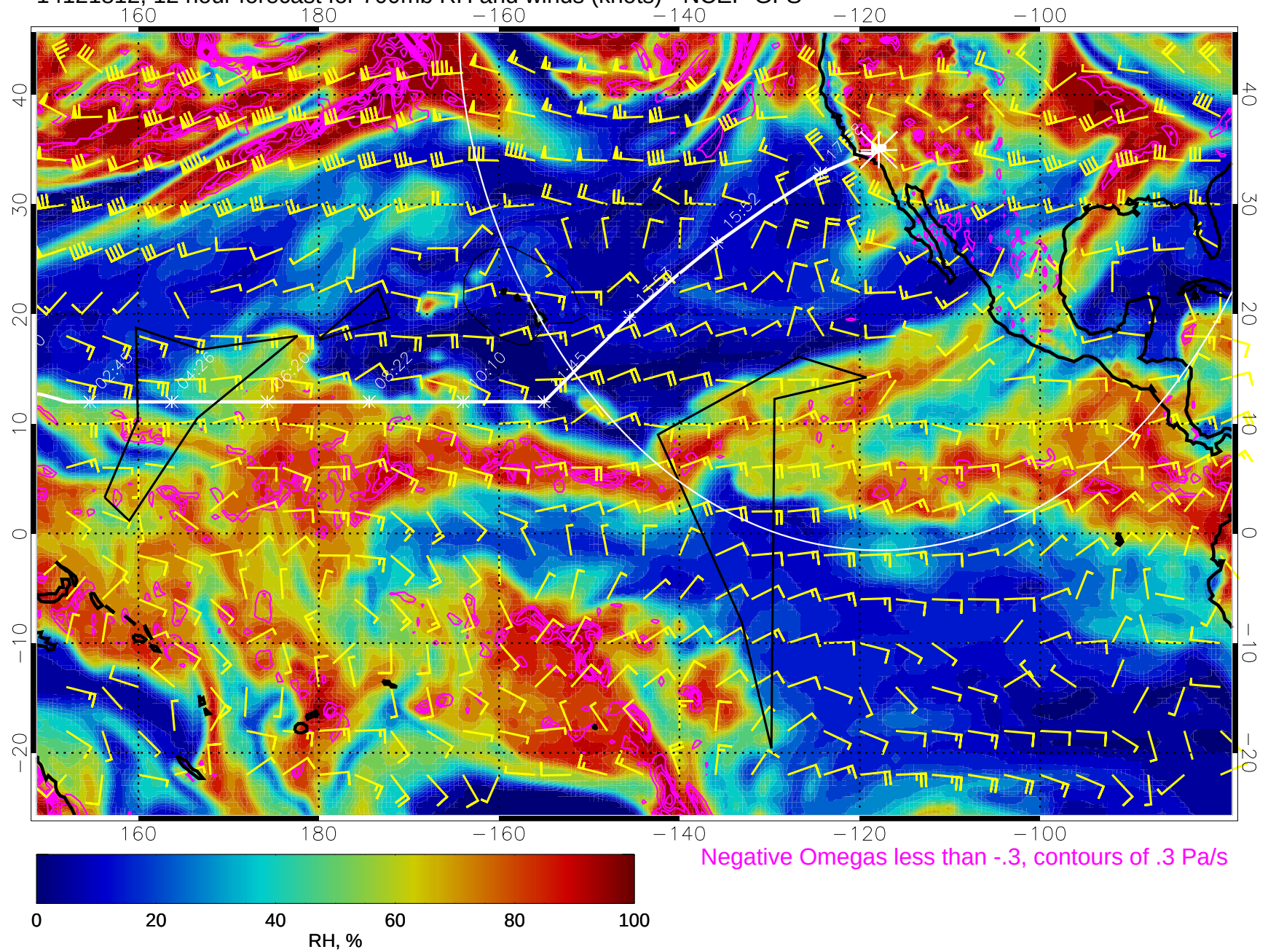
14121812, 12 hour forecast for 700mb RH and winds (knots) - NCEP GFS
