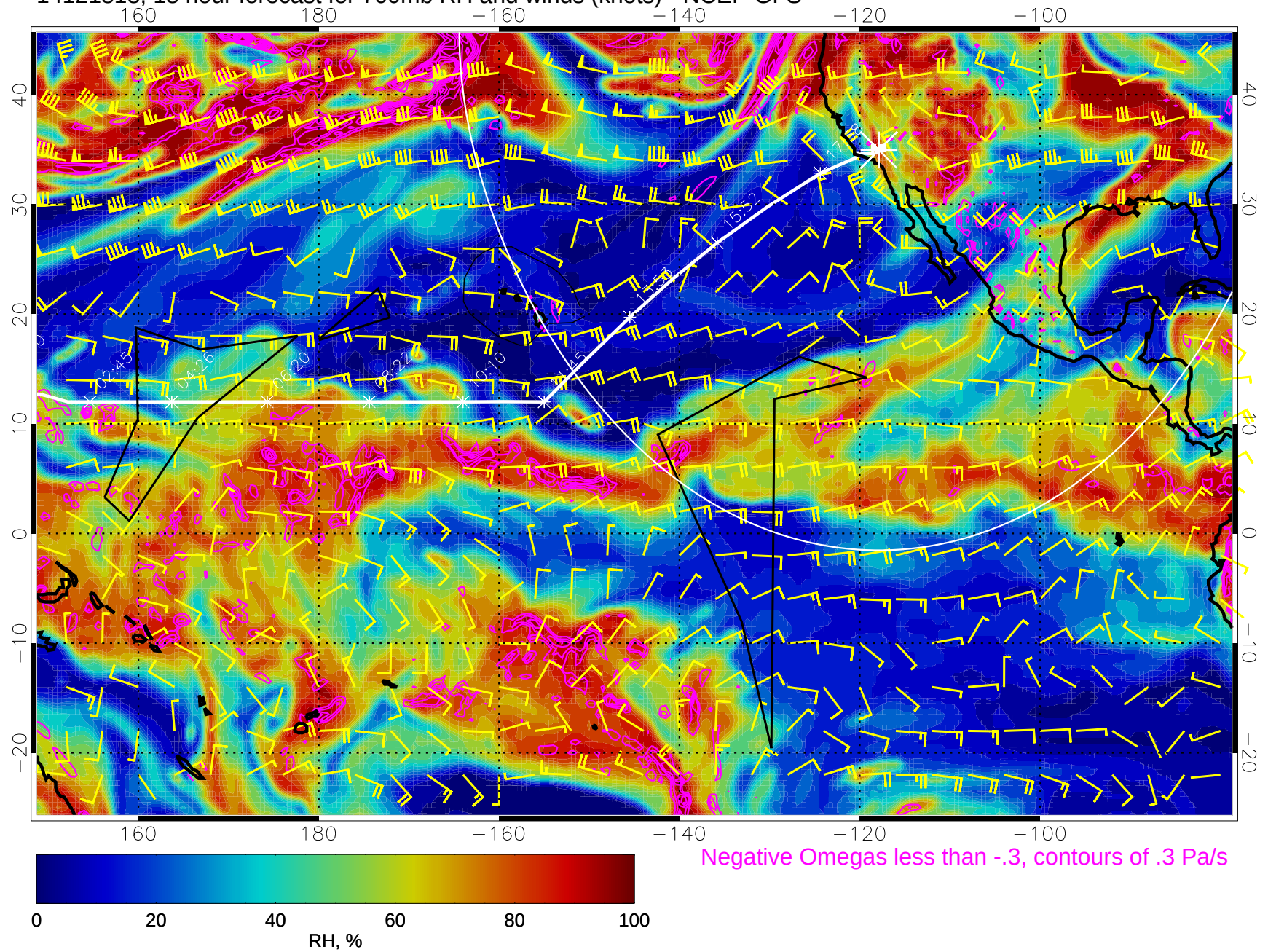
14121818, 18 hour forecast for 700mb RH and winds (knots) - NCEP GFS
