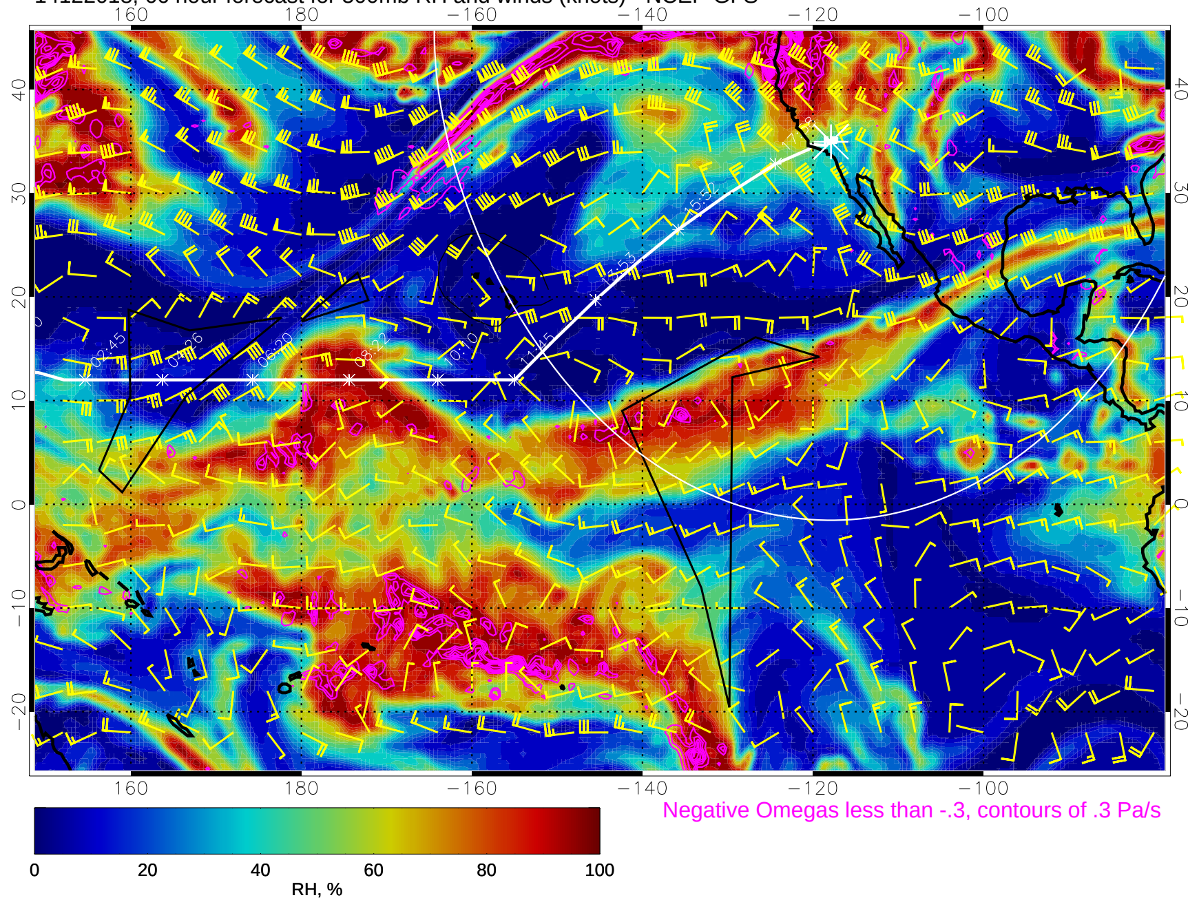
14122018, 66 hour forecast for 500mb RH and winds (knots) - NCEP GFS
