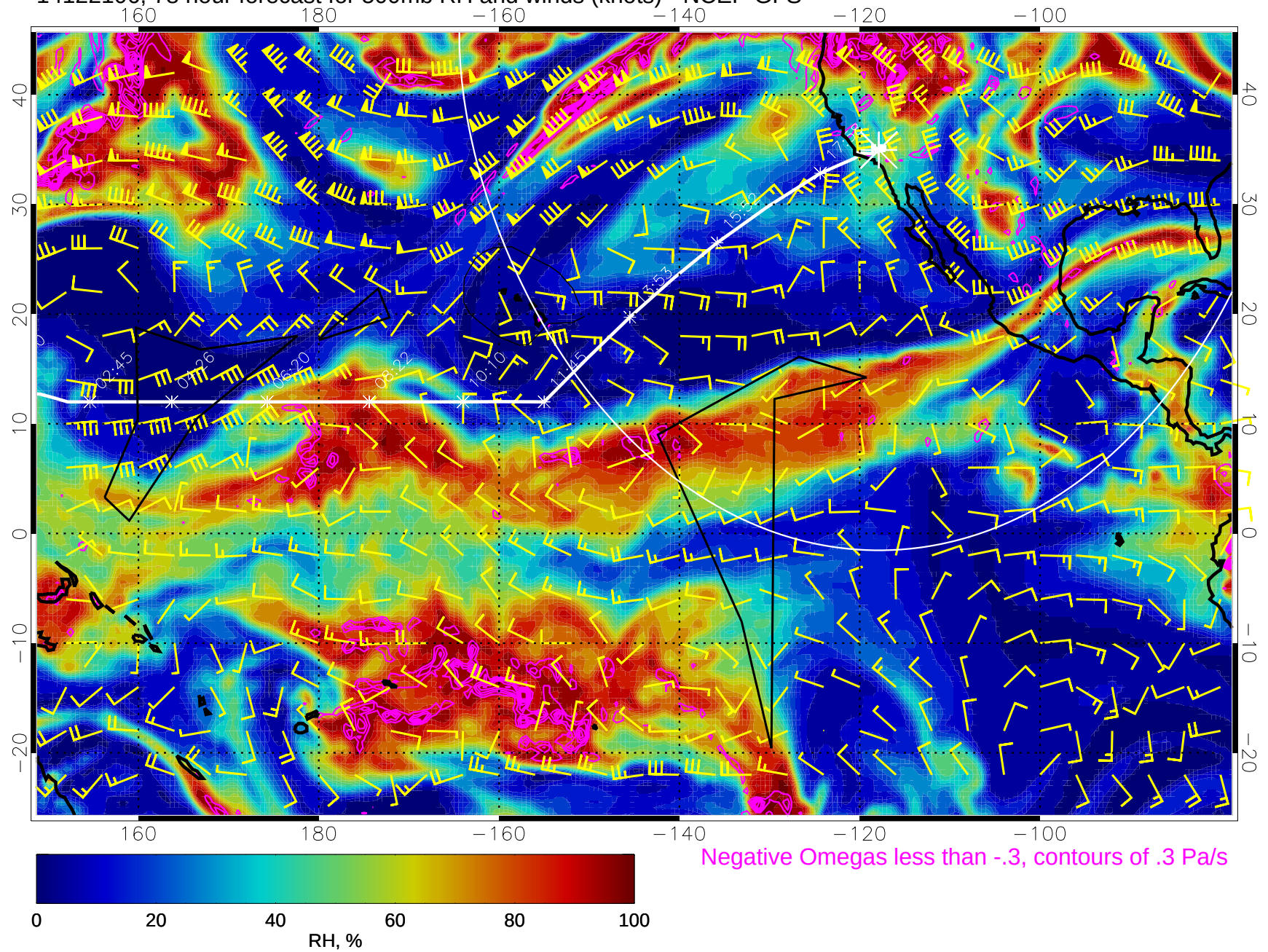
14122106, 78 hour forecast for 500mb RH and winds (knots) - NCEP GFS
