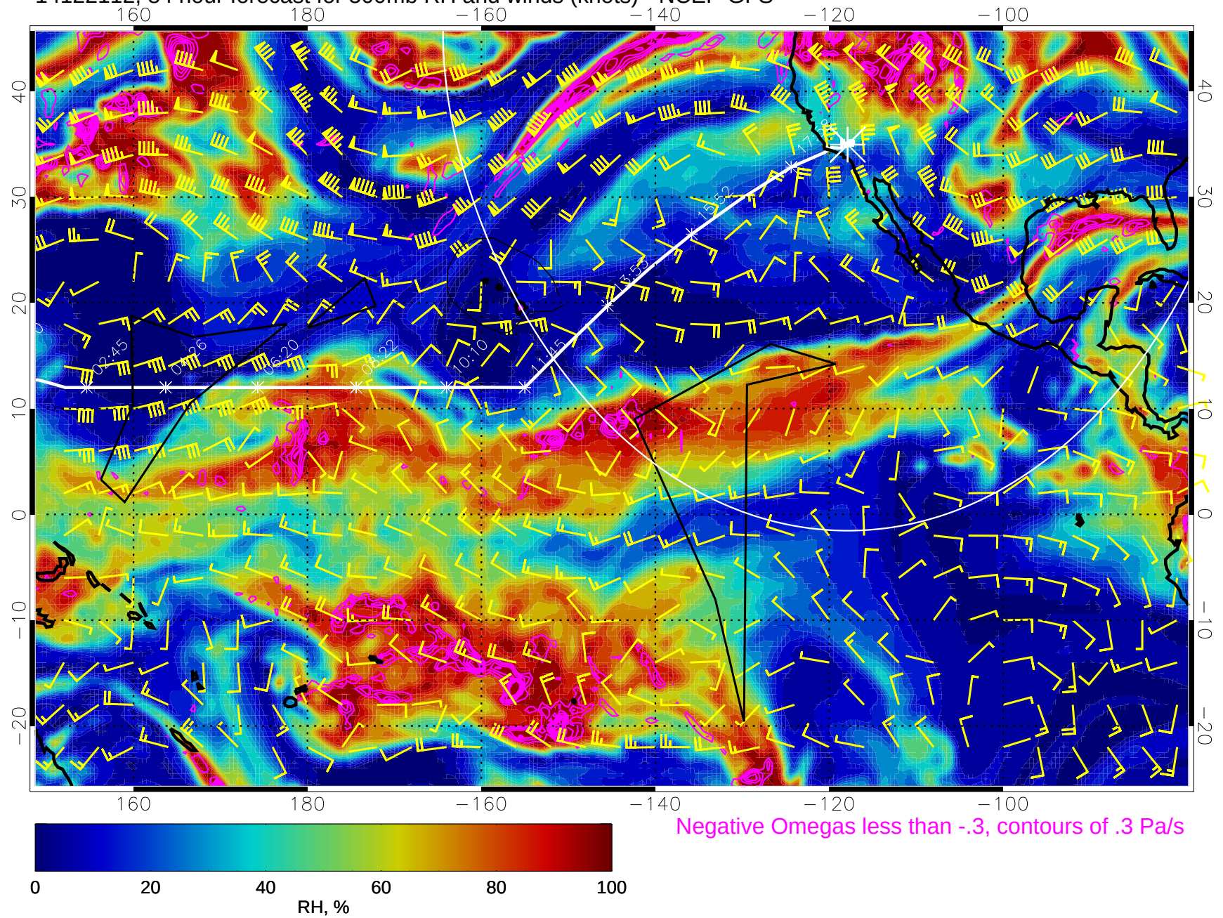
14122112, 84 hour forecast for 500mb RH and winds (knots) - NCEP GFS
