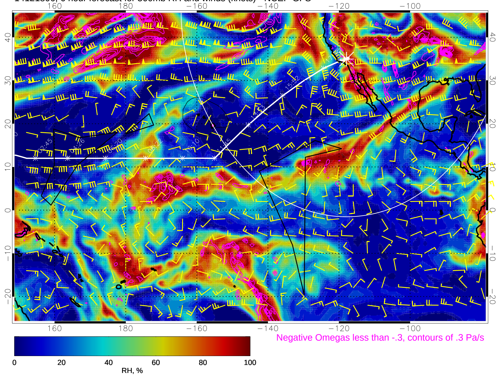
14121806, 6 hour forecast for 500mb RH and winds (knots) - NCEP GFS
