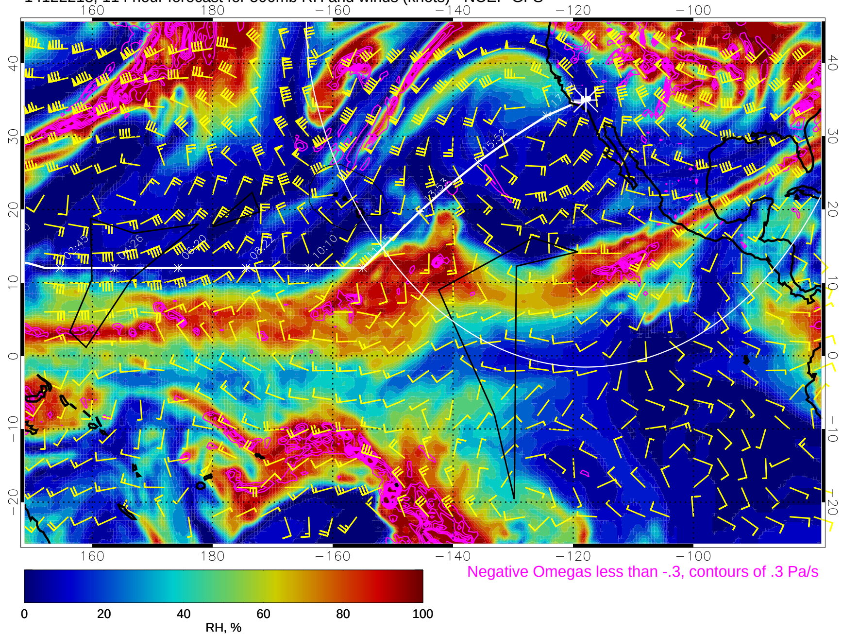
14122218, 114 hour forecast for 500mb RH and winds (knots) - NCEP GFS
