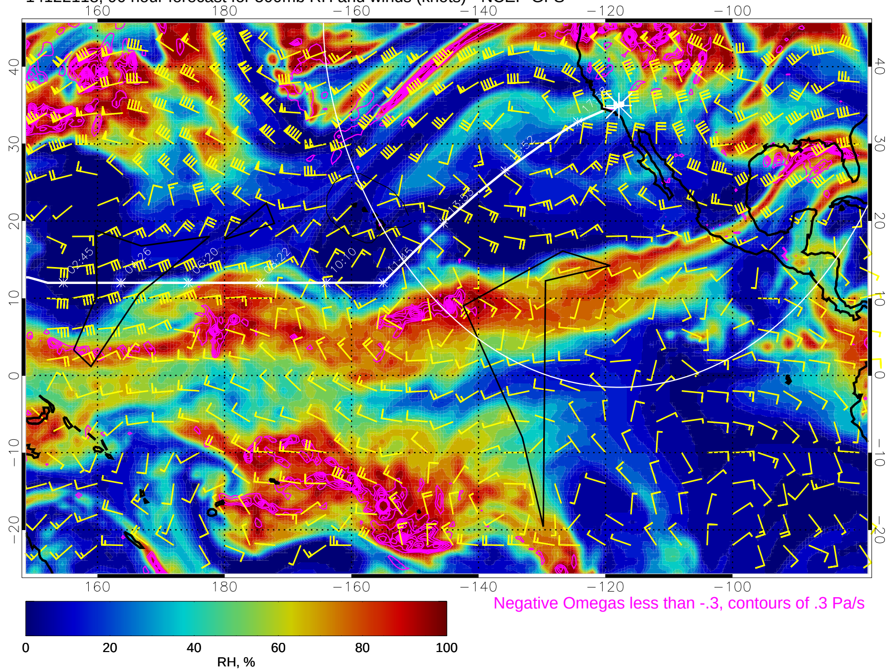
14122118, 90 hour forecast for 500mb RH and winds (knots) - NCEP GFS
