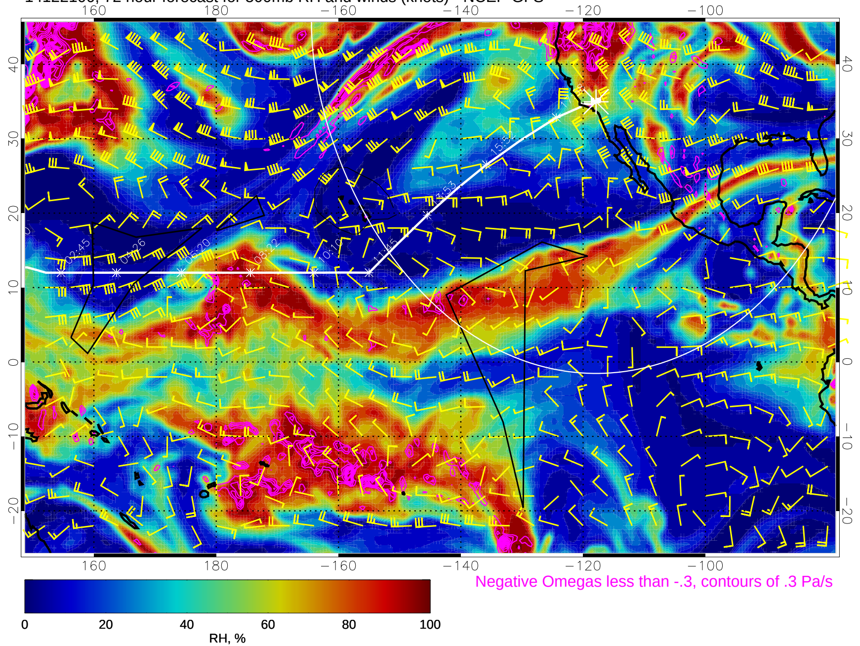
14122100, 72 hour forecast for 500mb RH and winds (knots) - NCEP GFS
