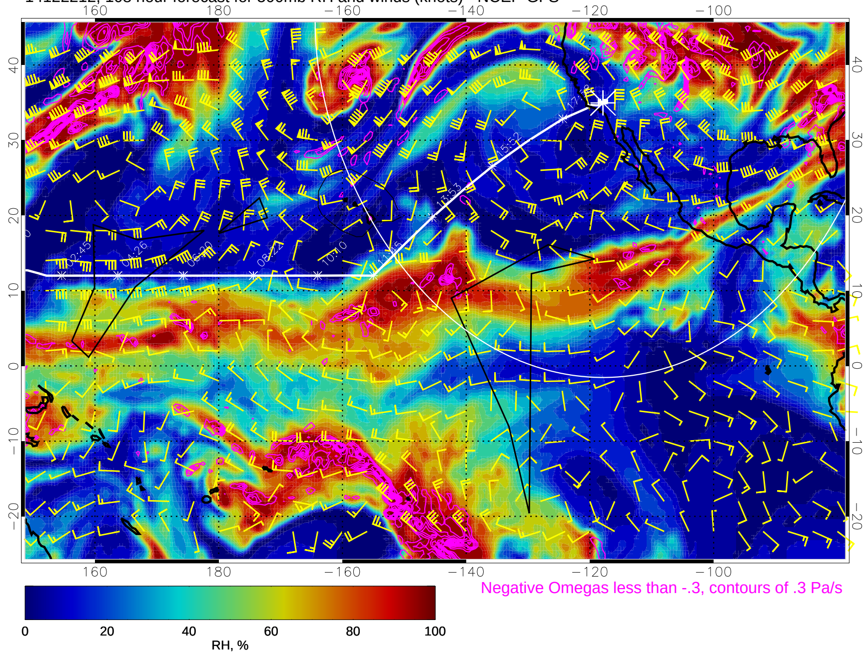
14122212, 108 hour forecast for 500mb RH and winds (knots) - NCEP GFS
