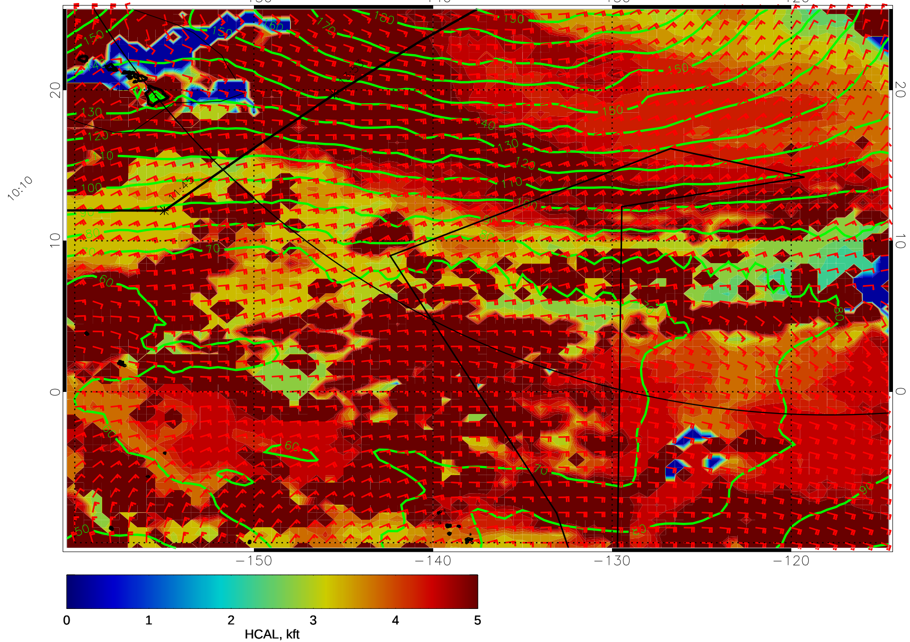
14122212, 108 hour forecast for HCAL, 1000mb Z, and winds (knots) -- NCEP GFS
