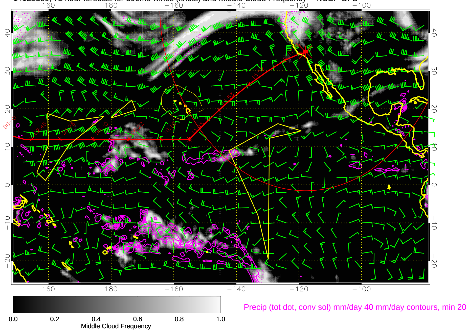
14122100, 72 hour forecast for 500mb winds (knots) and Middle Cloud Frequency -- NCEP GFS
