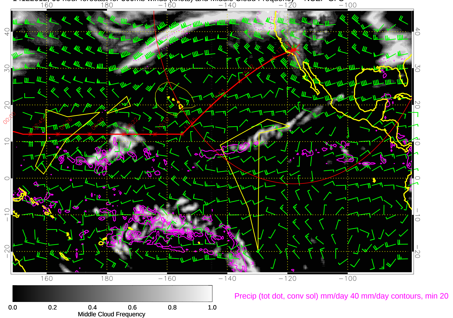
14122012, 60 hour forecast for 500mb winds (knots) and Middle Cloud Frequency -- NCEP GFS
