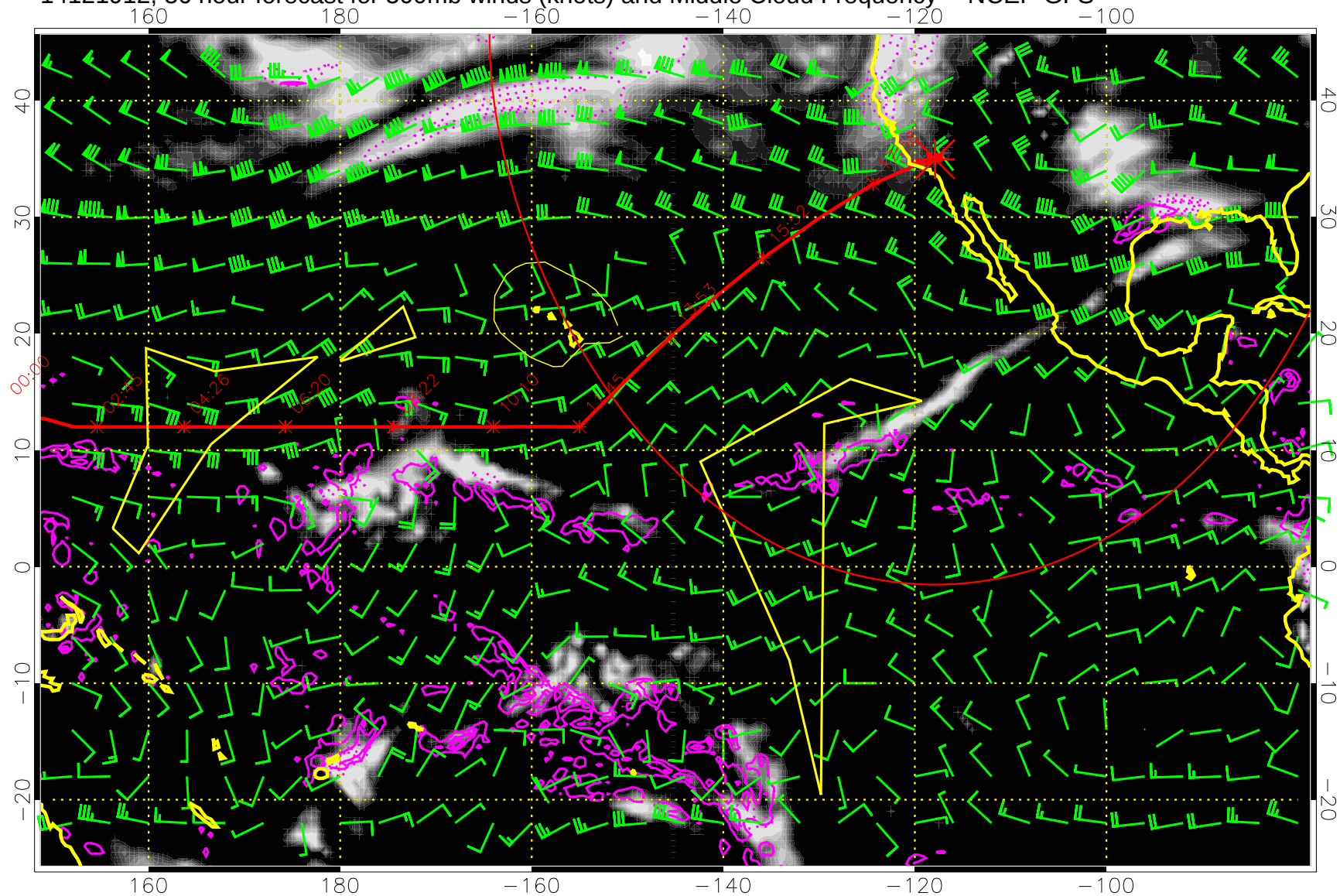
14121912, 36 hour forecast for 500mb winds (knots) and Middle Cloud Frequency -- NCEP GFS
