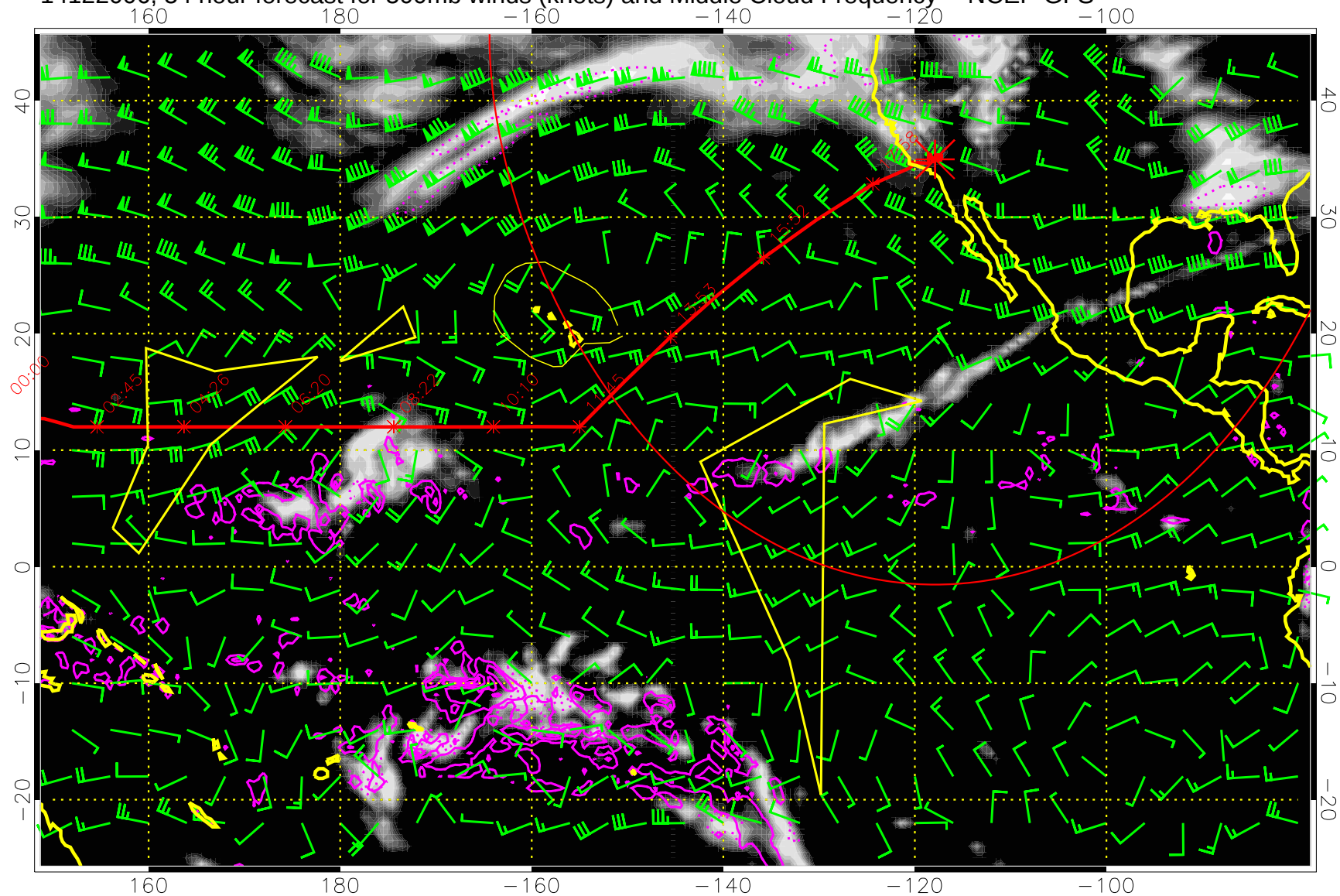
14122006, 54 hour forecast for 500mb winds (knots) and Middle Cloud Frequency -- NCEP GFS
