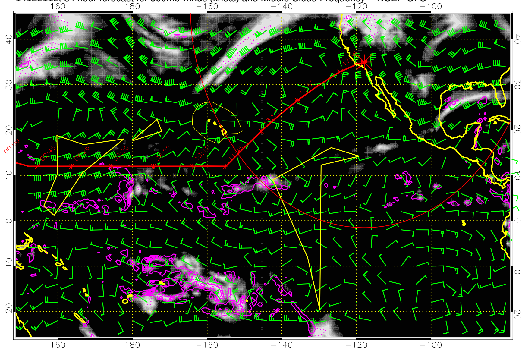
14122112, 84 hour forecast for 500mb winds (knots) and Middle Cloud Frequency -- NCEP GFS
