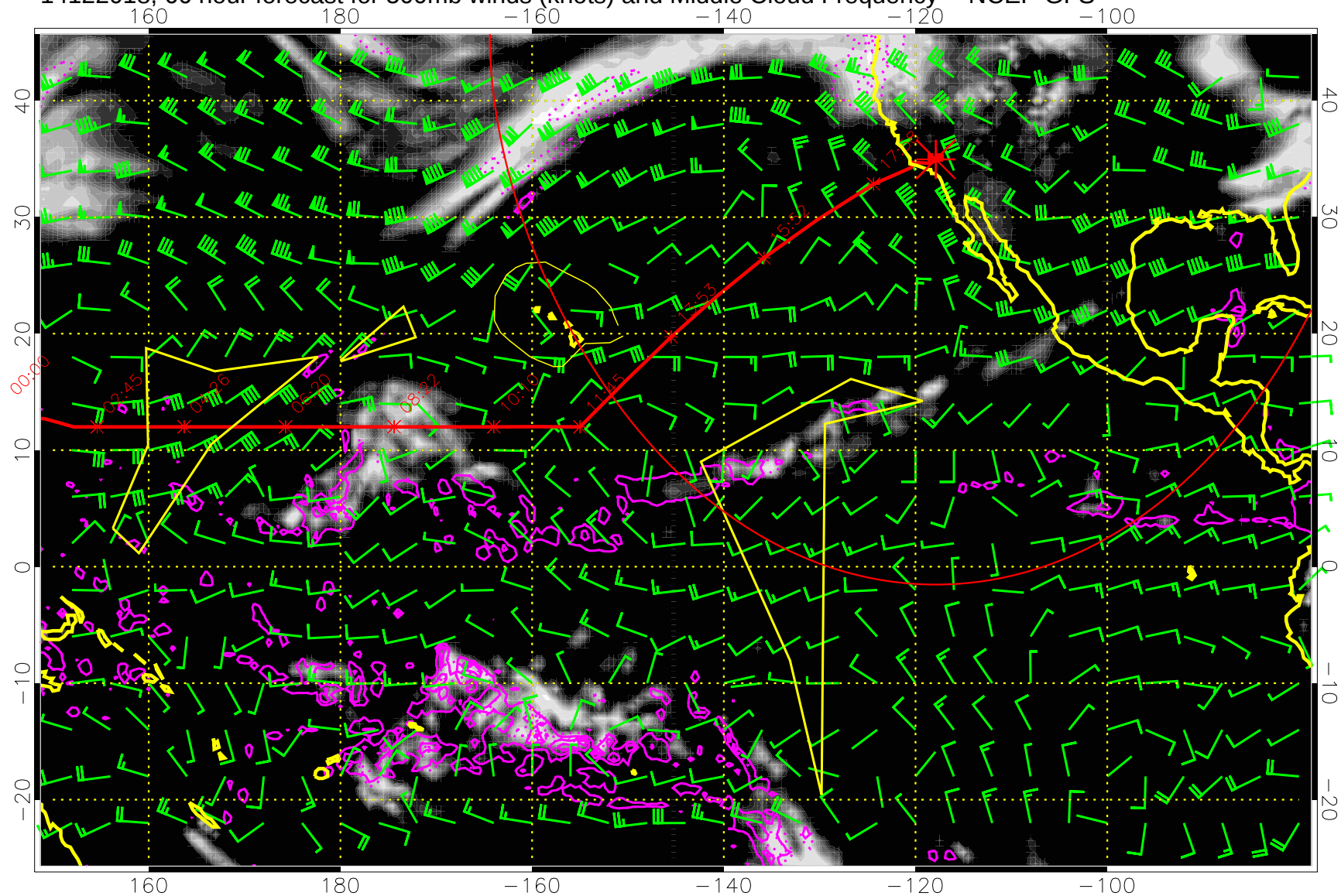
14122018, 66 hour forecast for 500mb winds (knots) and Middle Cloud Frequency -- NCEP GFS
