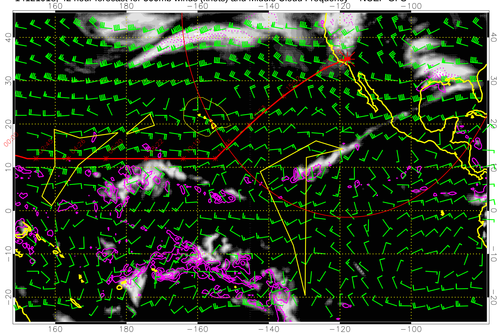
14121918, 42 hour forecast for 500mb winds (knots) and Middle Cloud Frequency -- NCEP GFS
