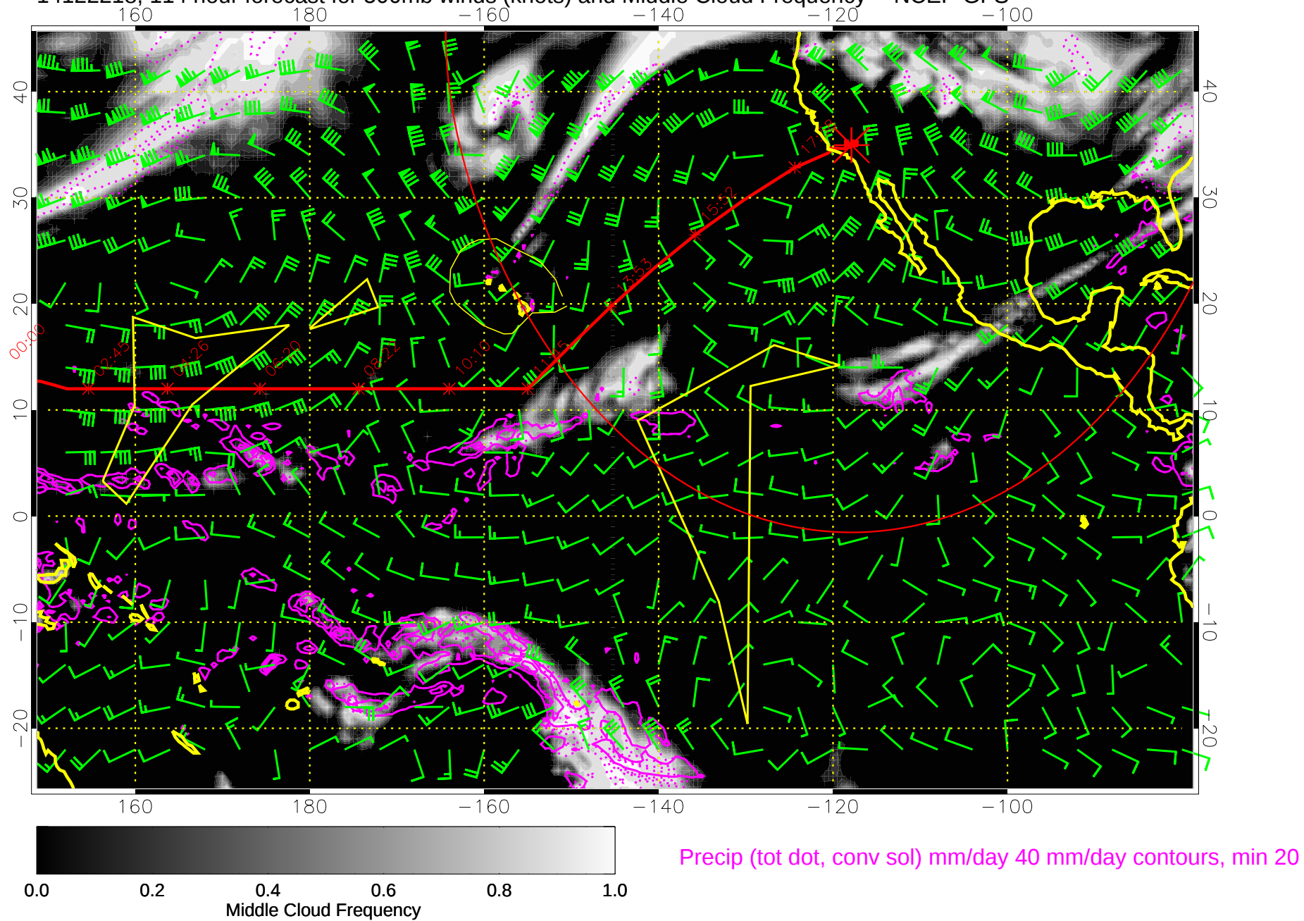
14122218, 114 hour forecast for 500mb winds (knots) and Middle Cloud Frequency -- NCEP GFS
