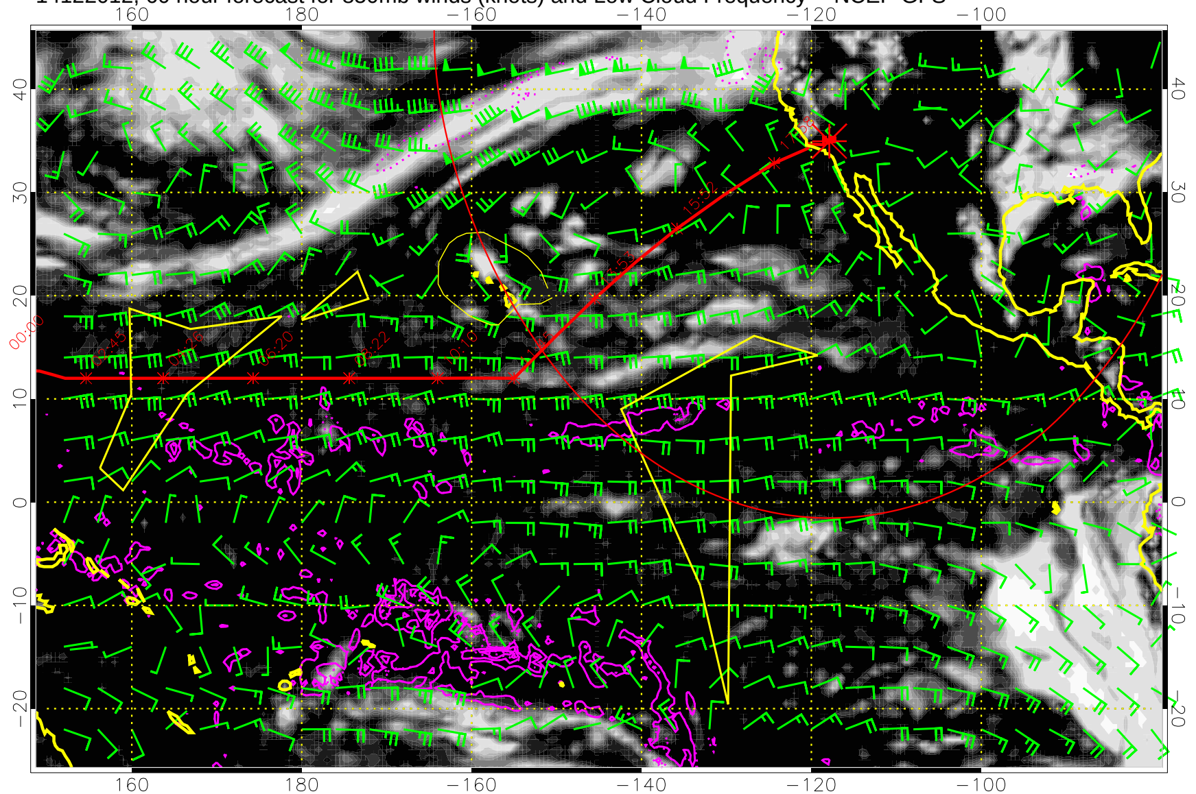
14122012, 60 hour forecast for 850mb winds (knots) and Low Cloud Frequency -- NCEP GFS
