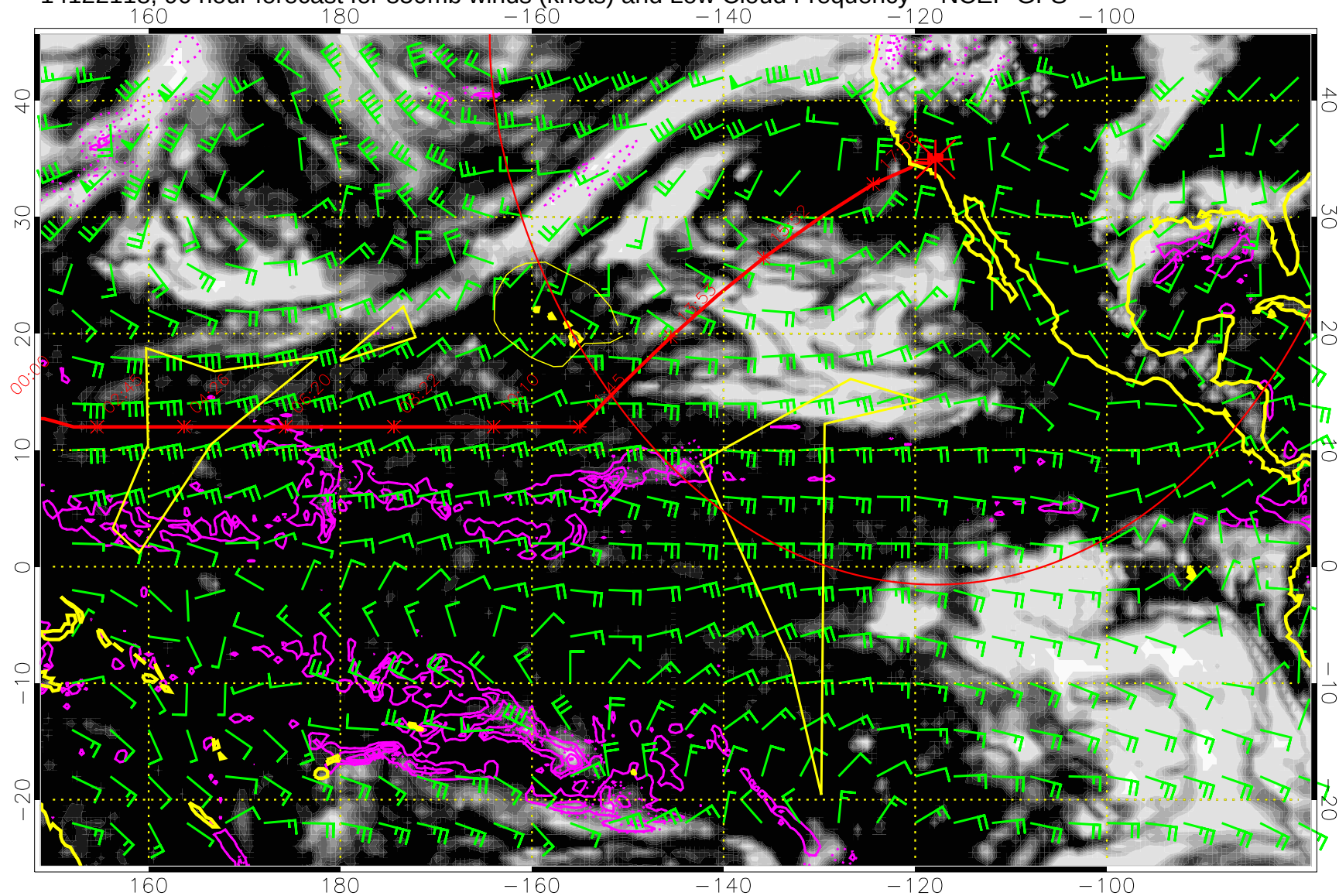
14122118, 90 hour forecast for 850mb winds (knots) and Low Cloud Frequency -- NCEP GFS
