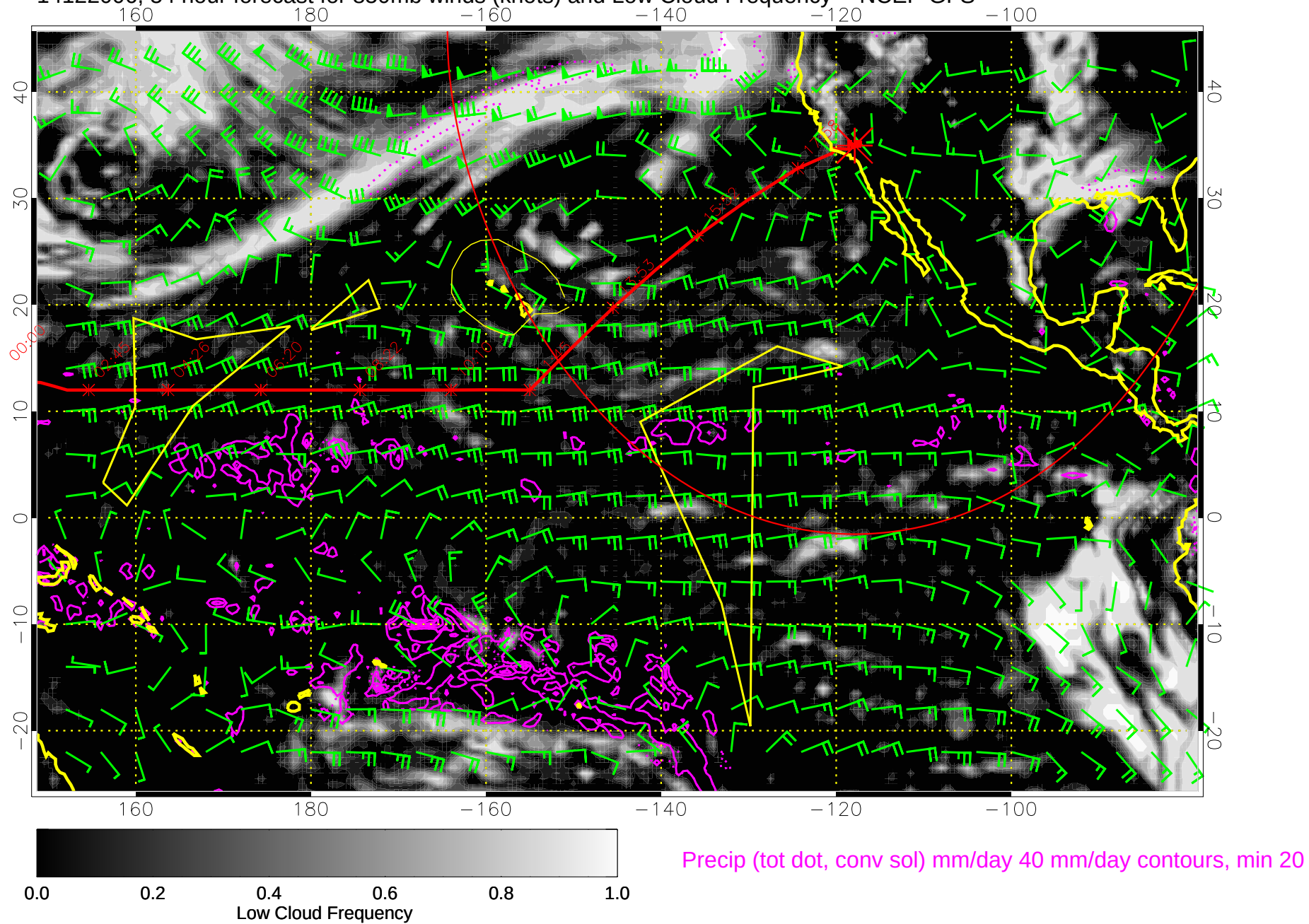
14122006, 54 hour forecast for 850mb winds (knots) and Low Cloud Frequency -- NCEP GFS
