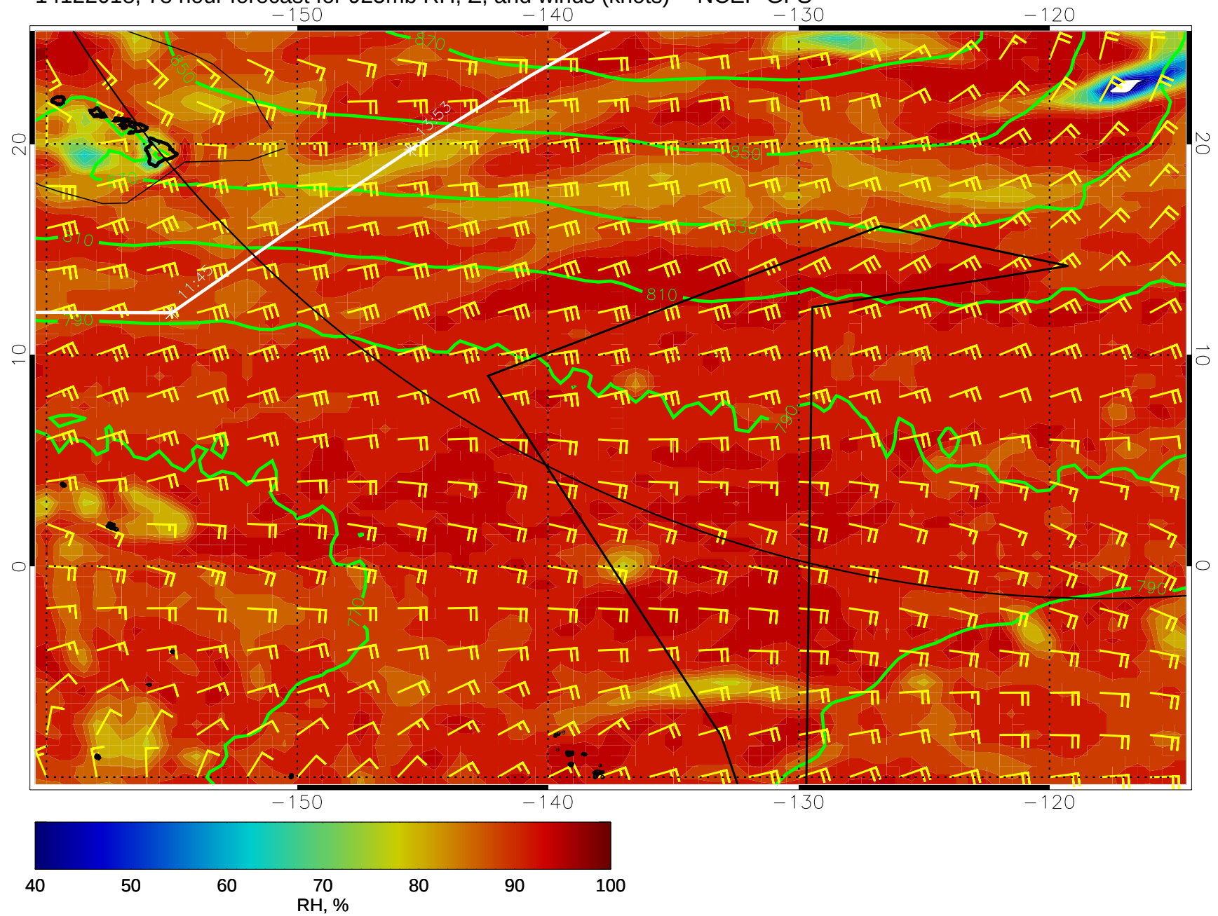
14122018, 78 hour forecast for 925mb RH, Z, and winds (knots) -- NCEP GFS
