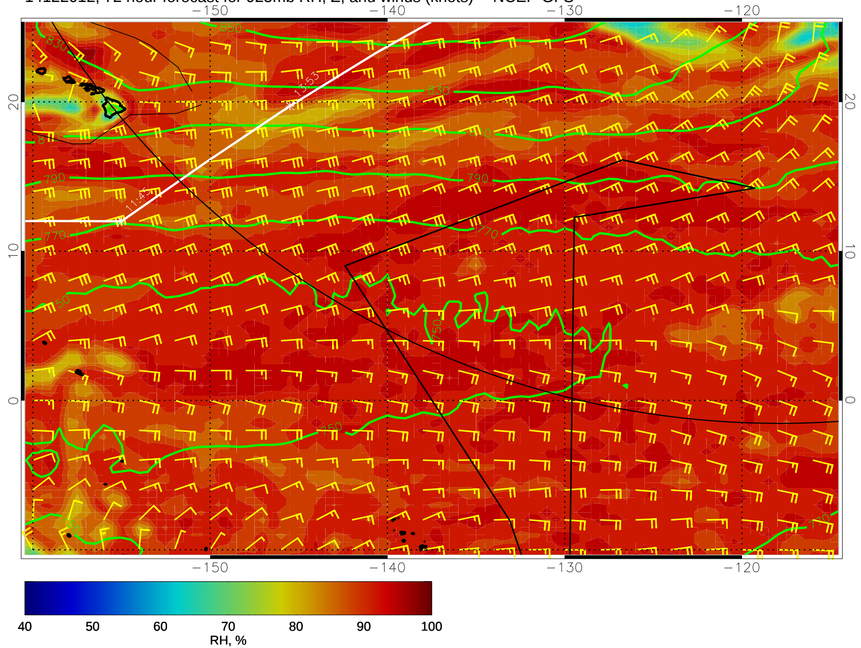
14122012, 72 hour forecast for 925mb RH, Z, and winds (knots) -- NCEP GFS
