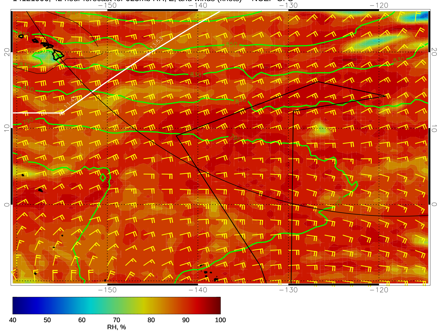
14121906, 42 hour forecast for 925mb RH, Z, and winds (knots) -- NCEP GFS
