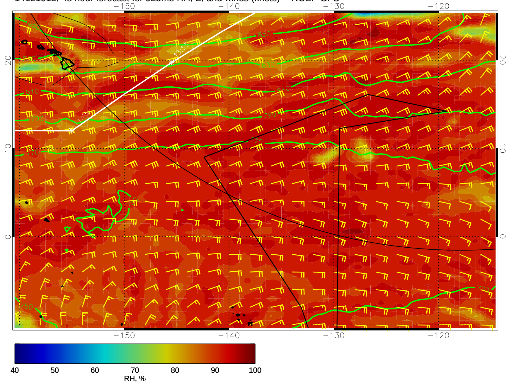
14121912, 48 hour forecast for 925mb RH, Z, and winds (knots) -- NCEP GFS
