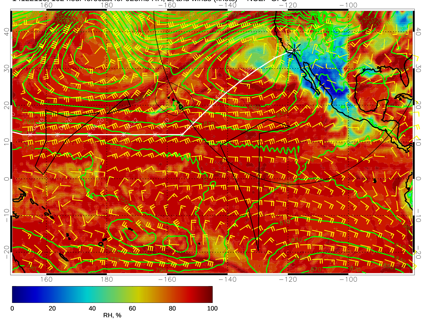
14122118, 102 hour forecast for 925mb RH, Z, and winds (knots) -- NCEP GFS
