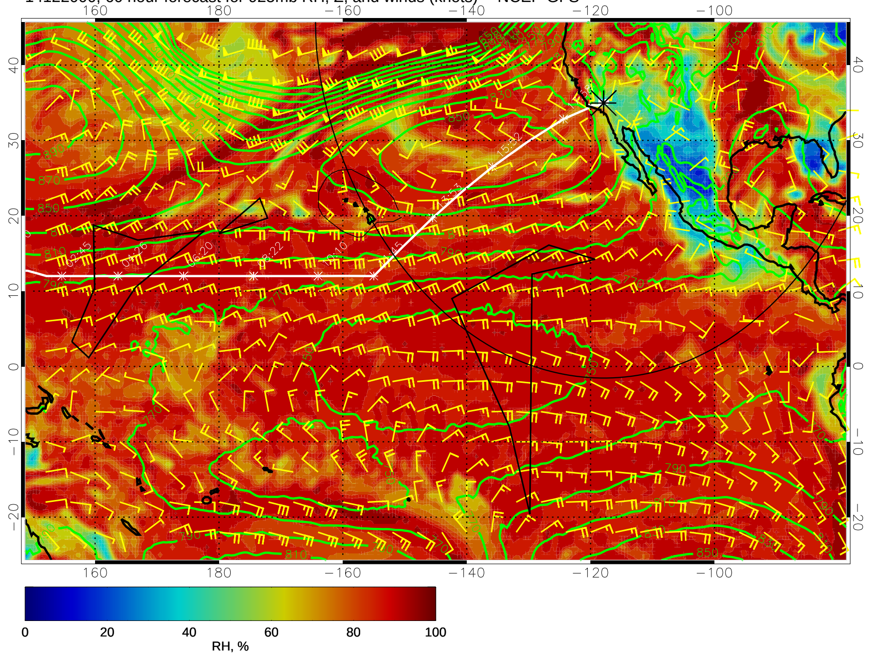
14122000, 60 hour forecast for 925mb RH, Z, and winds (knots) -- NCEP GFS
