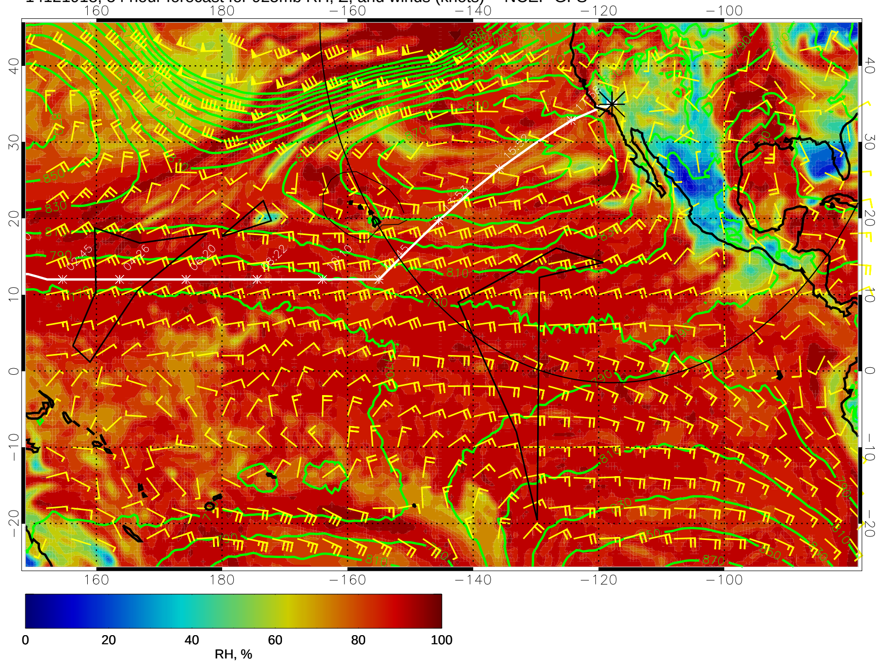
14121918, 54 hour forecast for 925mb RH, Z, and winds (knots) -- NCEP GFS
