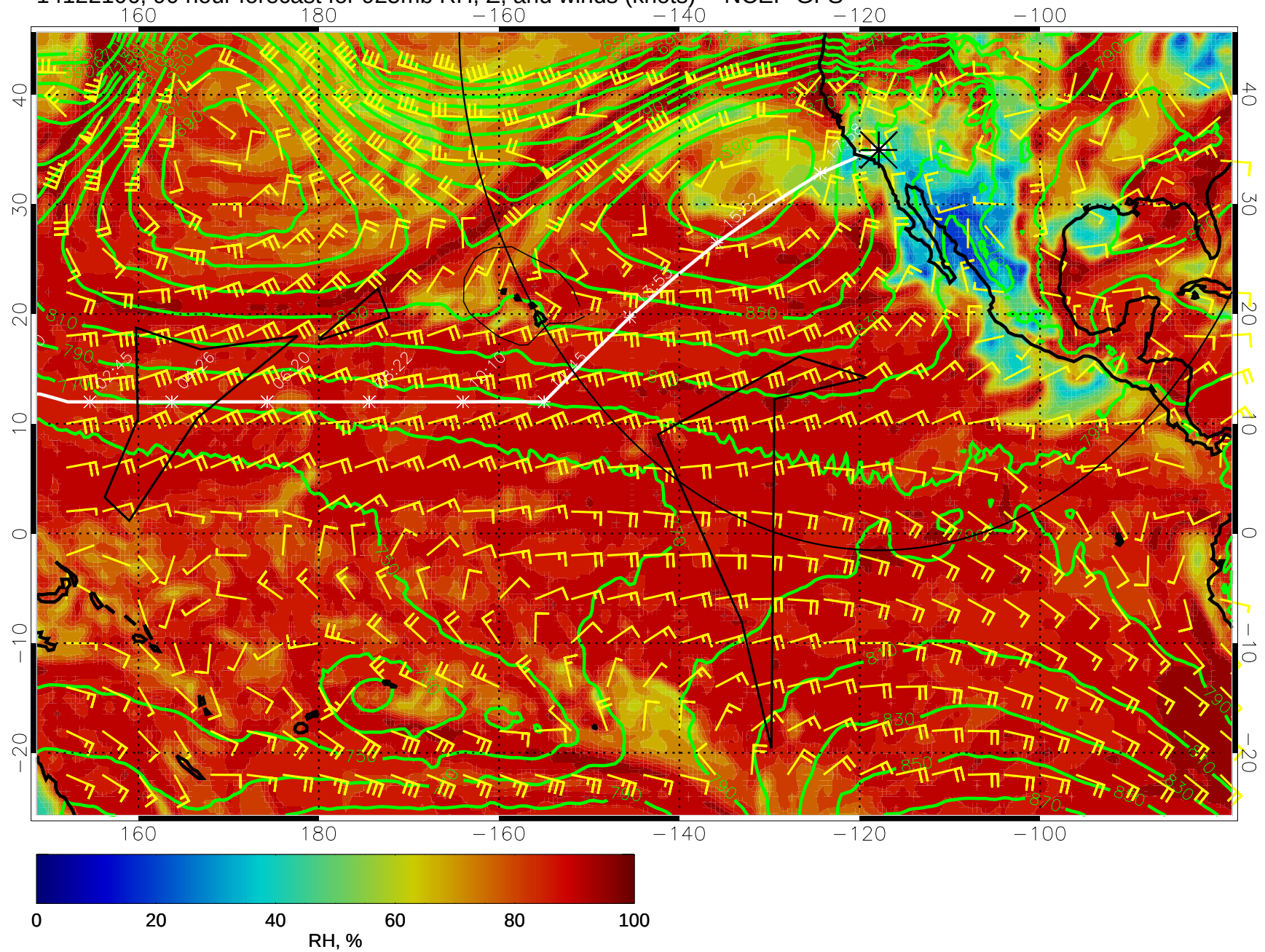
14122106, 90 hour forecast for 925mb RH, Z, and winds (knots) -- NCEP GFS
