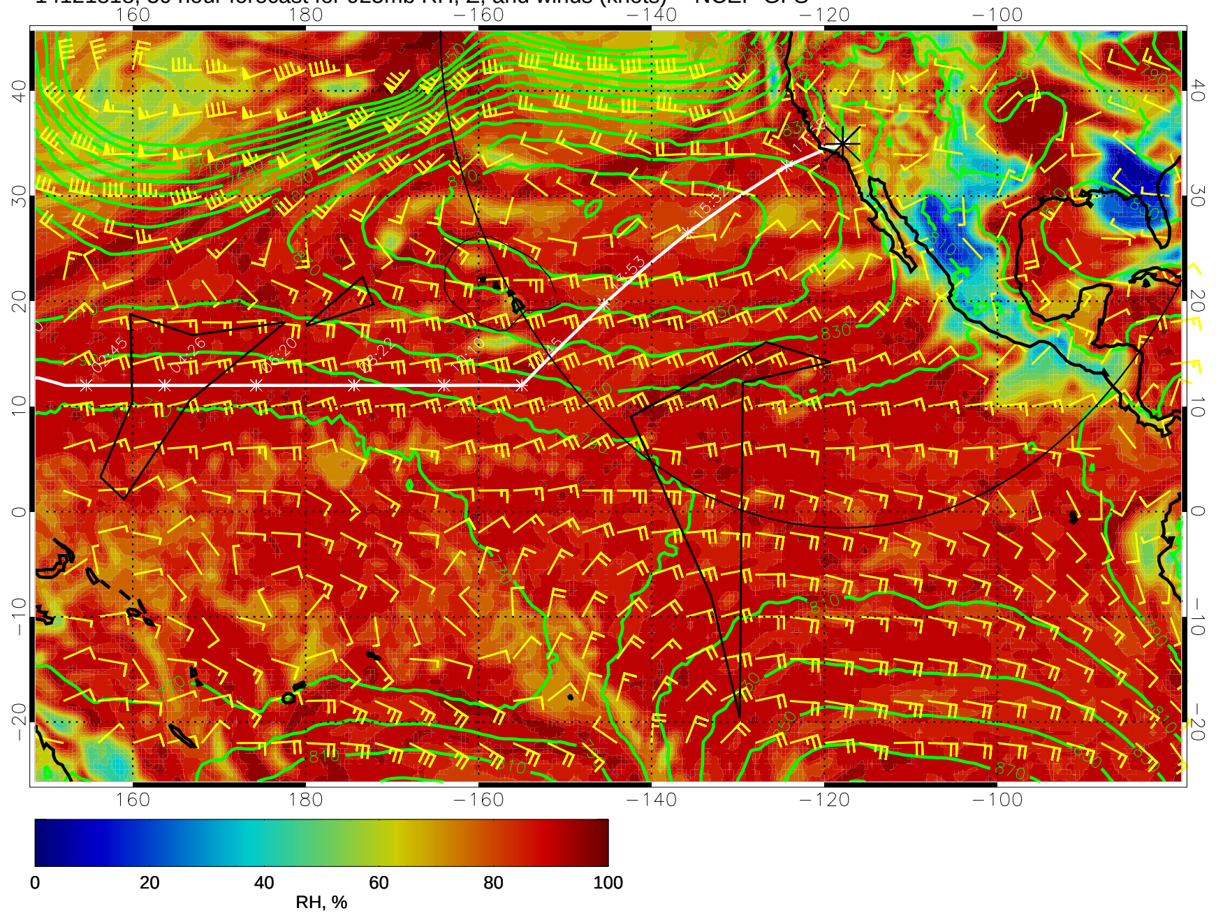
14121818, 30 hour forecast for 925mb RH, Z, and winds (knots) -- NCEP GFS
