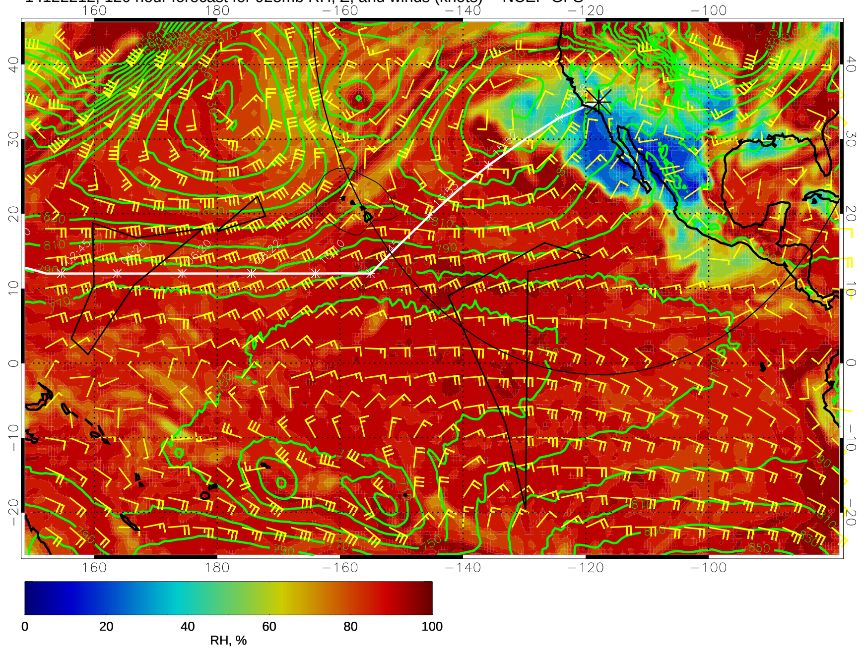
14122212, 120 hour forecast for 925mb RH, Z, and winds (knots) -- NCEP GFS
