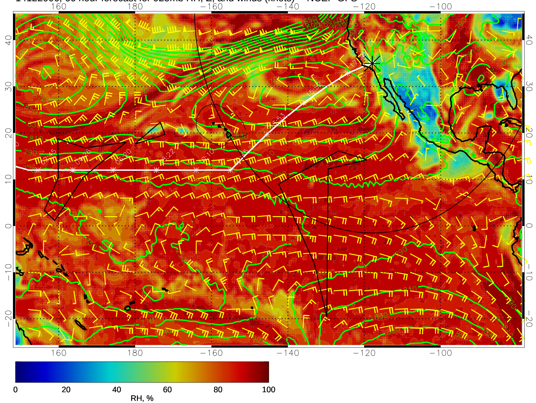
14122006, 66 hour forecast for 925mb RH, Z, and winds (knots) -- NCEP GFS
