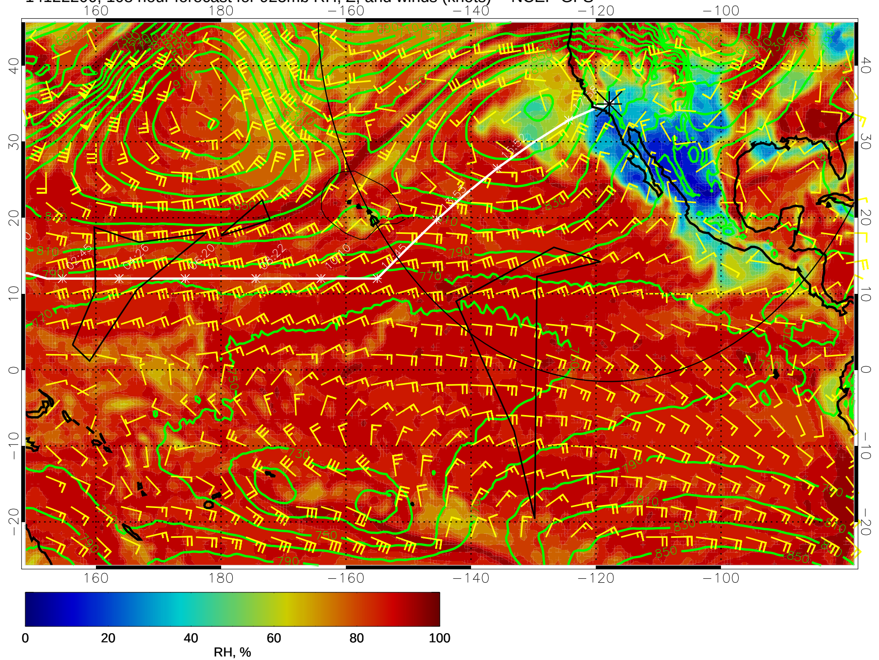
14122200, 108 hour forecast for 925mb RH, Z, and winds (knots) -- NCEP GFS
