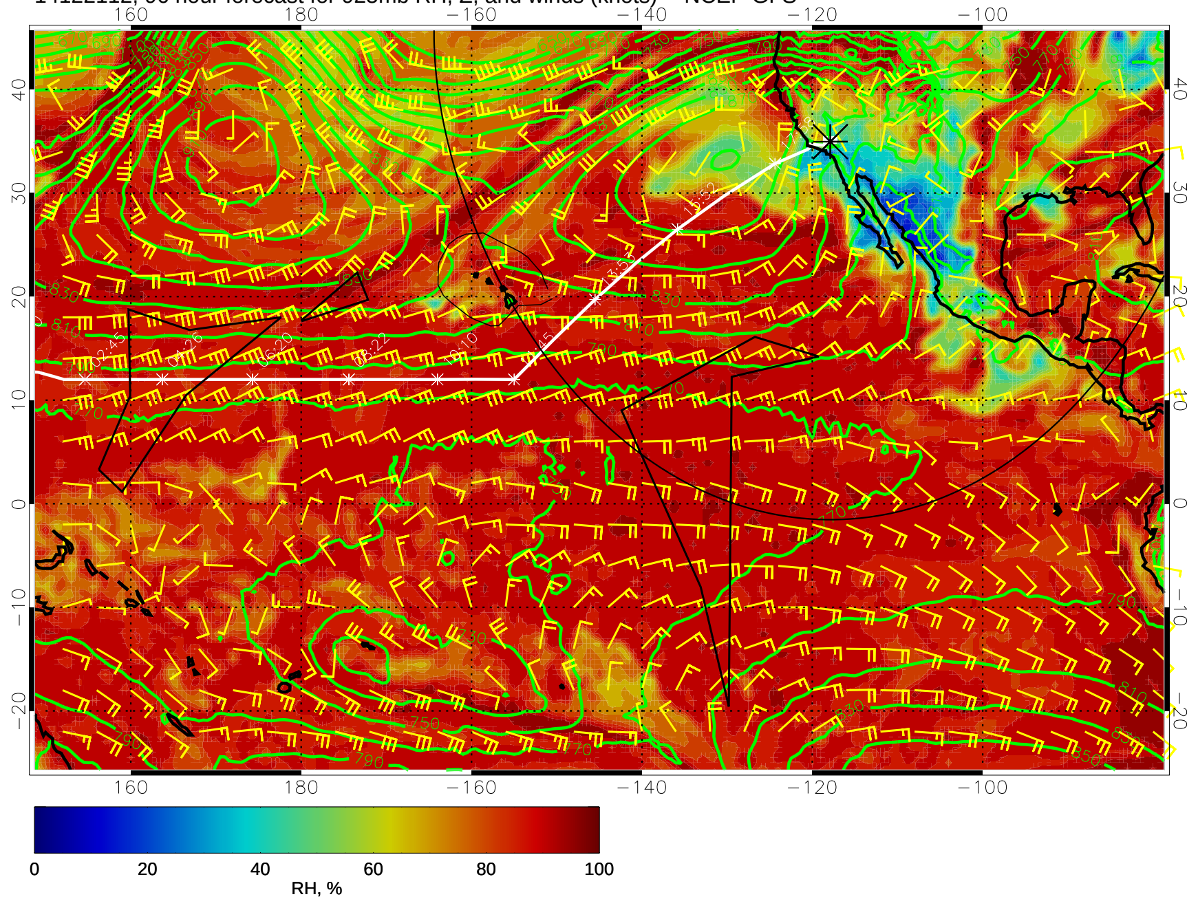
14122112, 96 hour forecast for 925mb RH, Z, and winds (knots) -- NCEP GFS
