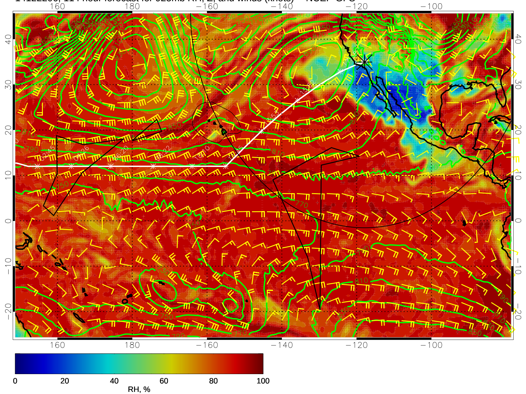
14122206, 114 hour forecast for 925mb RH, Z, and winds (knots) -- NCEP GFS
