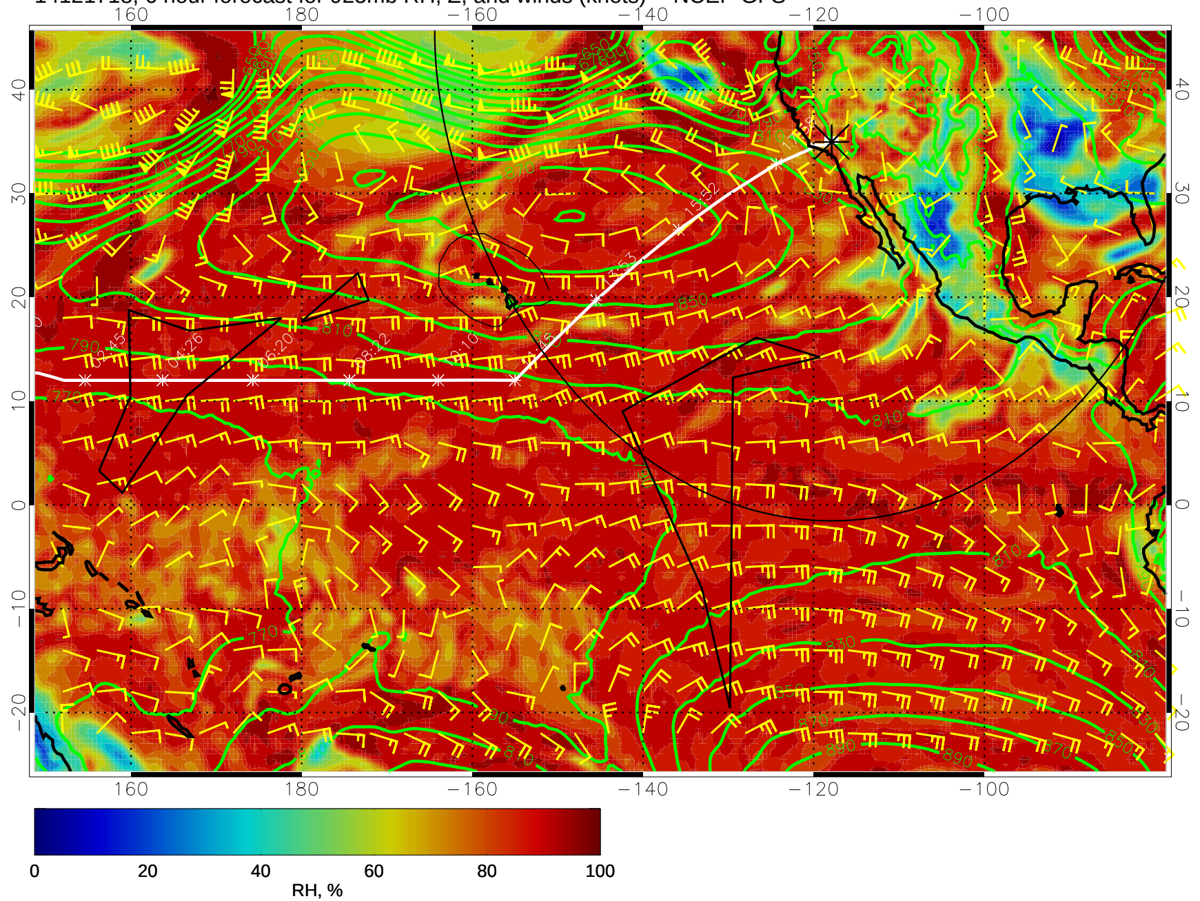
14121718, 6 hour forecast for 925mb RH, Z, and winds (knots) -- NCEP GFS
