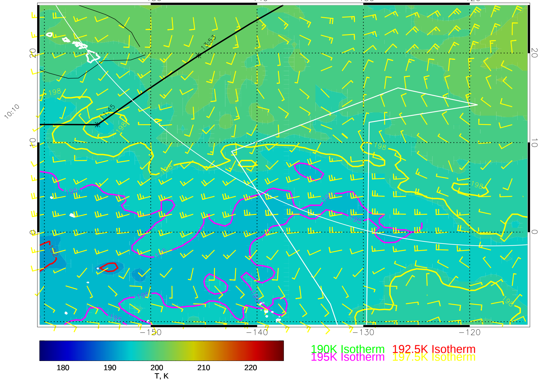
14122212, 120 hour forecast for 70mb T and winds (knots) -- NCEP GFS
