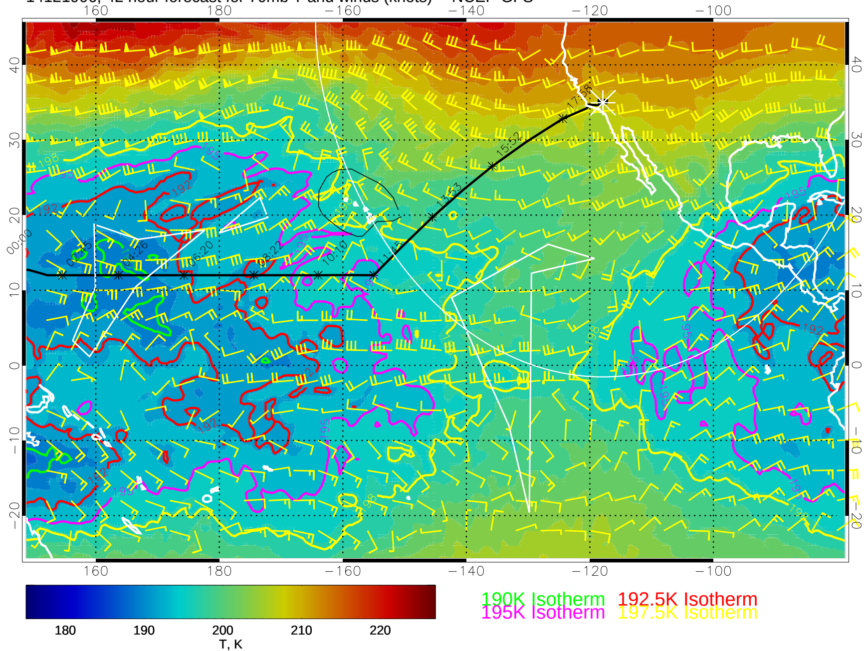
14121906, 42 hour forecast for 70mb T and winds (knots) -- NCEP GFS
