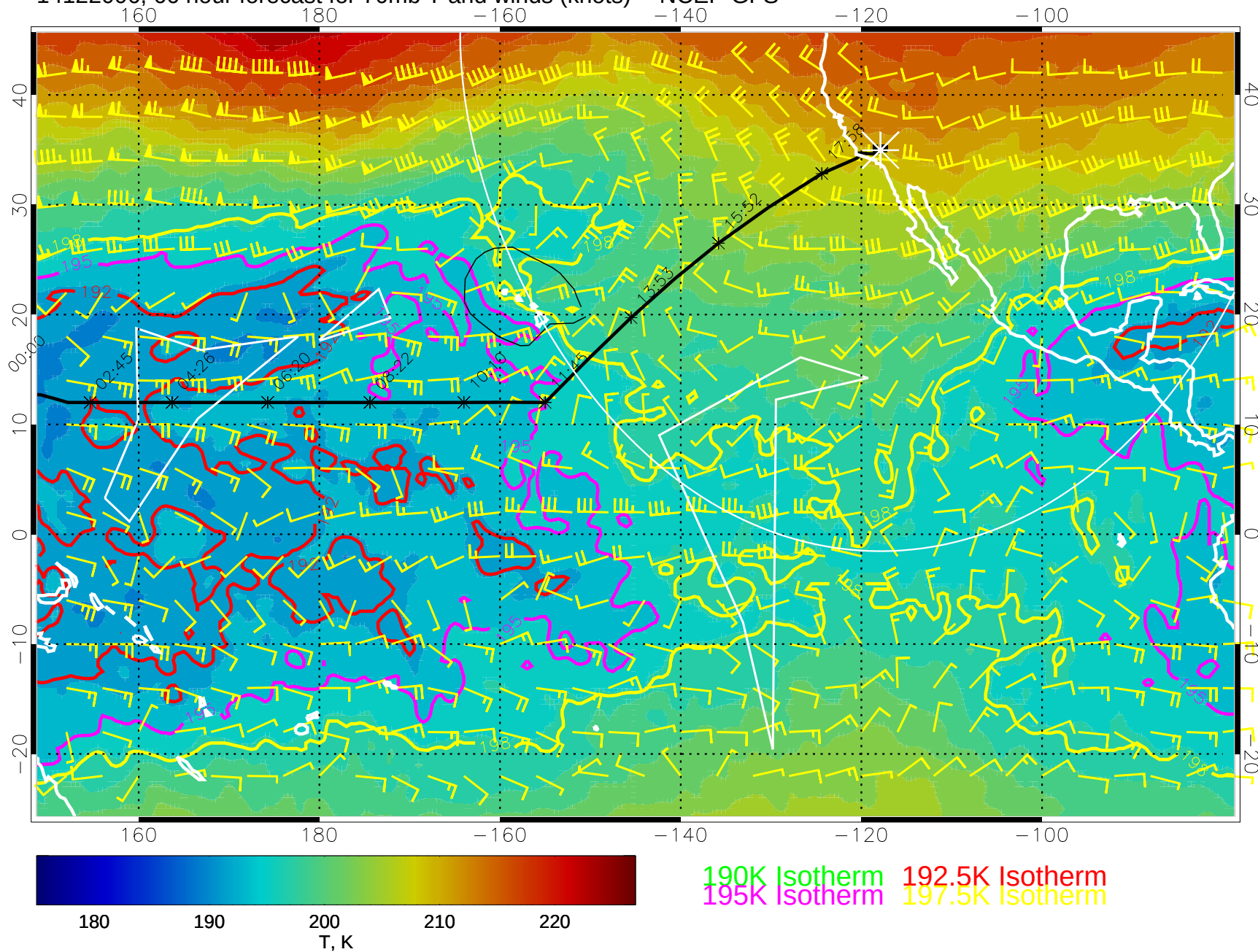
14122006, 66 hour forecast for 70mb T and winds (knots) -- NCEP GFS
