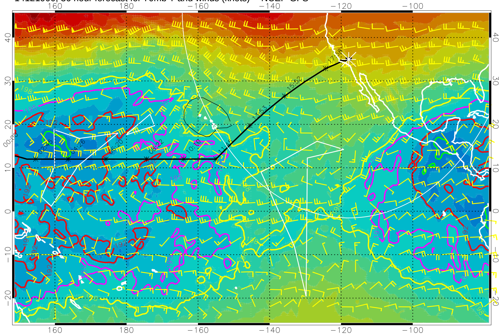
14121900, 36 hour forecast for 70mb T and winds (knots) -- NCEP GFS
