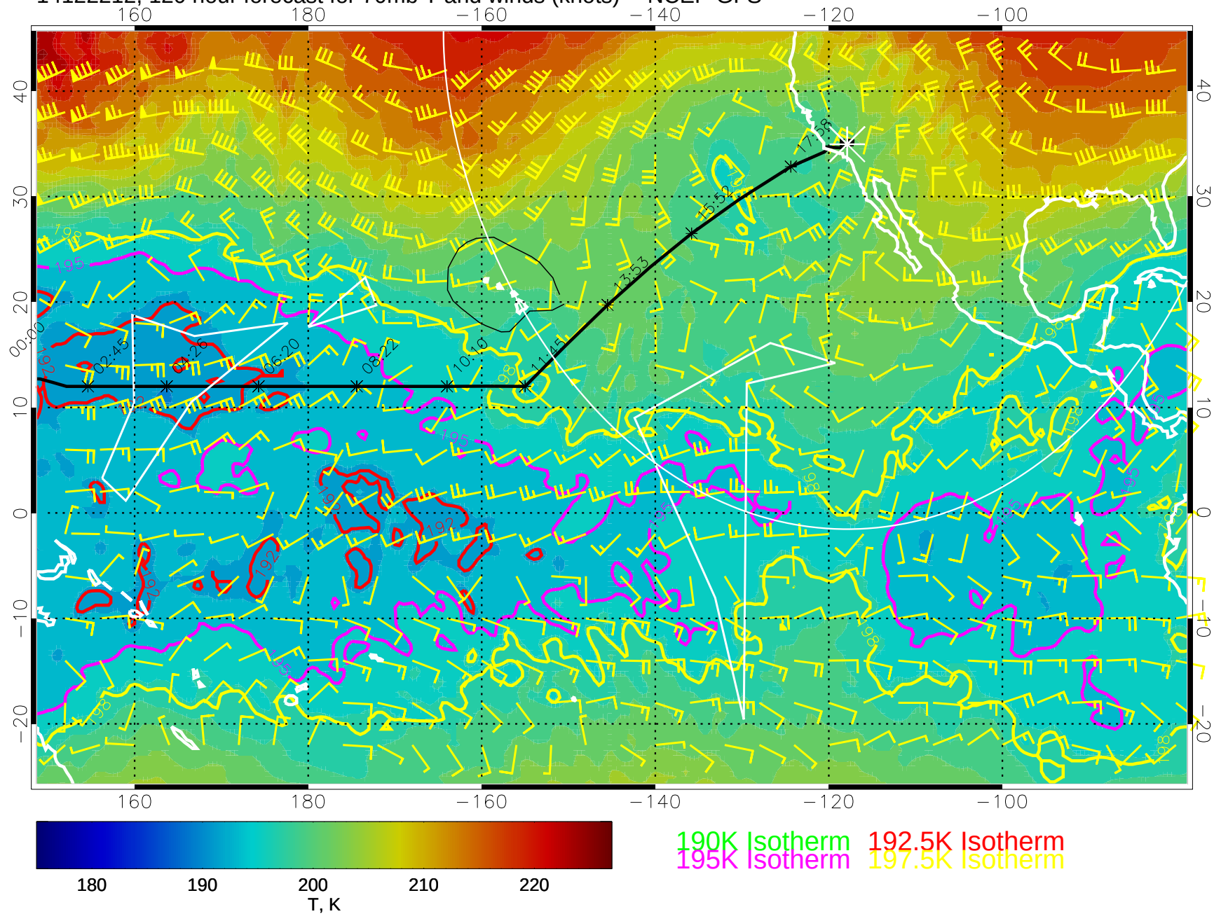
14122212, 120 hour forecast for 70mb T and winds (knots) -- NCEP GFS
