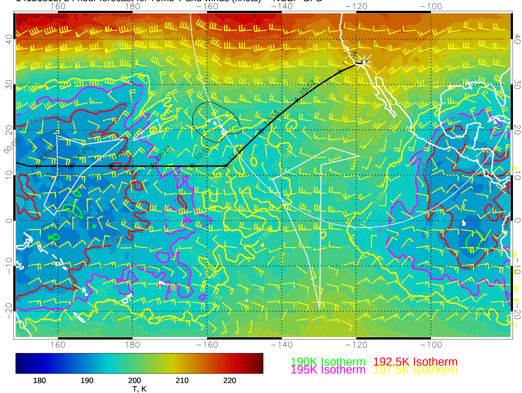
14121812, 24 hour forecast for 70mb T and winds (knots) -- NCEP GFS
