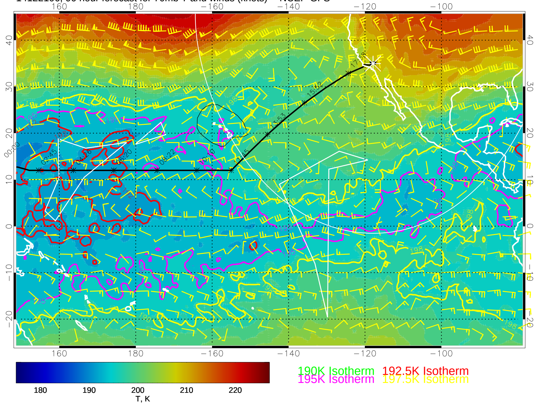
14122106, 90 hour forecast for 70mb T and winds (knots) -- NCEP GFS
