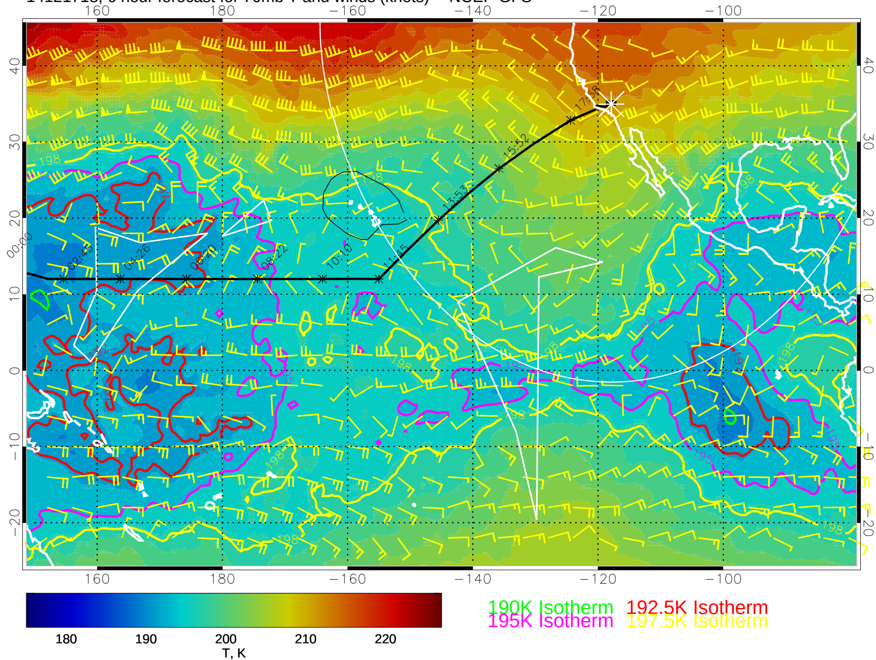
14121718, 6 hour forecast for 70mb T and winds (knots) -- NCEP GFS
