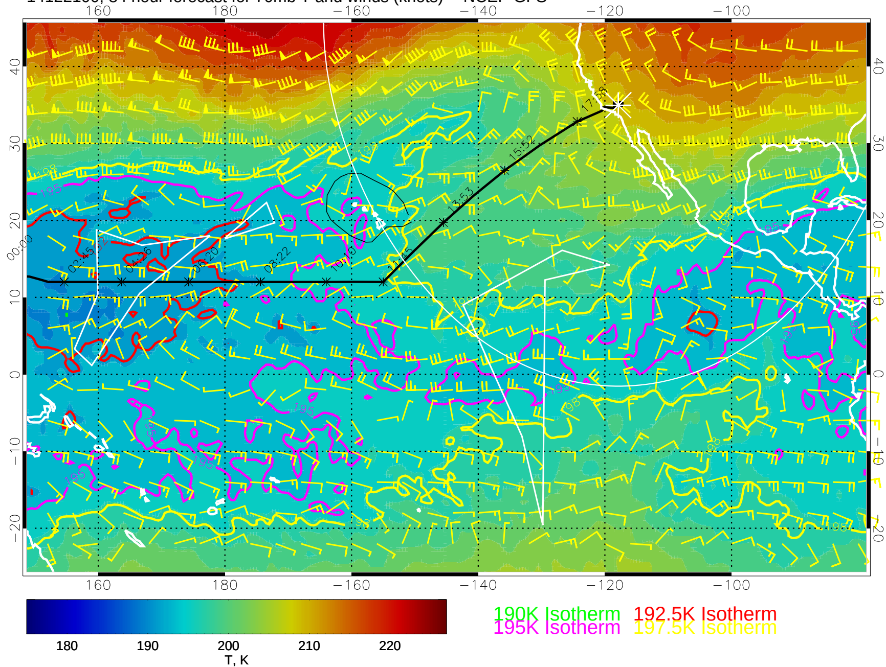
14122100, 84 hour forecast for 70mb T and winds (knots) -- NCEP GFS
