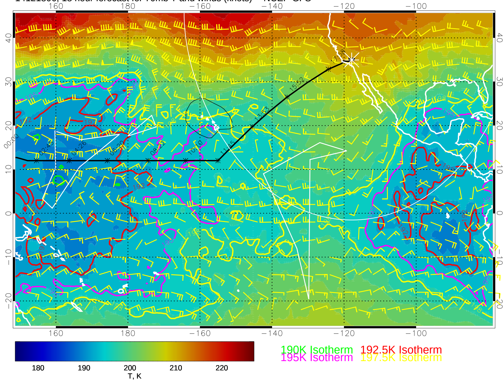
14121806, 18 hour forecast for 70mb T and winds (knots) -- NCEP GFS
