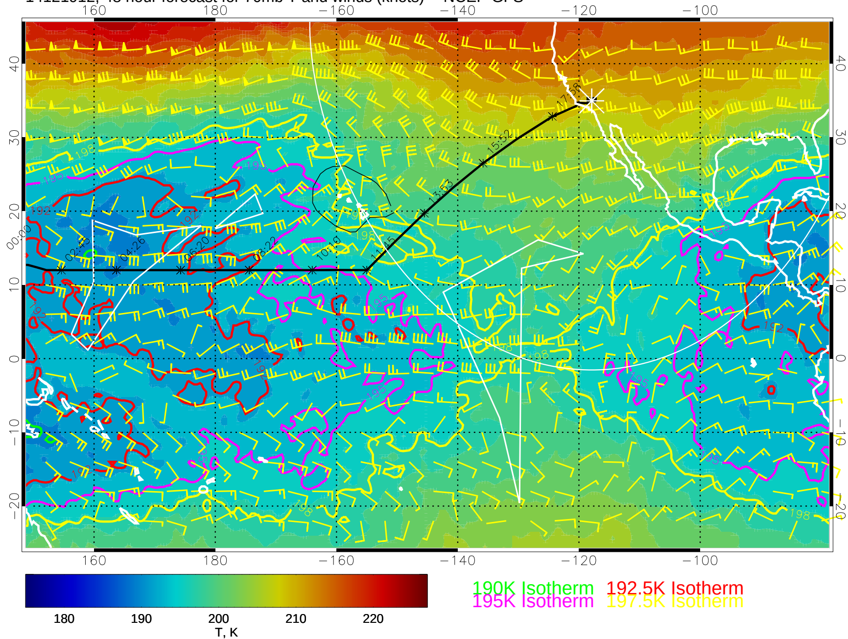
14121912, 48 hour forecast for 70mb T and winds (knots) -- NCEP GFS
