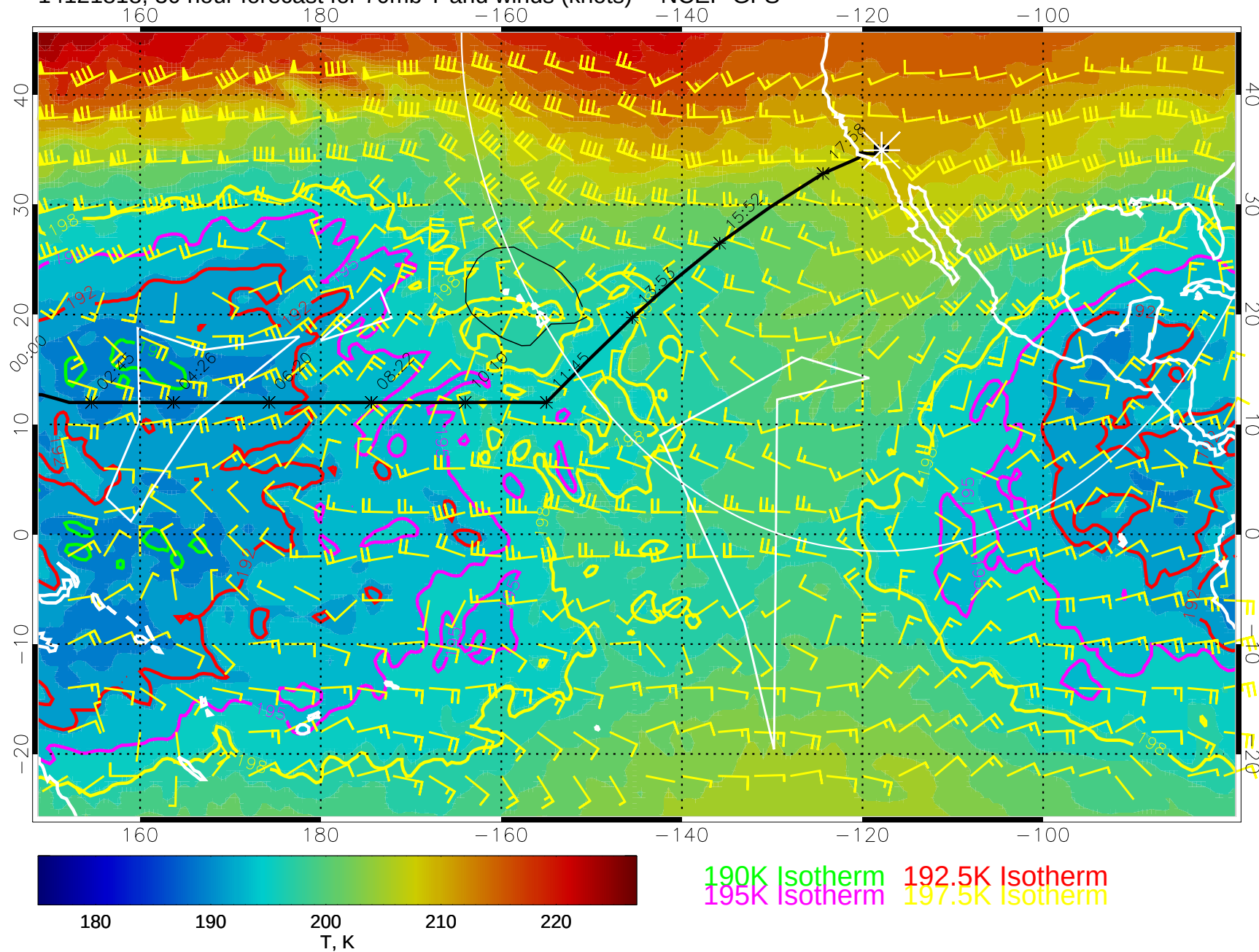
14121818, 30 hour forecast for 70mb T and winds (knots) -- NCEP GFS
