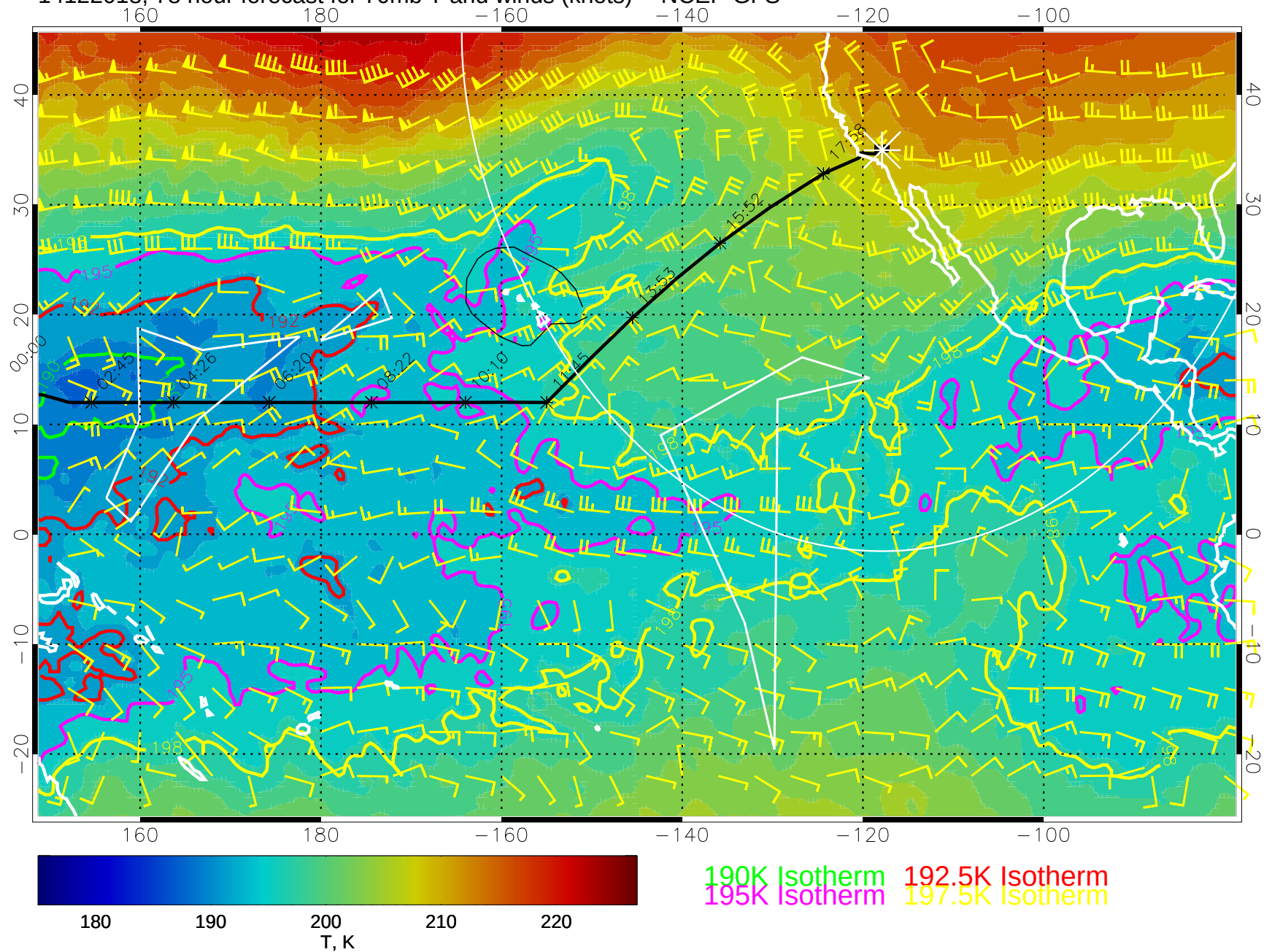
14122018, 78 hour forecast for 70mb T and winds (knots) -- NCEP GFS
