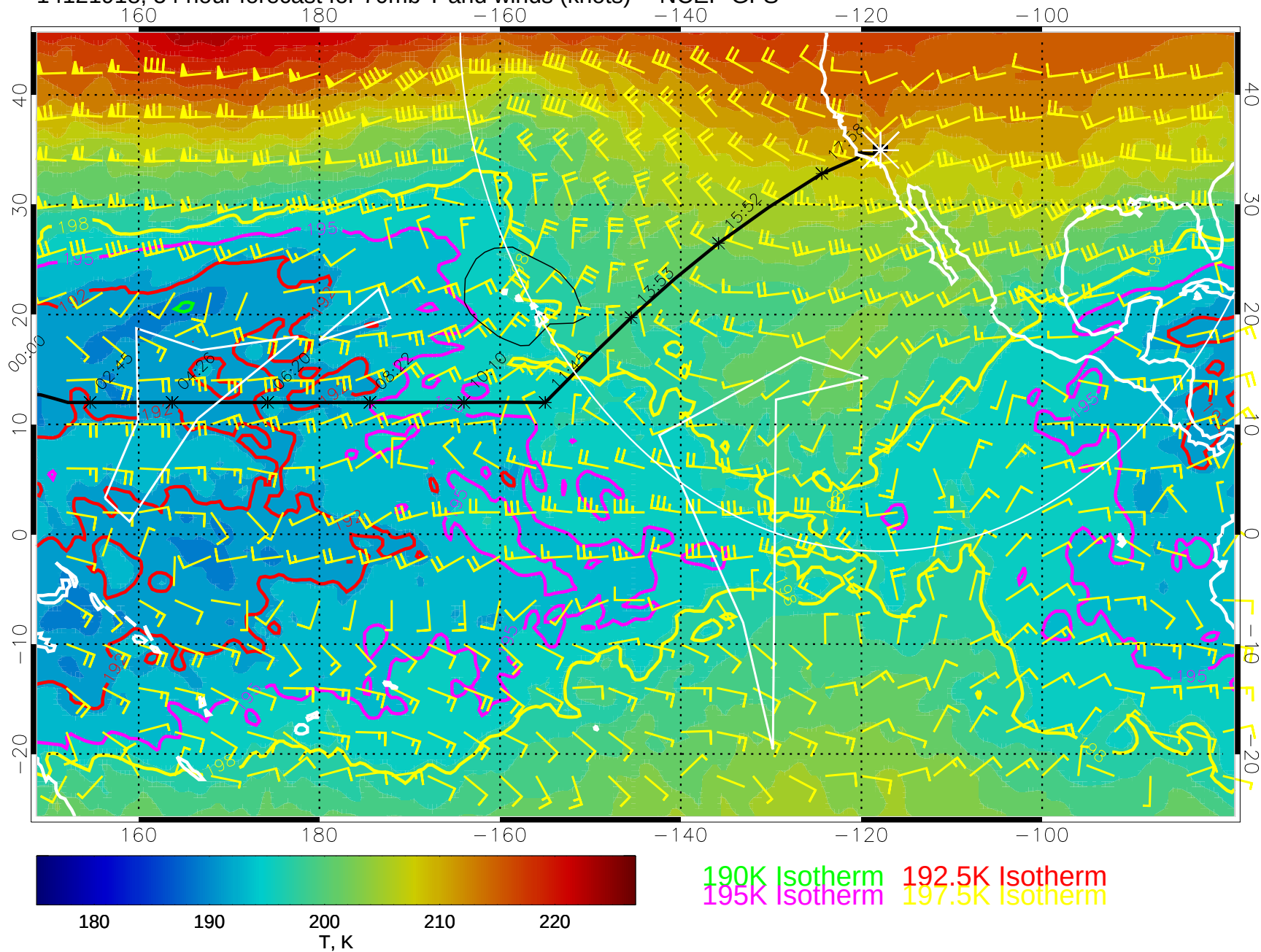
14121918, 54 hour forecast for 70mb T and winds (knots) -- NCEP GFS
