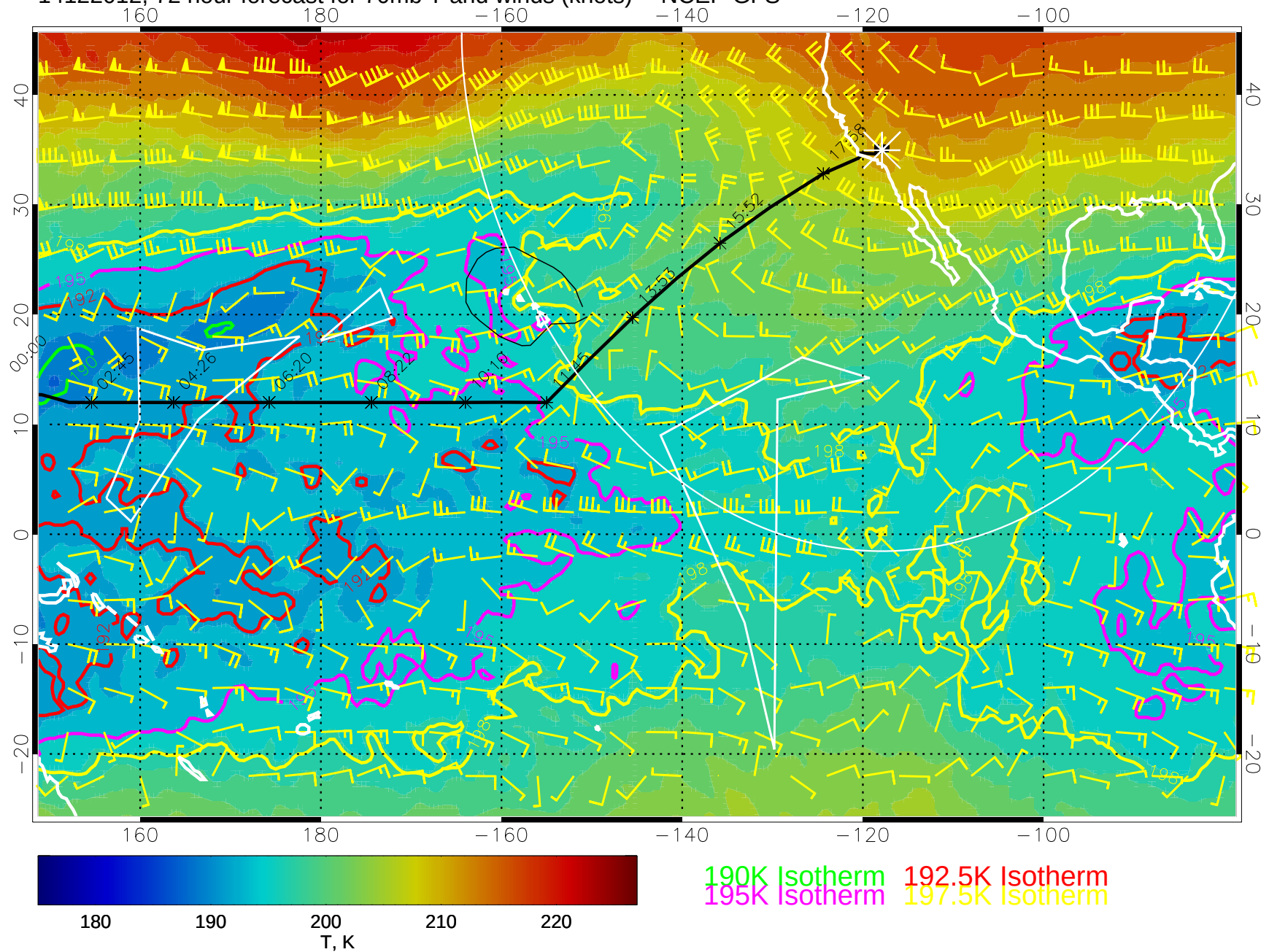
14122012, 72 hour forecast for 70mb T and winds (knots) -- NCEP GFS
