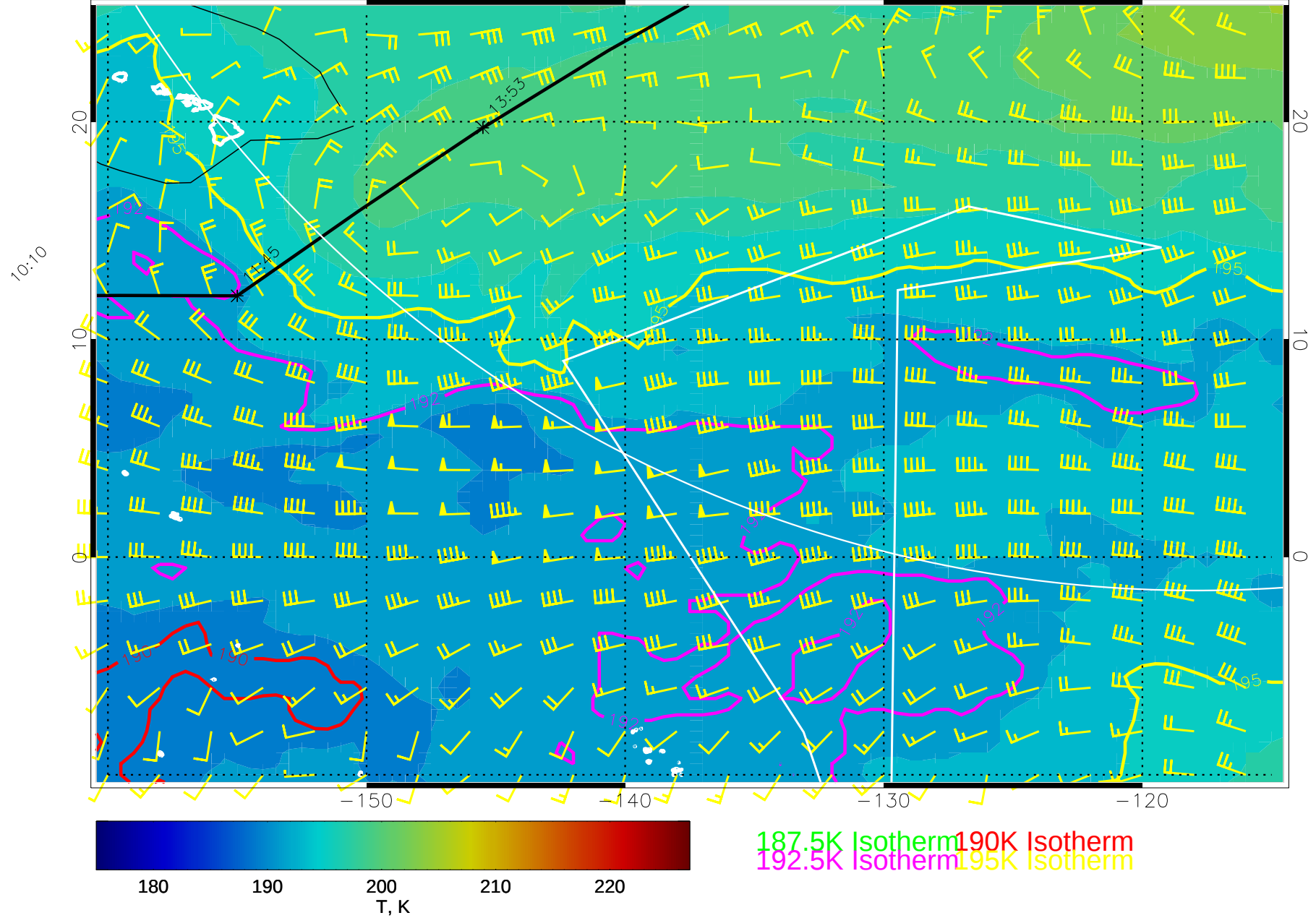
14122112, 96 hour forecast for 100mb T and winds (knots) -- NCEP GFS
