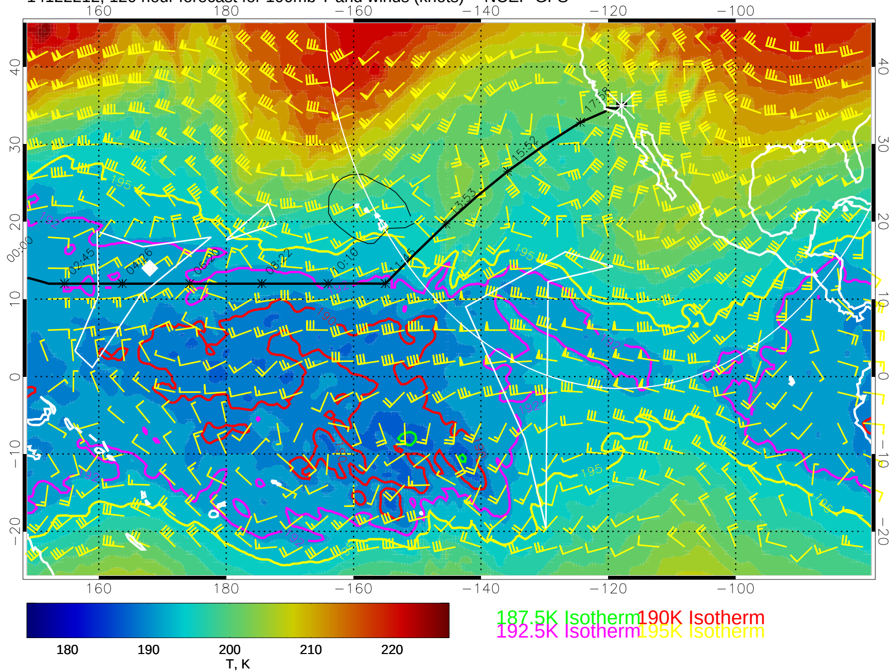
14122212, 120 hour forecast for 100mb T and winds (knots) -- NCEP GFS
