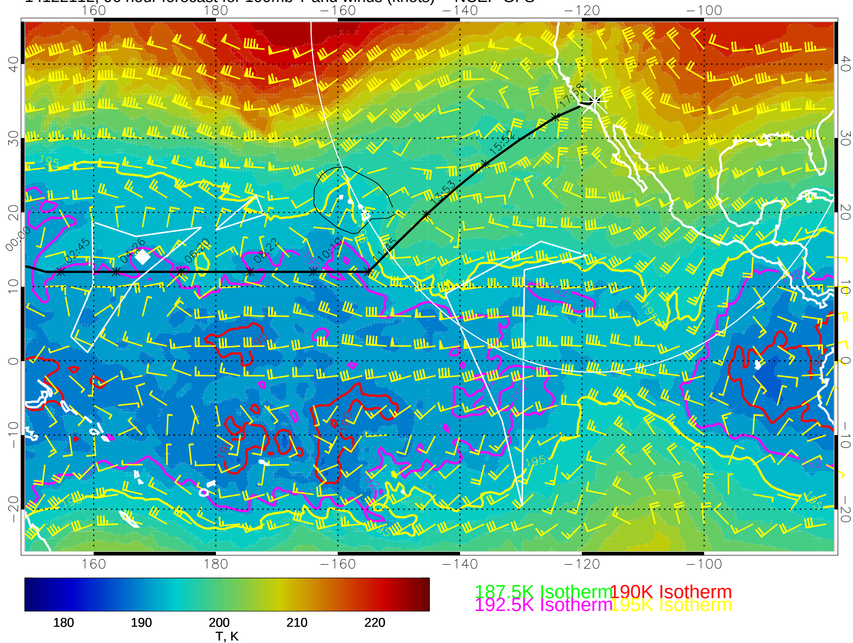
14122112, 96 hour forecast for 100mb T and winds (knots) -- NCEP GFS
