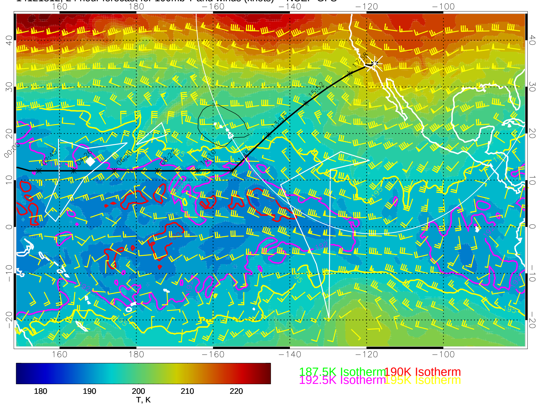
14121812, 24 hour forecast for 100mb T and winds (knots) -- NCEP GFS
