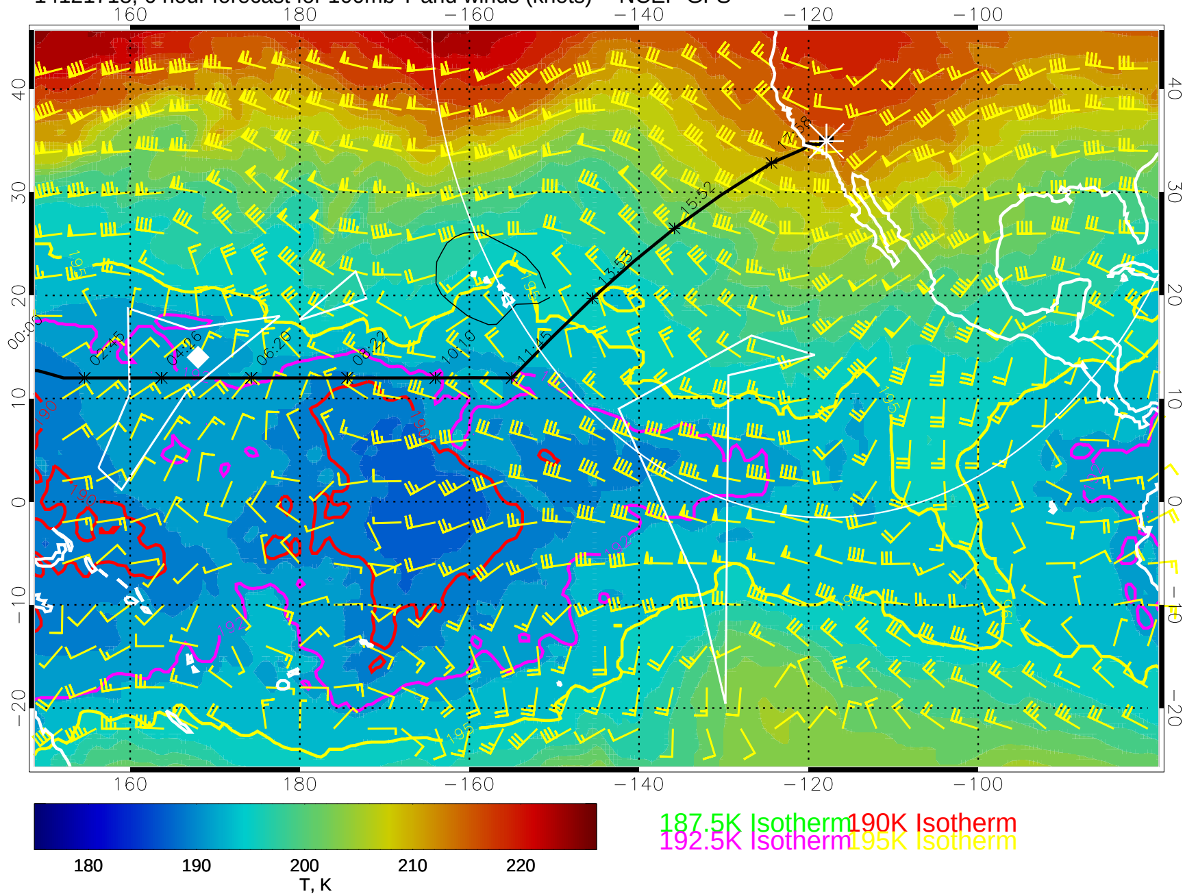
14121718, 6 hour forecast for 100mb T and winds (knots) -- NCEP GFS
