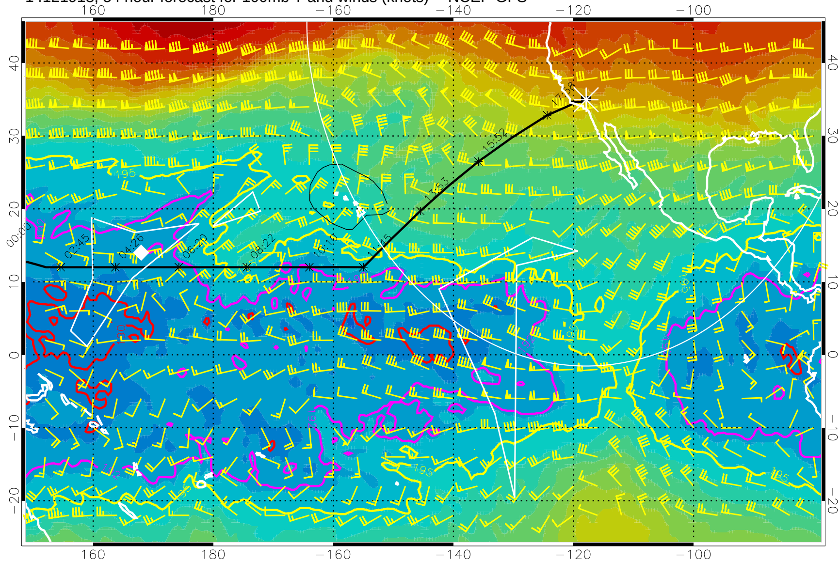
14121918, 54 hour forecast for 100mb T and winds (knots) -- NCEP GFS
