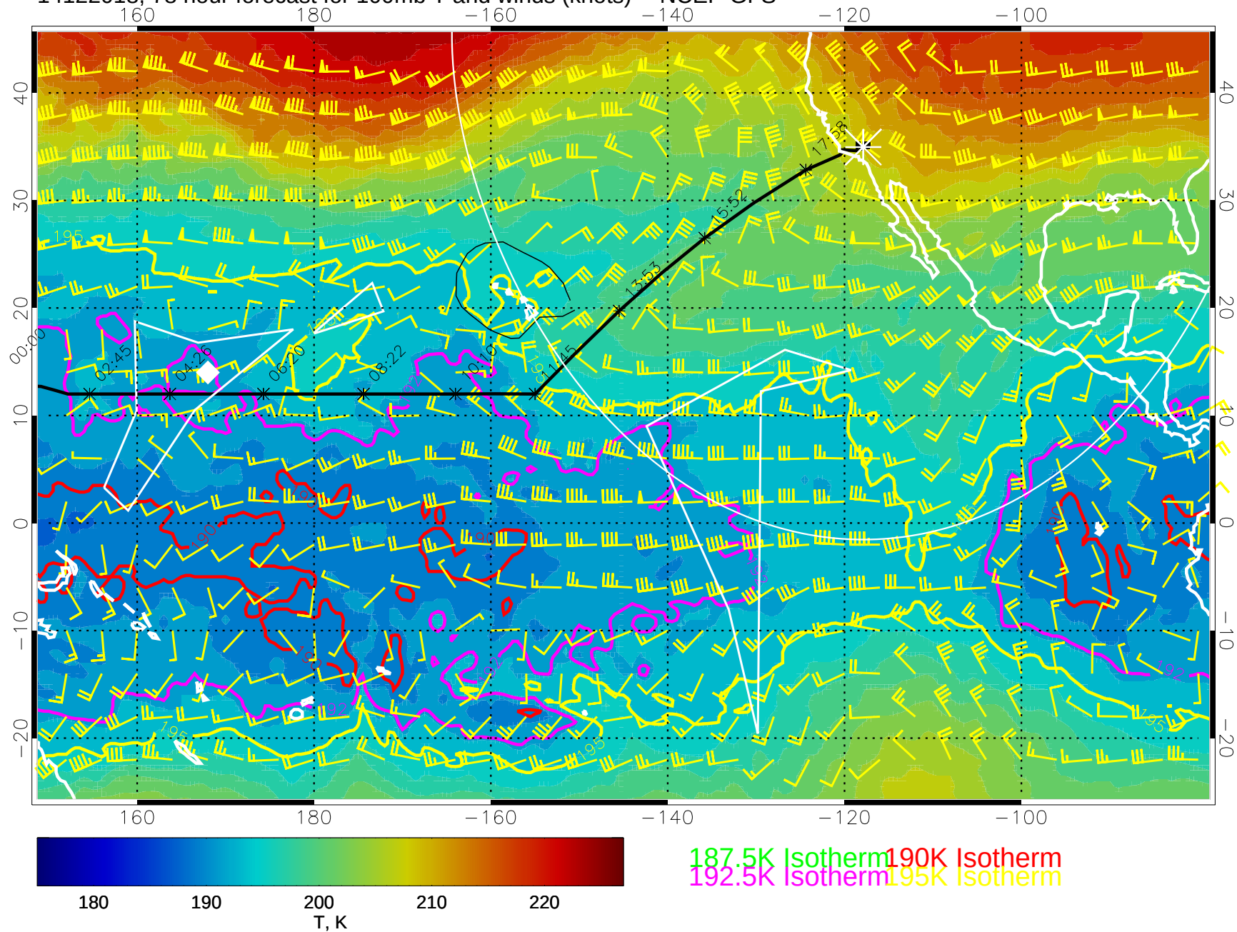
14122018, 78 hour forecast for 100mb T and winds (knots) -- NCEP GFS
