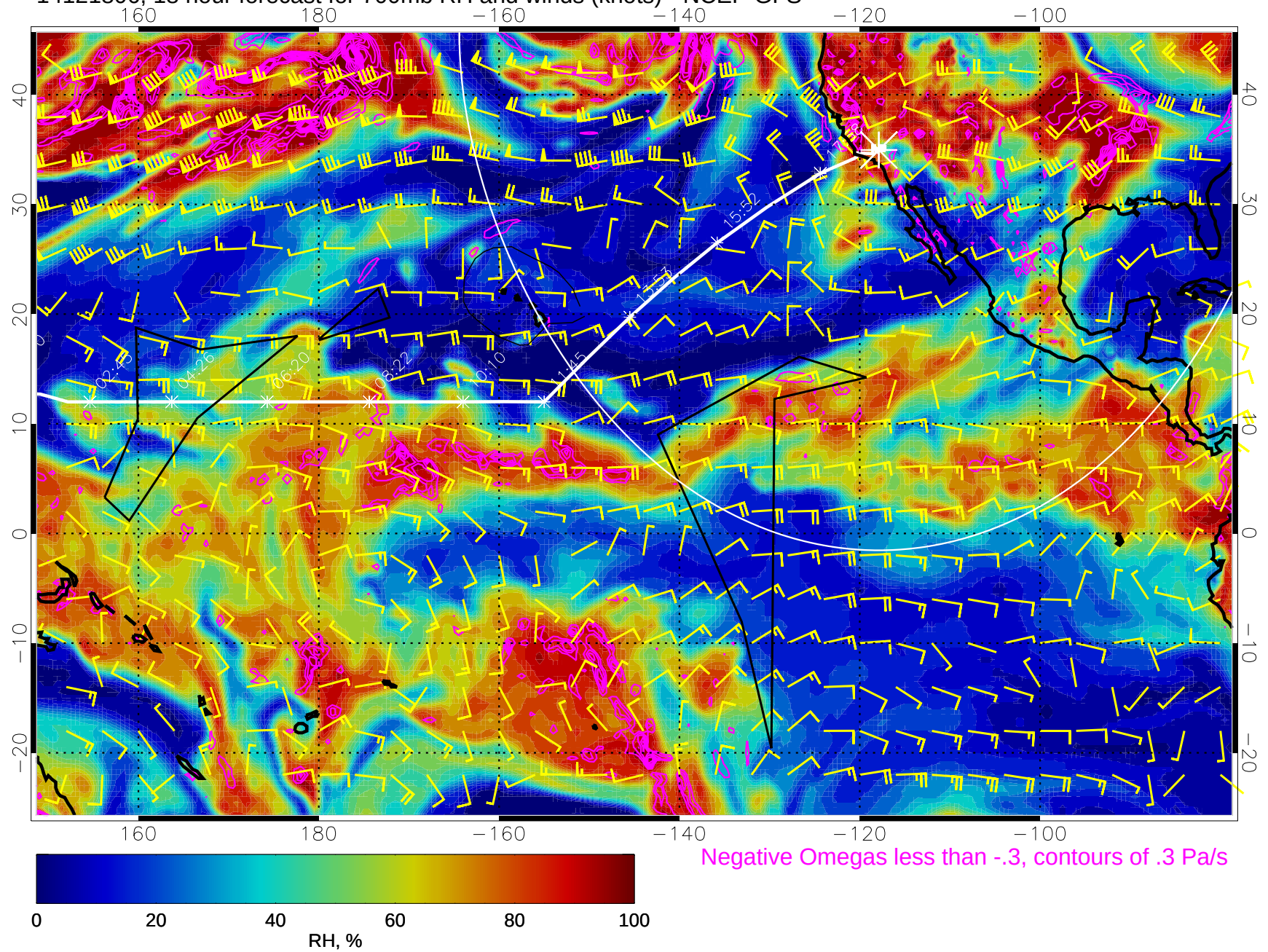
14121806, 18 hour forecast for 700mb RH and winds (knots) - NCEP GFS
