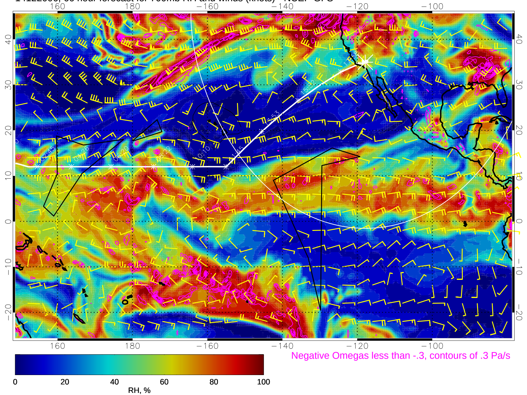
14122006, 66 hour forecast for 700mb RH and winds (knots) - NCEP GFS
