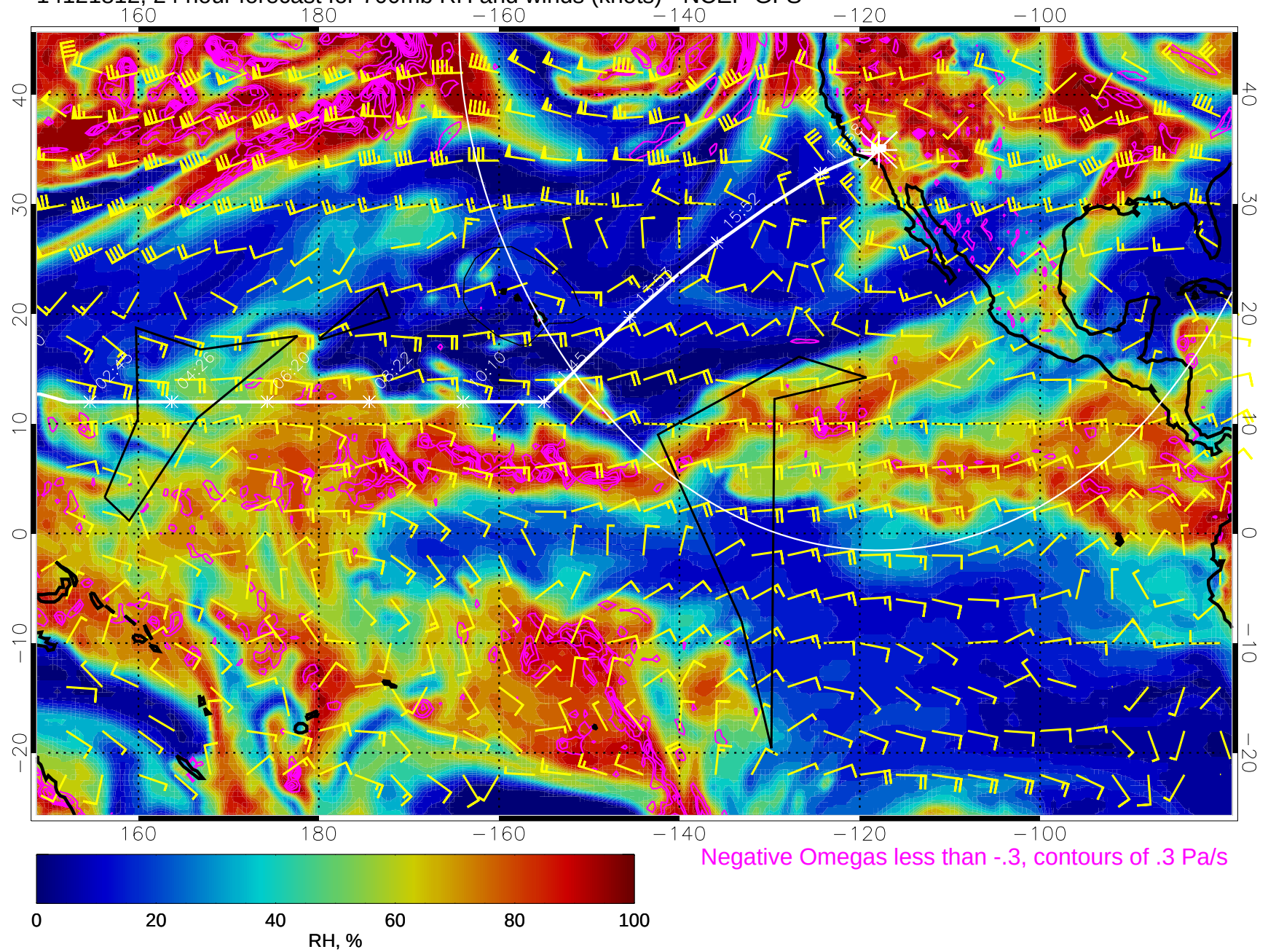
14121812, 24 hour forecast for 700mb RH and winds (knots) - NCEP GFS
