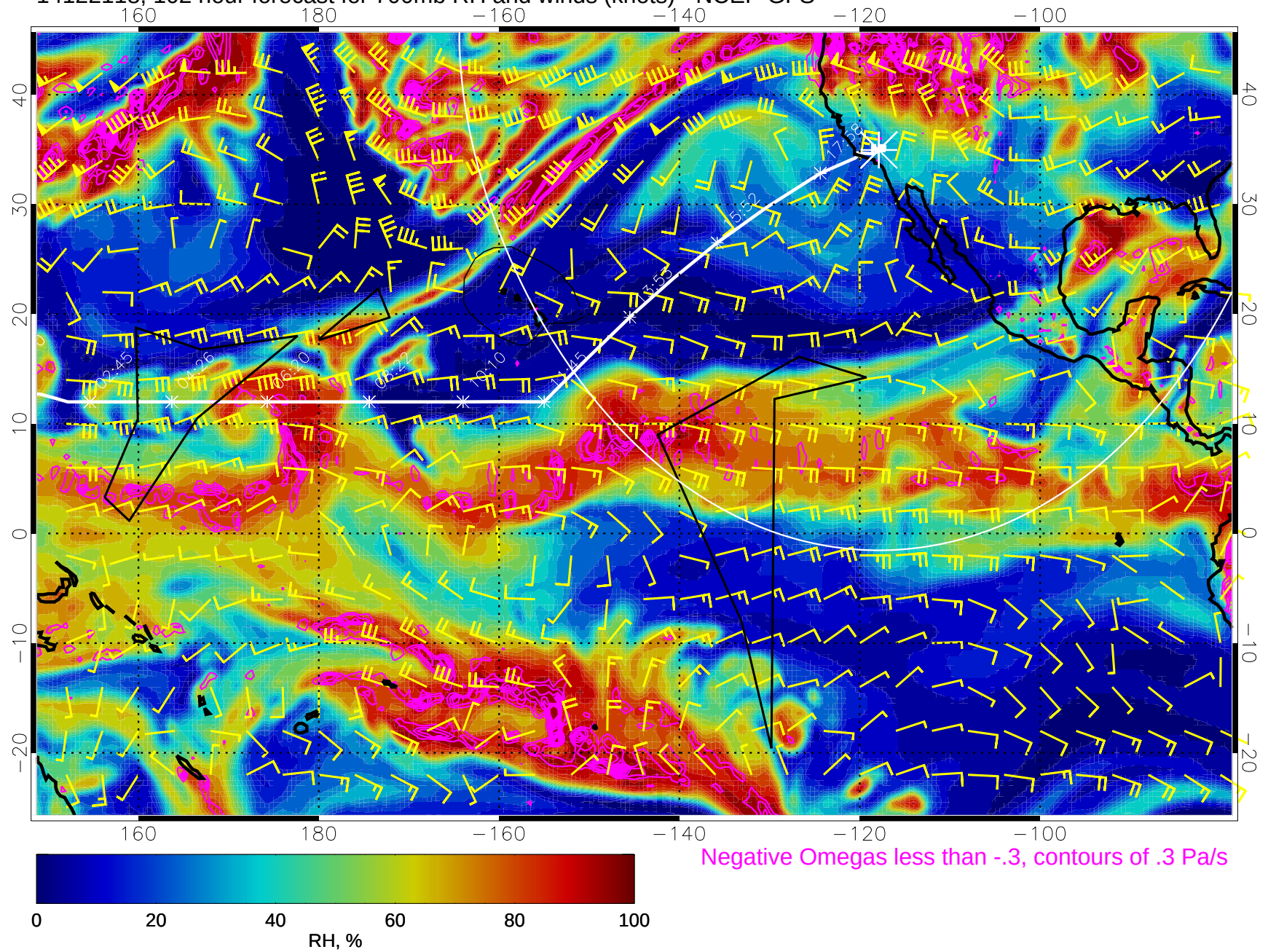
14122118, 102 hour forecast for 700mb RH and winds (knots) - NCEP GFS
