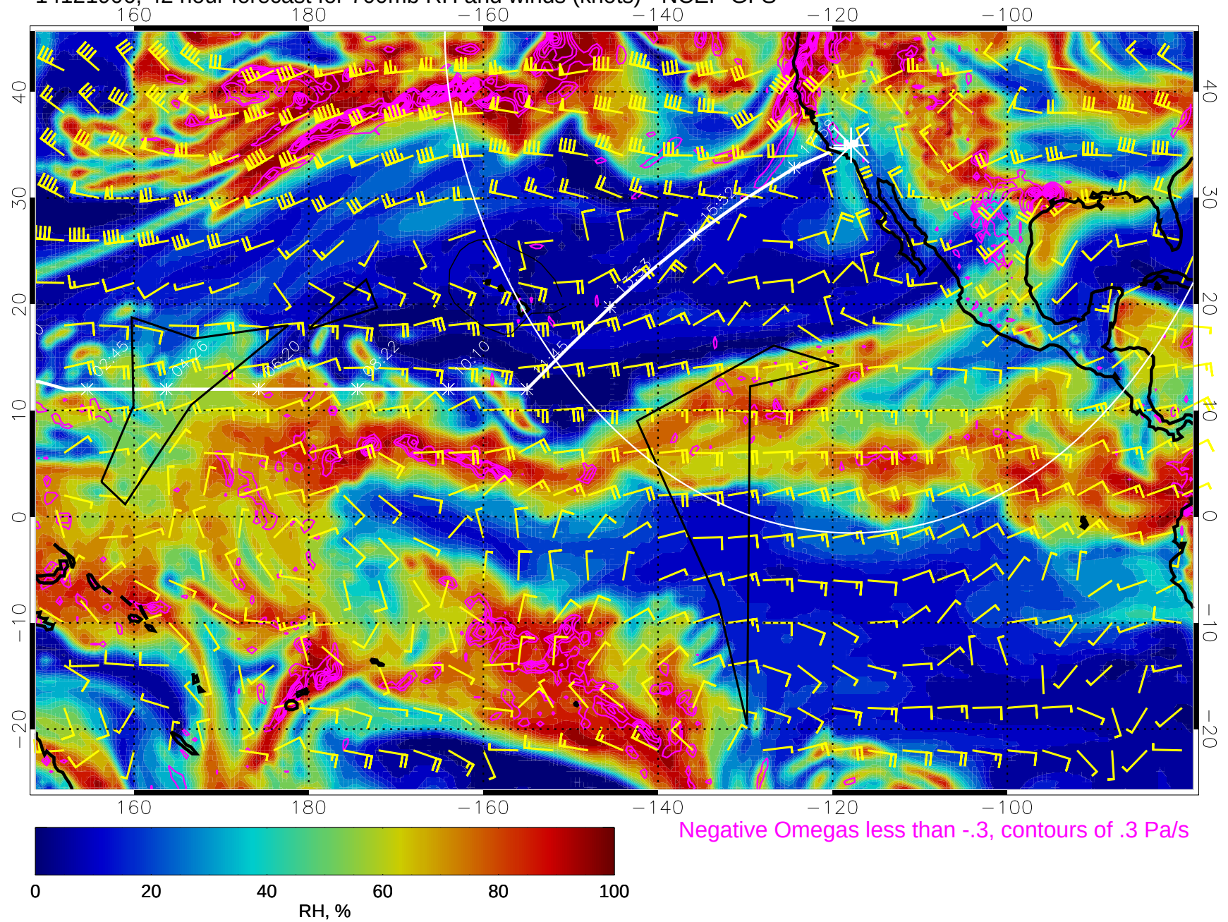
14121906, 42 hour forecast for 700mb RH and winds (knots) - NCEP GFS
