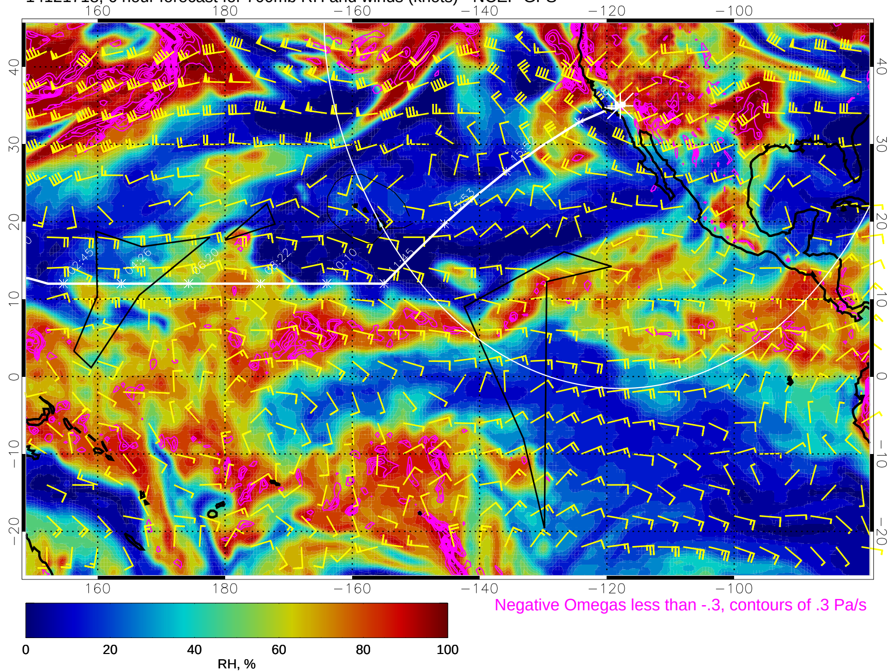
14121718, 6 hour forecast for 700mb RH and winds (knots) - NCEP GFS
