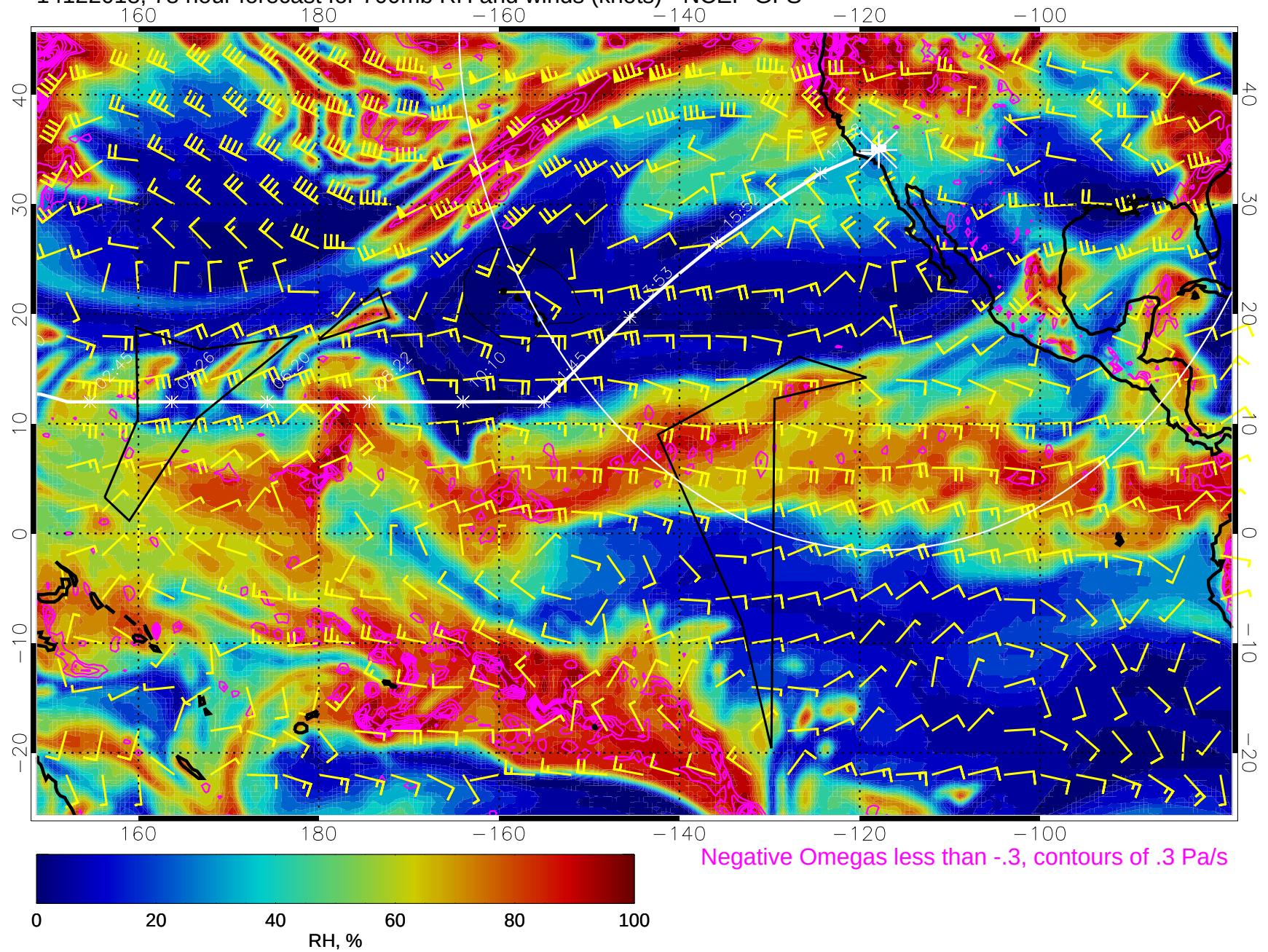
14122018, 78 hour forecast for 700mb RH and winds (knots) - NCEP GFS
