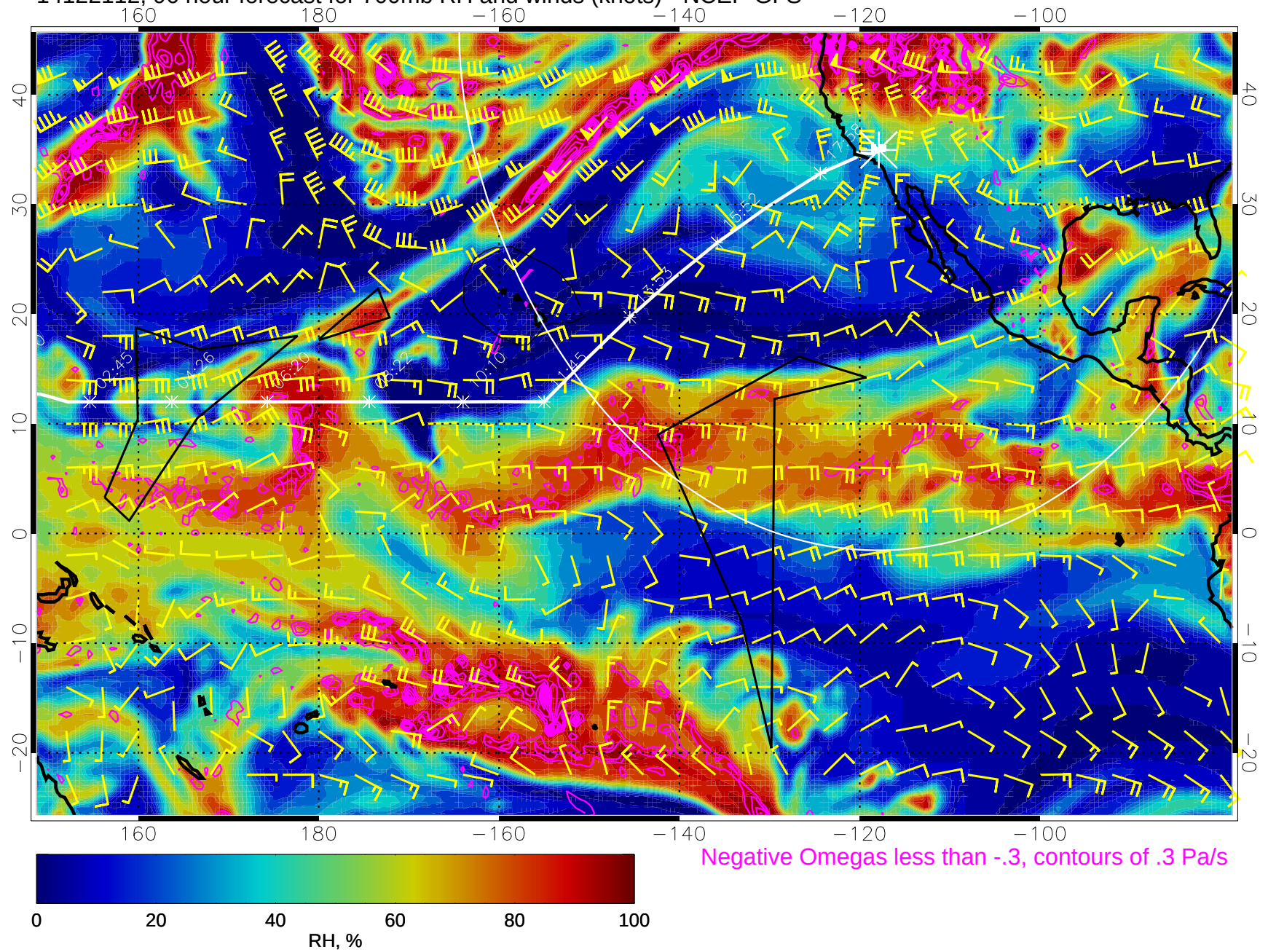
14122112, 96 hour forecast for 700mb RH and winds (knots) - NCEP GFS
