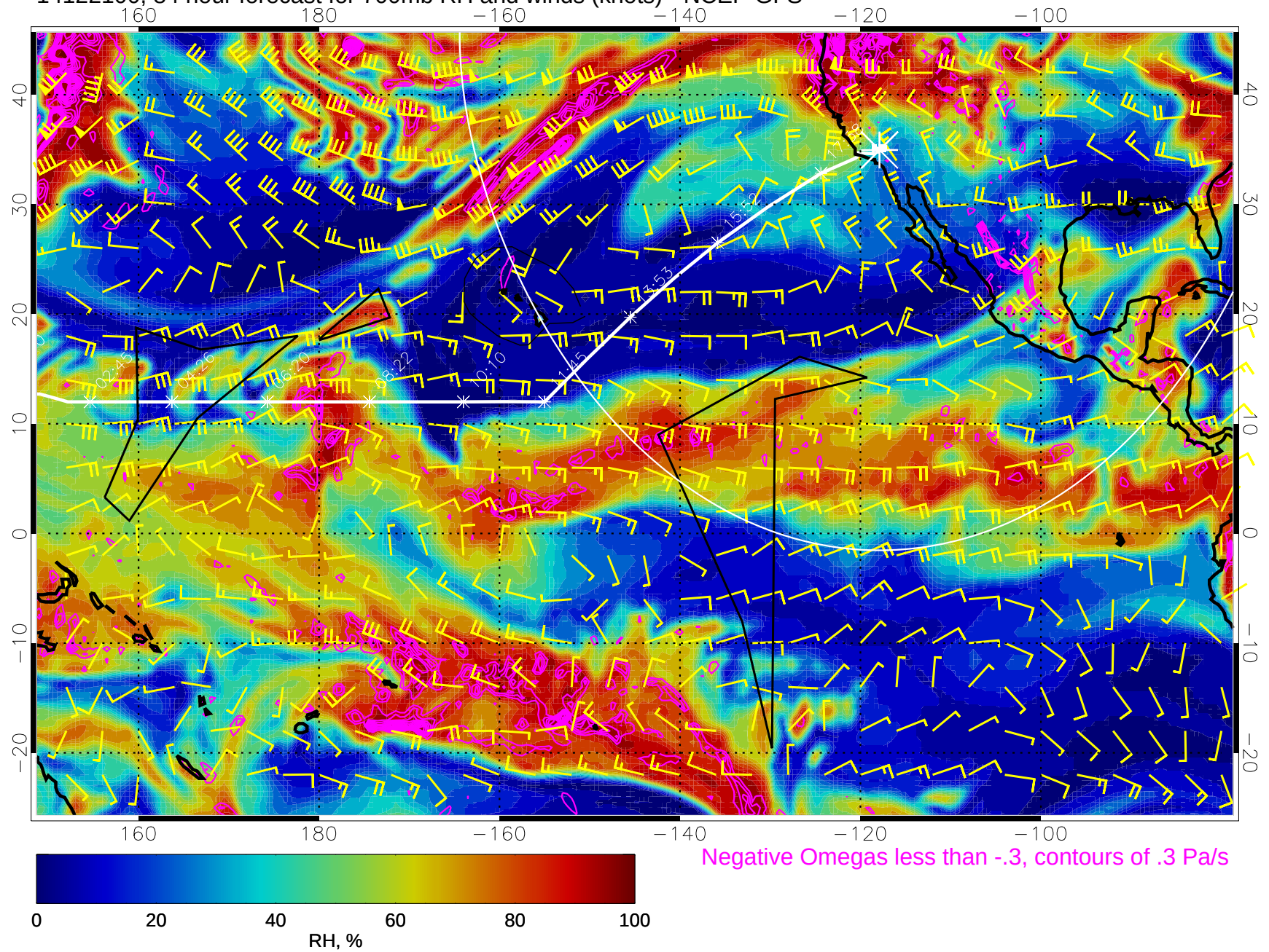
14122100, 84 hour forecast for 700mb RH and winds (knots) - NCEP GFS
