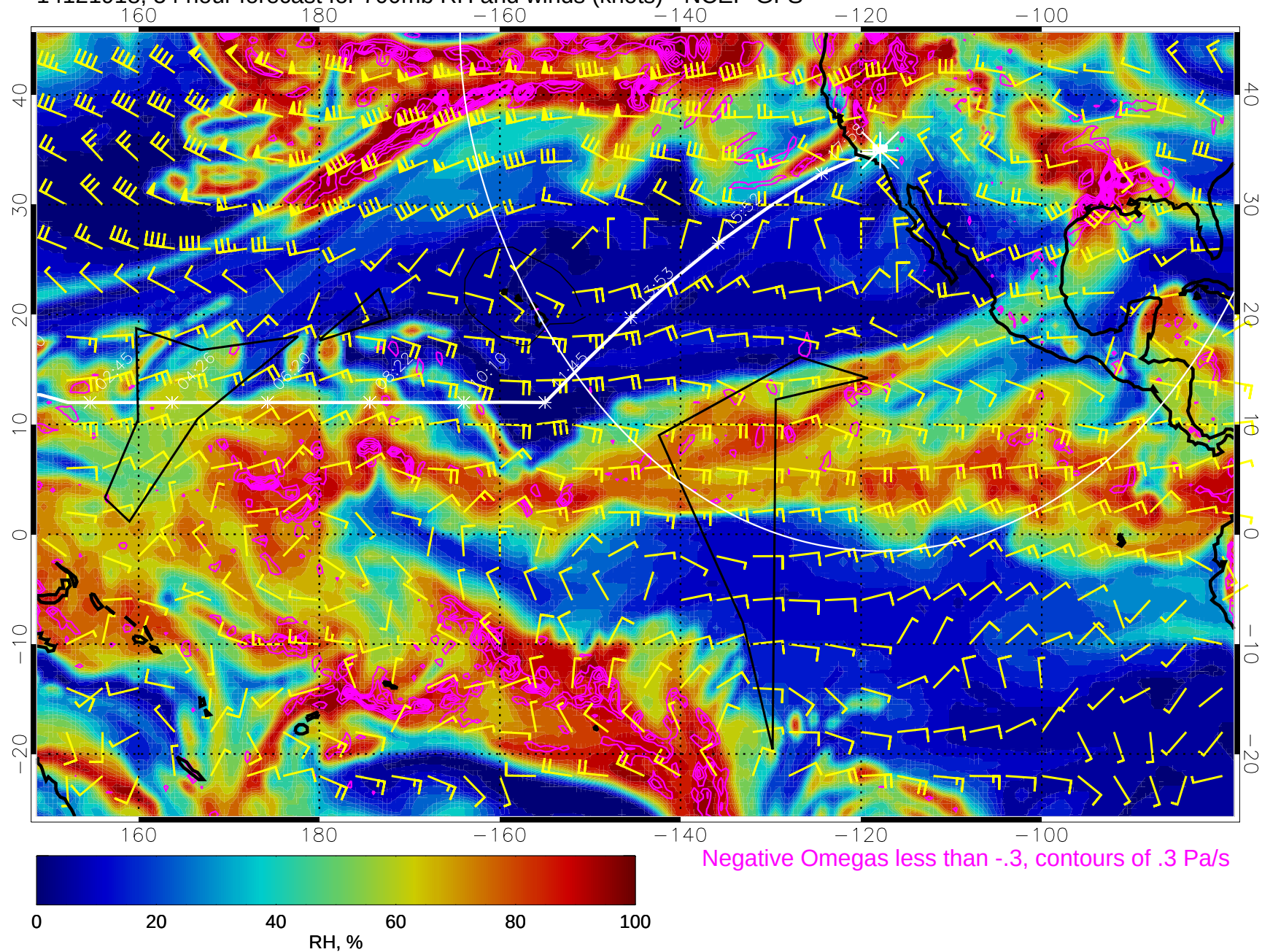
14121918, 54 hour forecast for 700mb RH and winds (knots) - NCEP GFS
