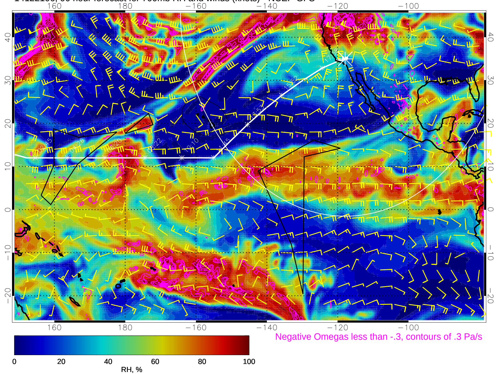
14122106, 90 hour forecast for 700mb RH and winds (knots) - NCEP GFS
