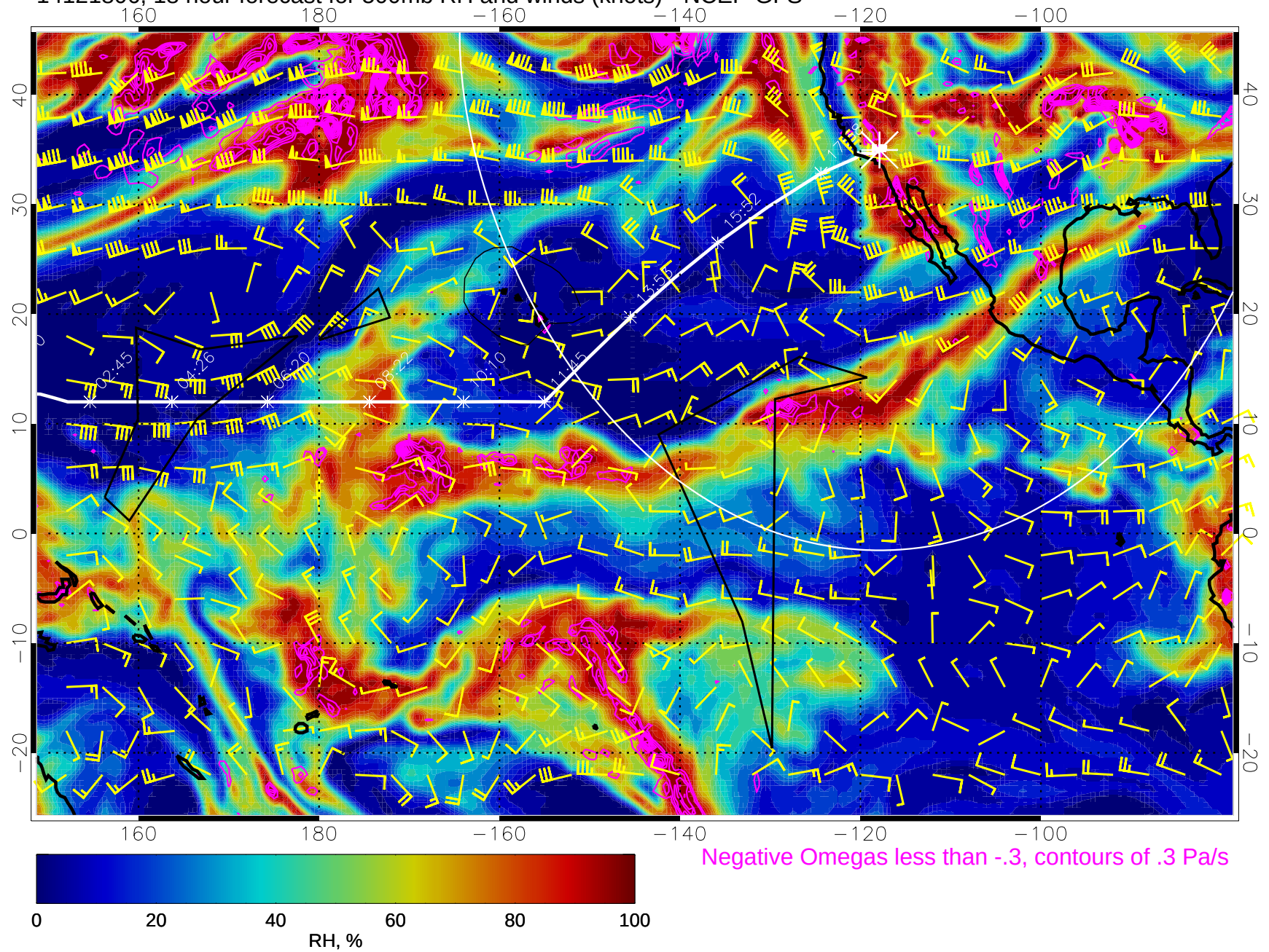
14121806, 18 hour forecast for 500mb RH and winds (knots) - NCEP GFS
