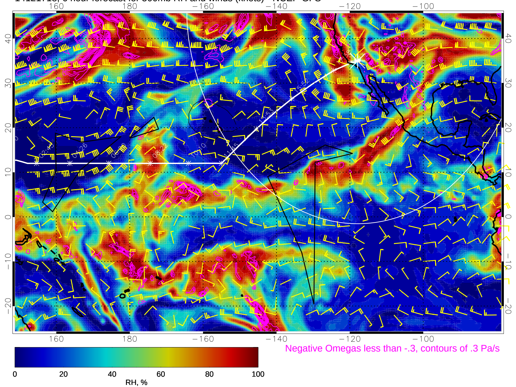
14121718, 6 hour forecast for 500mb RH and winds (knots) - NCEP GFS
