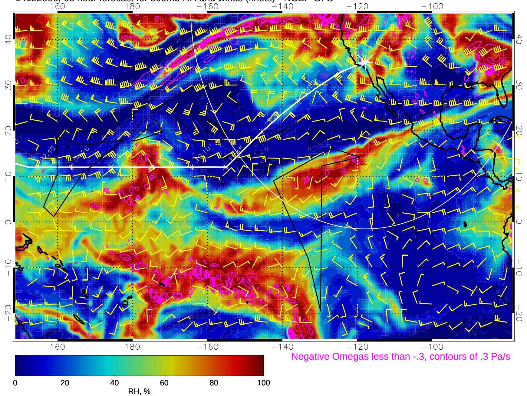
14122006, 66 hour forecast for 500mb RH and winds (knots) - NCEP GFS
