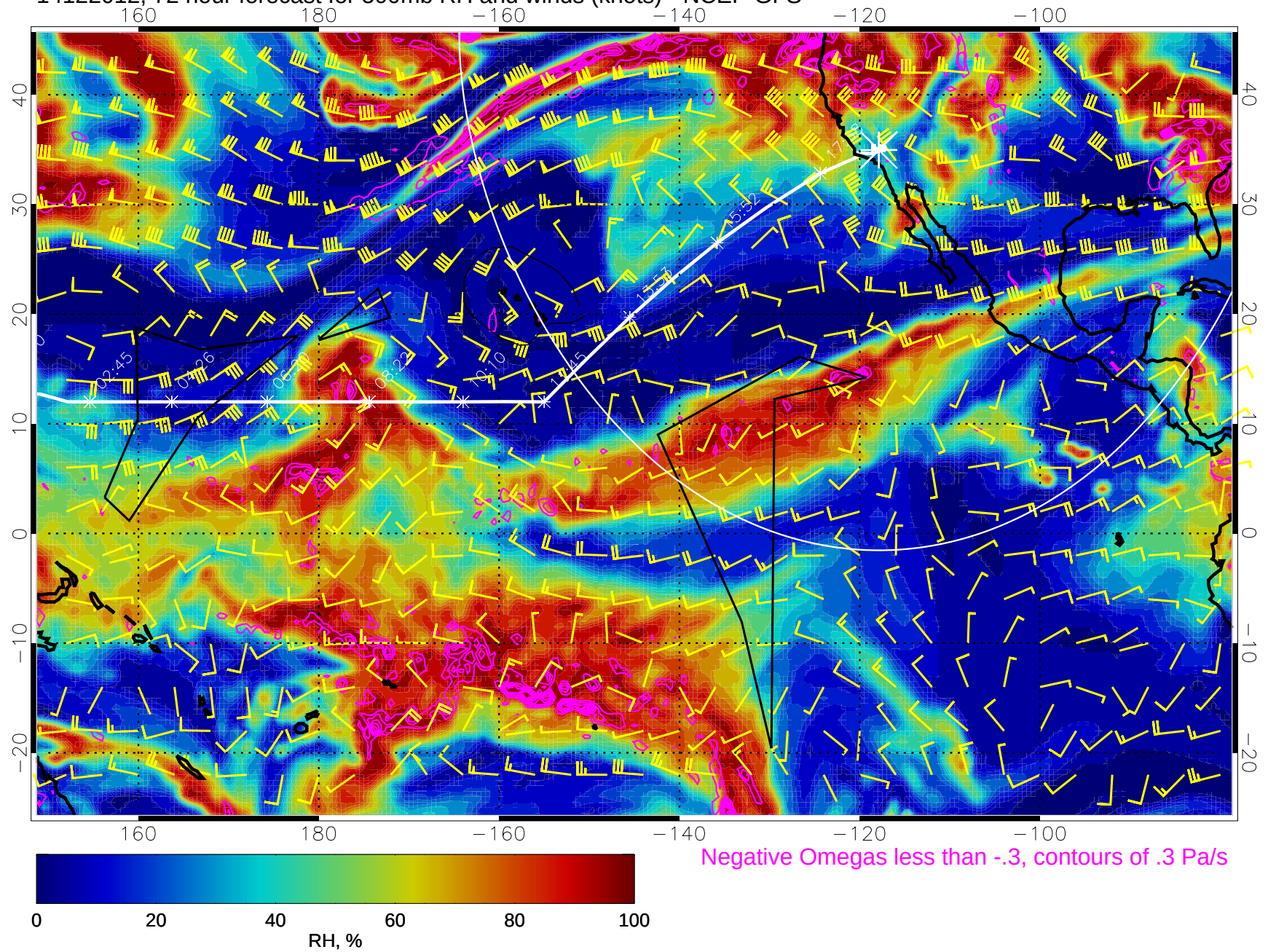
14122012, 72 hour forecast for 500mb RH and winds (knots) - NCEP GFS
