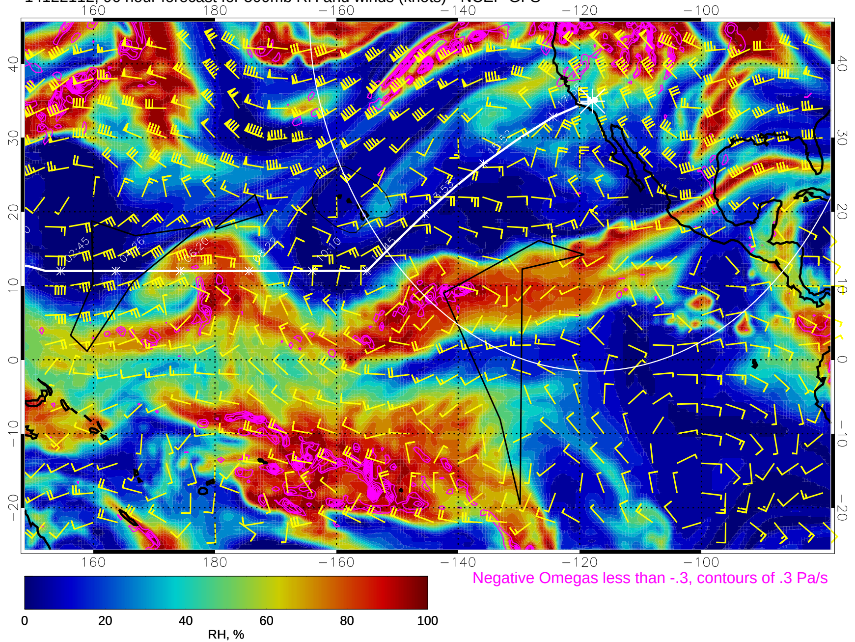
14122112, 96 hour forecast for 500mb RH and winds (knots) - NCEP GFS
