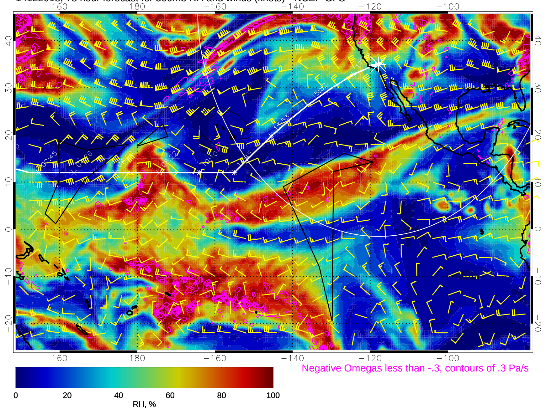
14122018, 78 hour forecast for 500mb RH and winds (knots) - NCEP GFS
