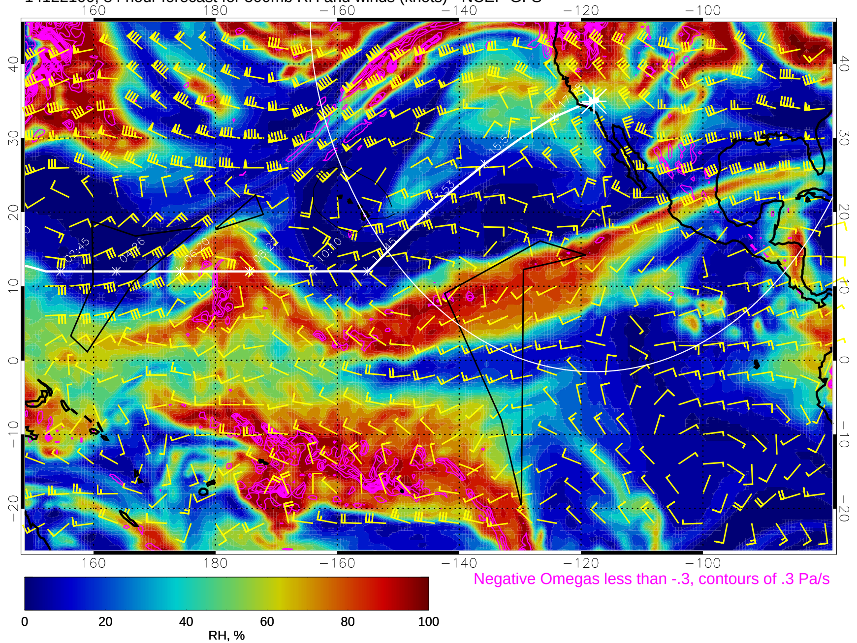
14122100, 84 hour forecast for 500mb RH and winds (knots) - NCEP GFS
