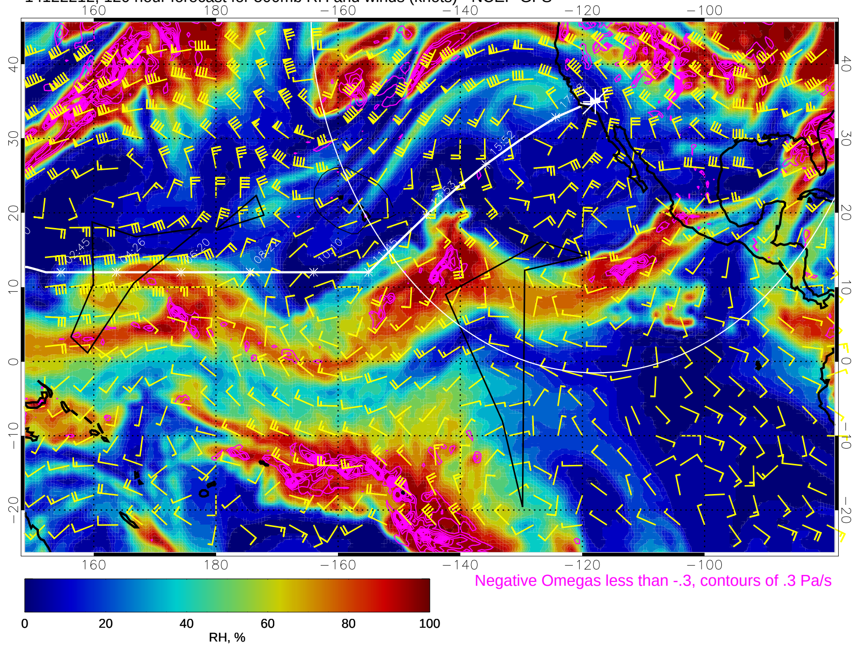
14122212, 120 hour forecast for 500mb RH and winds (knots) - NCEP GFS
