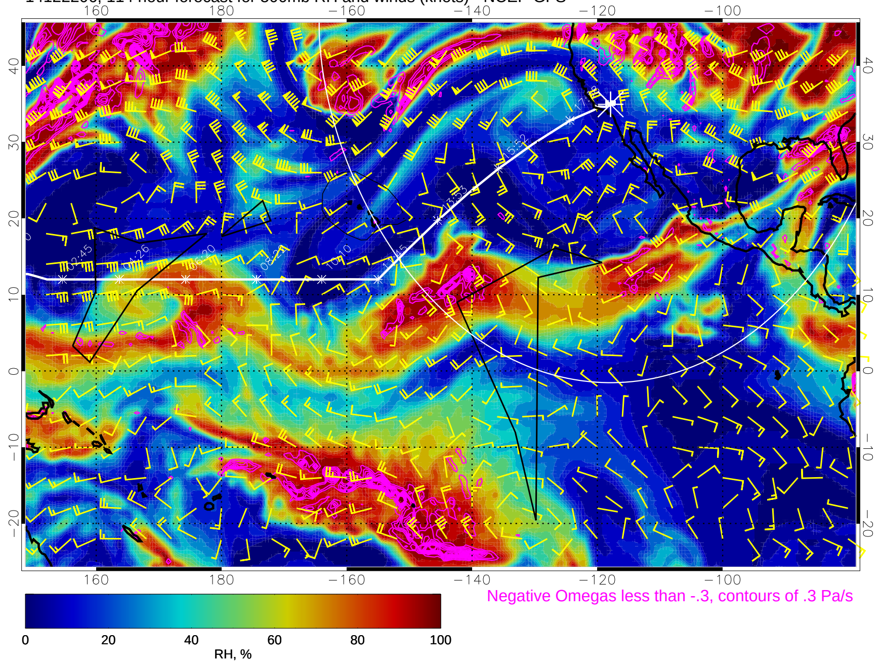
14122206, 114 hour forecast for 500mb RH and winds (knots) - NCEP GFS
