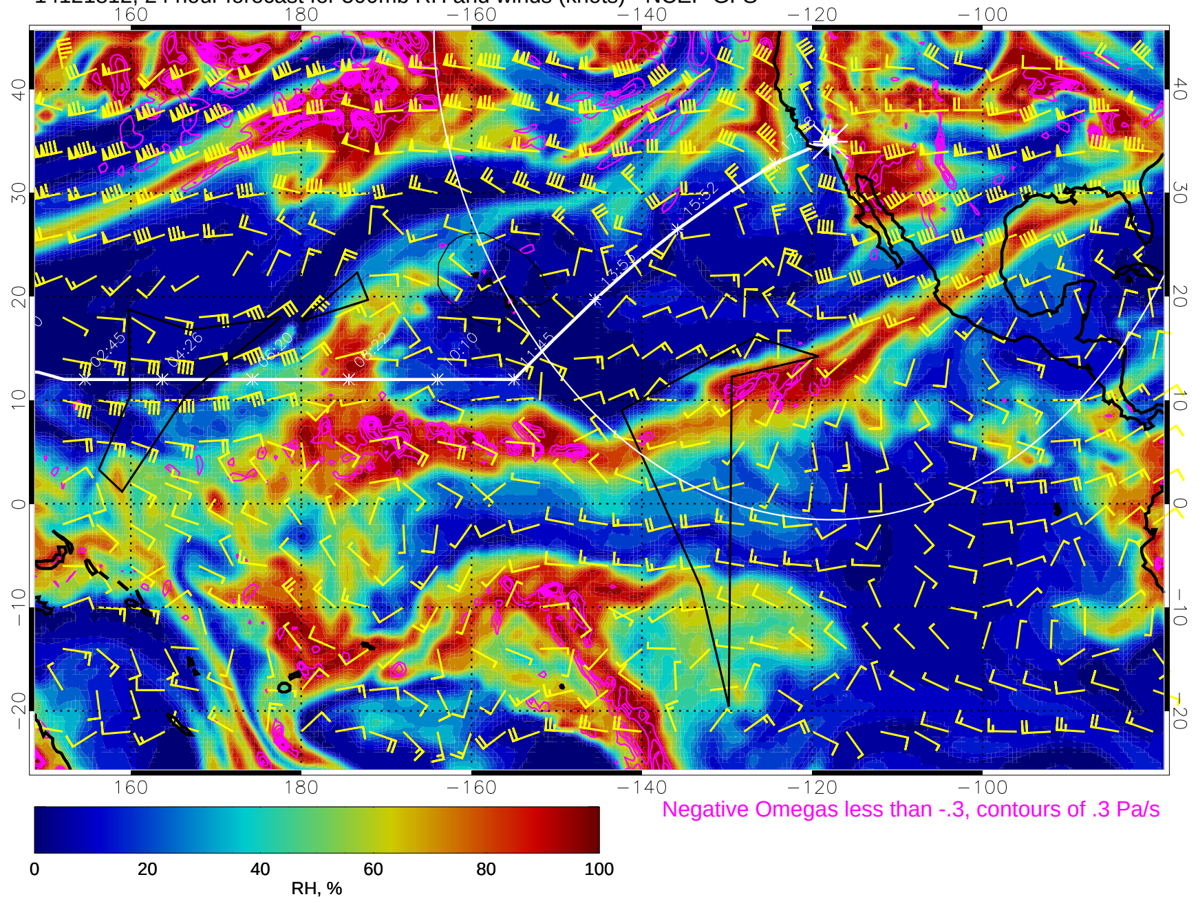
14121812, 24 hour forecast for 500mb RH and winds (knots) - NCEP GFS
