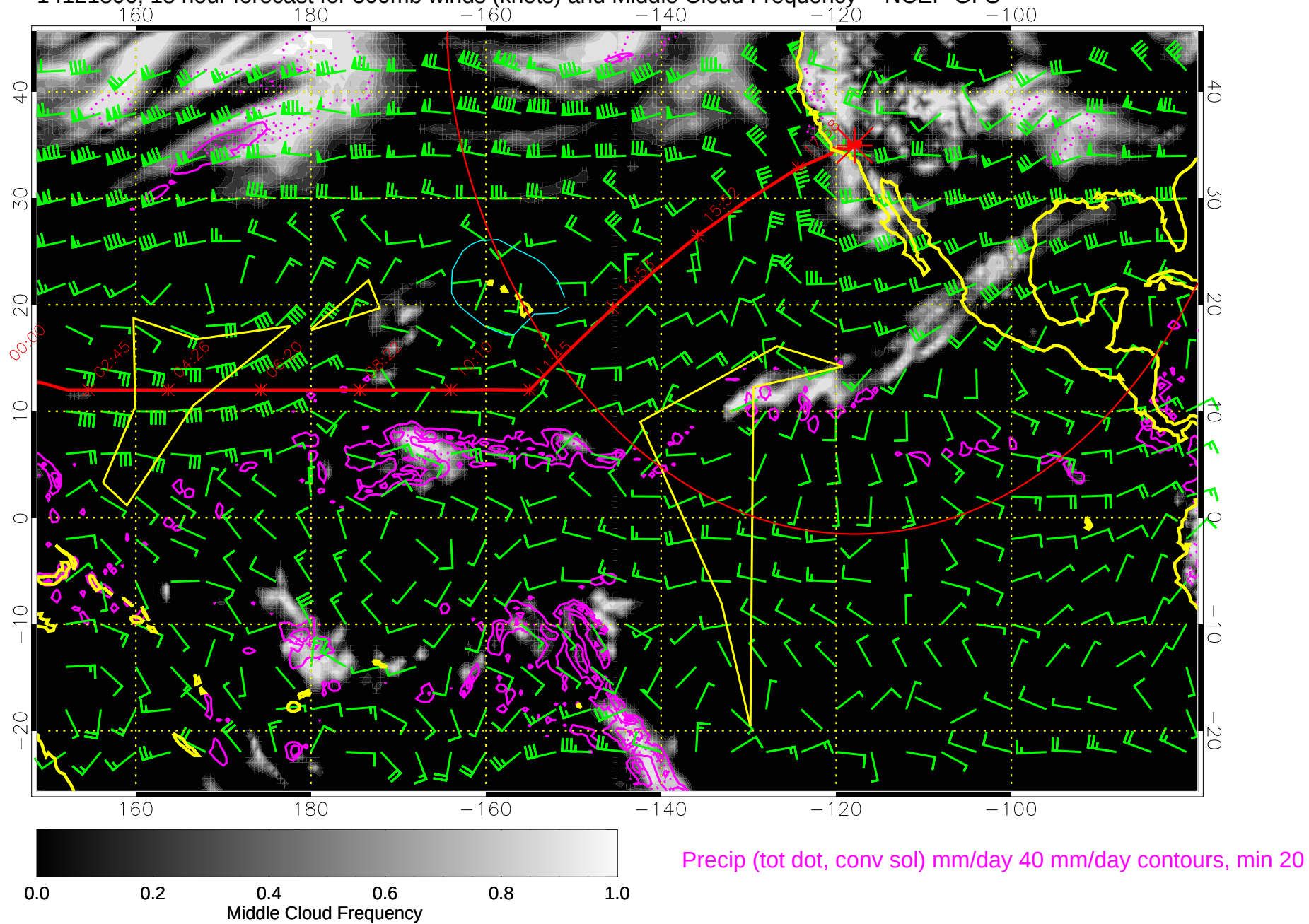
14121806, 18 hour forecast for 500mb winds (knots) and Middle Cloud Frequency -- NCEP GFS
