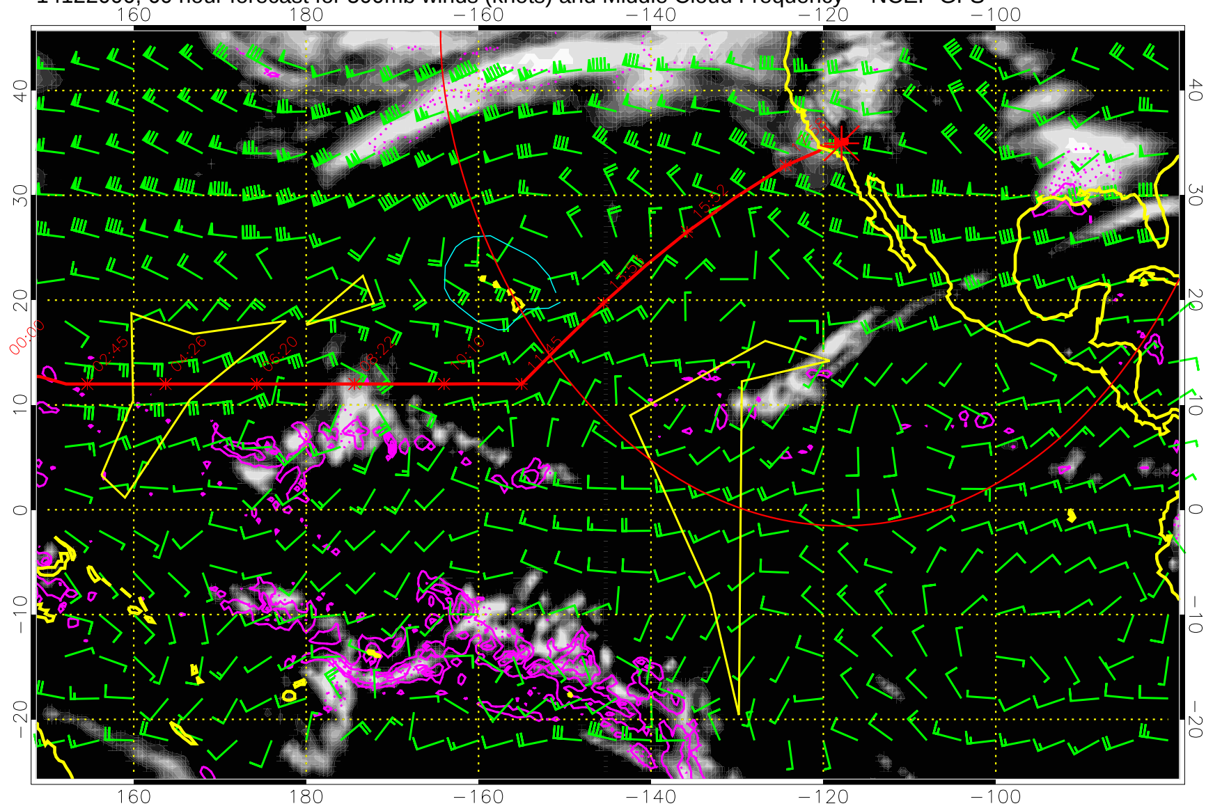
14122000, 60 hour forecast for 500mb winds (knots) and Middle Cloud Frequency -- NCEP GFS
