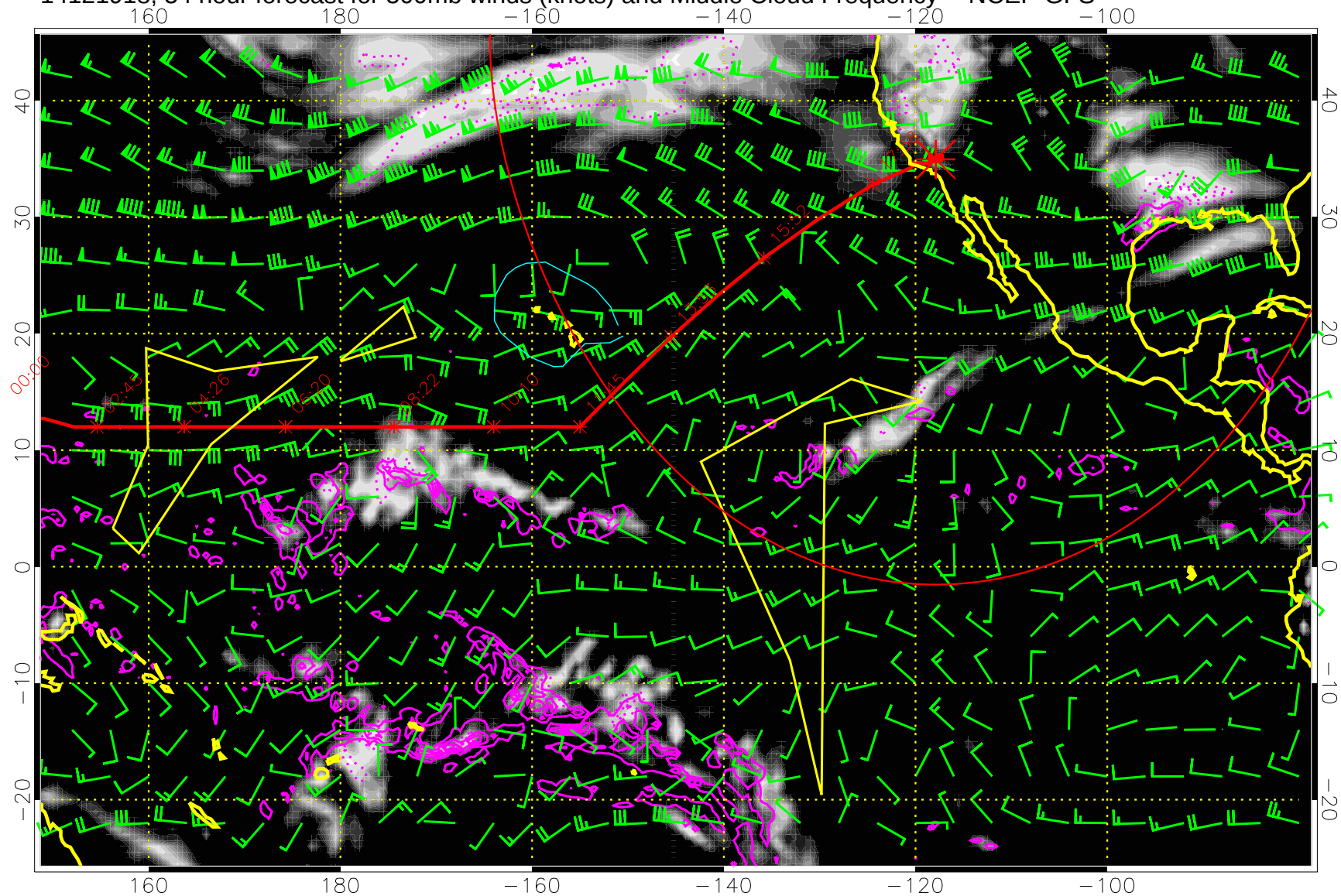
14121918, 54 hour forecast for 500mb winds (knots) and Middle Cloud Frequency -- NCEP GFS
