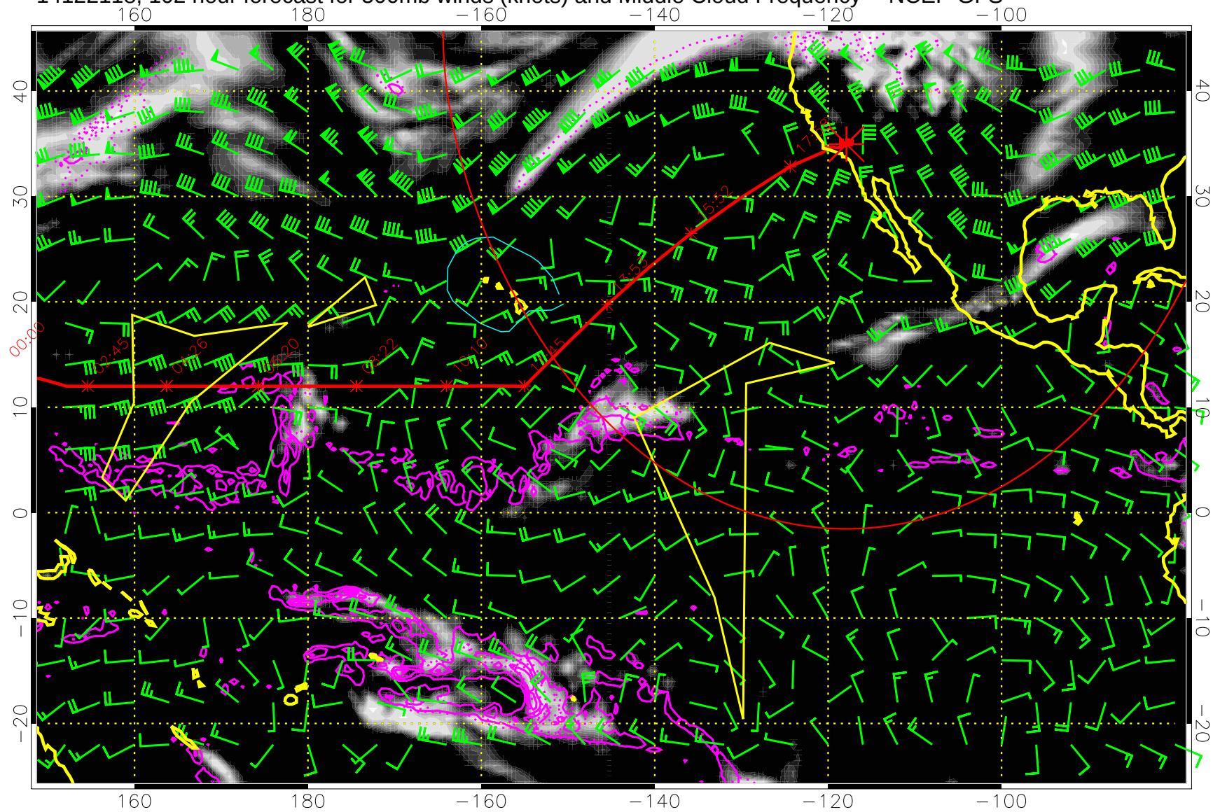
14122118, 102 hour forecast for 500mb winds (knots) and Middle Cloud Frequency -- NCEP GFS
