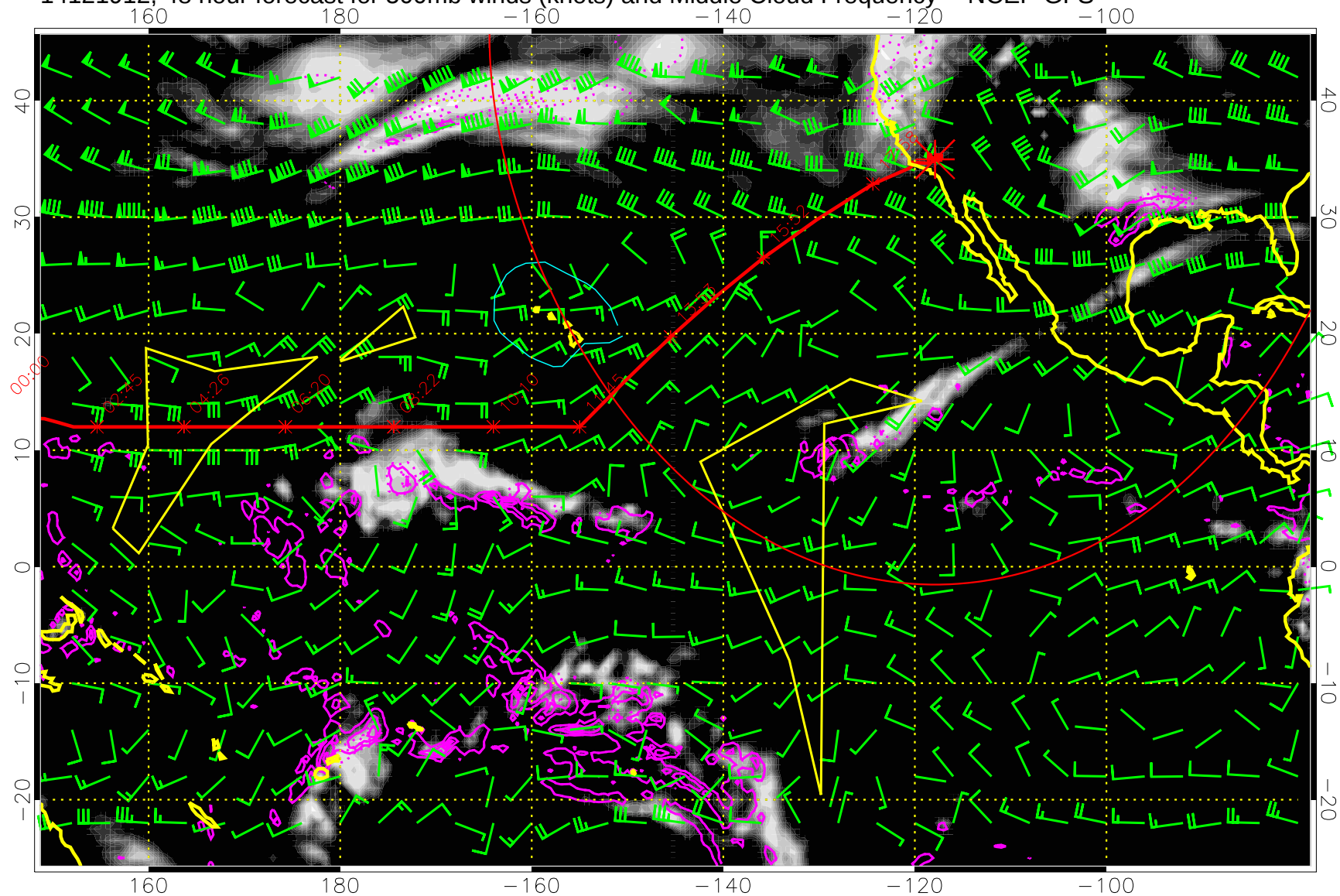
14121912, 48 hour forecast for 500mb winds (knots) and Middle Cloud Frequency -- NCEP GFS
