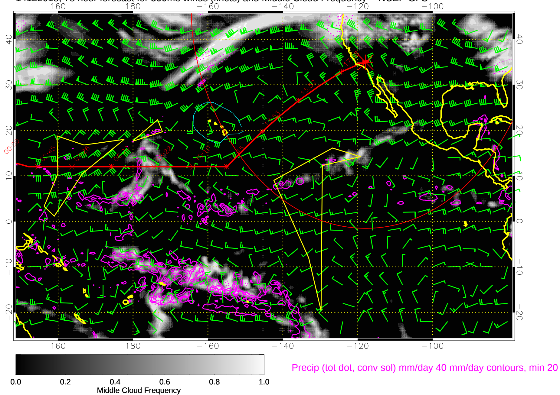
14122018, 78 hour forecast for 500mb winds (knots) and Middle Cloud Frequency -- NCEP GFS
