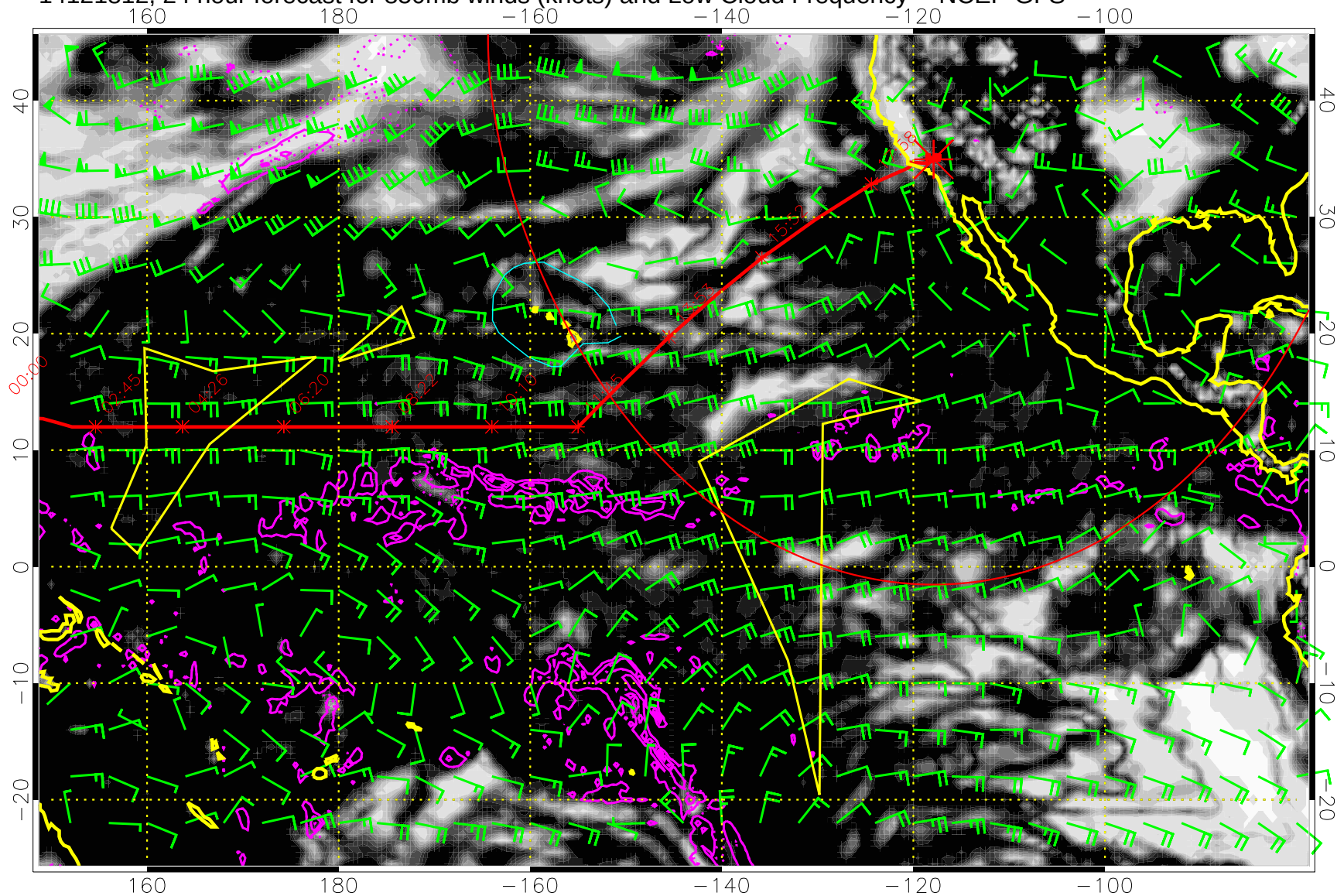
14121812, 24 hour forecast for 850mb winds (knots) and Low Cloud Frequency -- NCEP GFS
