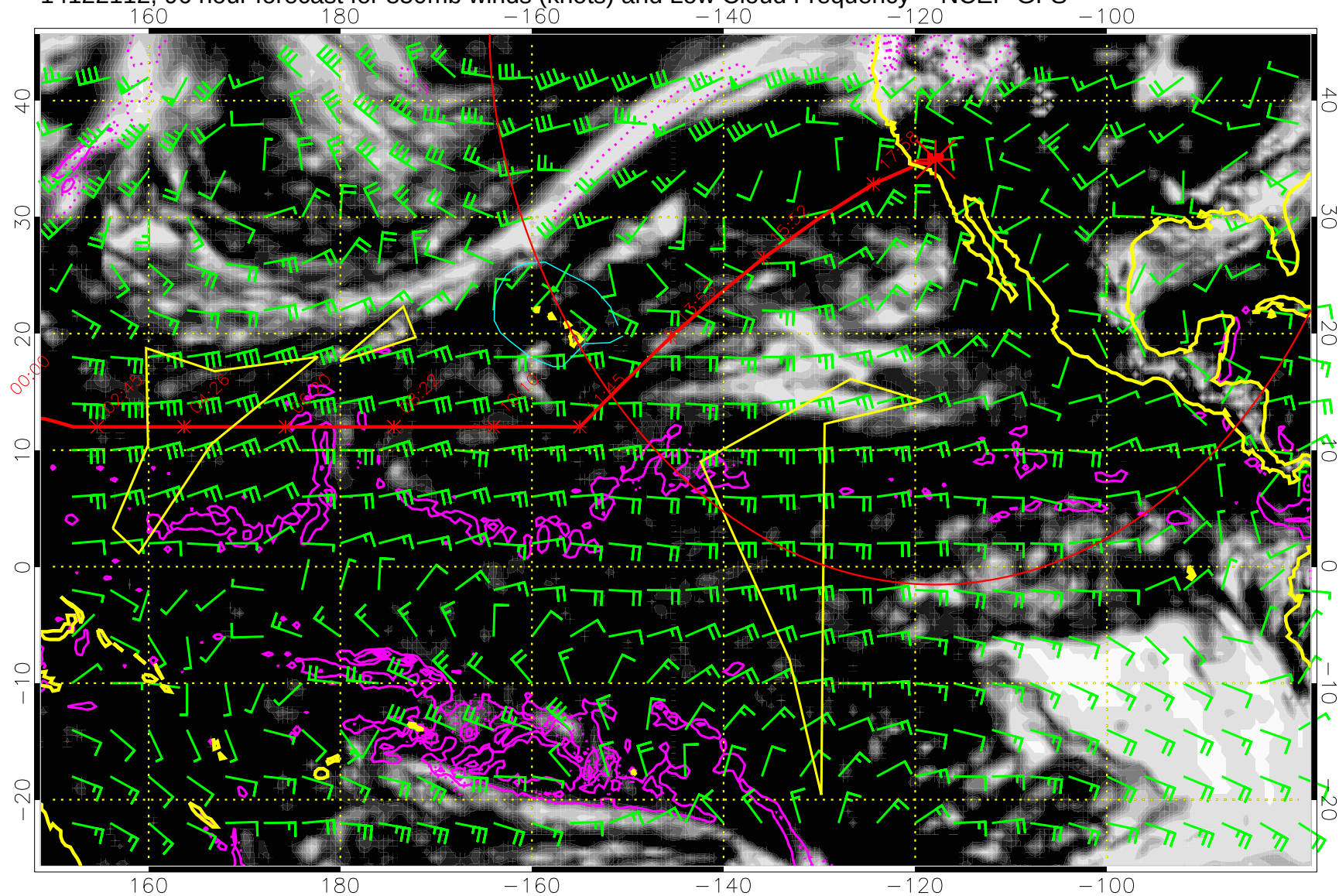
14122112, 96 hour forecast for 850mb winds (knots) and Low Cloud Frequency -- NCEP GFS
