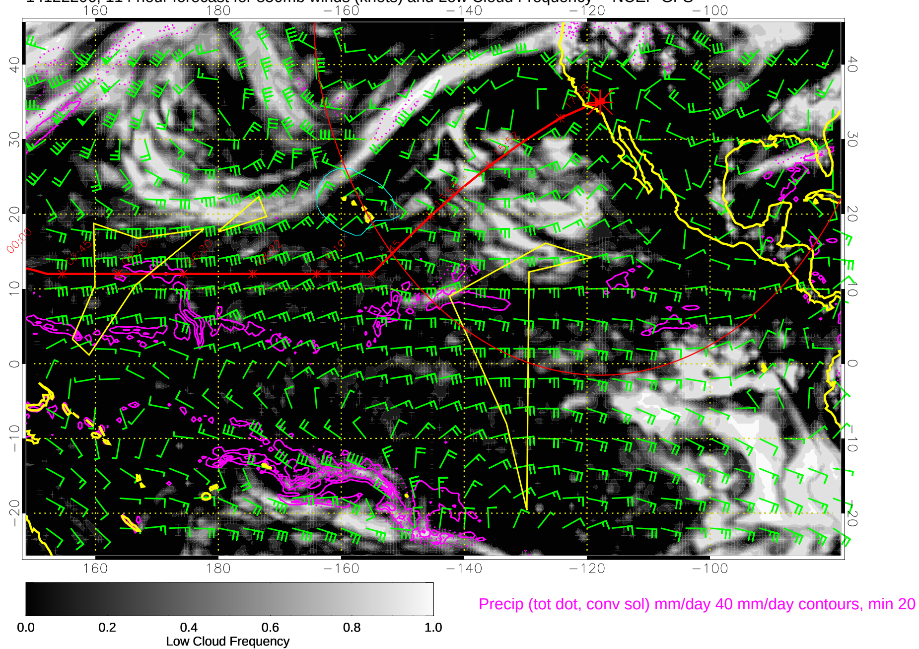
14122206, 114 hour forecast for 850mb winds (knots) and Low Cloud Frequency -- NCEP GFS
