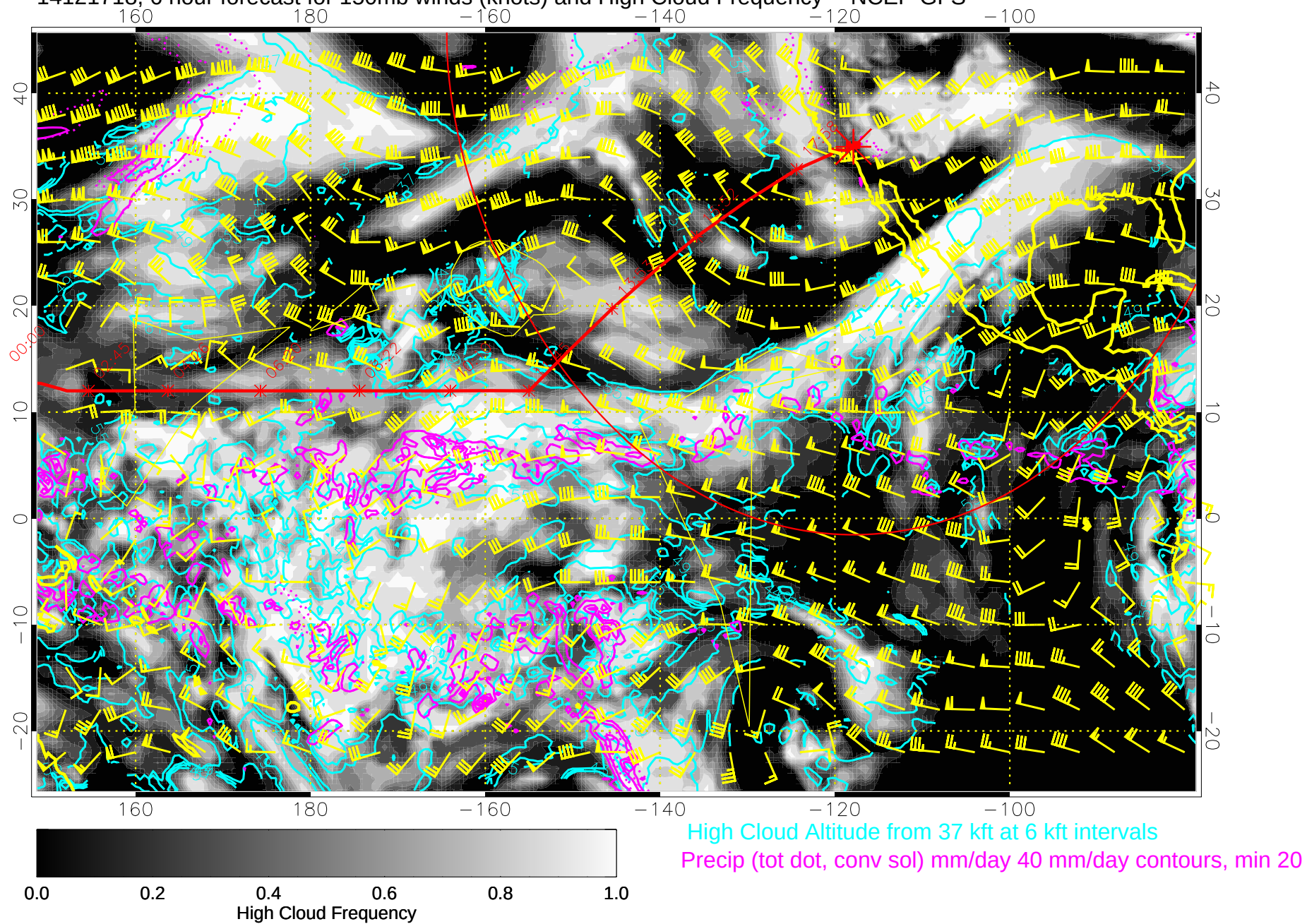
14121718, 6 hour forecast for 150mb winds (knots) and High Cloud Frequency -- NCEP GFS
