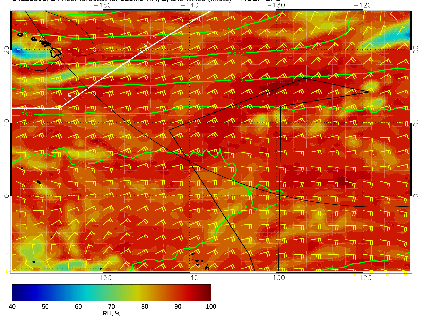
14121800, 24 hour forecast for 925mb RH, Z, and winds (knots) -- NCEP GFS
