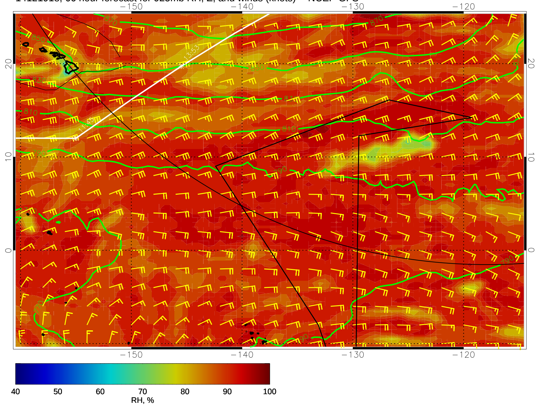
14121918, 66 hour forecast for 925mb RH, Z, and winds (knots) -- NCEP GFS
