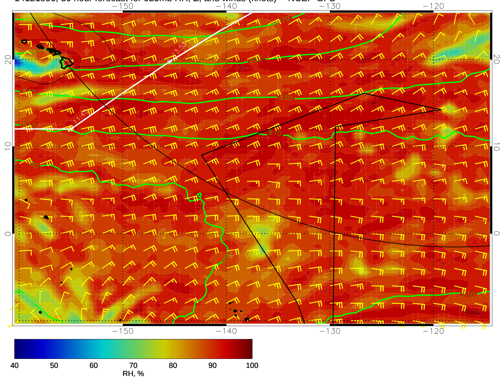
14121806, 30 hour forecast for 925mb RH, Z, and winds (knots) -- NCEP GFS
