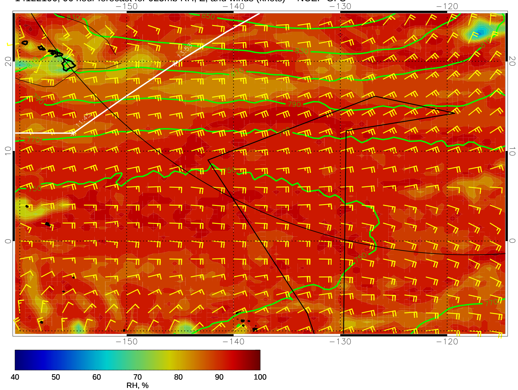
14122100, 96 hour forecast for 925mb RH, Z, and winds (knots) -- NCEP GFS
