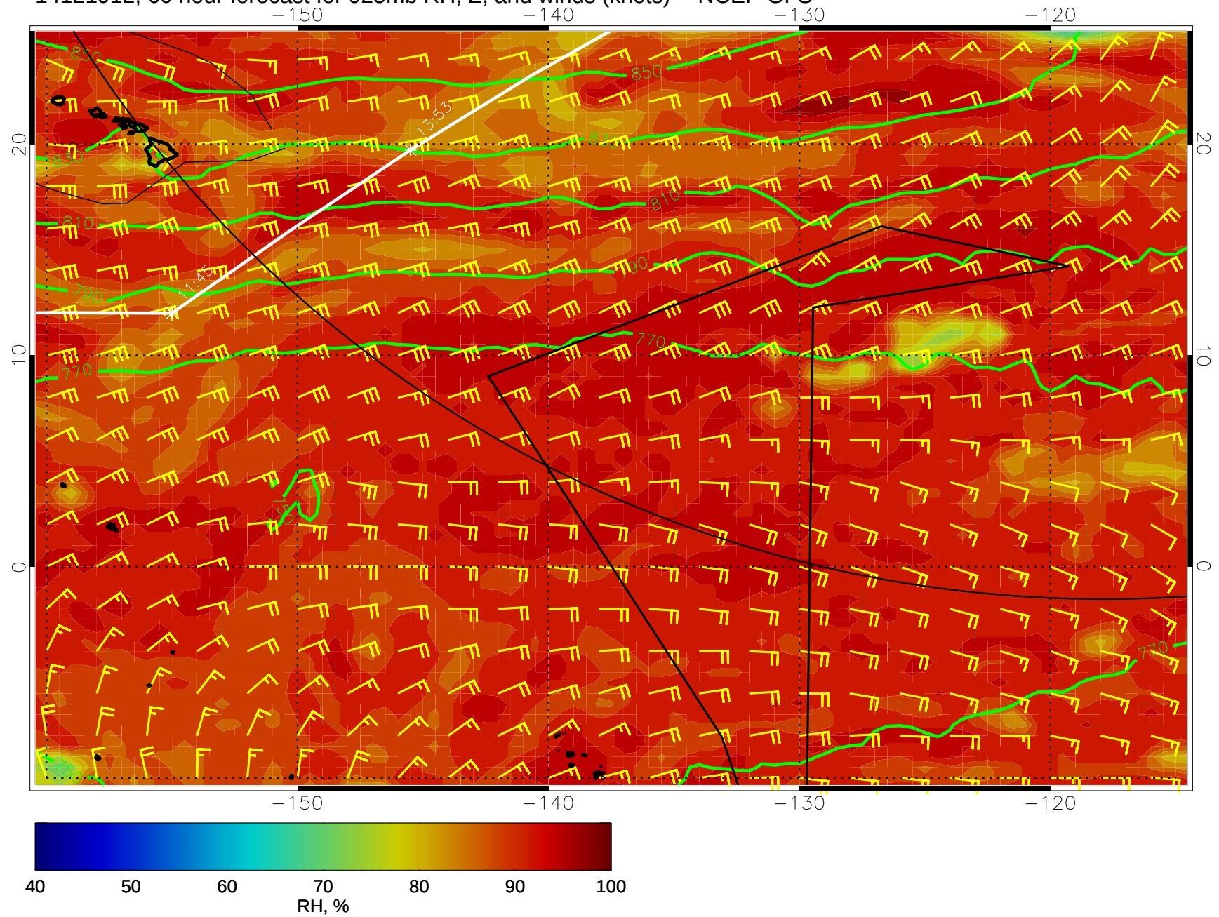
14121912, 60 hour forecast for 925mb RH, Z, and winds (knots) -- NCEP GFS
