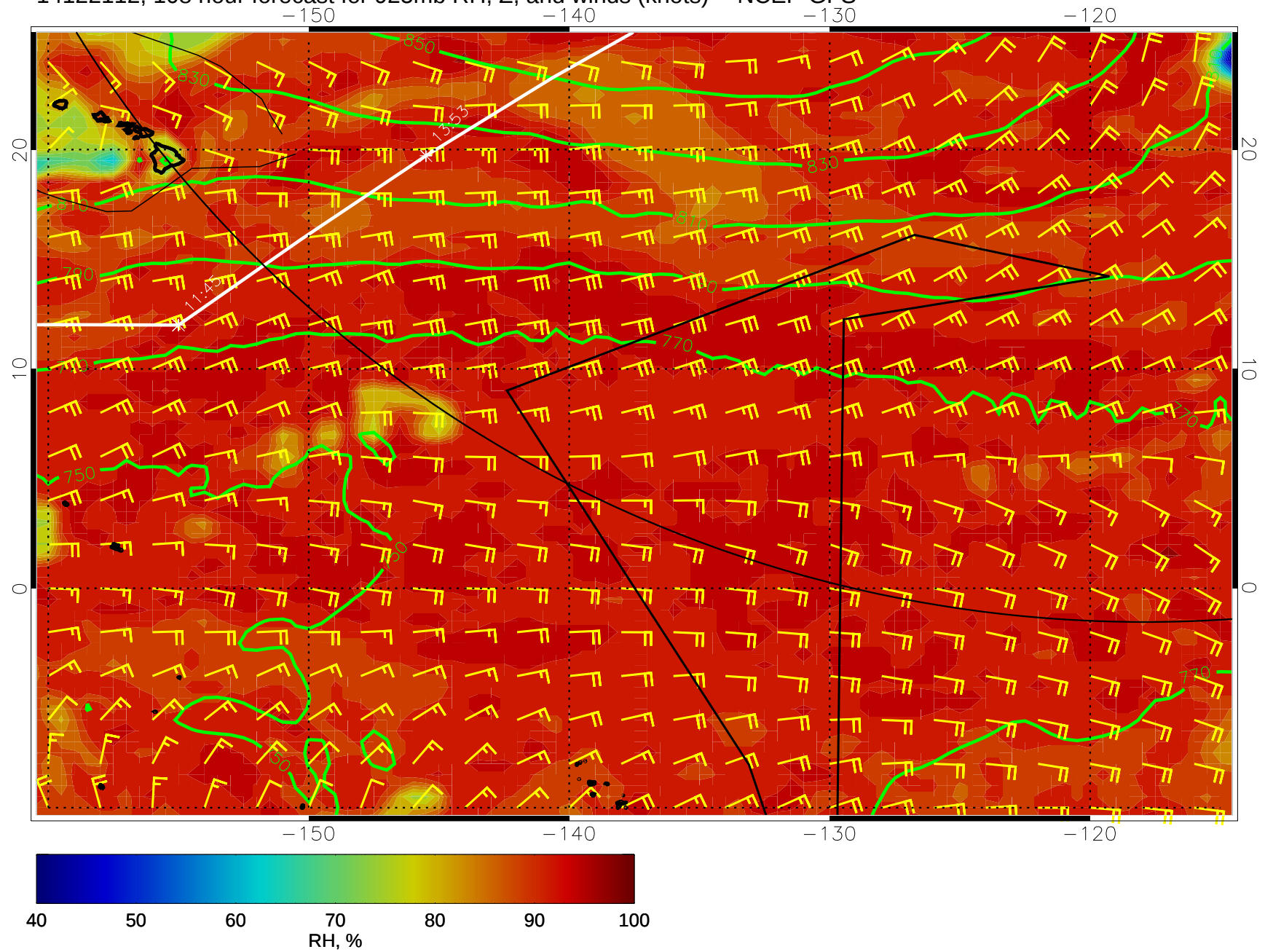
14122112, 108 hour forecast for 925mb RH, Z, and winds (knots) -- NCEP GFS
