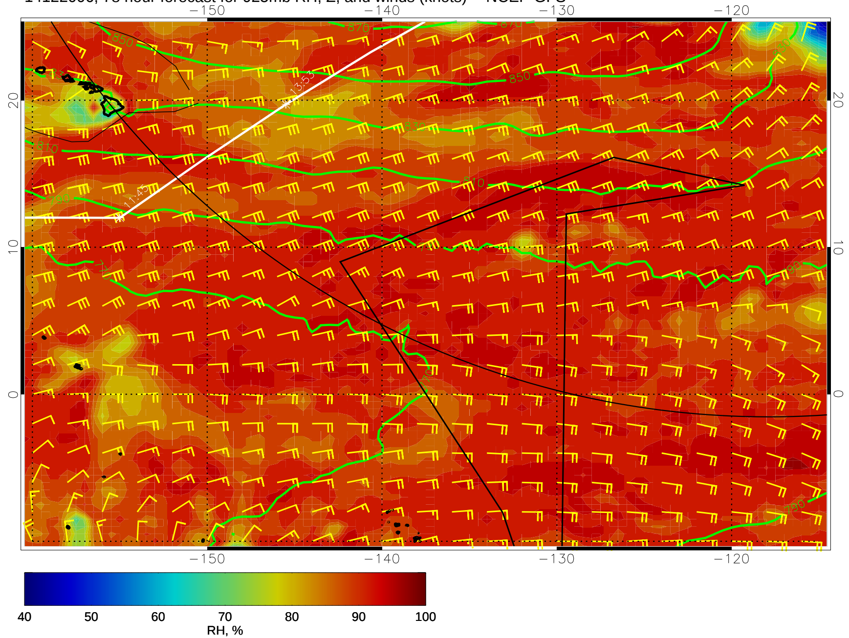
14122006, 78 hour forecast for 925mb RH, Z, and winds (knots) -- NCEP GFS
