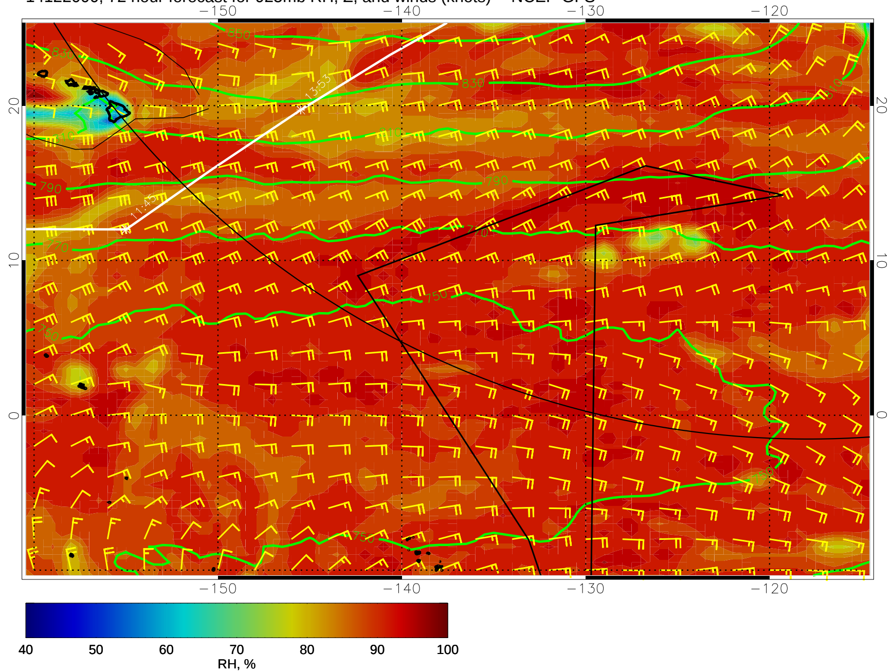
14122000, 72 hour forecast for 925mb RH, Z, and winds (knots) -- NCEP GFS
