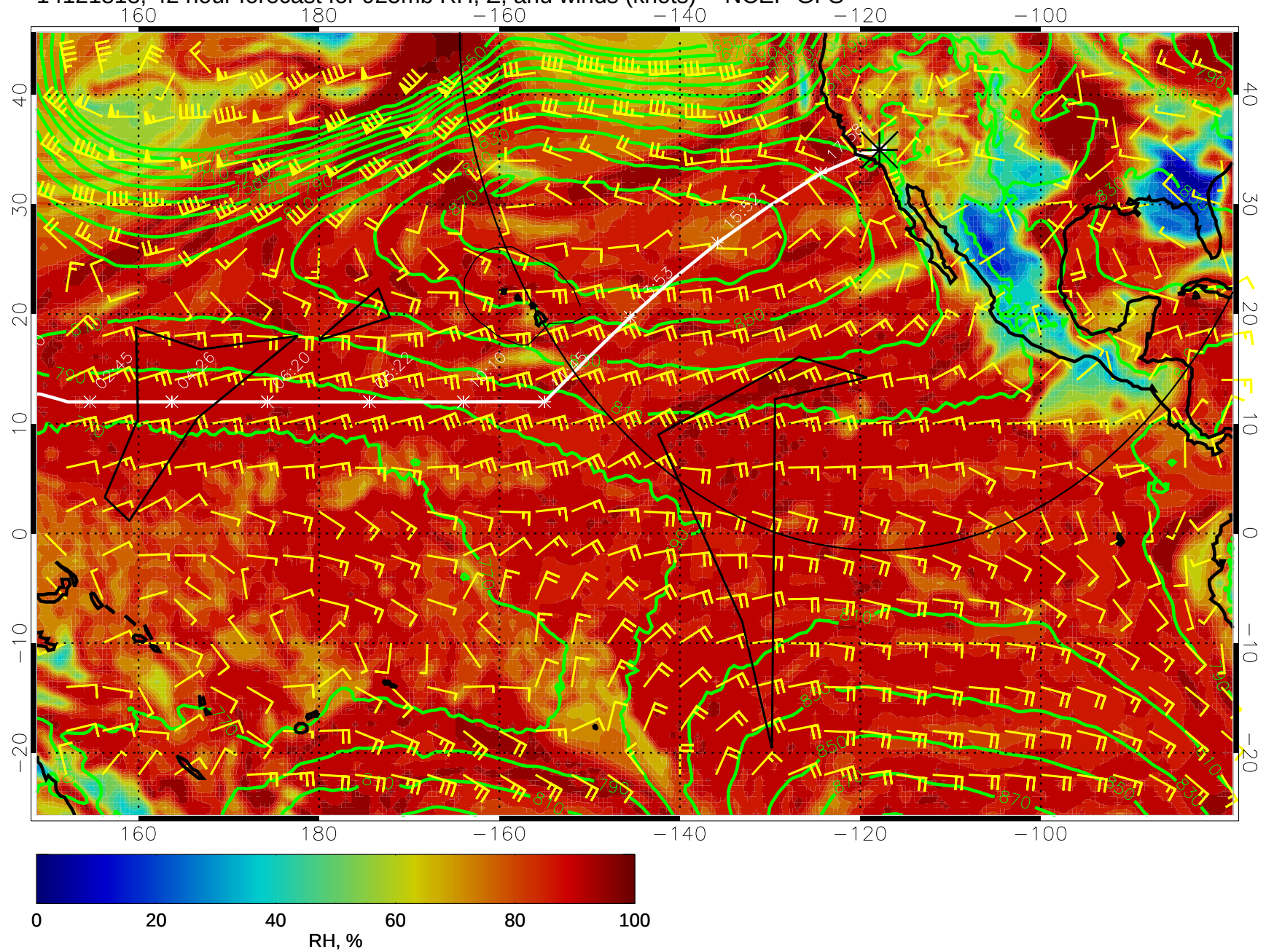
14121818, 42 hour forecast for 925mb RH, Z, and winds (knots) -- NCEP GFS
