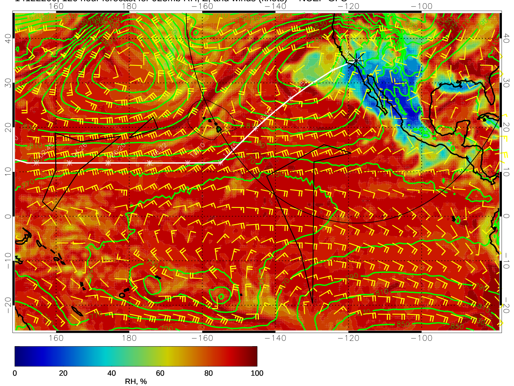
14122200, 120 hour forecast for 925mb RH, Z, and winds (knots) -- NCEP GFS
