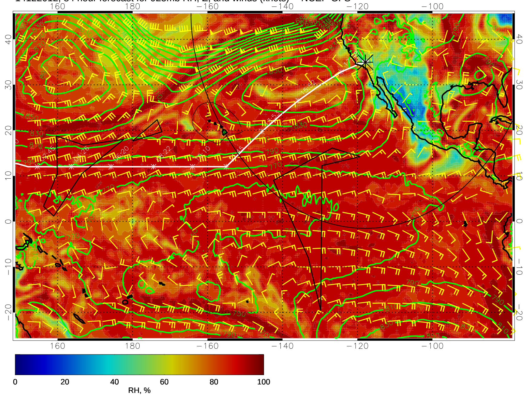
14122012, 84 hour forecast for 925mb RH, Z, and winds (knots) -- NCEP GFS
