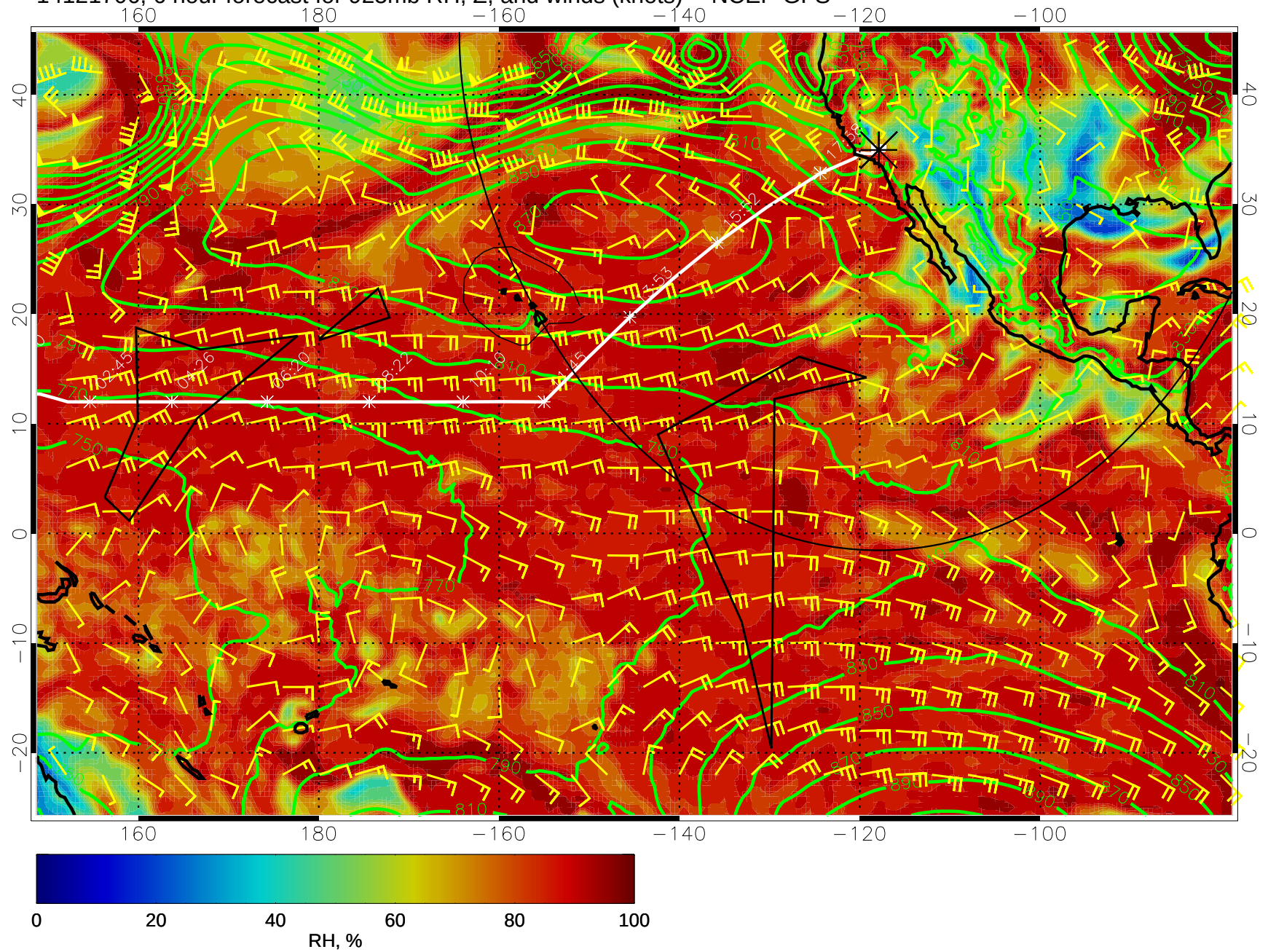
14121706, 6 hour forecast for 925mb RH, Z, and winds (knots) -- NCEP GFS
