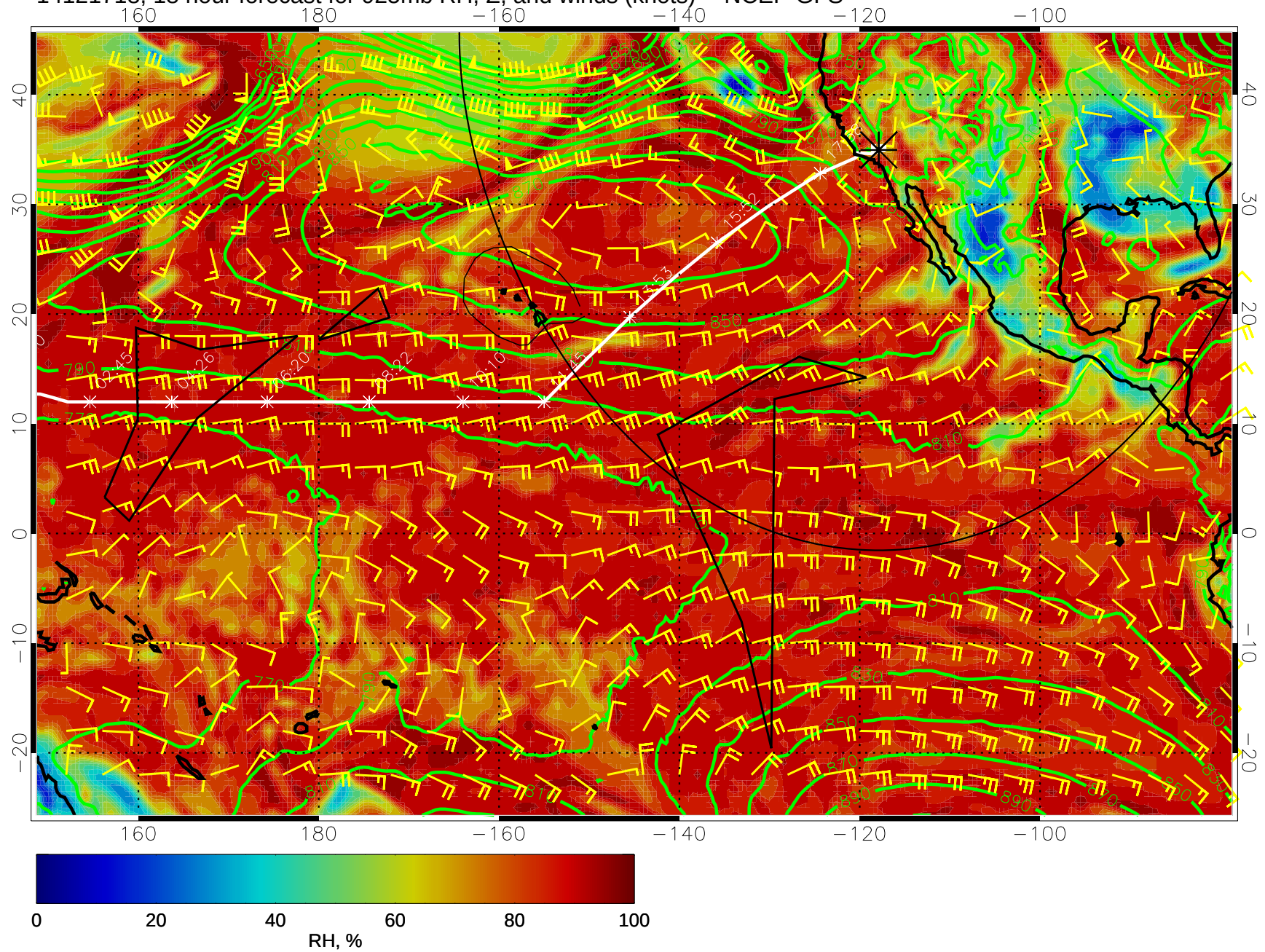
14121718, 18 hour forecast for 925mb RH, Z, and winds (knots) -- NCEP GFS
