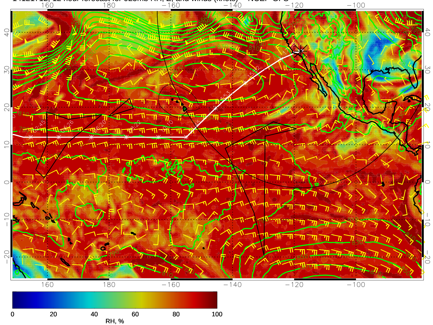
14121712, 12 hour forecast for 925mb RH, Z, and winds (knots) -- NCEP GFS
