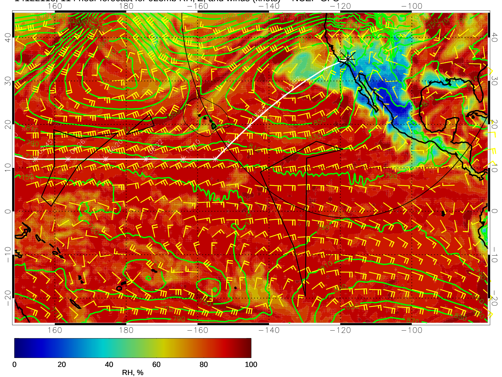
14122118, 114 hour forecast for 925mb RH, Z, and winds (knots) -- NCEP GFS
