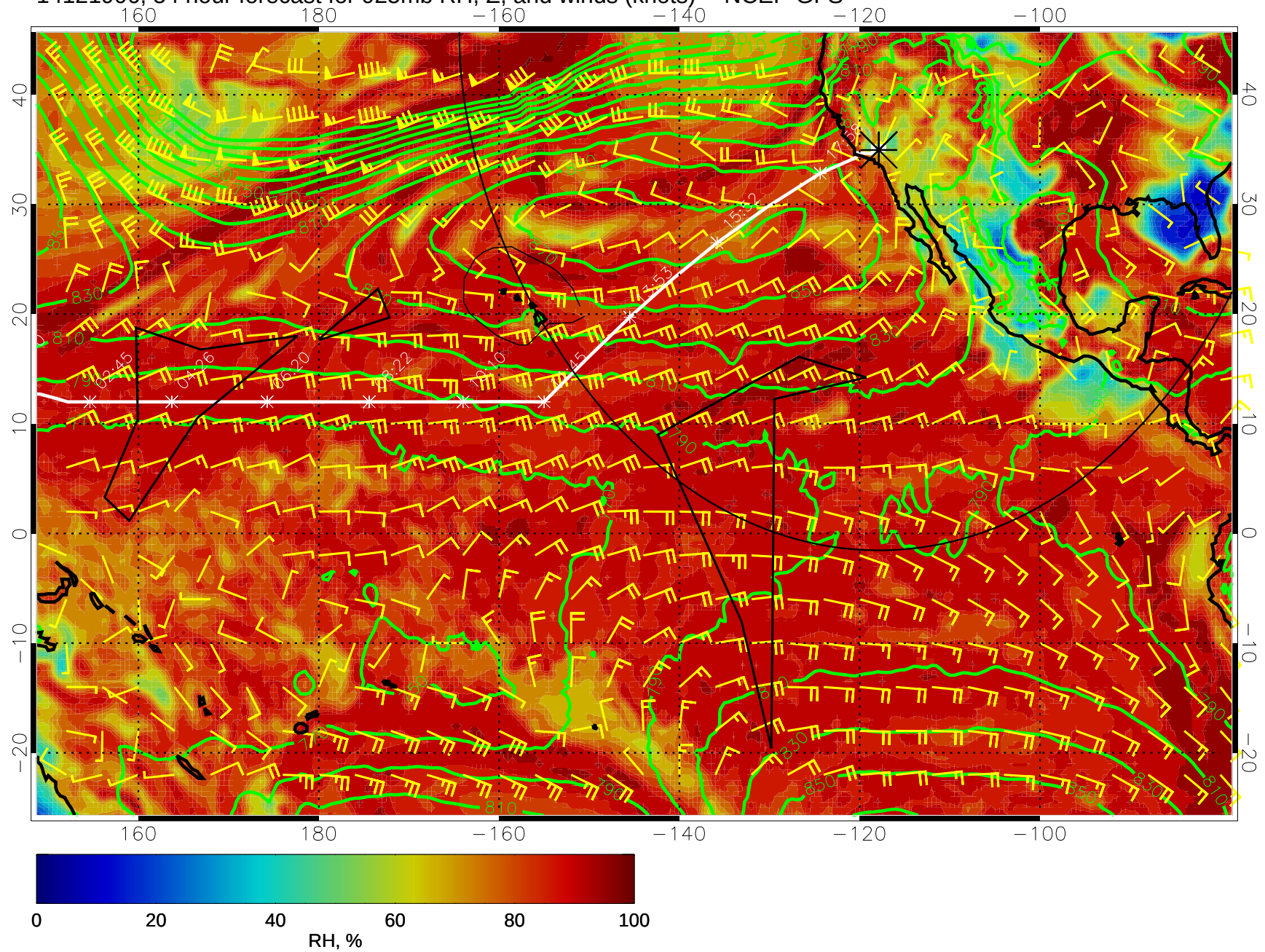
14121906, 54 hour forecast for 925mb RH, Z, and winds (knots) -- NCEP GFS
