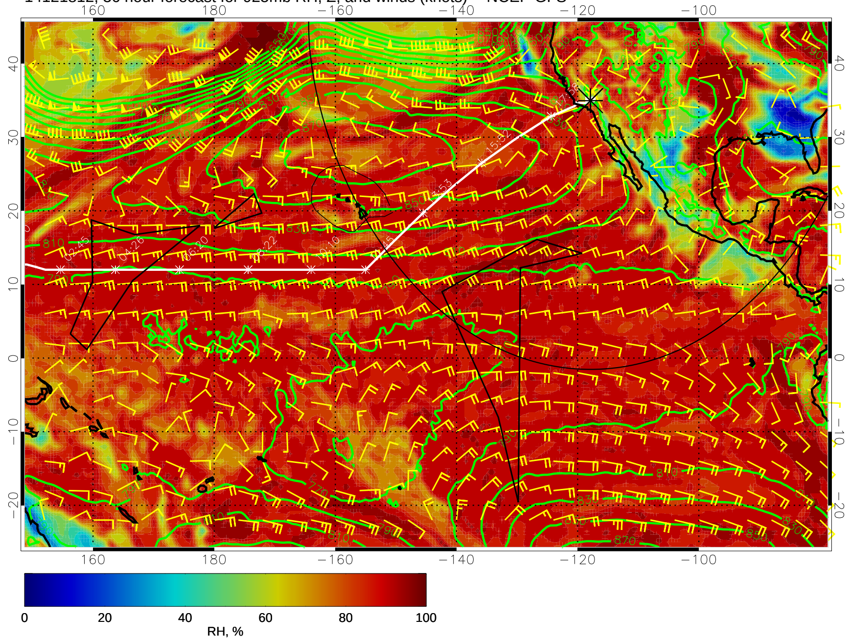
14121812, 36 hour forecast for 925mb RH, Z, and winds (knots) -- NCEP GFS
