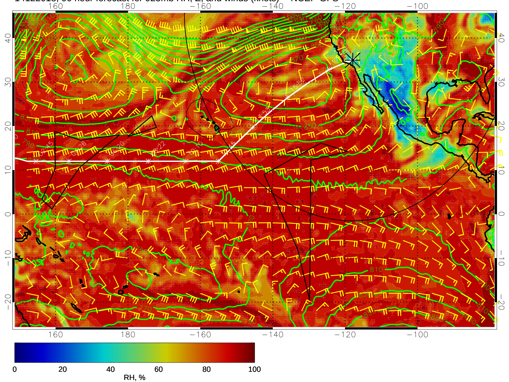
14122018, 90 hour forecast for 925mb RH, Z, and winds (knots) -- NCEP GFS
