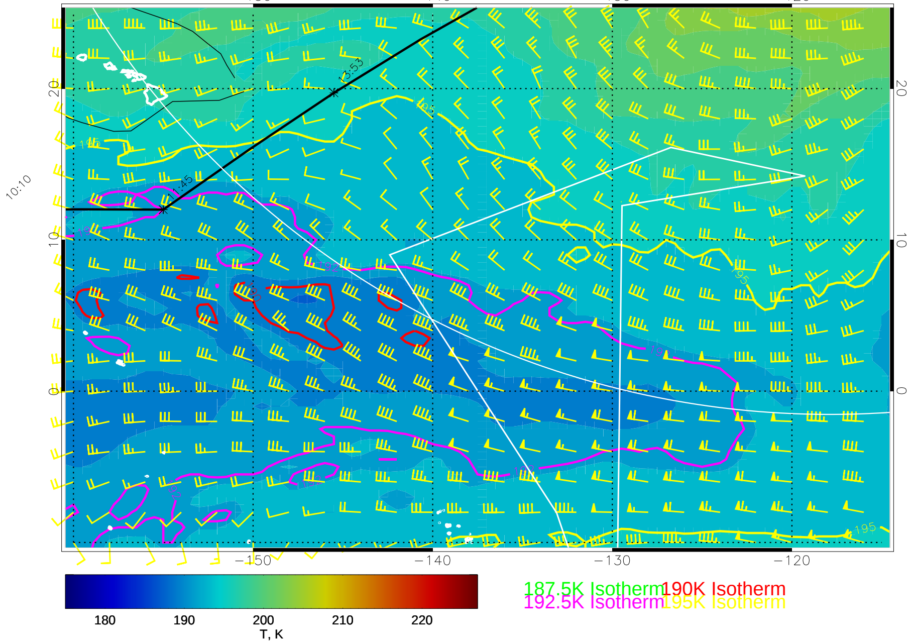
14121812, 36 hour forecast for 100mb T and winds (knots) -- NCEP GFS
