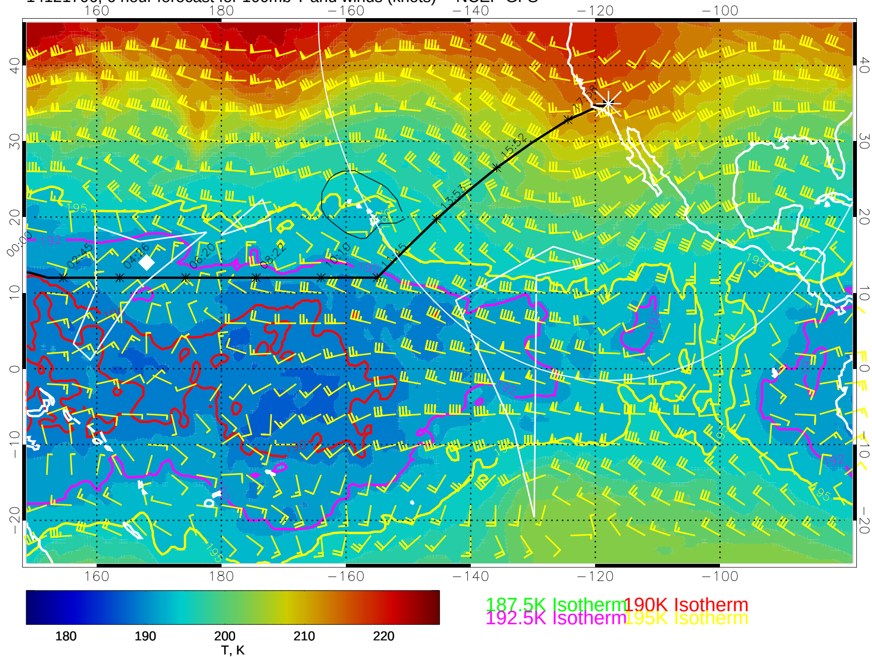
14121706, 6 hour forecast for 100mb T and winds (knots) -- NCEP GFS
