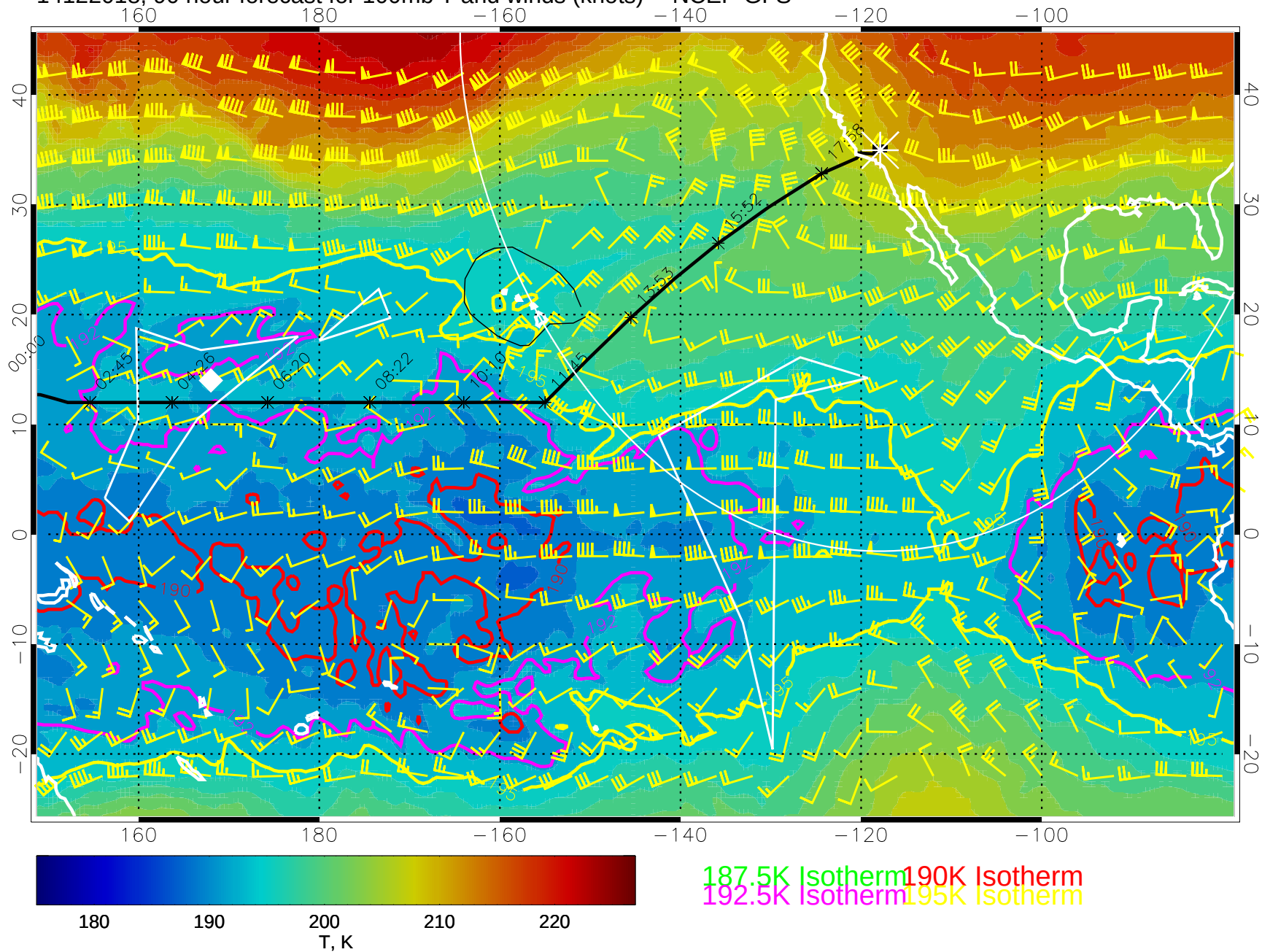
14122018, 90 hour forecast for 100mb T and winds (knots) -- NCEP GFS
