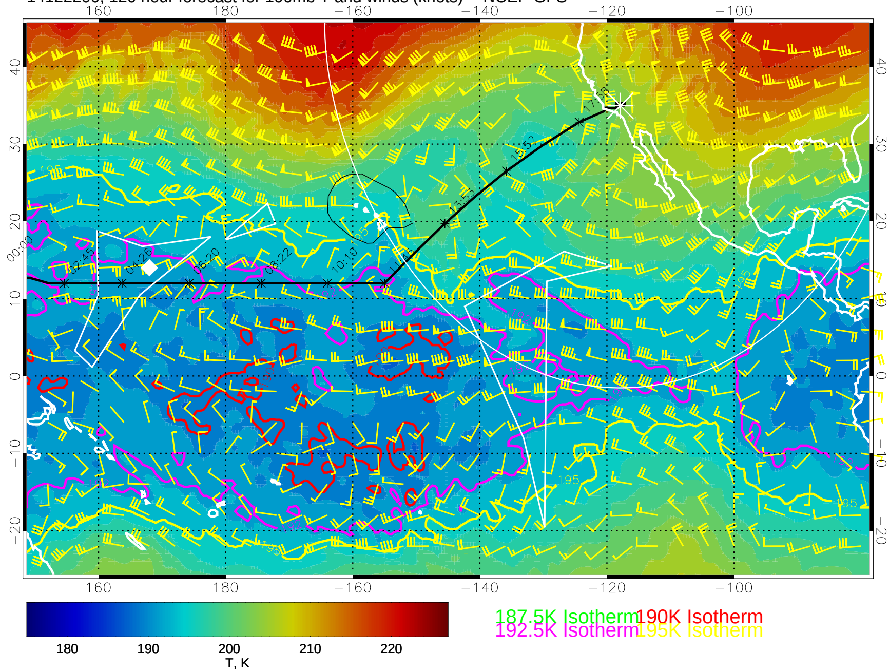
14122200, 120 hour forecast for 100mb T and winds (knots) -- NCEP GFS
