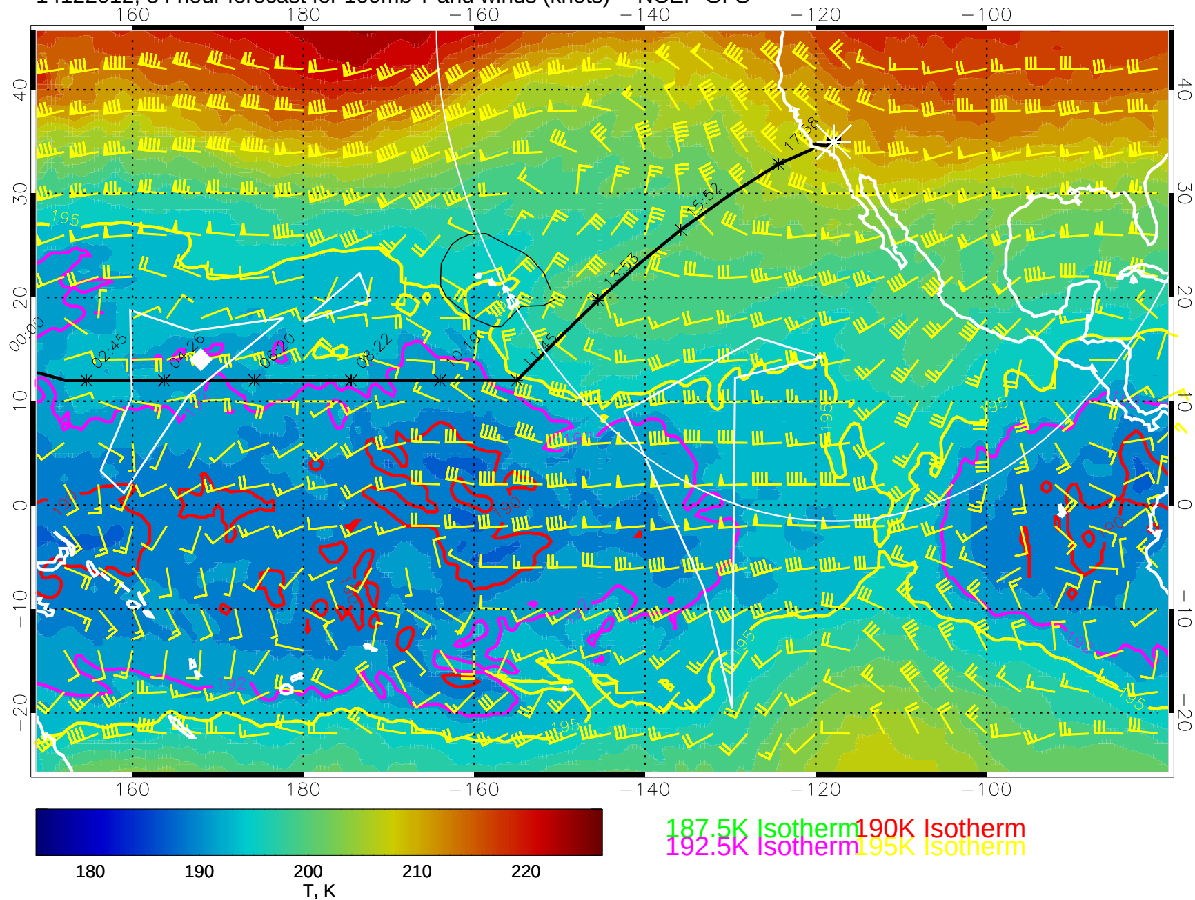
14122012, 84 hour forecast for 100mb T and winds (knots) -- NCEP GFS
