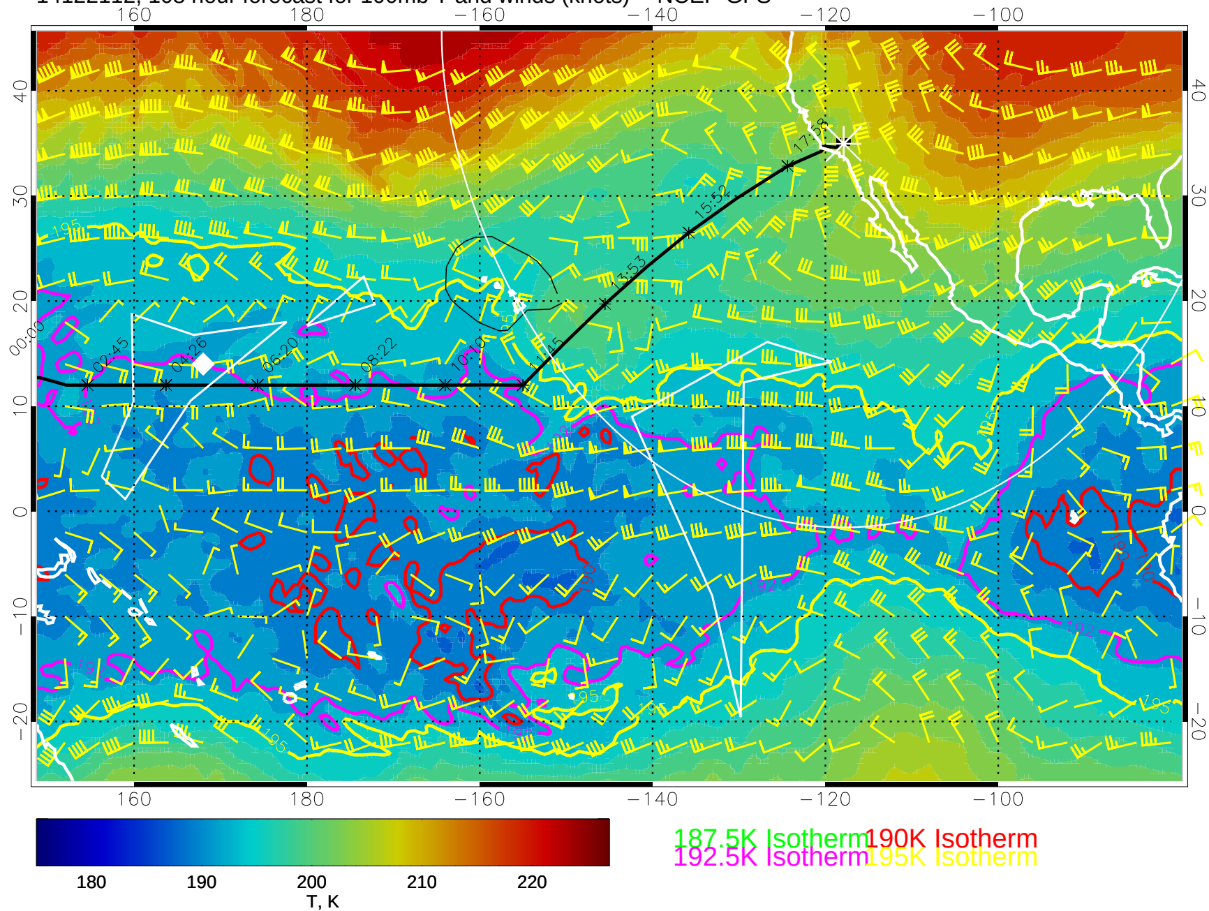
14122112, 108 hour forecast for 100mb T and winds (knots) -- NCEP GFS
