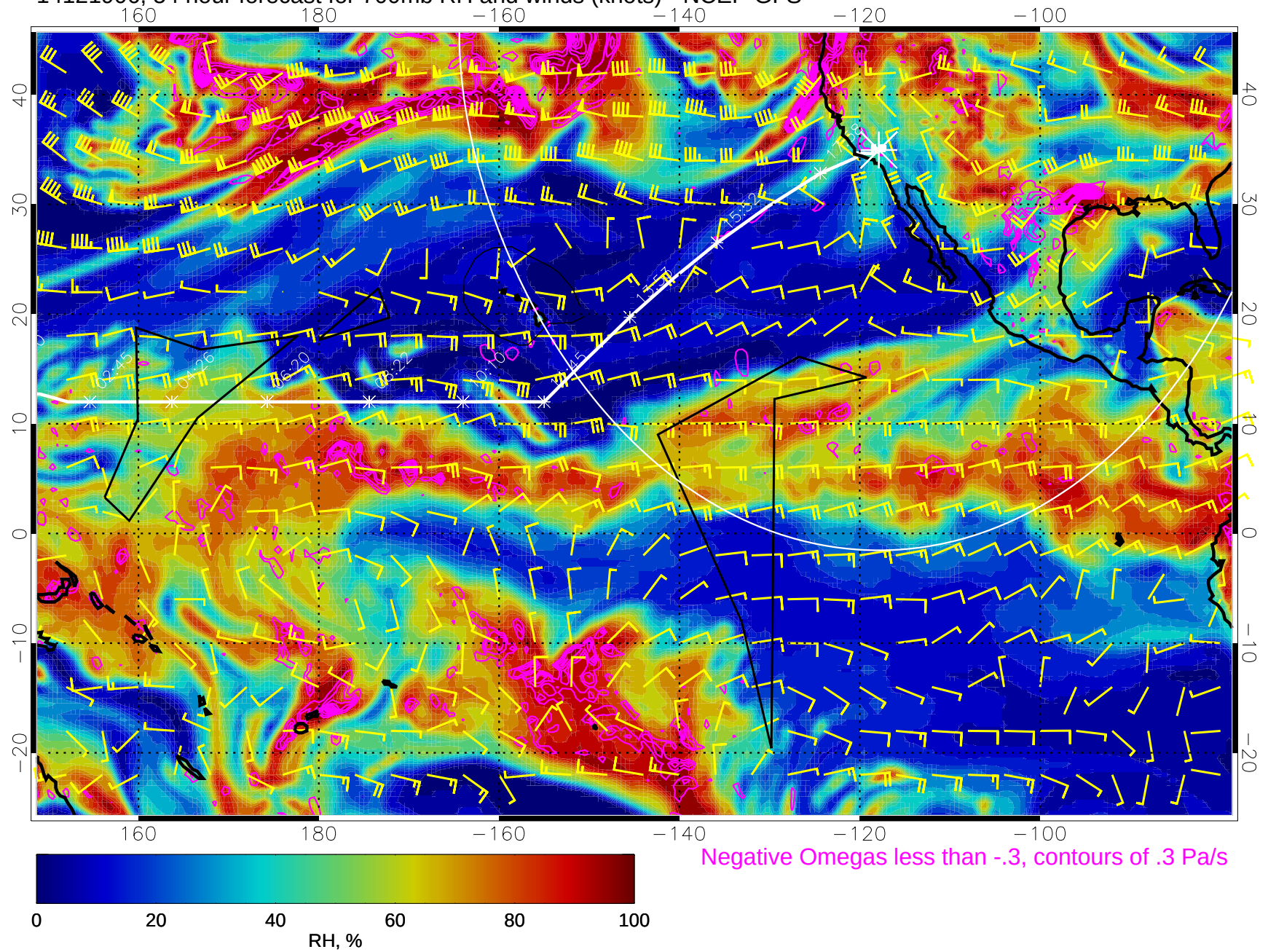
14121906, 54 hour forecast for 700mb RH and winds (knots) - NCEP GFS
