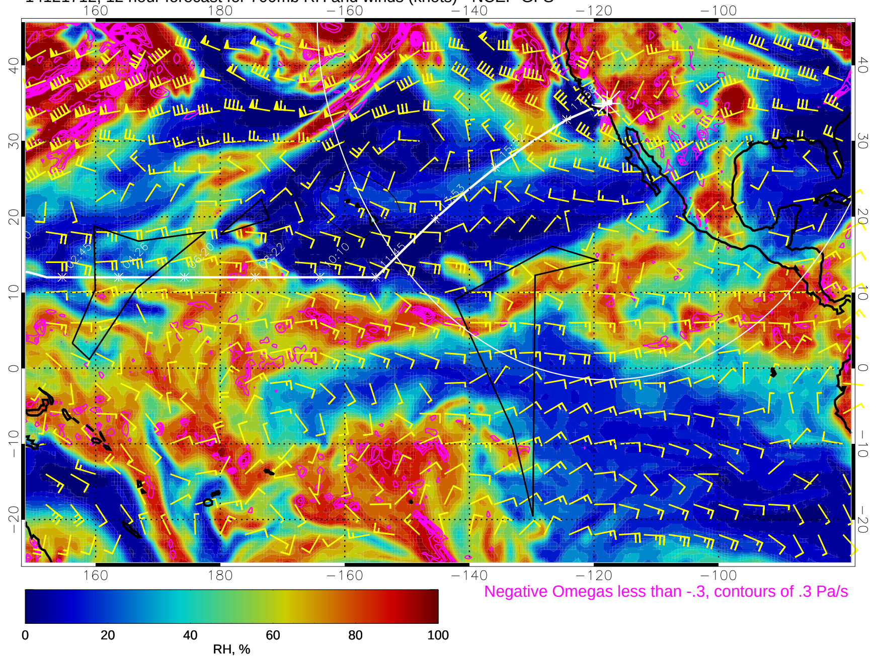
14121712, 12 hour forecast for 700mb RH and winds (knots) - NCEP GFS
