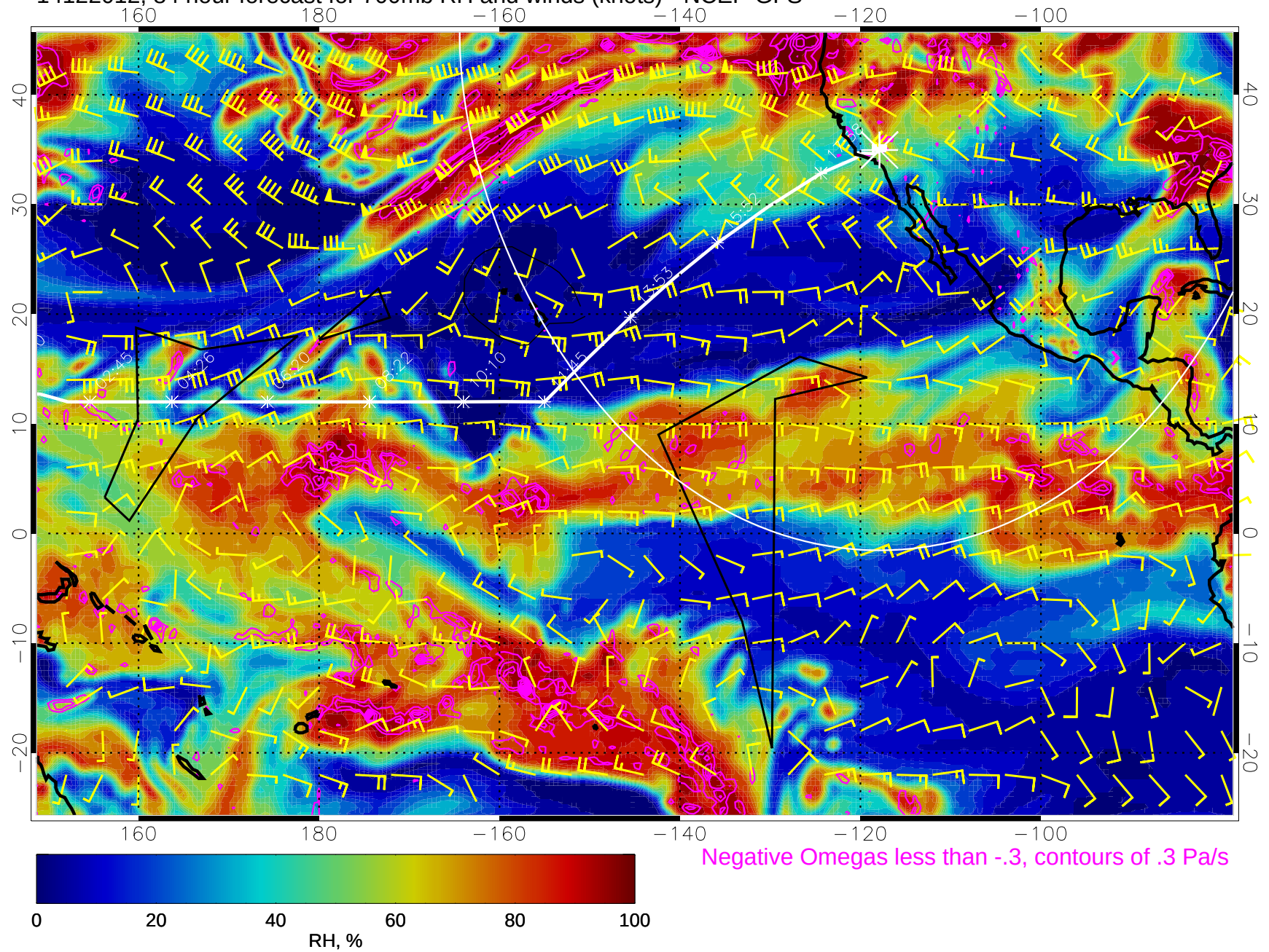
14122012, 84 hour forecast for 700mb RH and winds (knots) - NCEP GFS
