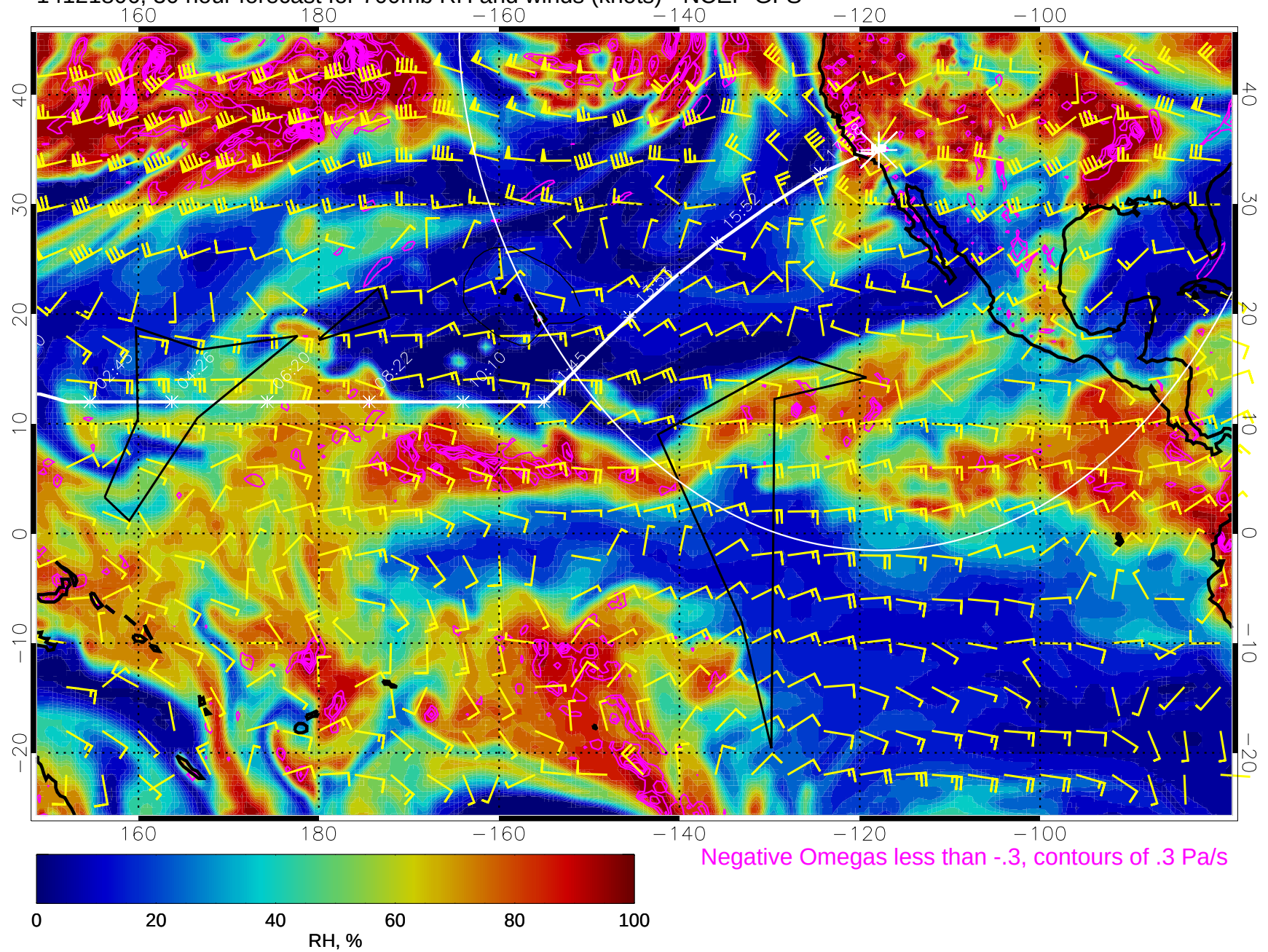
14121806, 30 hour forecast for 700mb RH and winds (knots) - NCEP GFS
