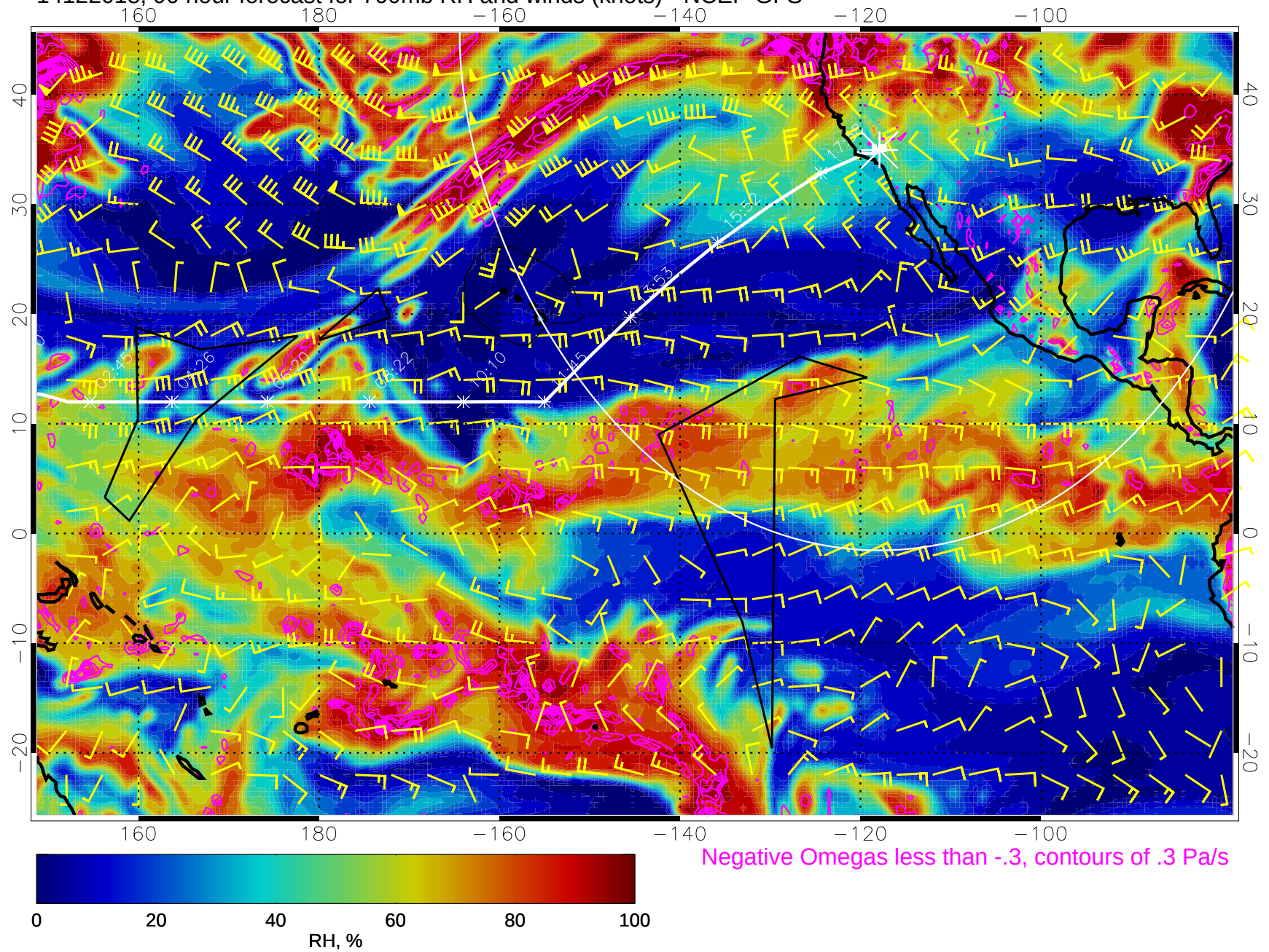
14122018, 90 hour forecast for 700mb RH and winds (knots) - NCEP GFS
