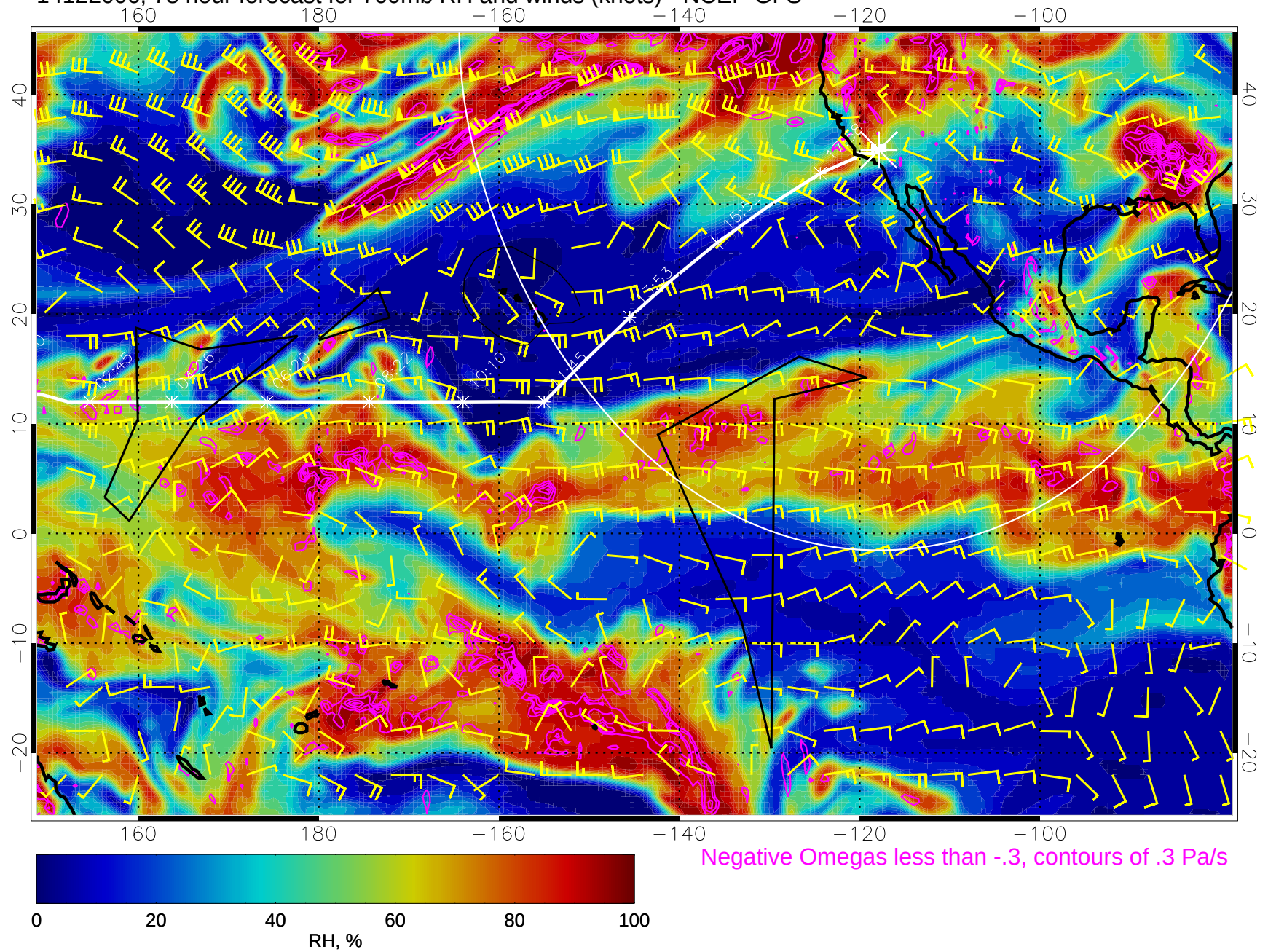
14122006, 78 hour forecast for 700mb RH and winds (knots) - NCEP GFS
