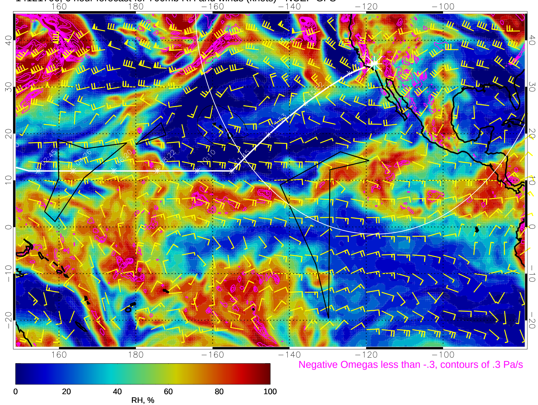
14121706, 6 hour forecast for 700mb RH and winds (knots) - NCEP GFS
