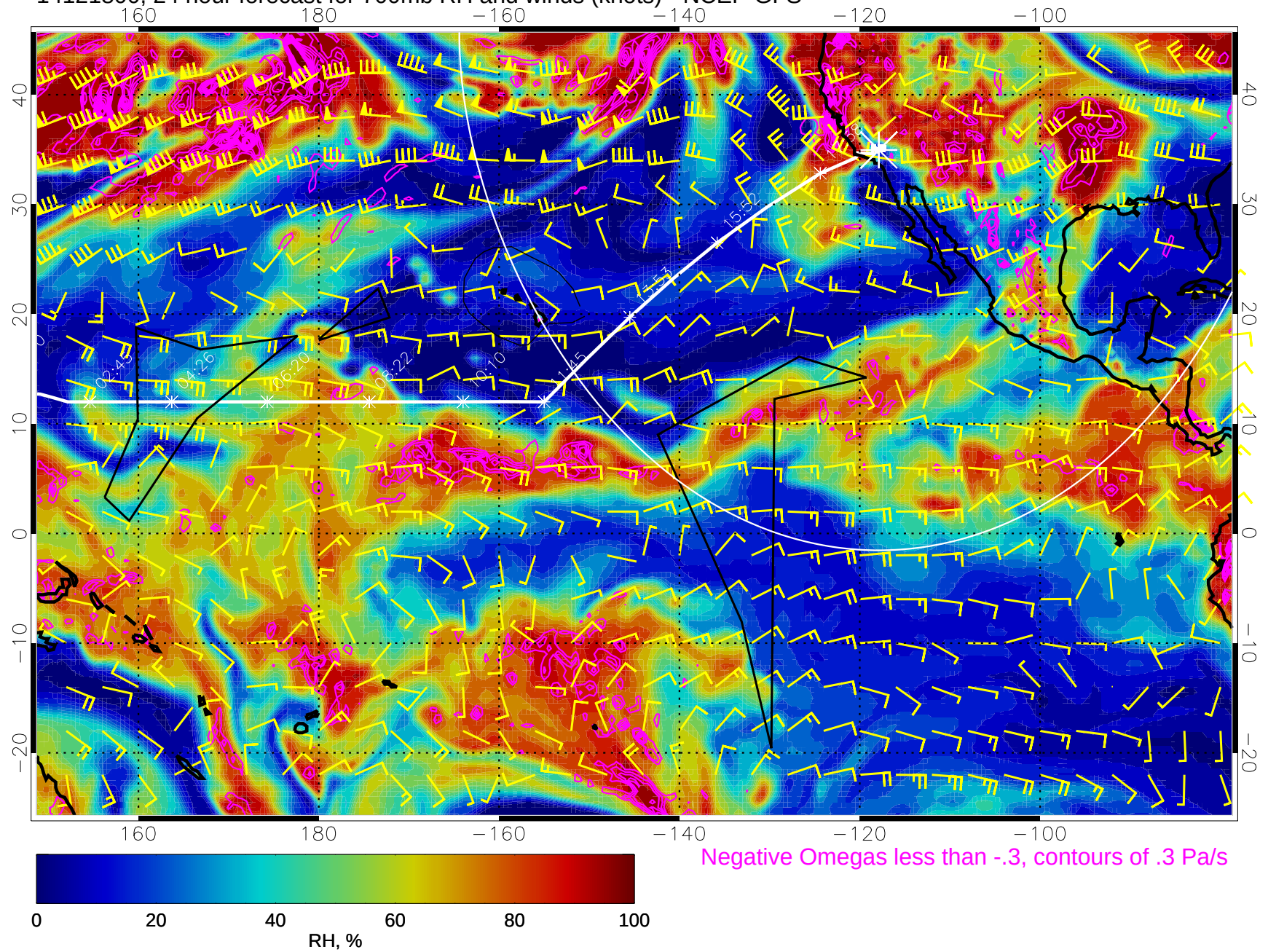
14121800, 24 hour forecast for 700mb RH and winds (knots) - NCEP GFS
