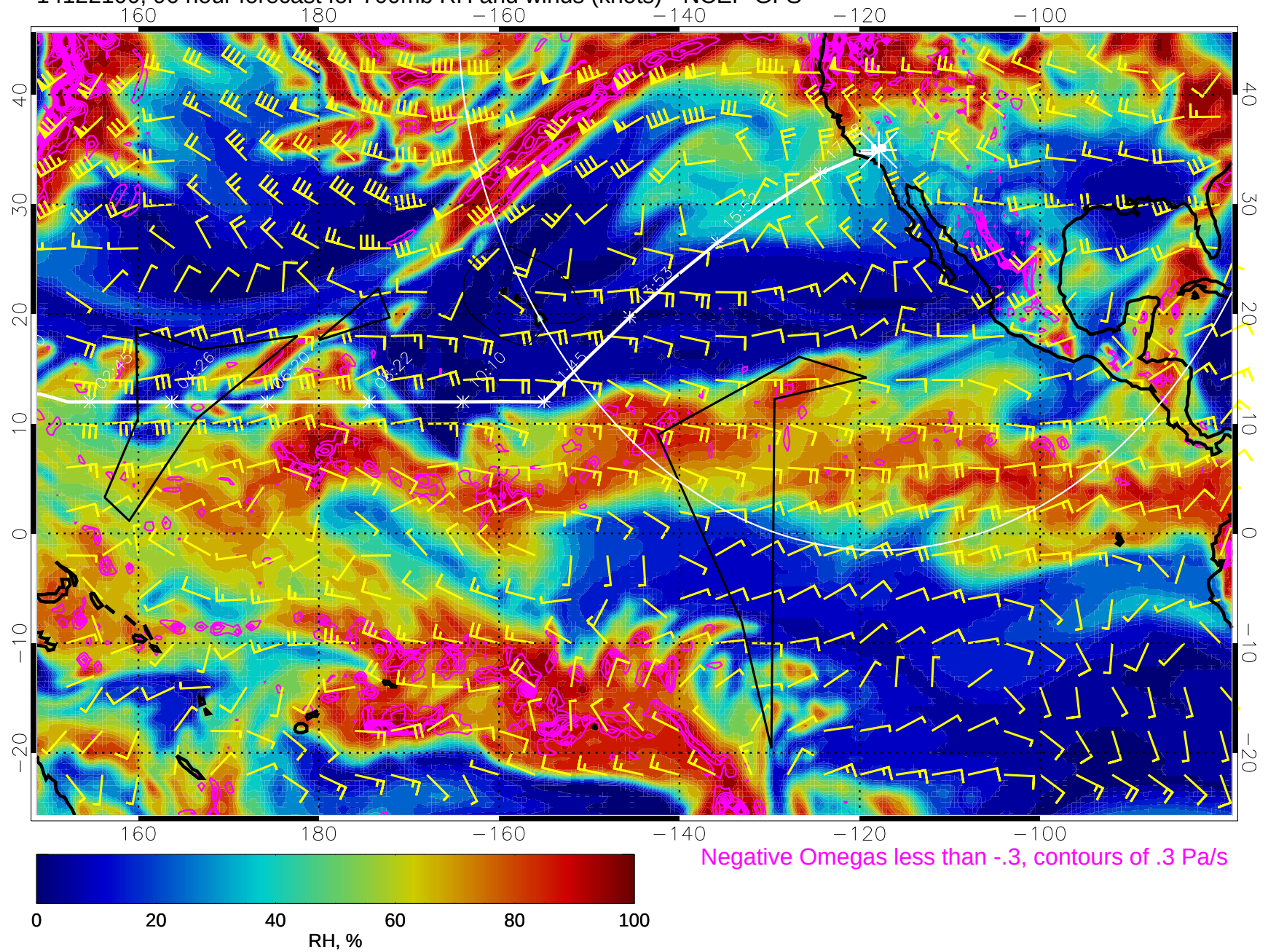
14122100, 96 hour forecast for 700mb RH and winds (knots) - NCEP GFS
