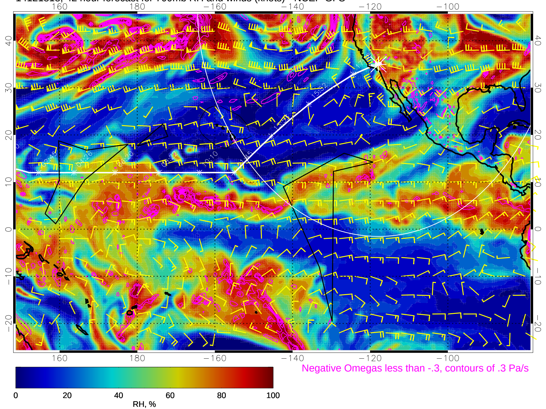
14121818, 42 hour forecast for 700mb RH and winds (knots) - NCEP GFS
