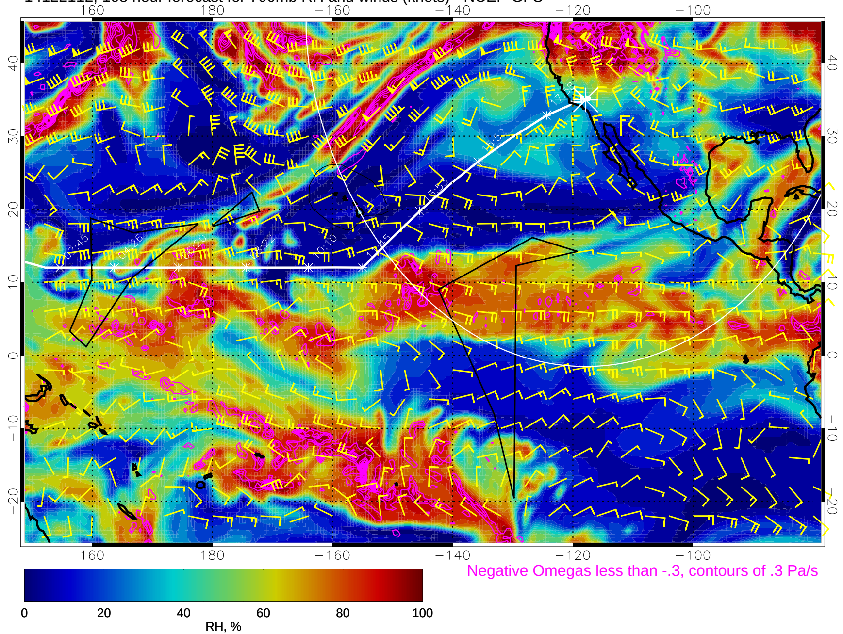
14122112, 108 hour forecast for 700mb RH and winds (knots) - NCEP GFS
