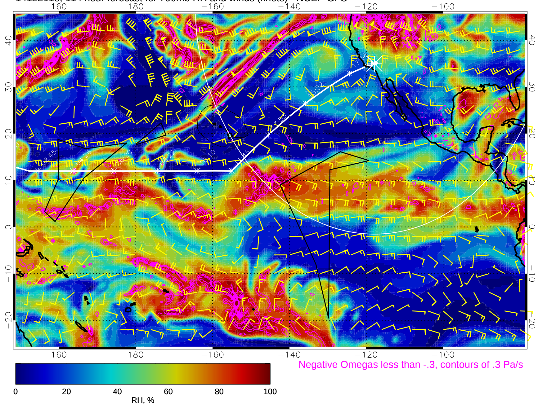
14122118, 114 hour forecast for 700mb RH and winds (knots) - NCEP GFS
