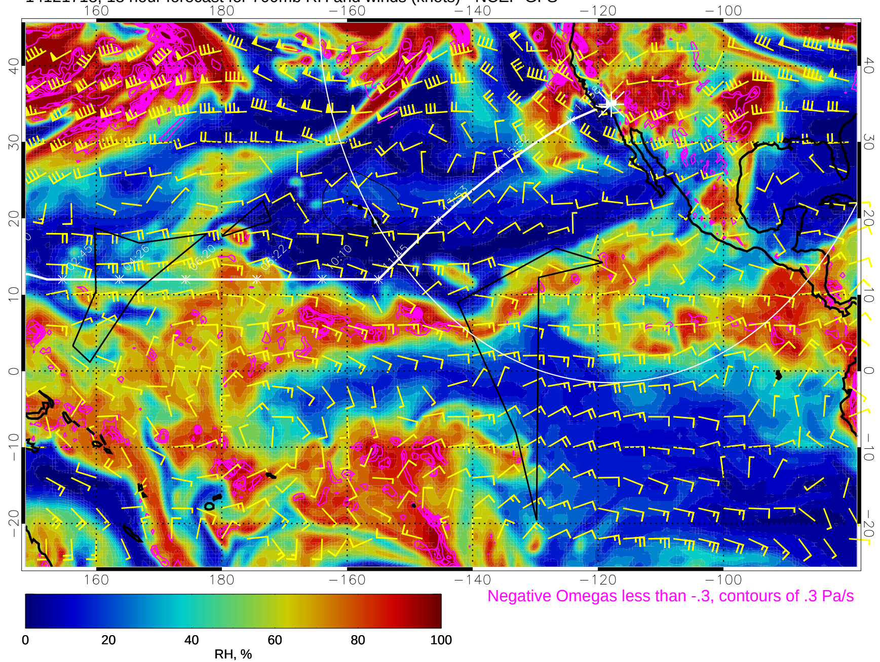
14121718, 18 hour forecast for 700mb RH and winds (knots) - NCEP GFS
