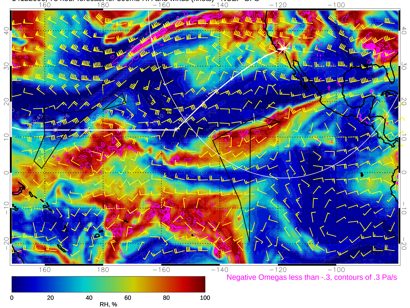
14122006, 78 hour forecast for 500mb RH and winds (knots) - NCEP GFS
