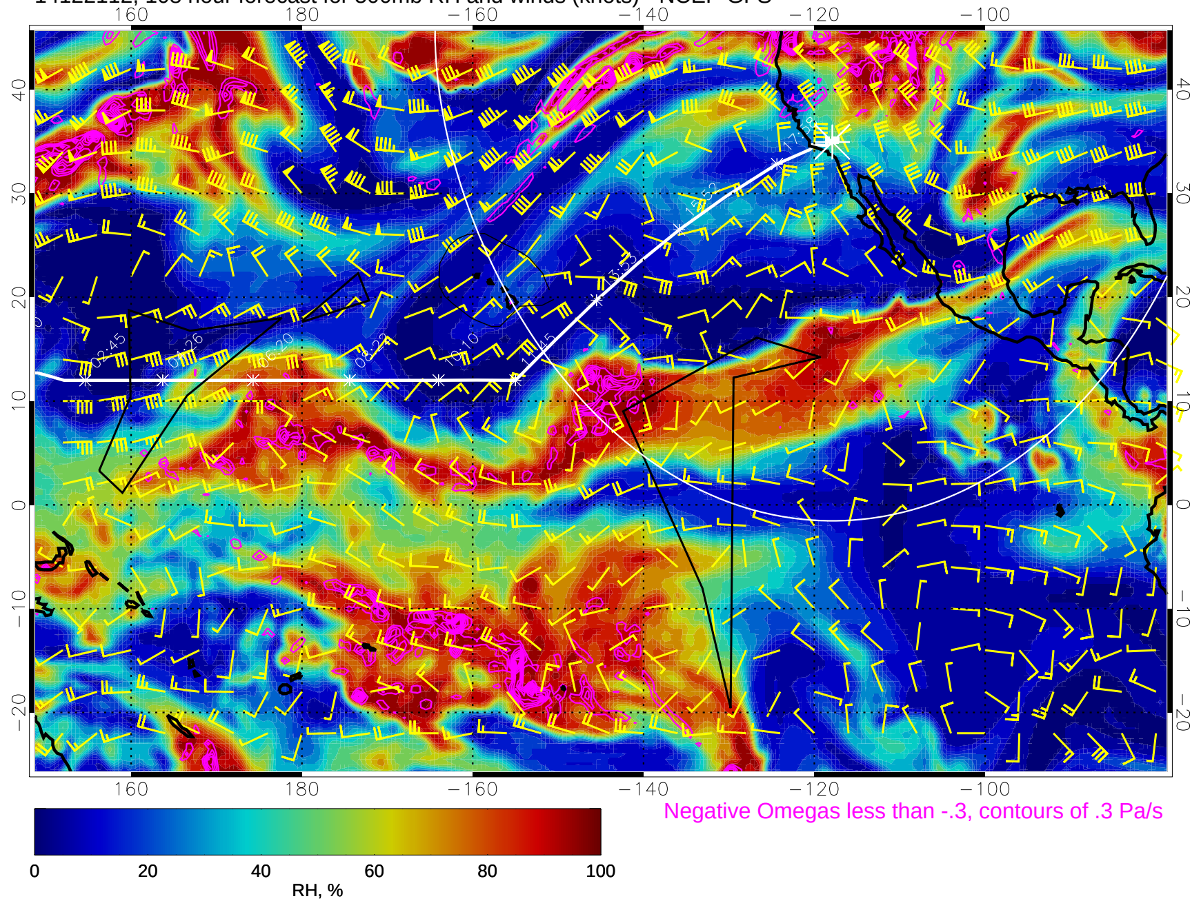
14122112, 108 hour forecast for 500mb RH and winds (knots) - NCEP GFS
