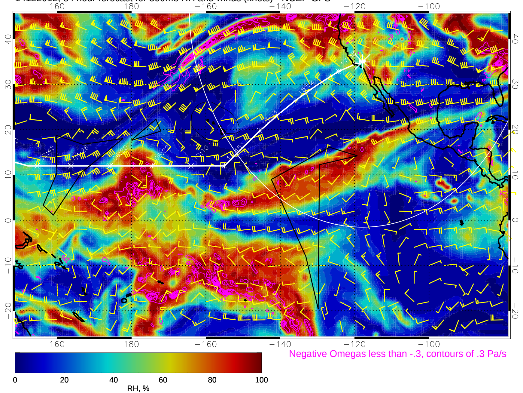
14122012, 84 hour forecast for 500mb RH and winds (knots) - NCEP GFS
