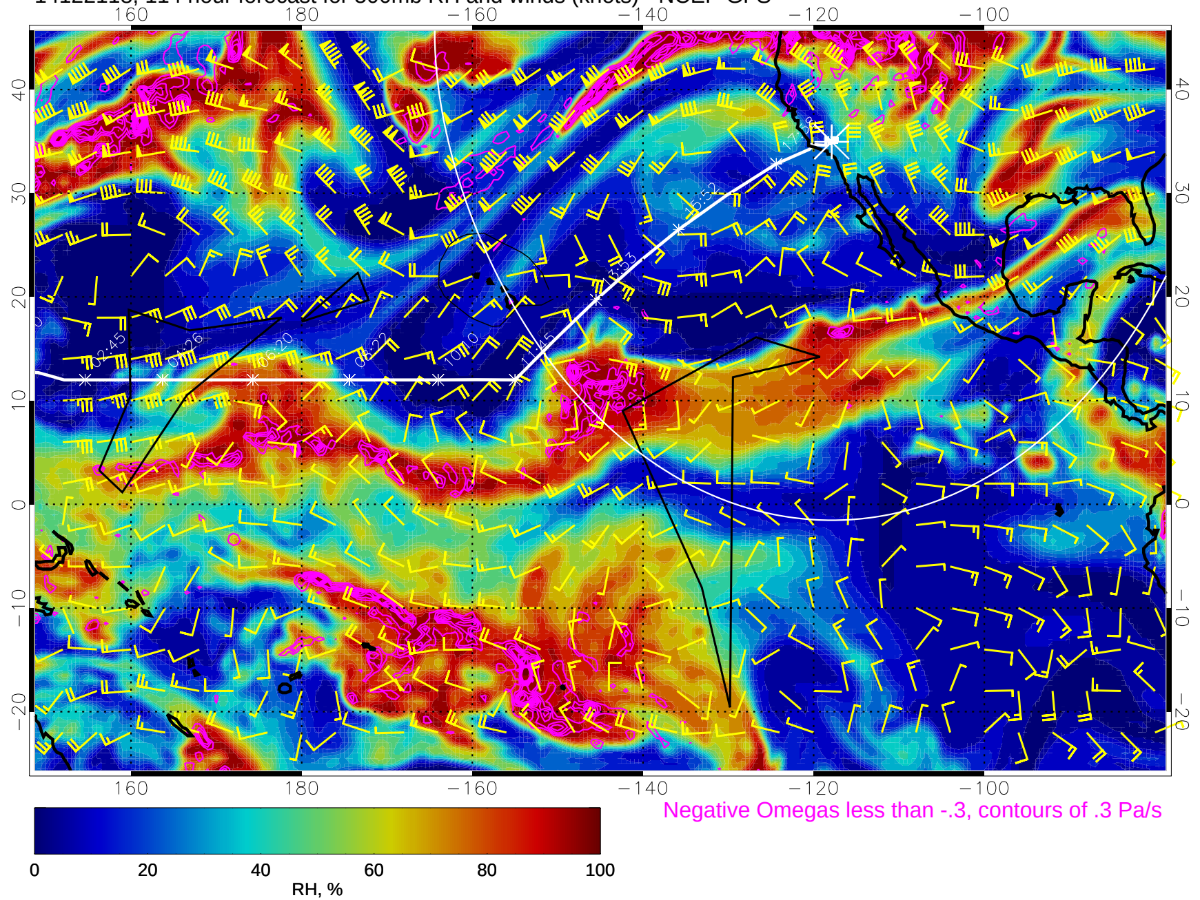
14122118, 114 hour forecast for 500mb RH and winds (knots) - NCEP GFS
