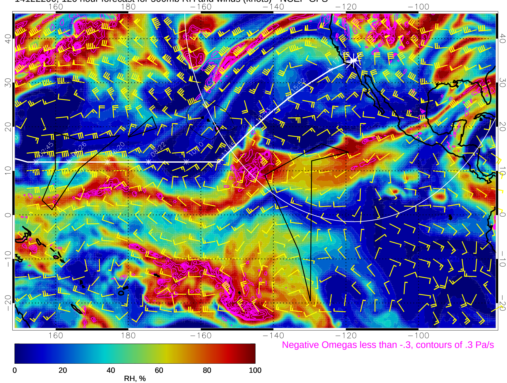
14122200, 120 hour forecast for 500mb RH and winds (knots) - NCEP GFS
