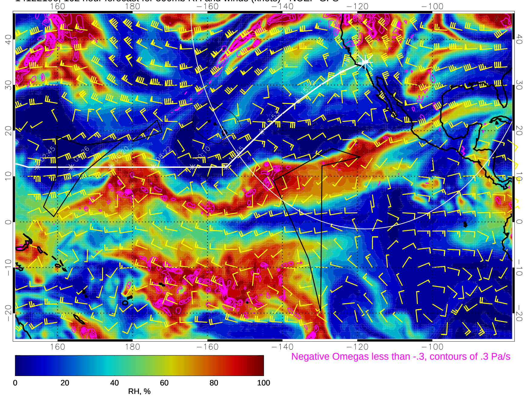
14122106, 102 hour forecast for 500mb RH and winds (knots) - NCEP GFS
