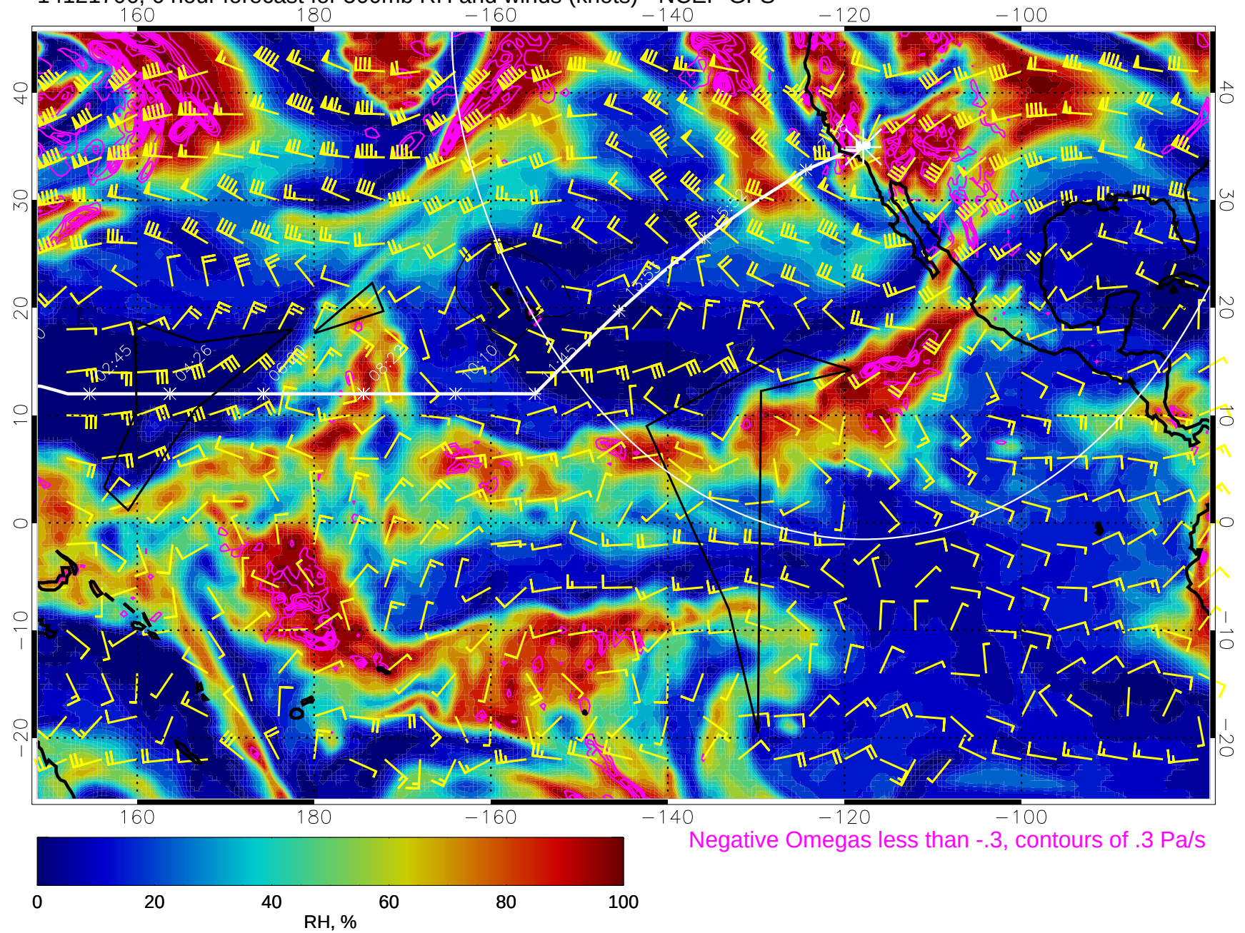
14121706, 6 hour forecast for 500mb RH and winds (knots) - NCEP GFS
