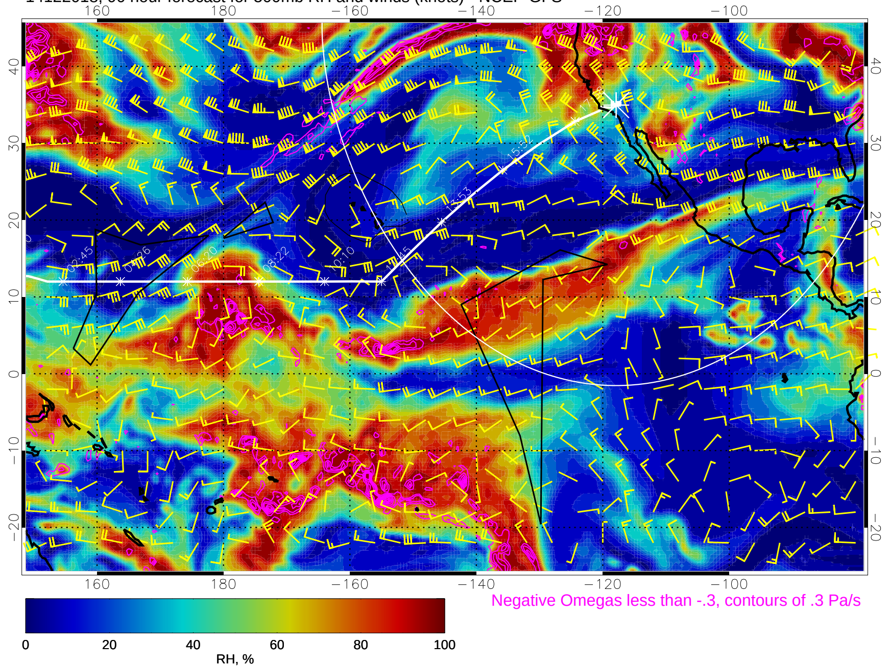
14122018, 90 hour forecast for 500mb RH and winds (knots) - NCEP GFS
