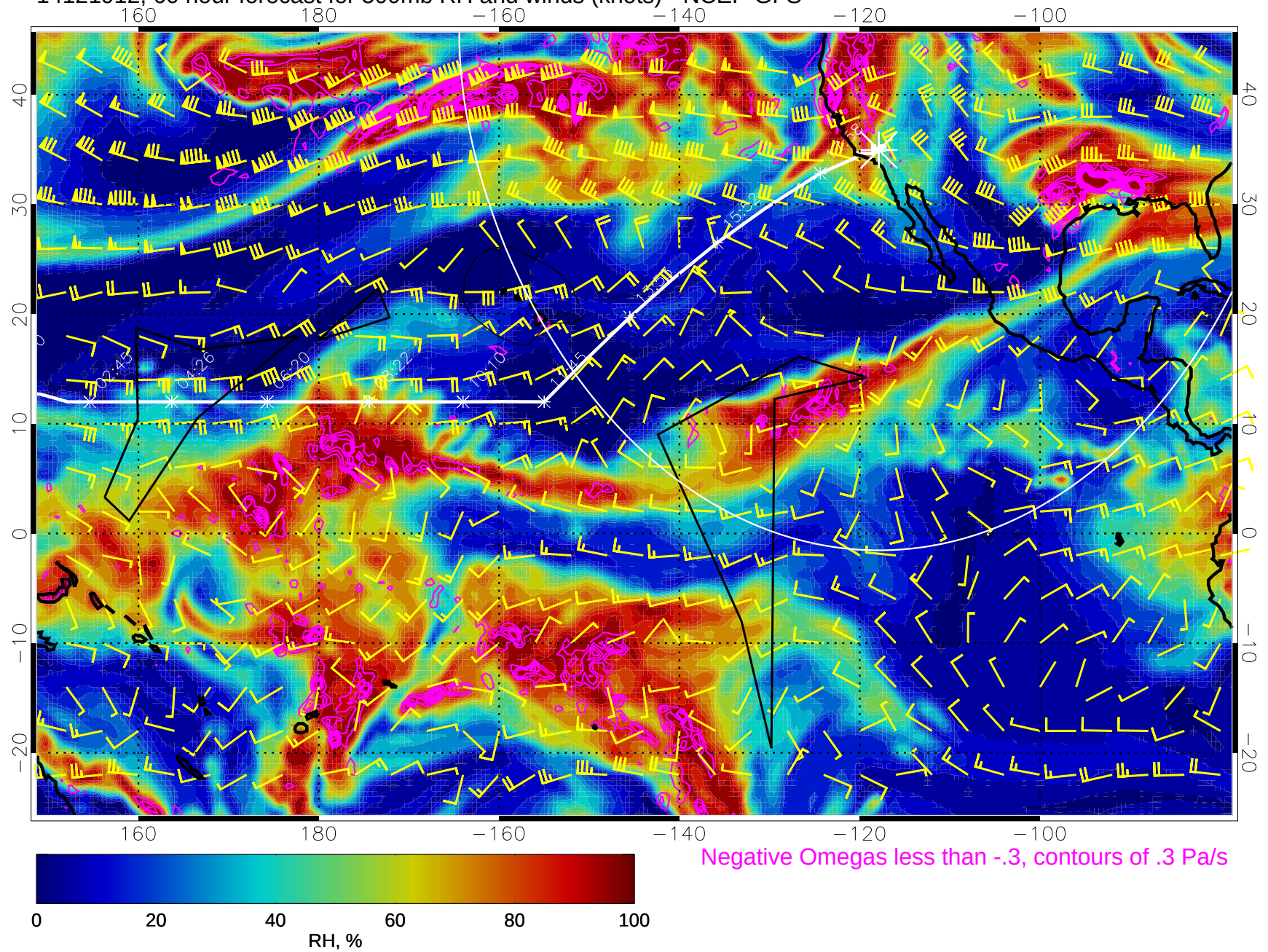
14121912, 60 hour forecast for 500mb RH and winds (knots) - NCEP GFS
