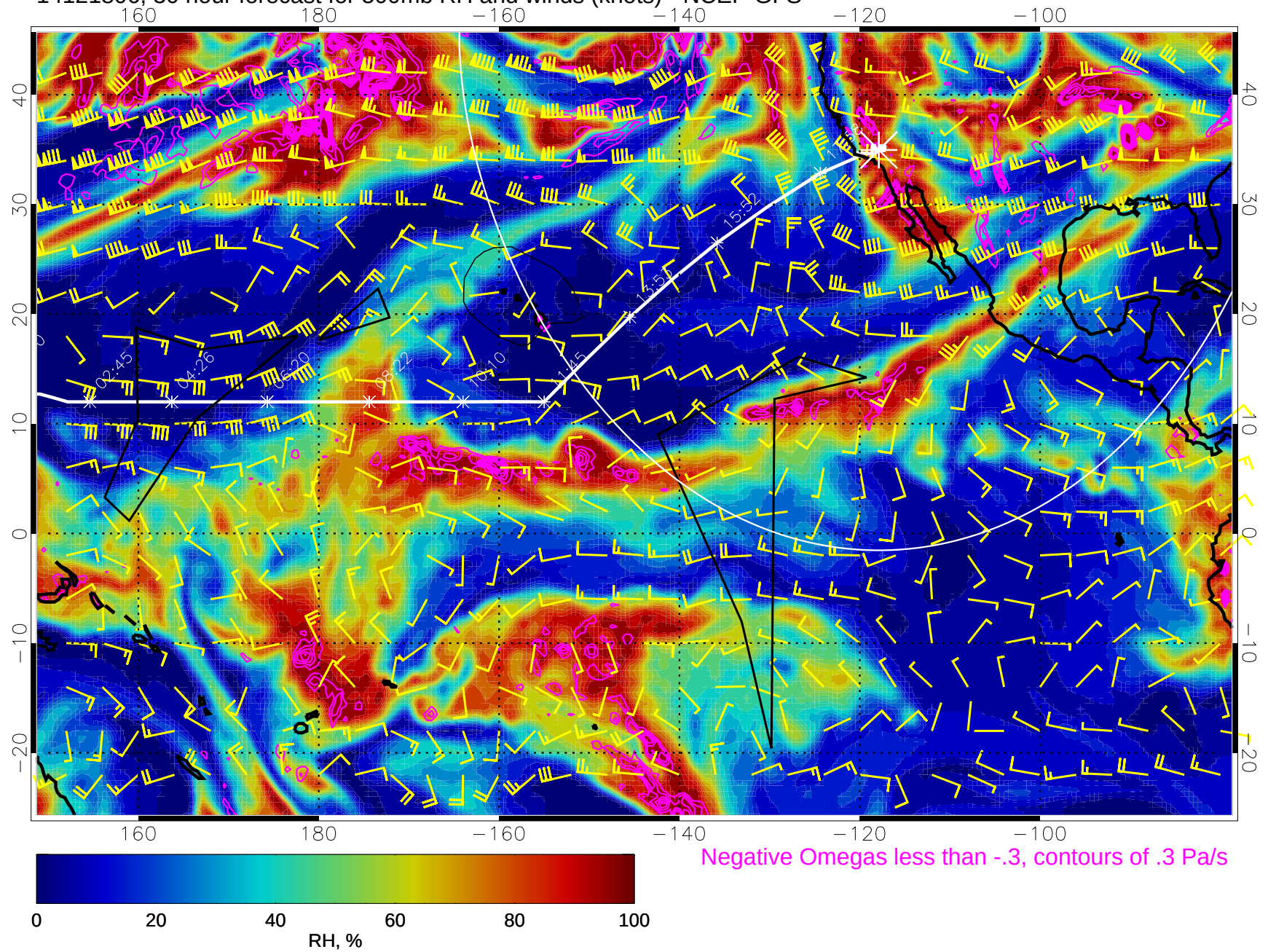
14121806, 30 hour forecast for 500mb RH and winds (knots) - NCEP GFS
