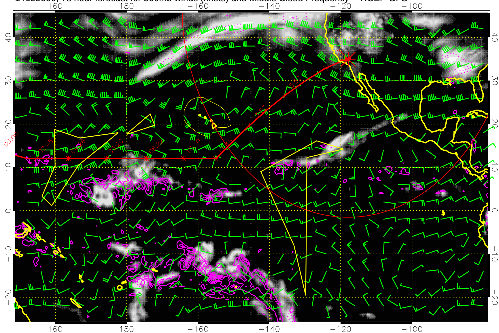
14122006, 78 hour forecast for 500mb winds (knots) and Middle Cloud Frequency -- NCEP GFS
