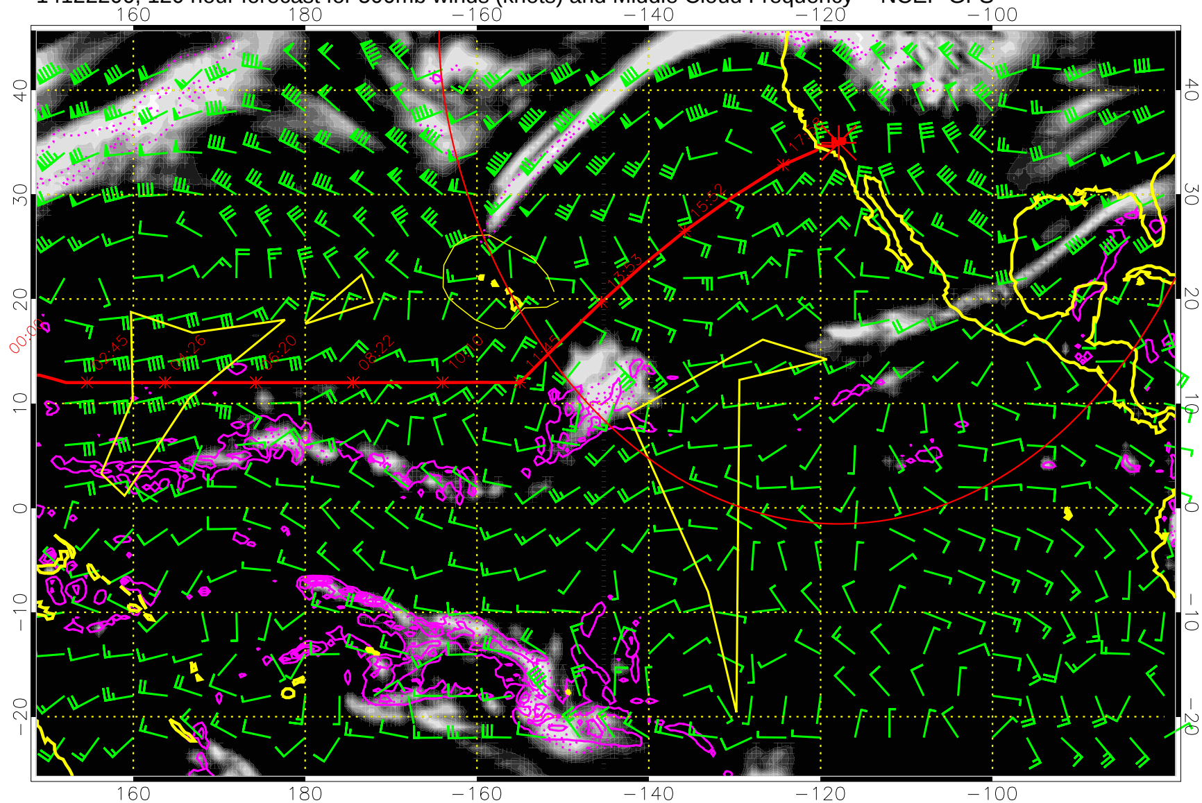
14122200, 120 hour forecast for 500mb winds (knots) and Middle Cloud Frequency -- NCEP GFS
