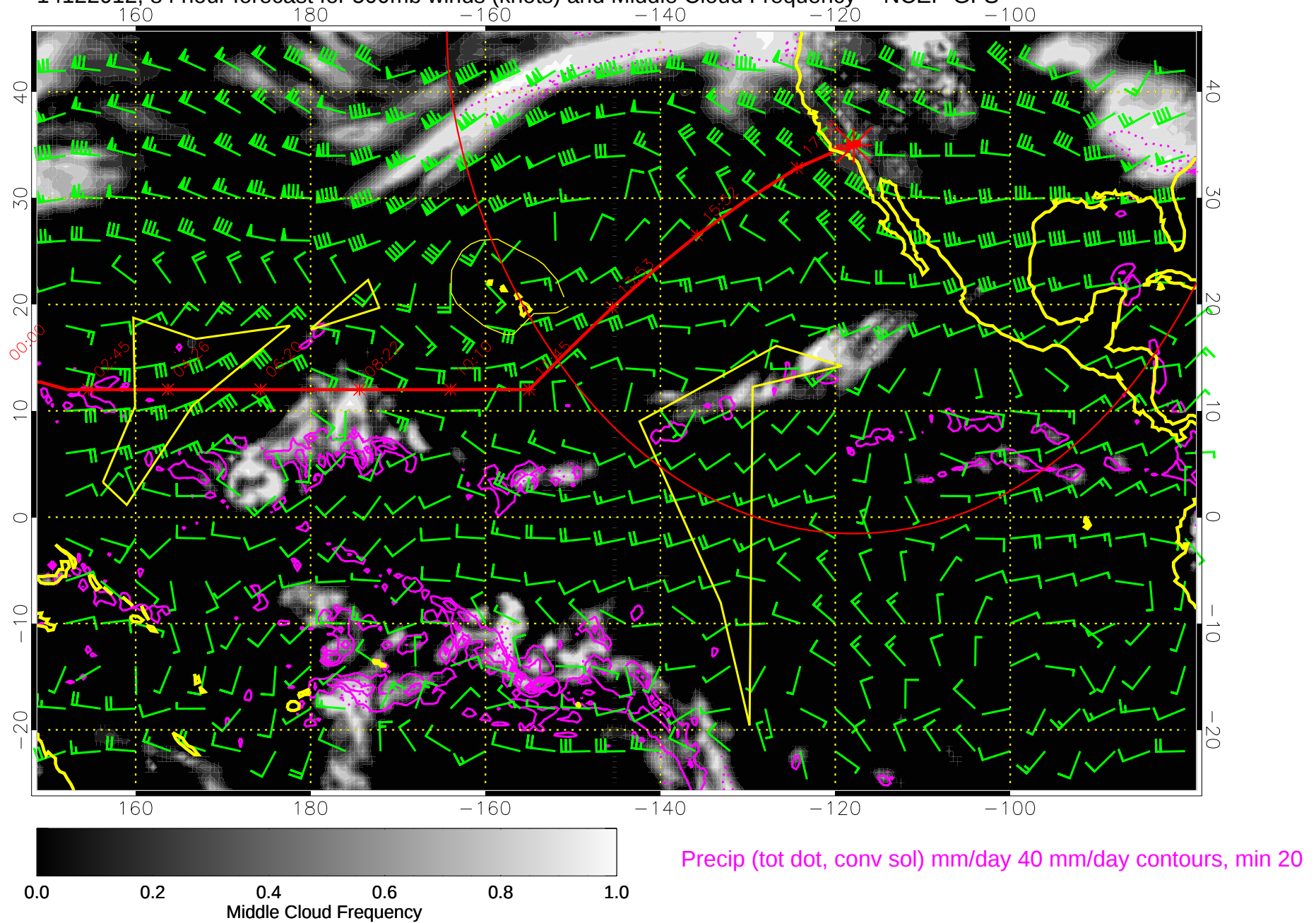
14122012, 84 hour forecast for 500mb winds (knots) and Middle Cloud Frequency -- NCEP GFS
