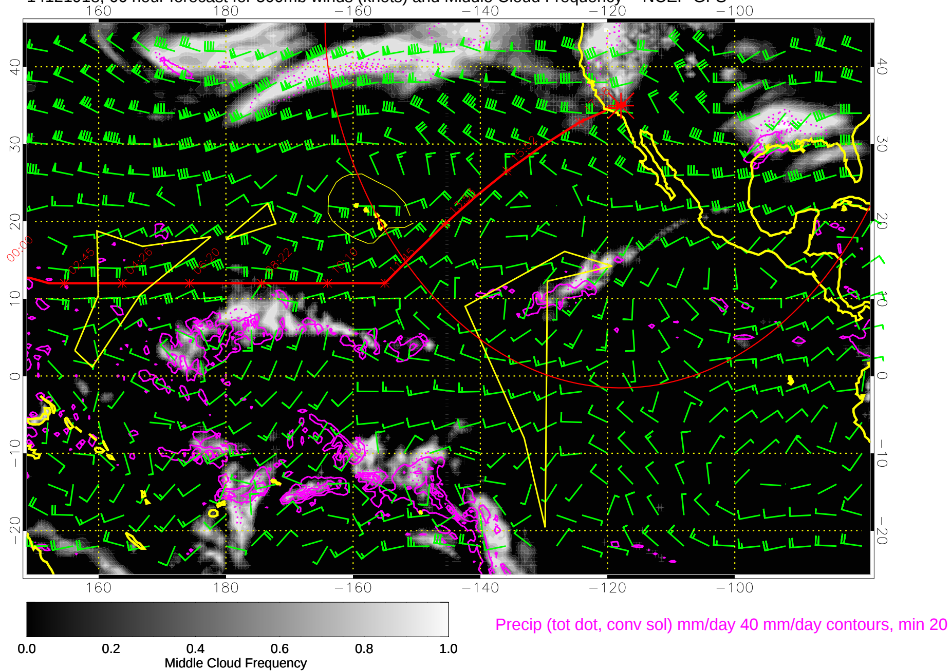
14121918, 66 hour forecast for 500mb winds (knots) and Middle Cloud Frequency -- NCEP GFS
