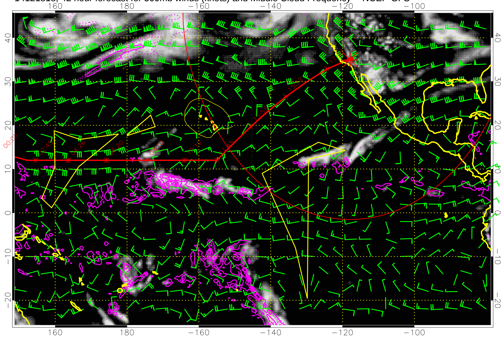
14121818, 42 hour forecast for 500mb winds (knots) and Middle Cloud Frequency -- NCEP GFS
