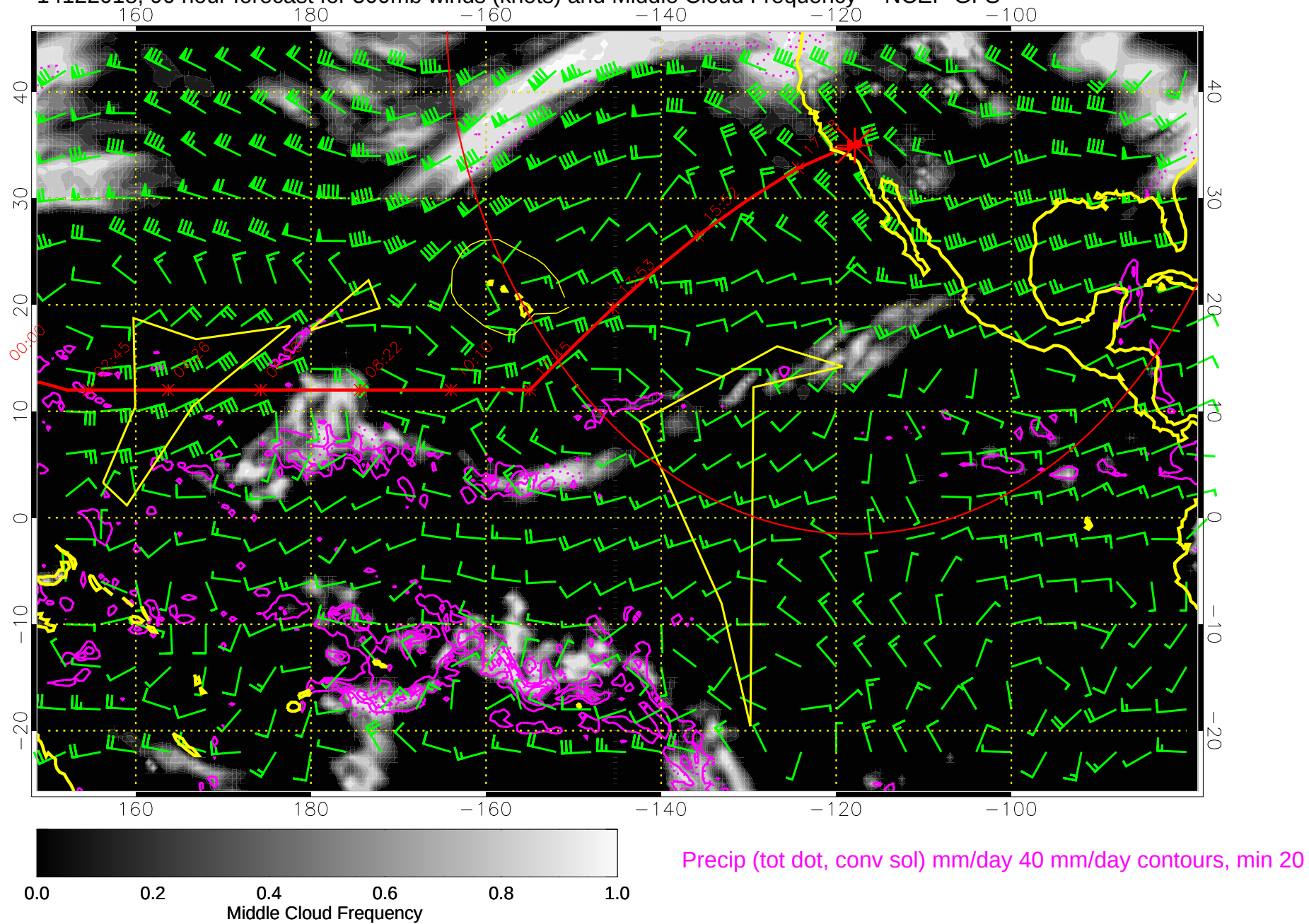
14122018, 90 hour forecast for 500mb winds (knots) and Middle Cloud Frequency -- NCEP GFS
