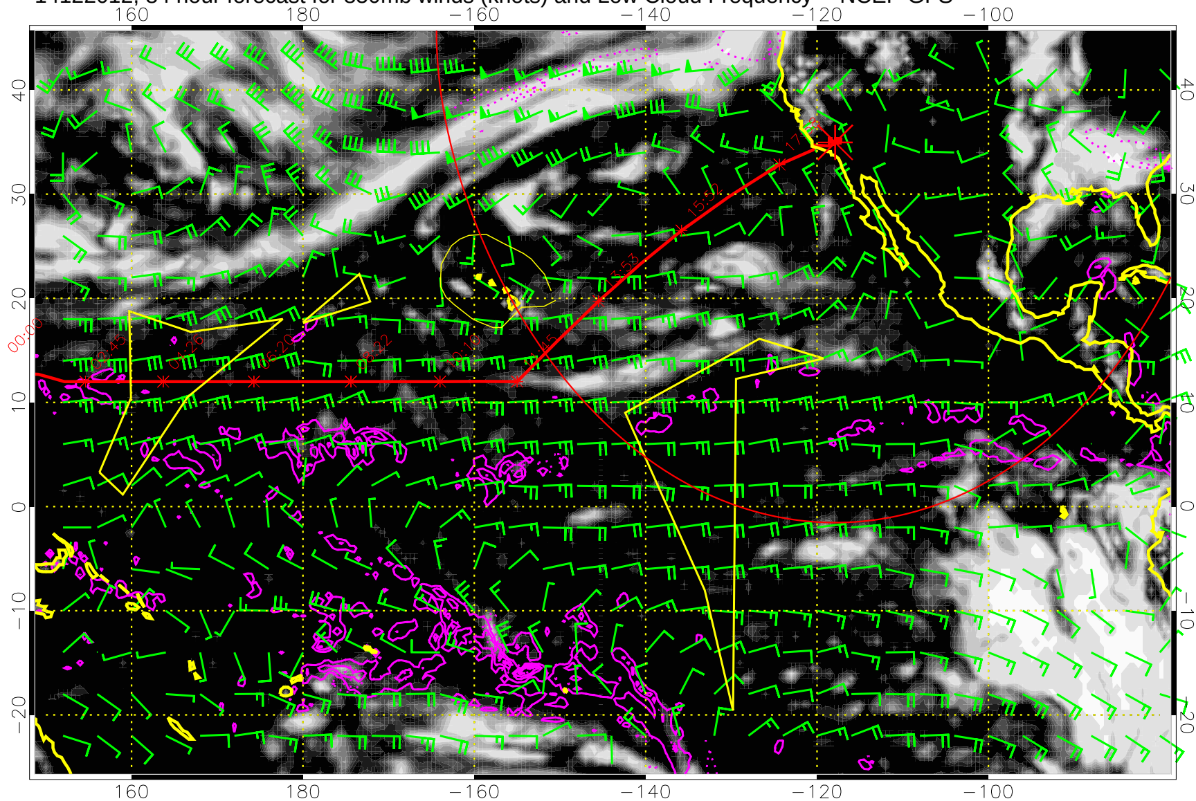
14122012, 84 hour forecast for 850mb winds (knots) and Low Cloud Frequency -- NCEP GFS
