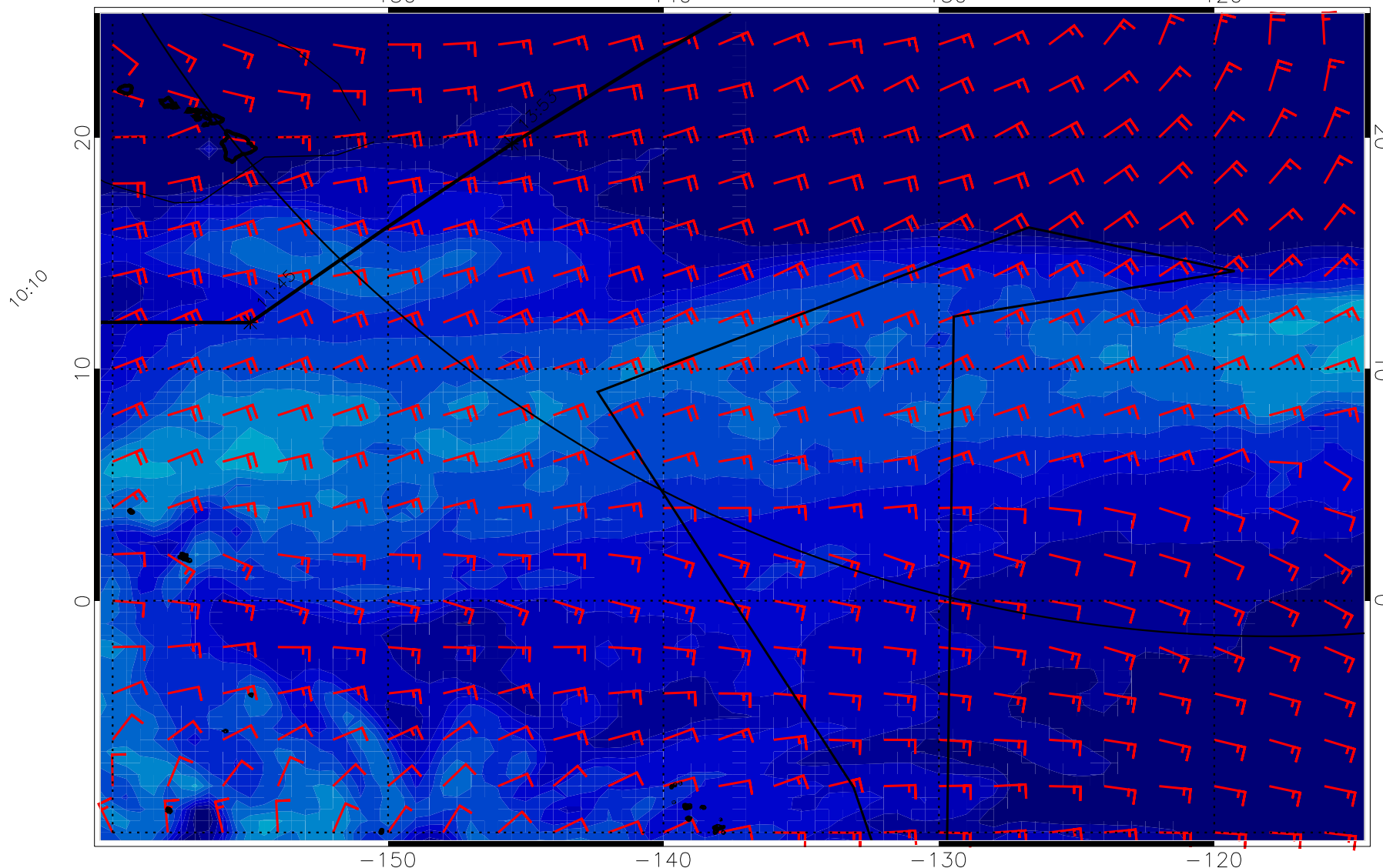
14122012, 84 hour forecast for CAPE and surface winds (knots) -- NCEP GFS
