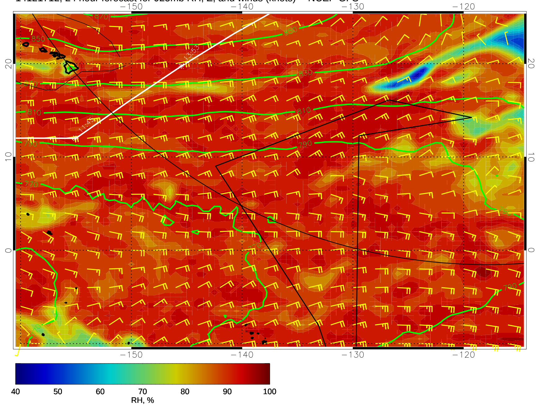
14121712, 24 hour forecast for 925mb RH, Z, and winds (knots) -- NCEP GFS
