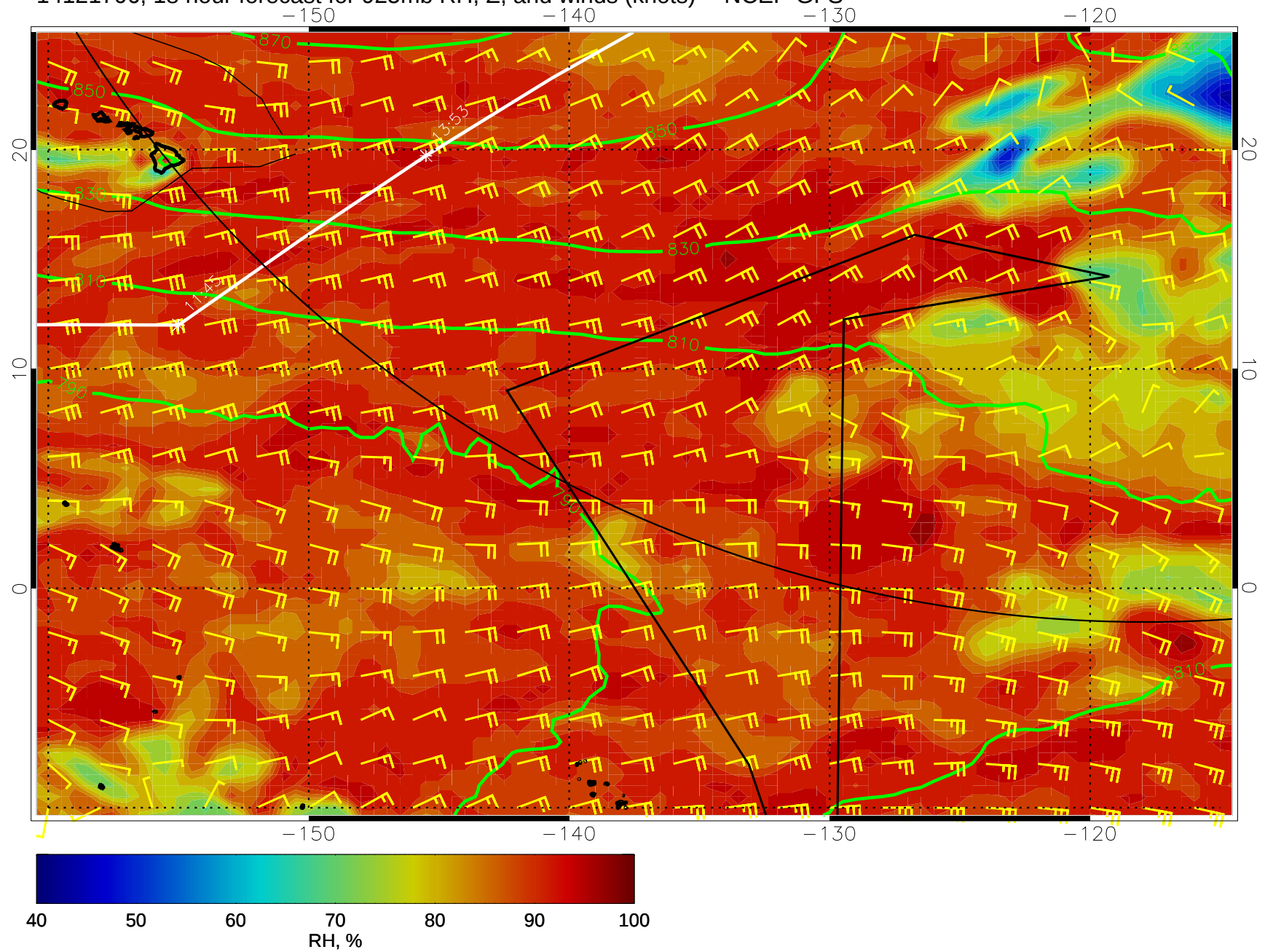
14121706, 18 hour forecast for 925mb RH, Z, and winds (knots) -- NCEP GFS
