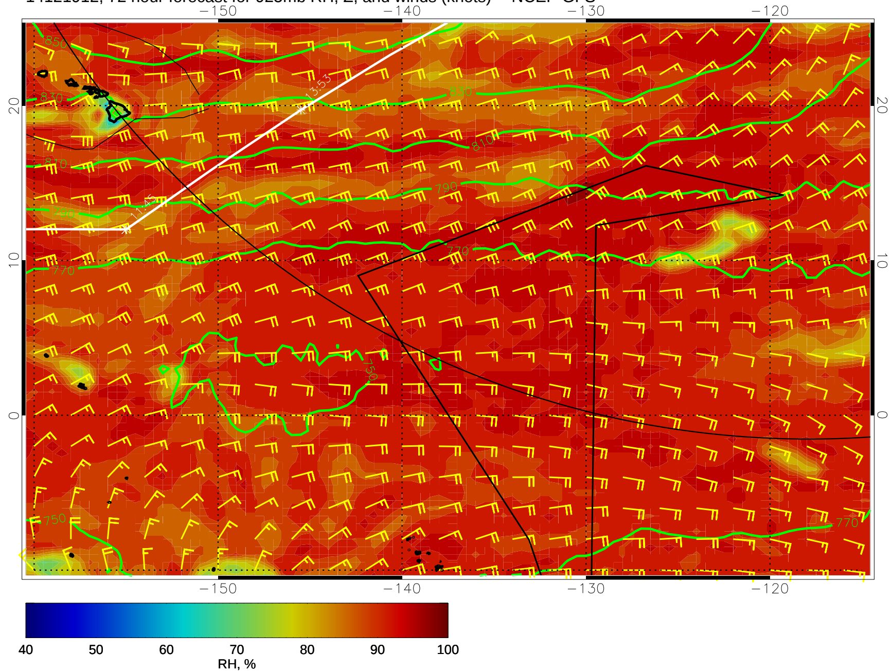
14121912, 72 hour forecast for 925mb RH, Z, and winds (knots) -- NCEP GFS
