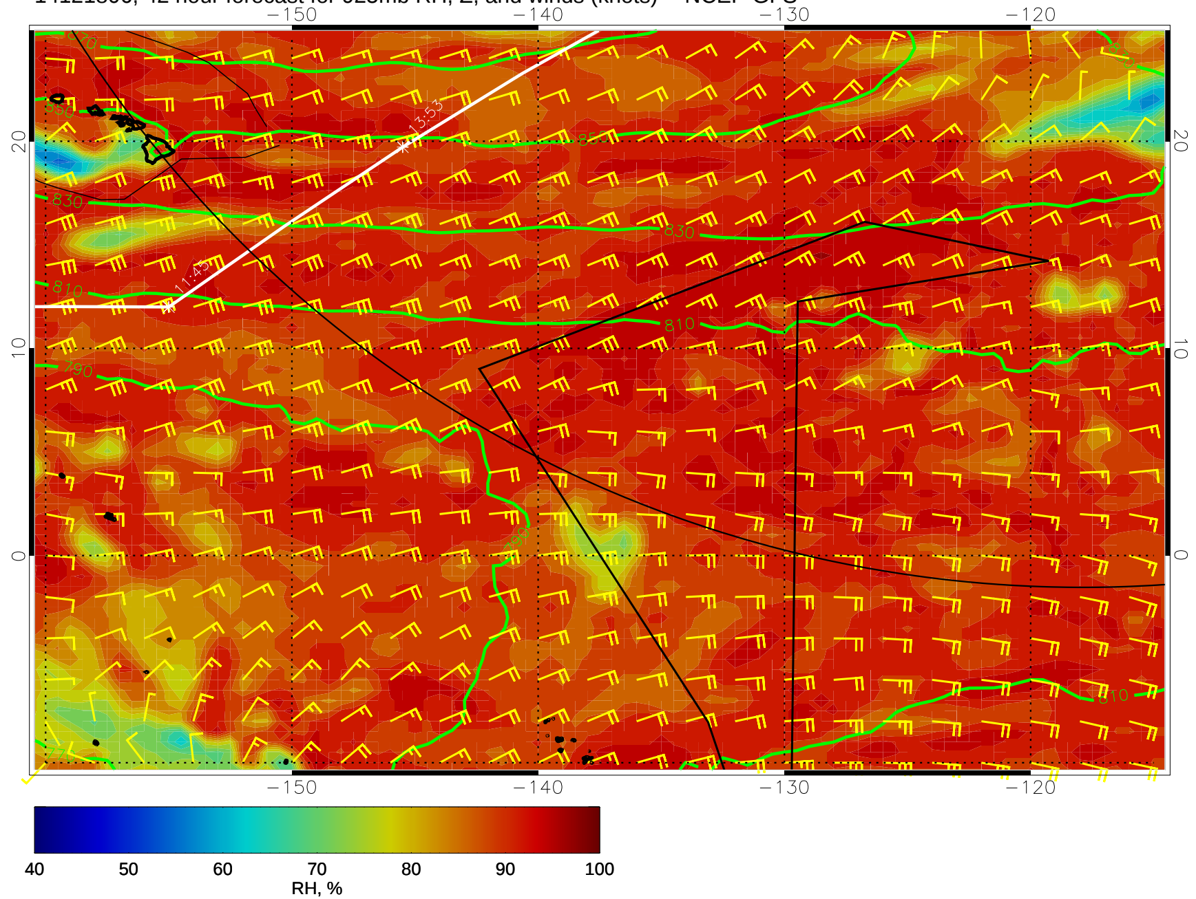
14121806, 42 hour forecast for 925mb RH, Z, and winds (knots) -- NCEP GFS
