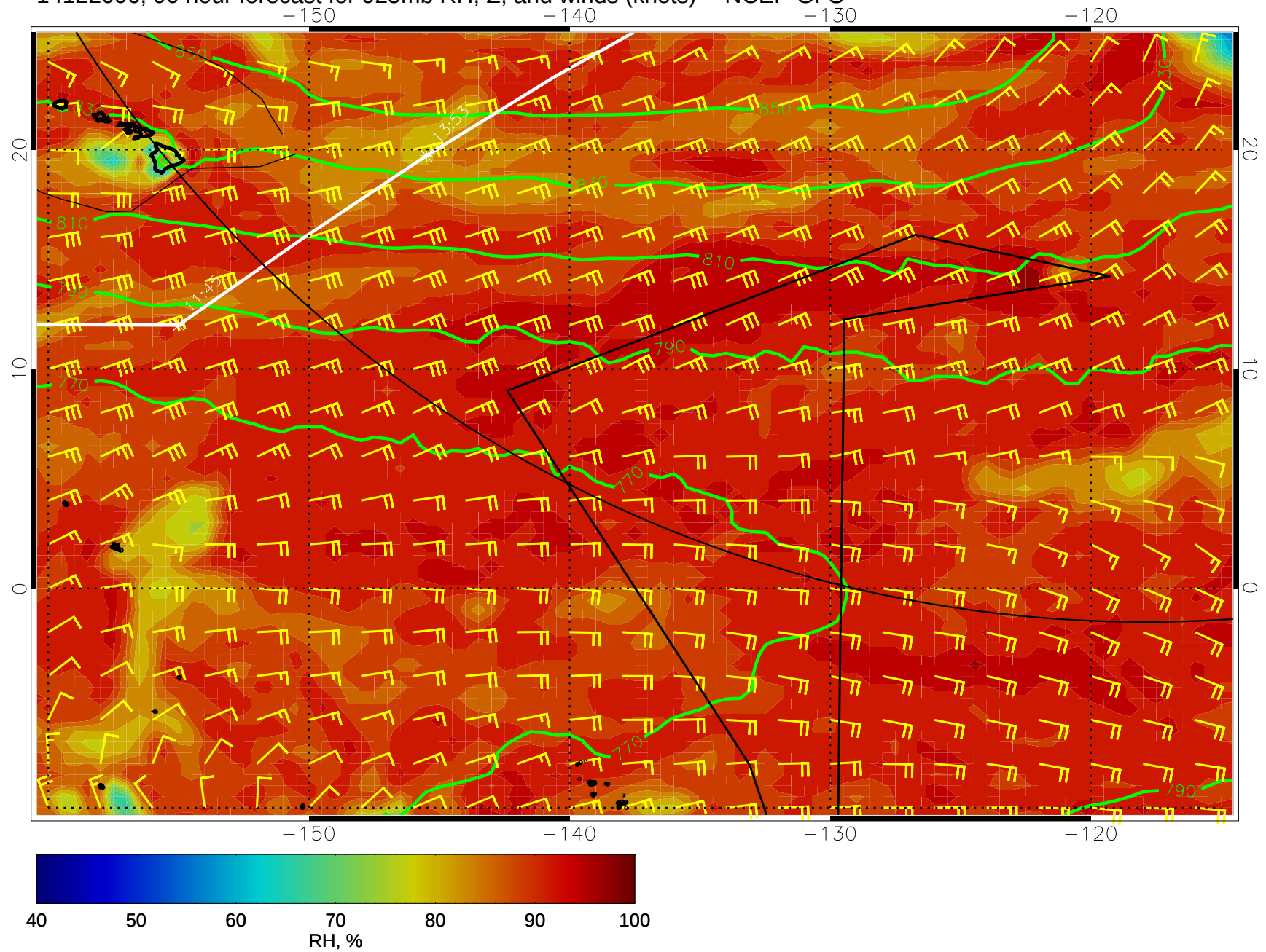
14122006, 90 hour forecast for 925mb RH, Z, and winds (knots) -- NCEP GFS
