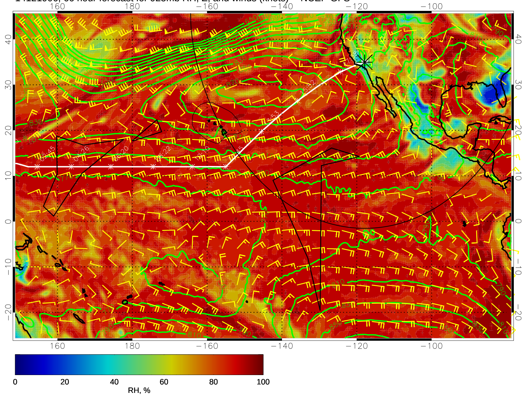
14121906, 66 hour forecast for 925mb RH, Z, and winds (knots) -- NCEP GFS
