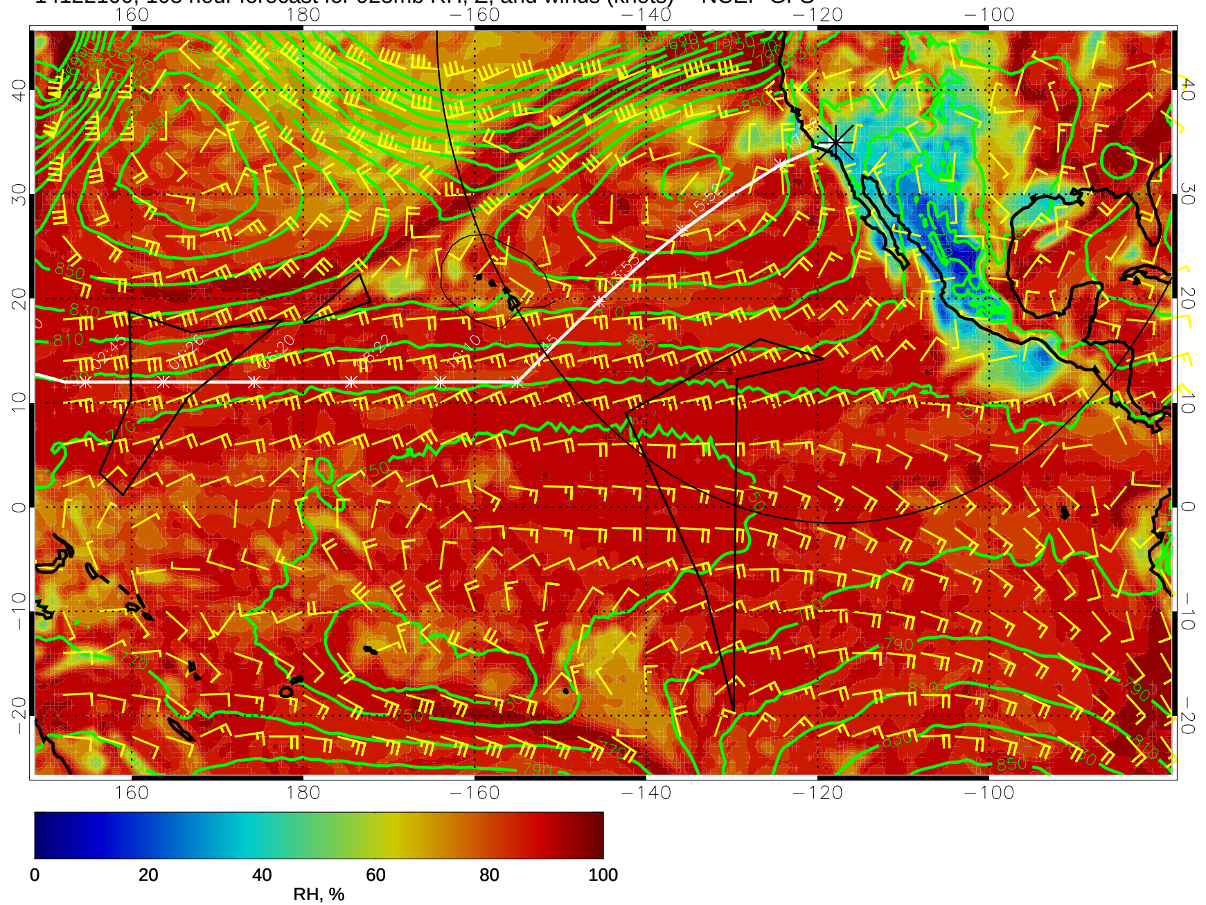
14122100, 108 hour forecast for 925mb RH, Z, and winds (knots) -- NCEP GFS
