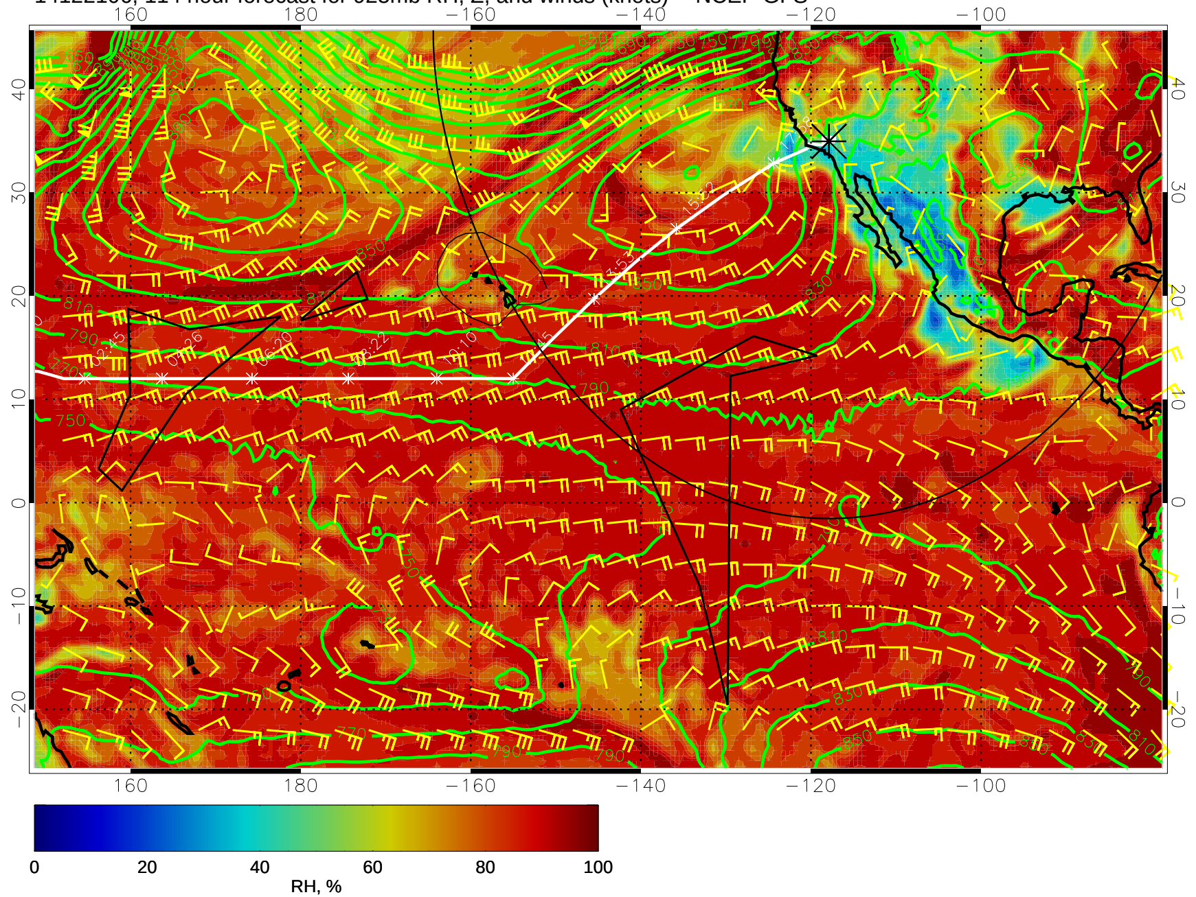
14122106, 114 hour forecast for 925mb RH, Z, and winds (knots) -- NCEP GFS
