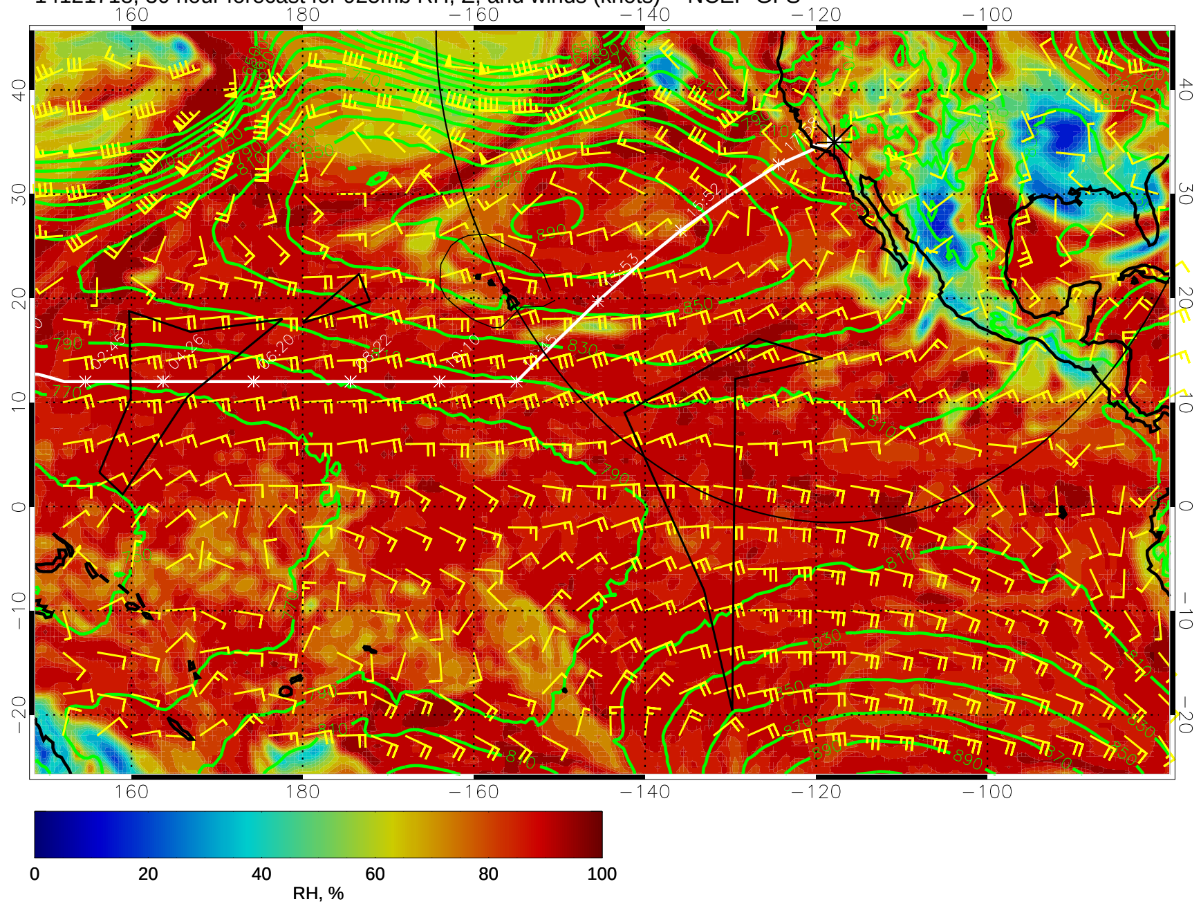
14121718, 30 hour forecast for 925mb RH, Z, and winds (knots) -- NCEP GFS
