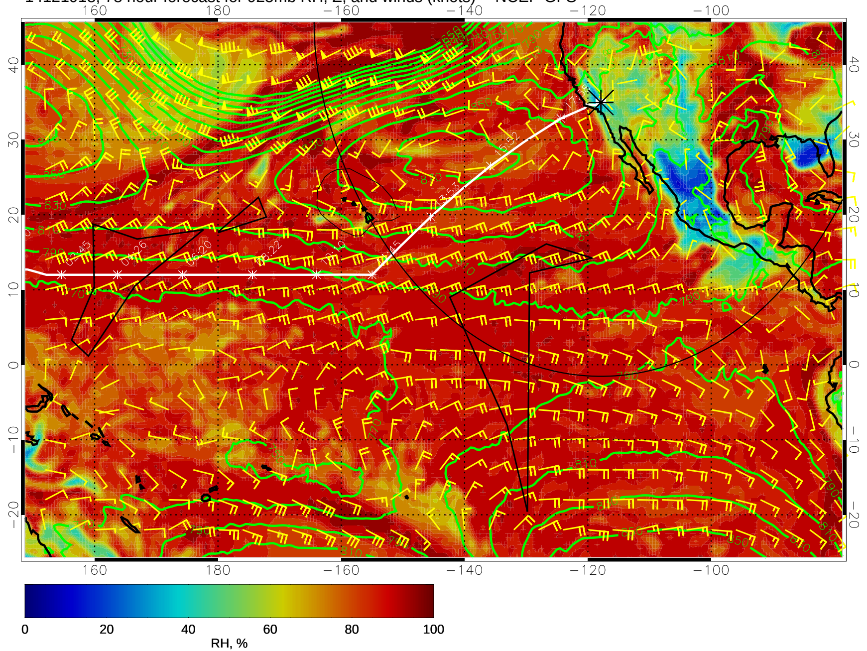
14121918, 78 hour forecast for 925mb RH, Z, and winds (knots) -- NCEP GFS
