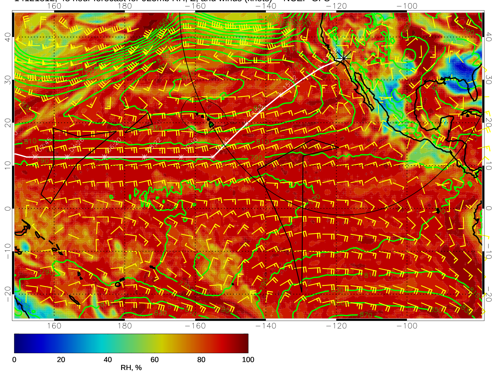
14121812, 48 hour forecast for 925mb RH, Z, and winds (knots) -- NCEP GFS
