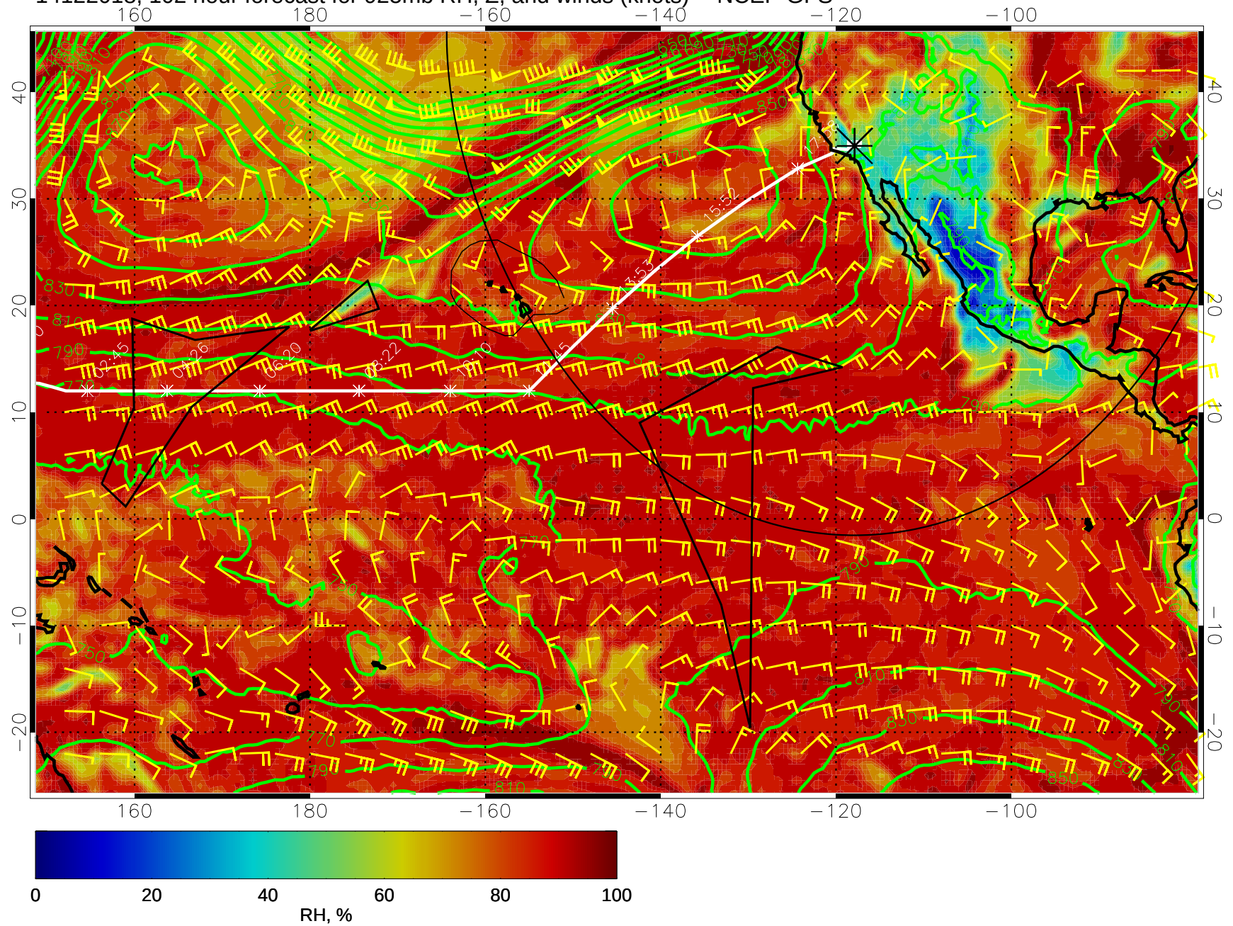
14122018, 102 hour forecast for 925mb RH, Z, and winds (knots) -- NCEP GFS
