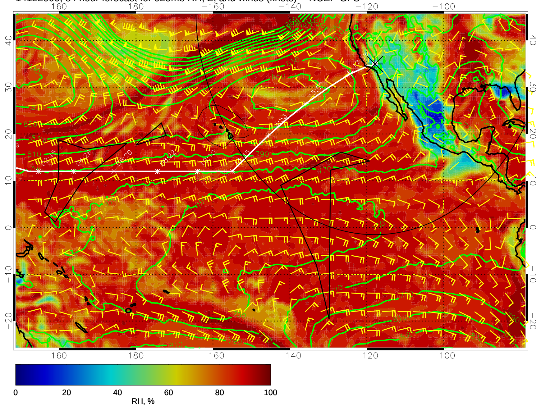
14122000, 84 hour forecast for 925mb RH, Z, and winds (knots) -- NCEP GFS
