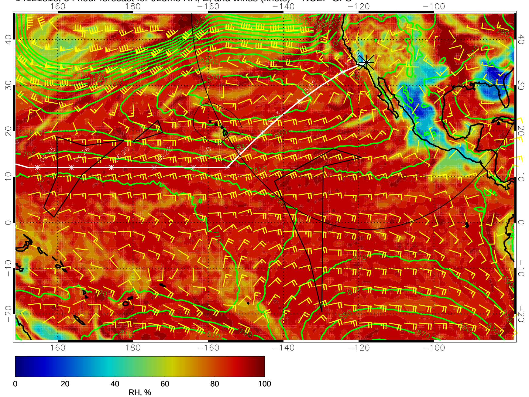
14121818, 54 hour forecast for 925mb RH, Z, and winds (knots) -- NCEP GFS
