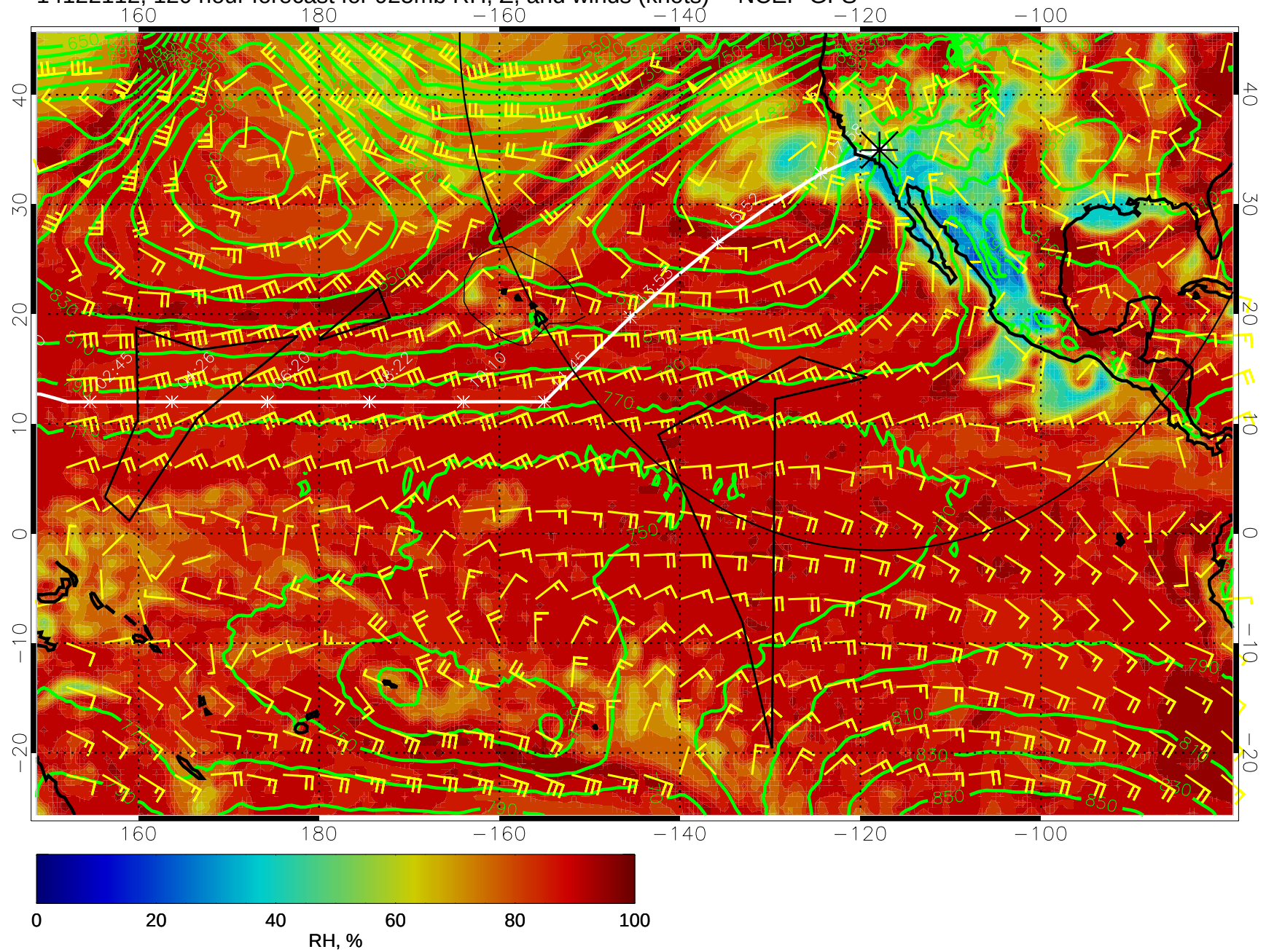
14122112, 120 hour forecast for 925mb RH, Z, and winds (knots) -- NCEP GFS
