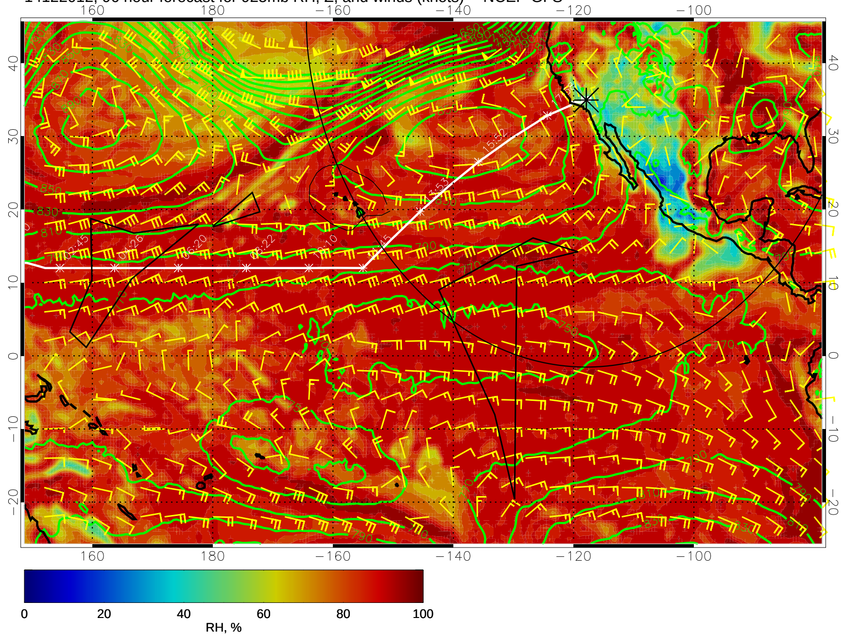
14122012, 96 hour forecast for 925mb RH, Z, and winds (knots) -- NCEP GFS
