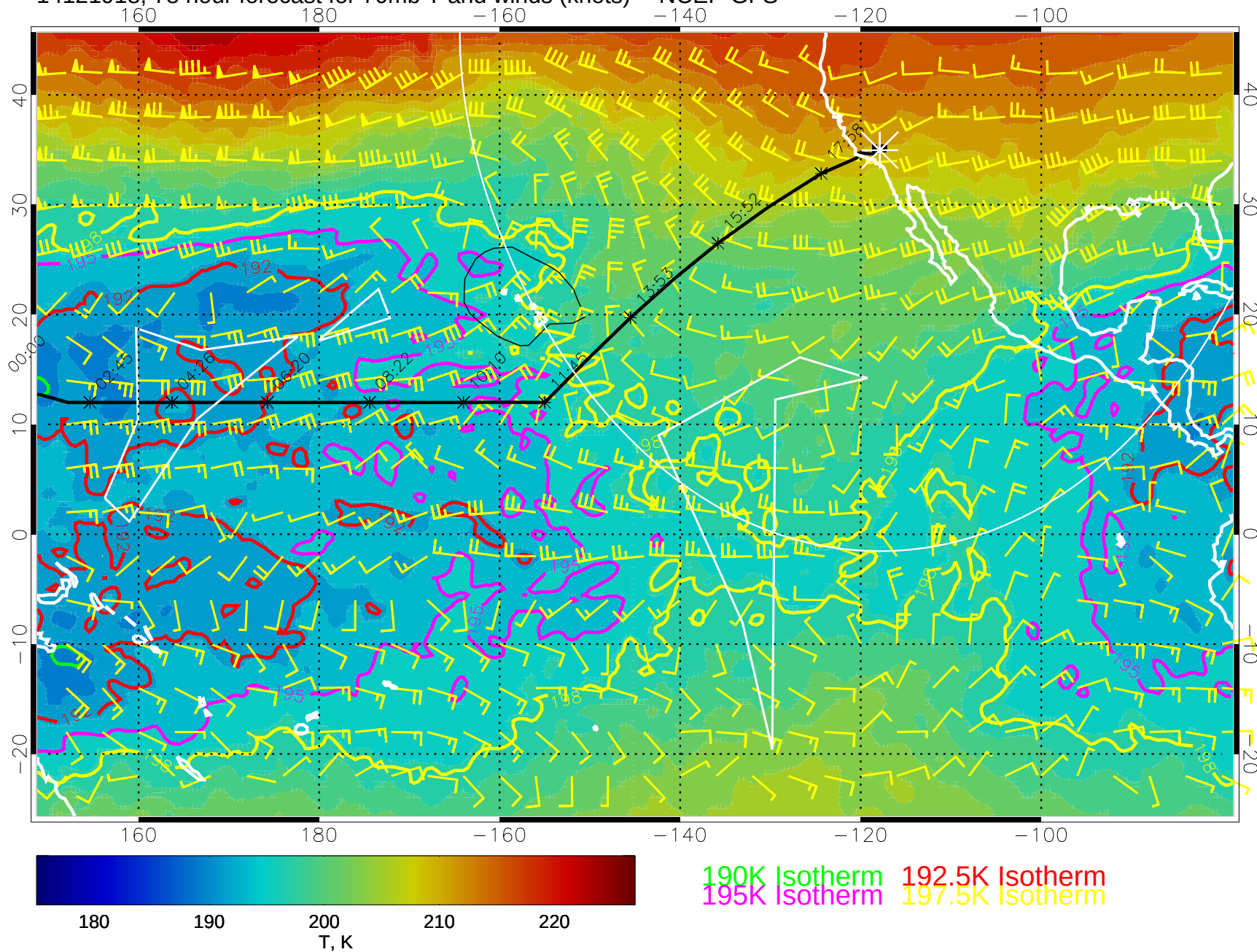
14121918, 78 hour forecast for 70mb T and winds (knots) -- NCEP GFS
