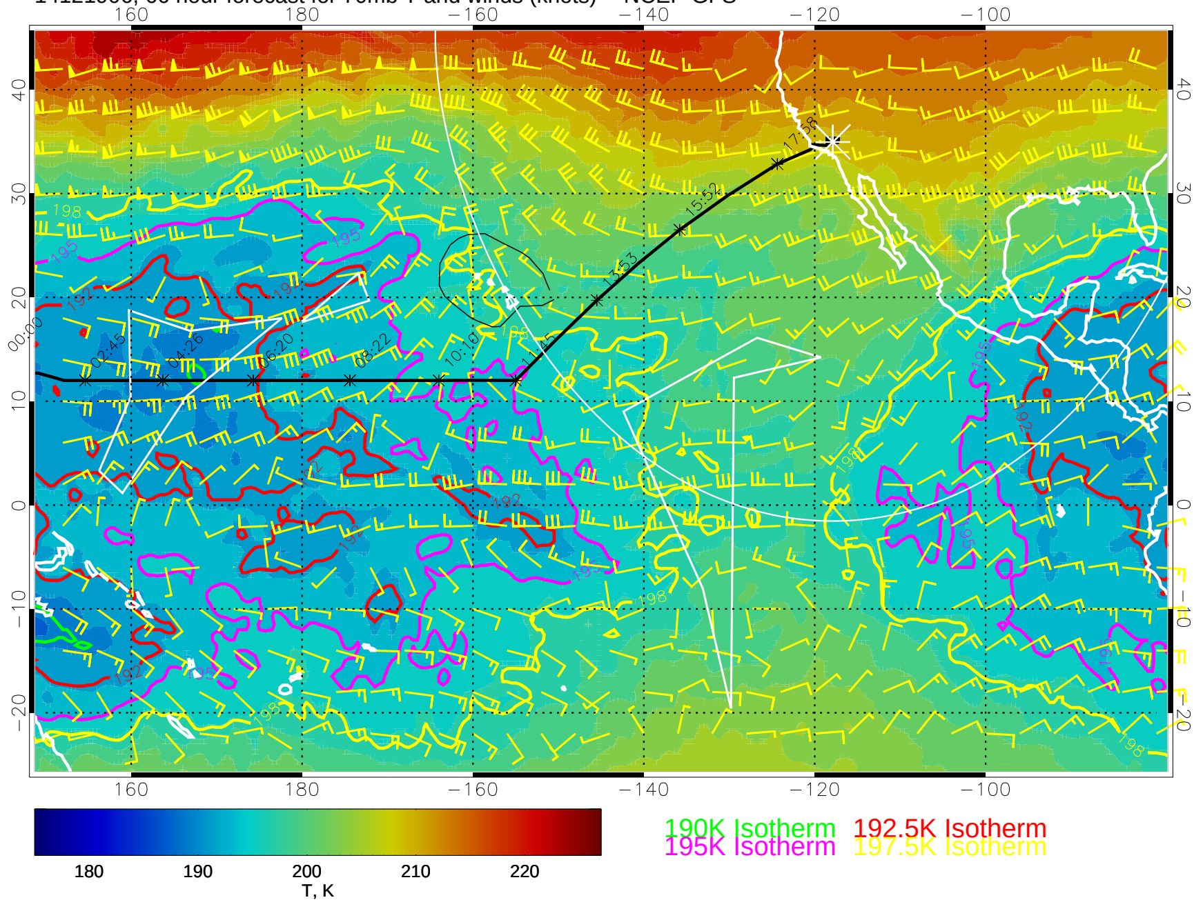
14121906, 66 hour forecast for 70mb T and winds (knots) -- NCEP GFS
