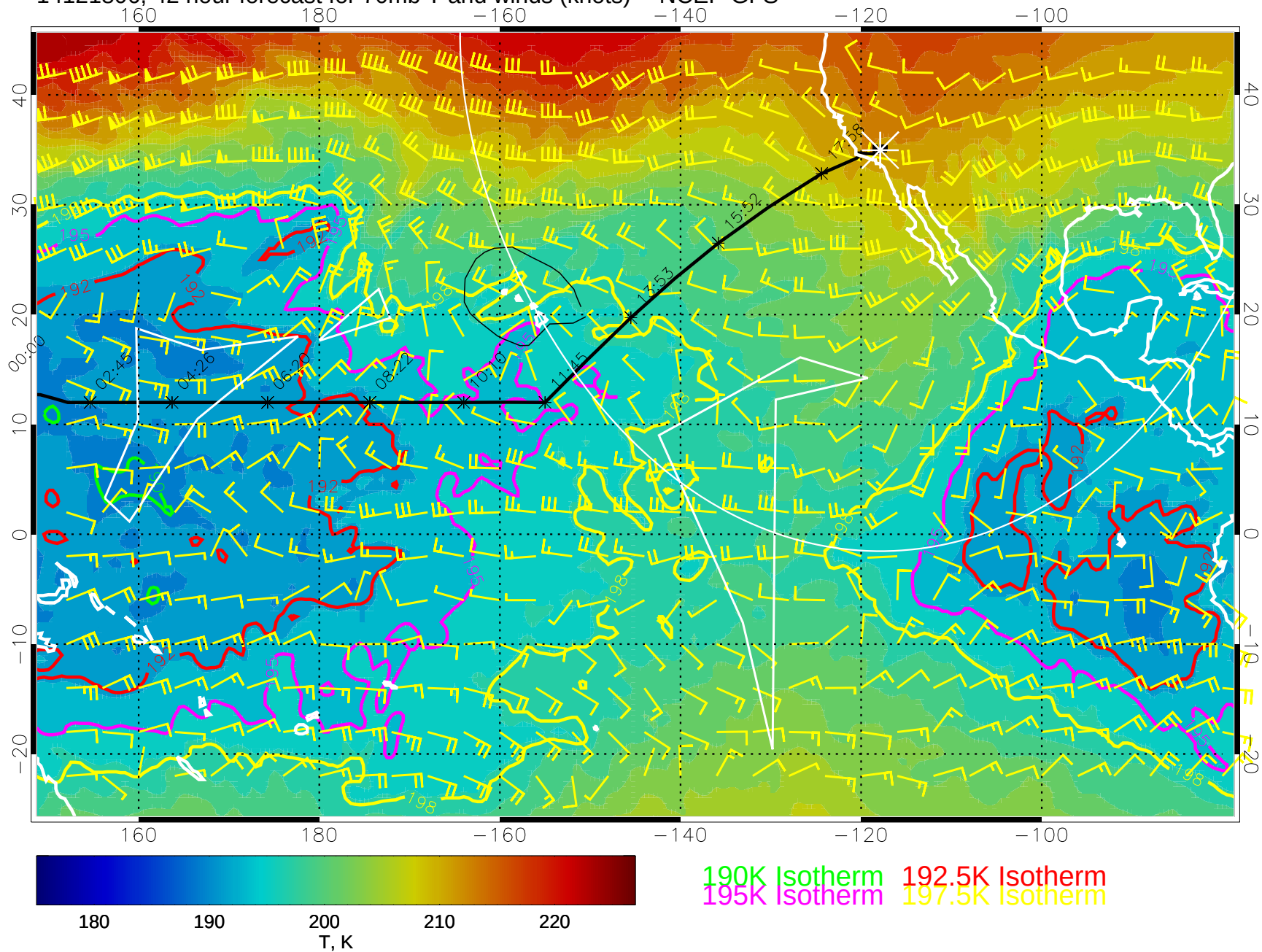
14121806, 42 hour forecast for 70mb T and winds (knots) -- NCEP GFS
