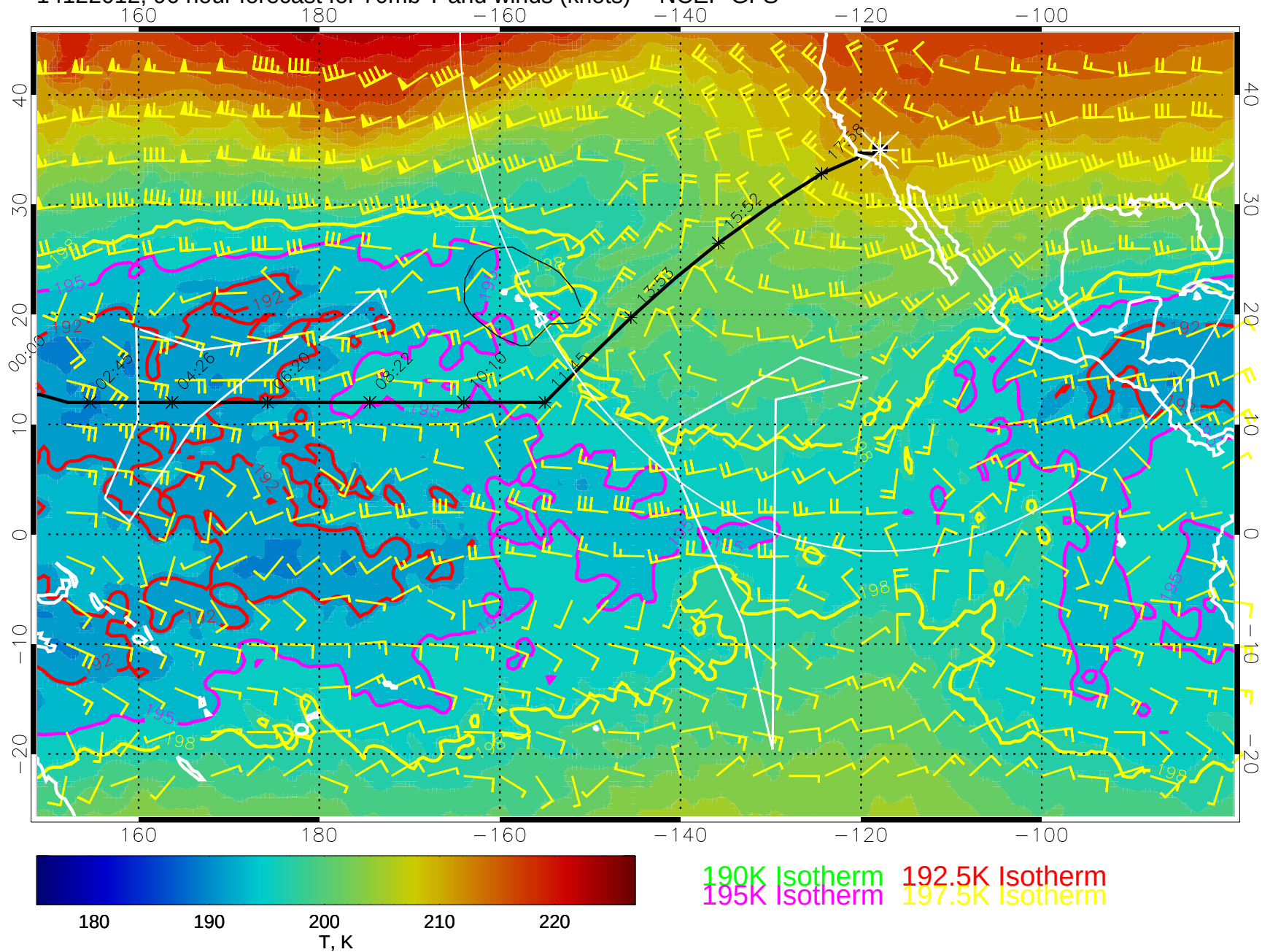
14122012, 96 hour forecast for 70mb T and winds (knots) -- NCEP GFS
