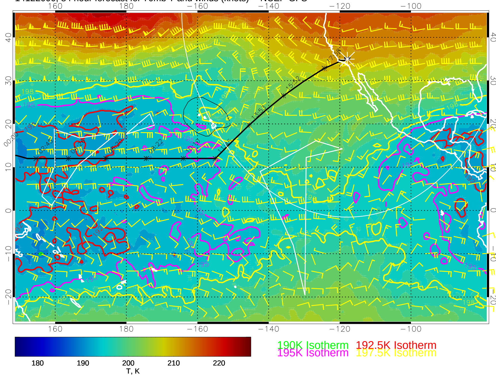
14122000, 84 hour forecast for 70mb T and winds (knots) -- NCEP GFS
