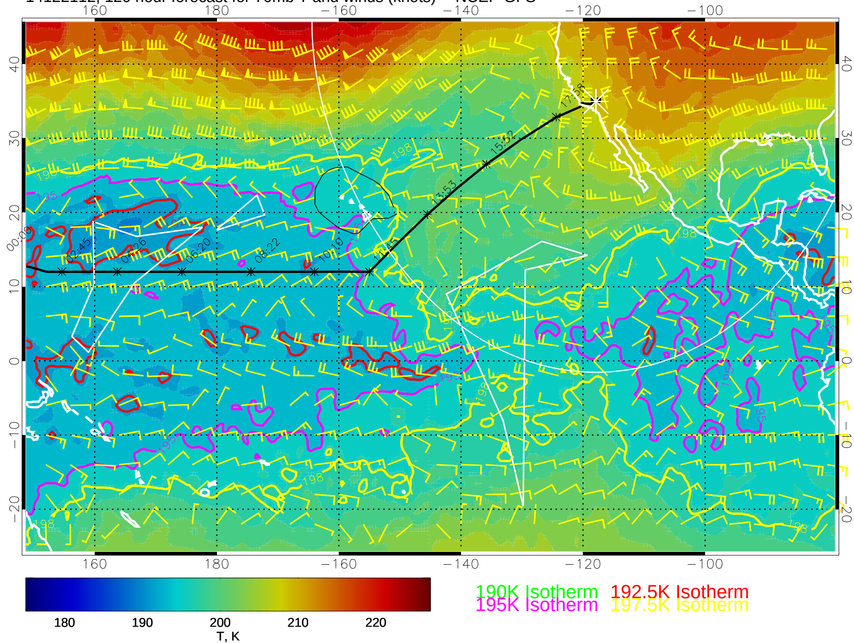
14122112, 120 hour forecast for 70mb T and winds (knots) -- NCEP GFS
