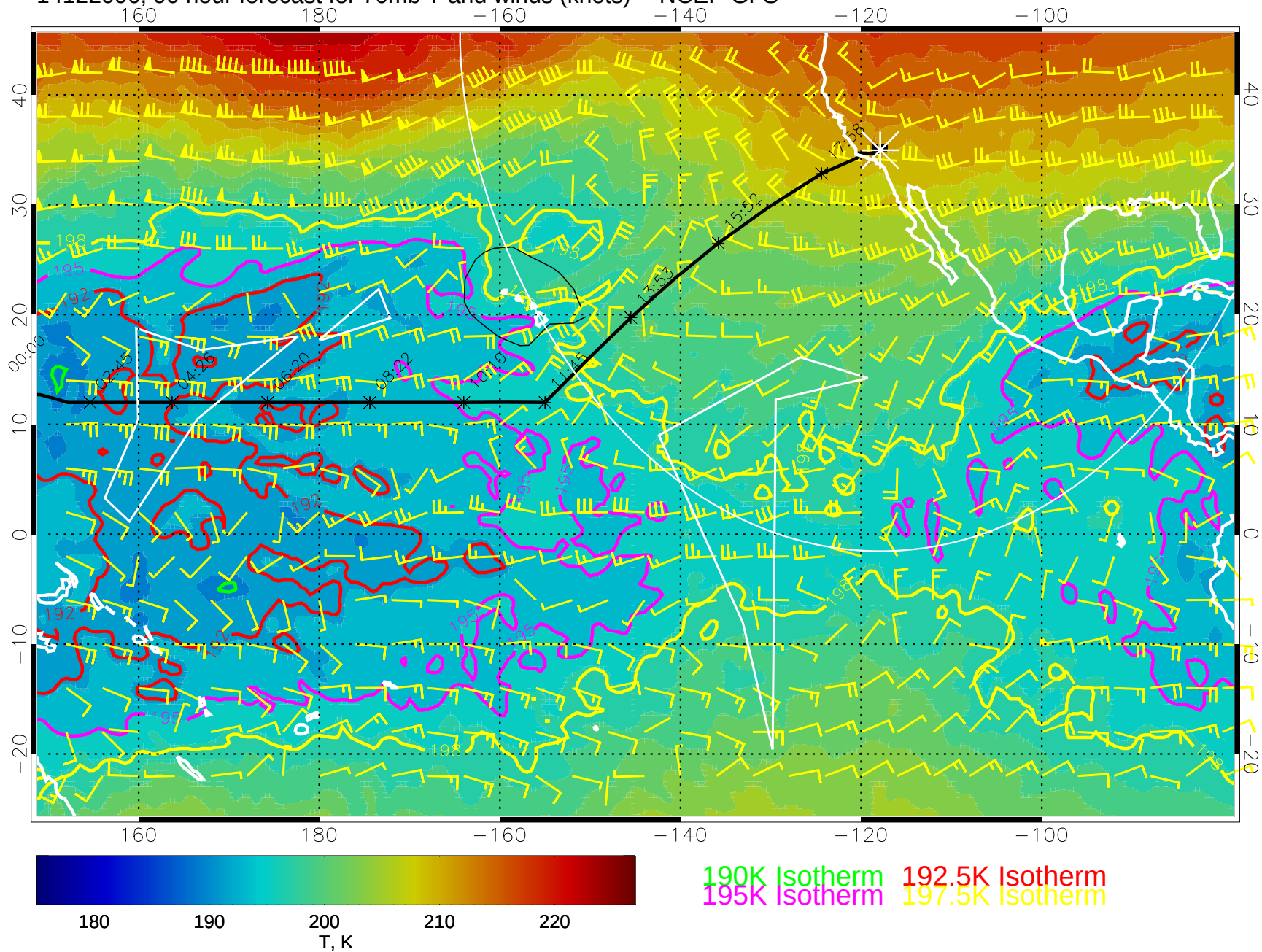
14122006, 90 hour forecast for 70mb T and winds (knots) -- NCEP GFS
