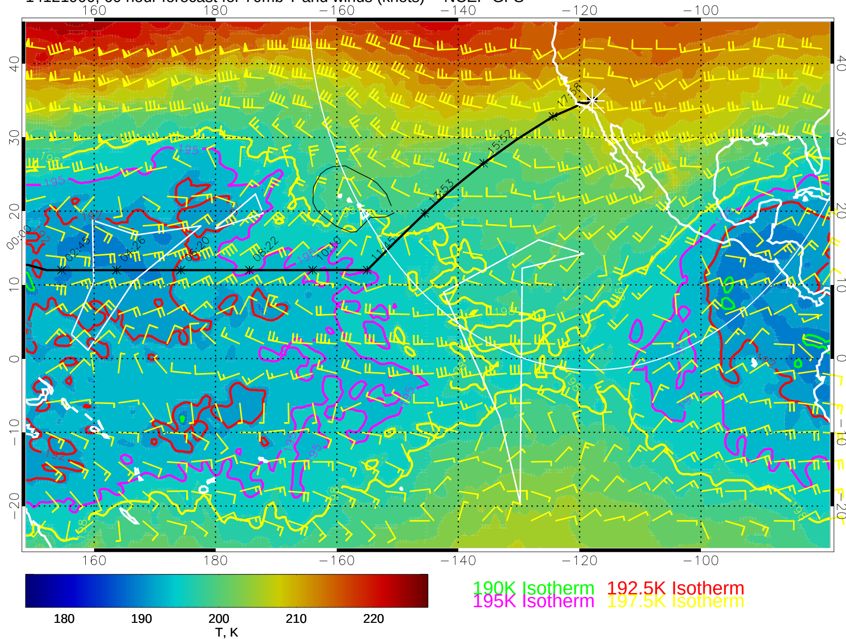
14121900, 60 hour forecast for 70mb T and winds (knots) -- NCEP GFS
