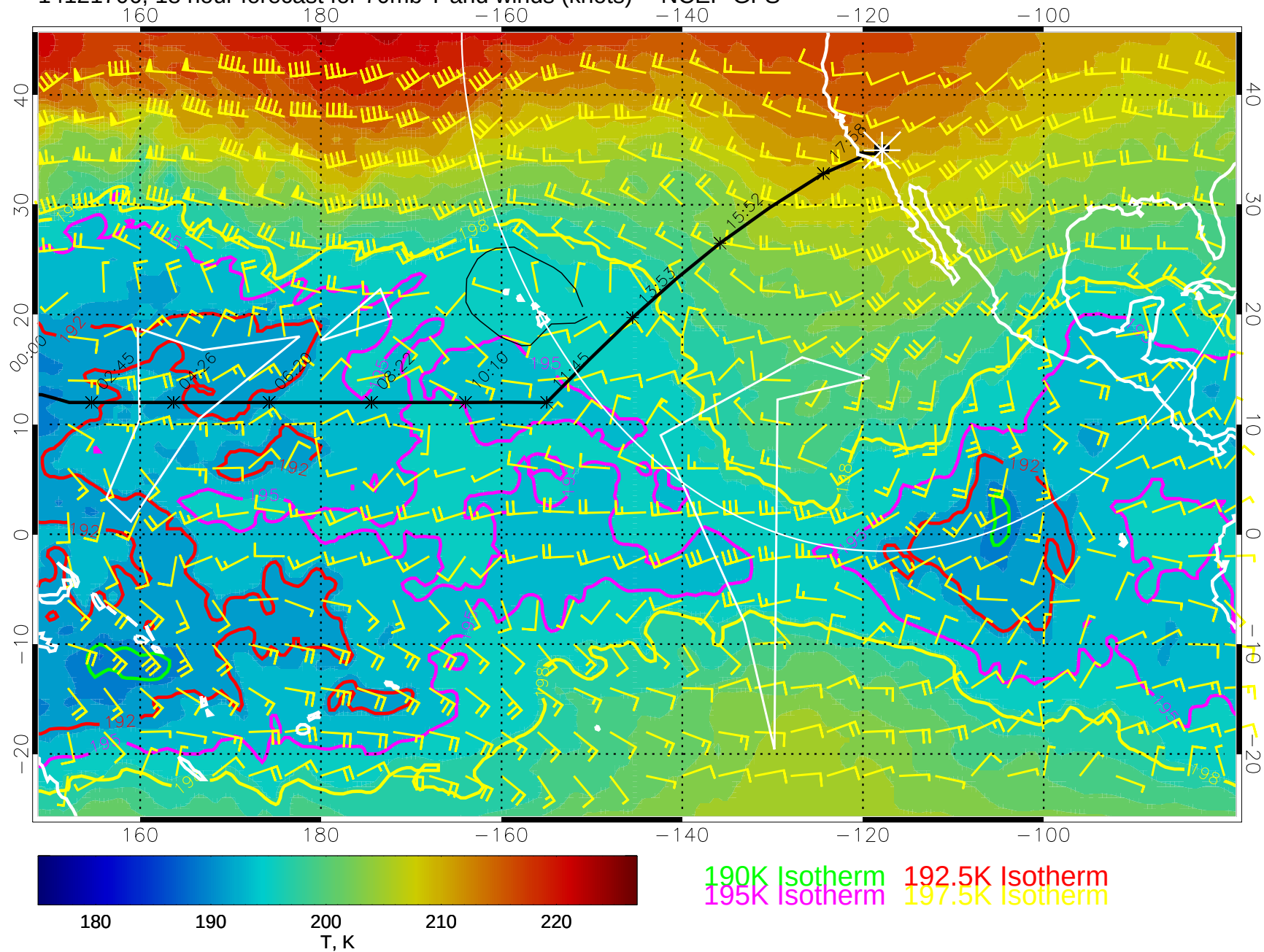
14121706, 18 hour forecast for 70mb T and winds (knots) -- NCEP GFS
