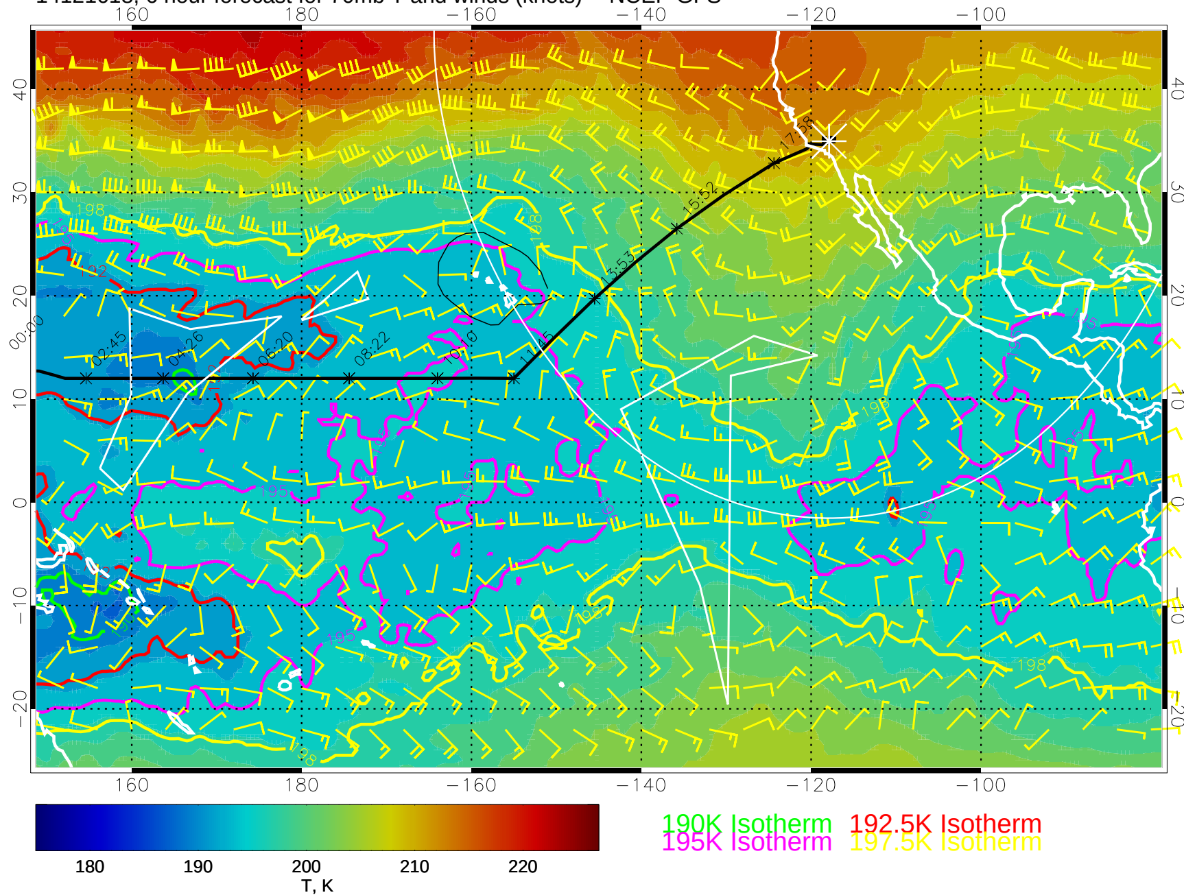
14121618, 6 hour forecast for 70mb T and winds (knots) -- NCEP GFS
