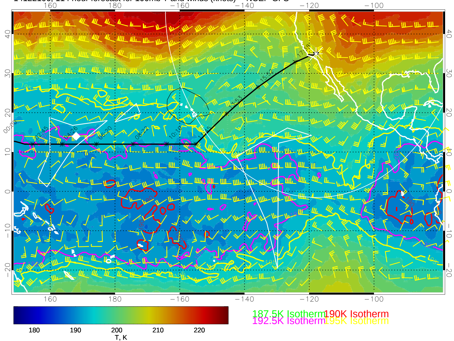
14122106, 114 hour forecast for 100mb T and winds (knots) -- NCEP GFS
