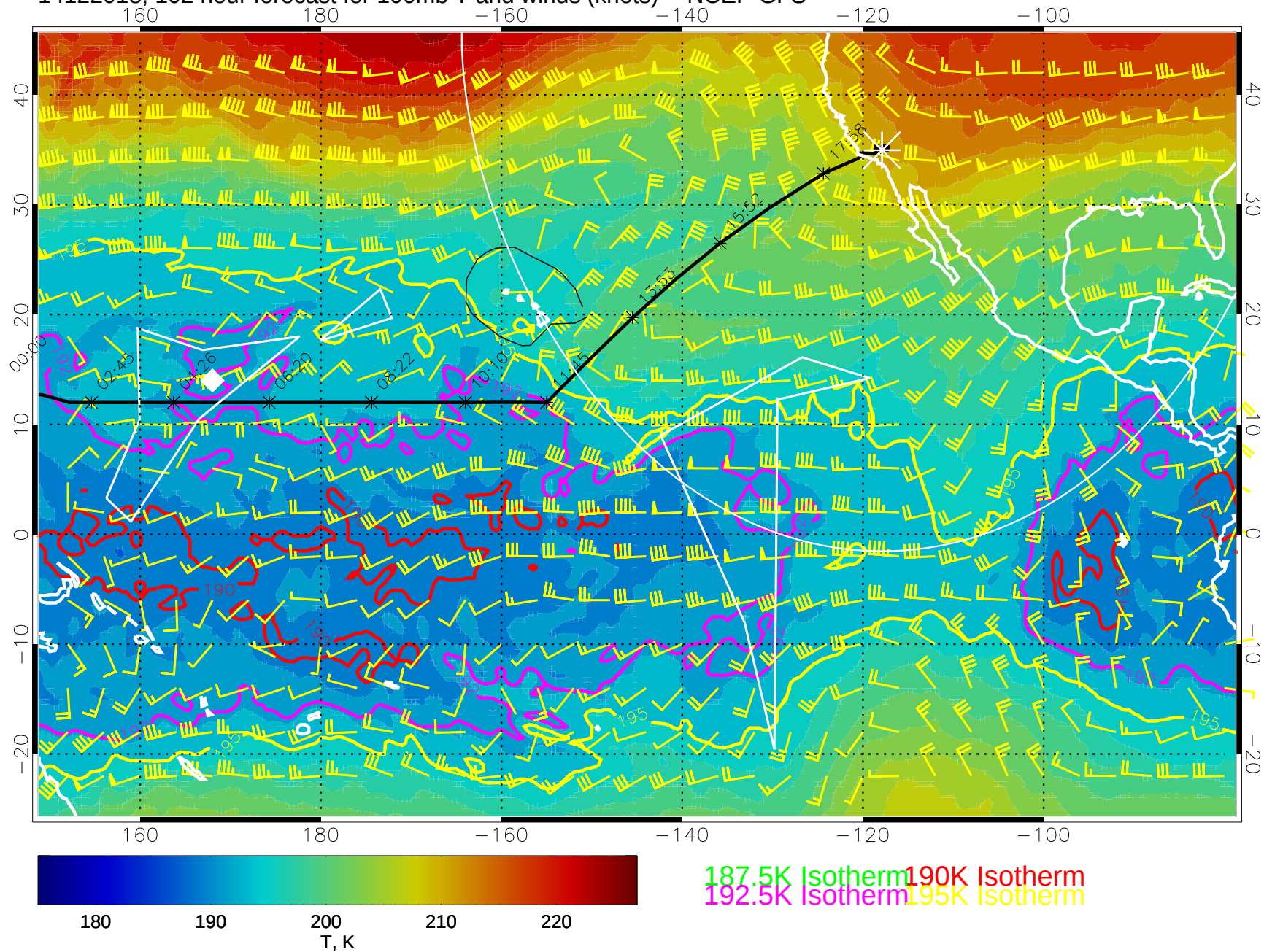
14122018, 102 hour forecast for 100mb T and winds (knots) -- NCEP GFS
