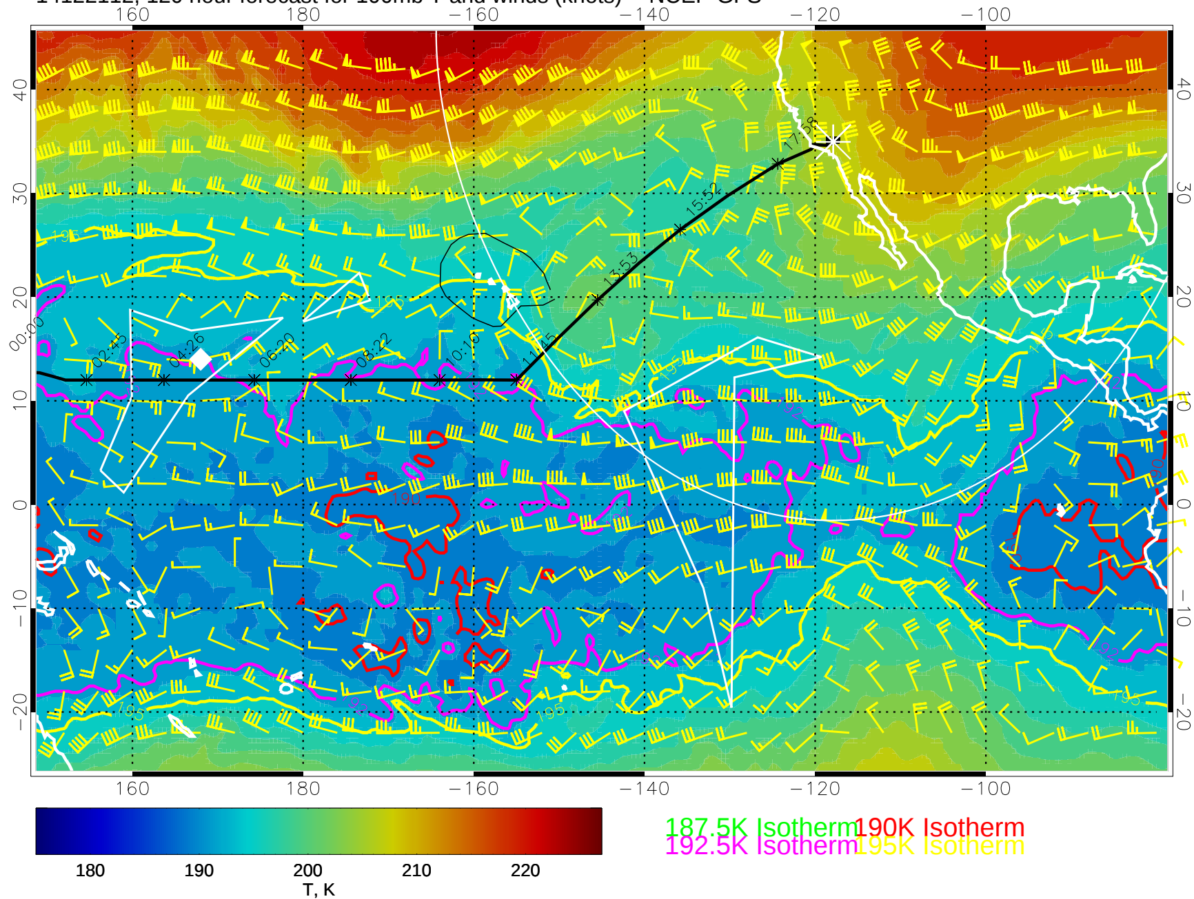
14122112, 120 hour forecast for 100mb T and winds (knots) -- NCEP GFS
