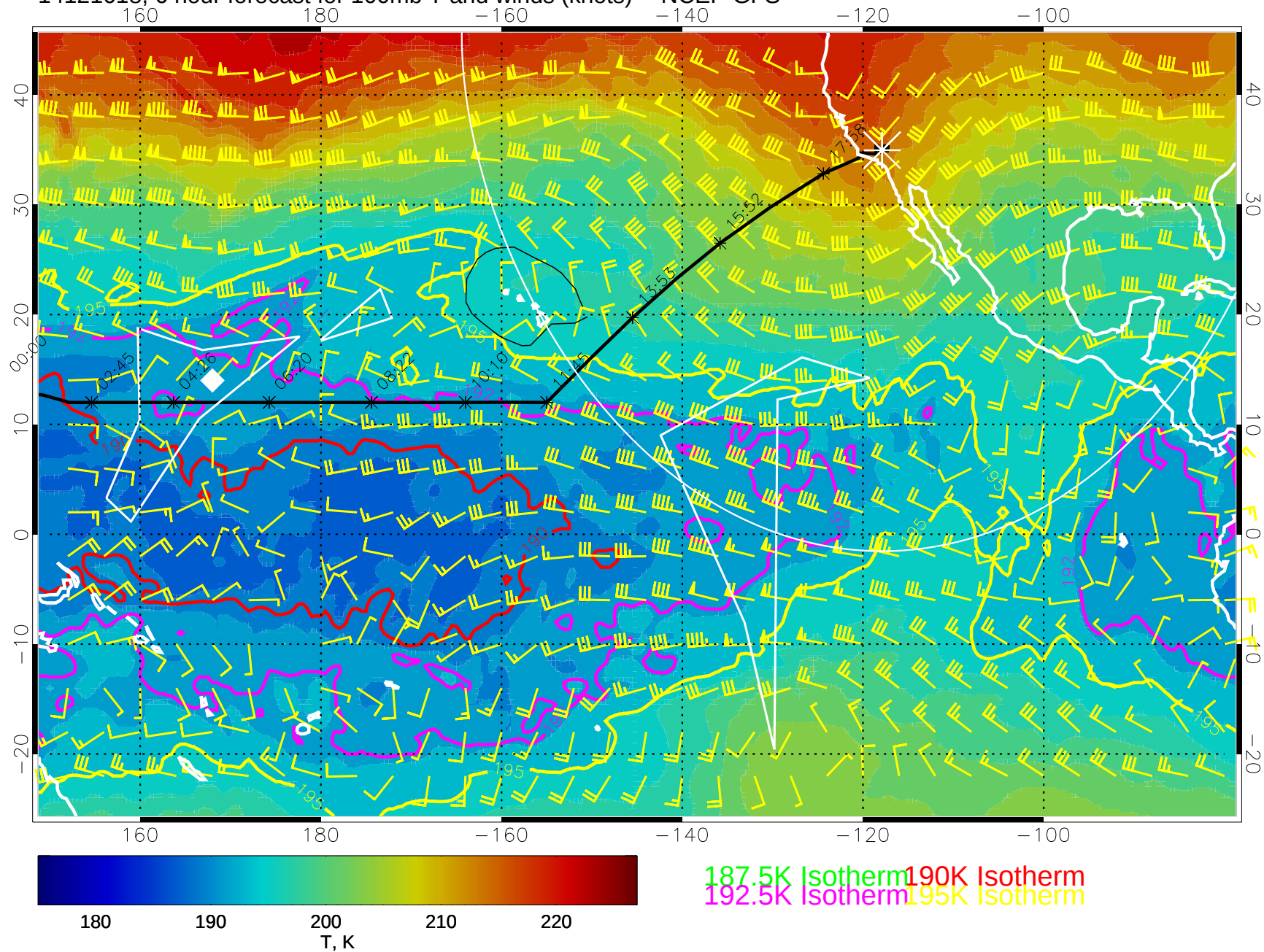
14121618, 6 hour forecast for 100mb T and winds (knots) -- NCEP GFS
