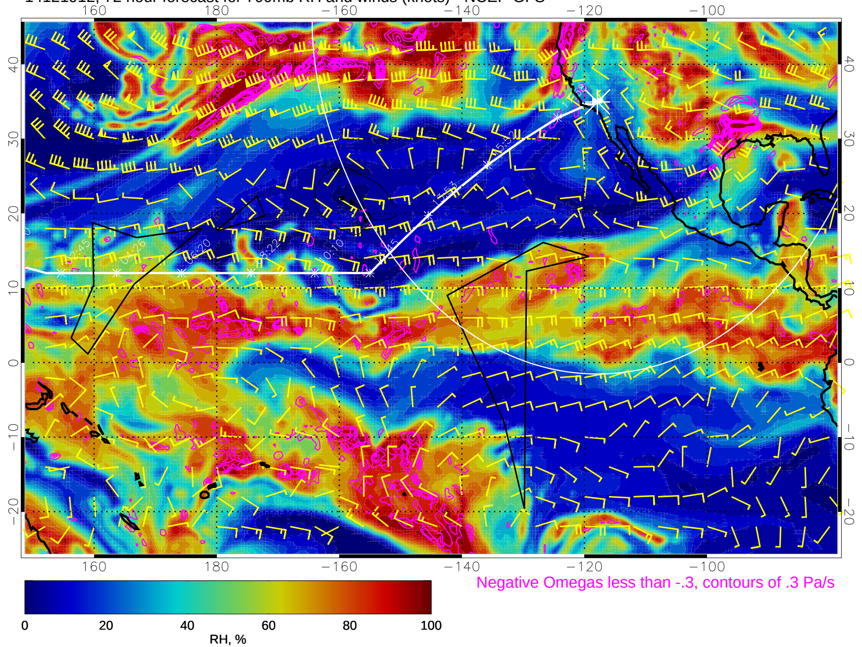
14121912, 72 hour forecast for 700mb RH and winds (knots) - NCEP GFS
