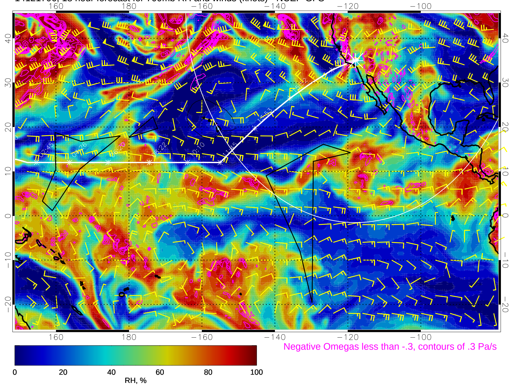
14121706, 18 hour forecast for 700mb RH and winds (knots) - NCEP GFS
