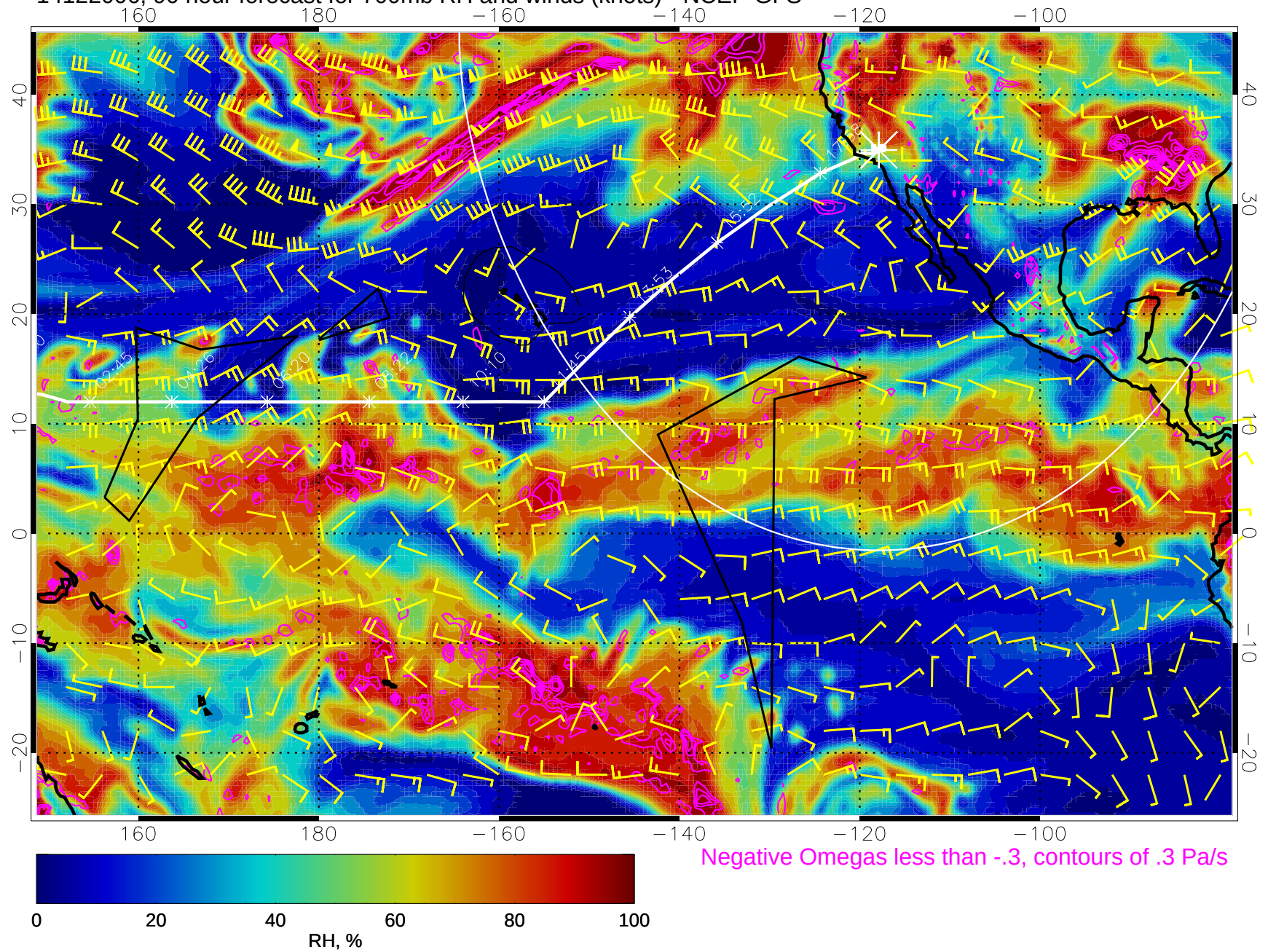
14122006, 90 hour forecast for 700mb RH and winds (knots) - NCEP GFS
