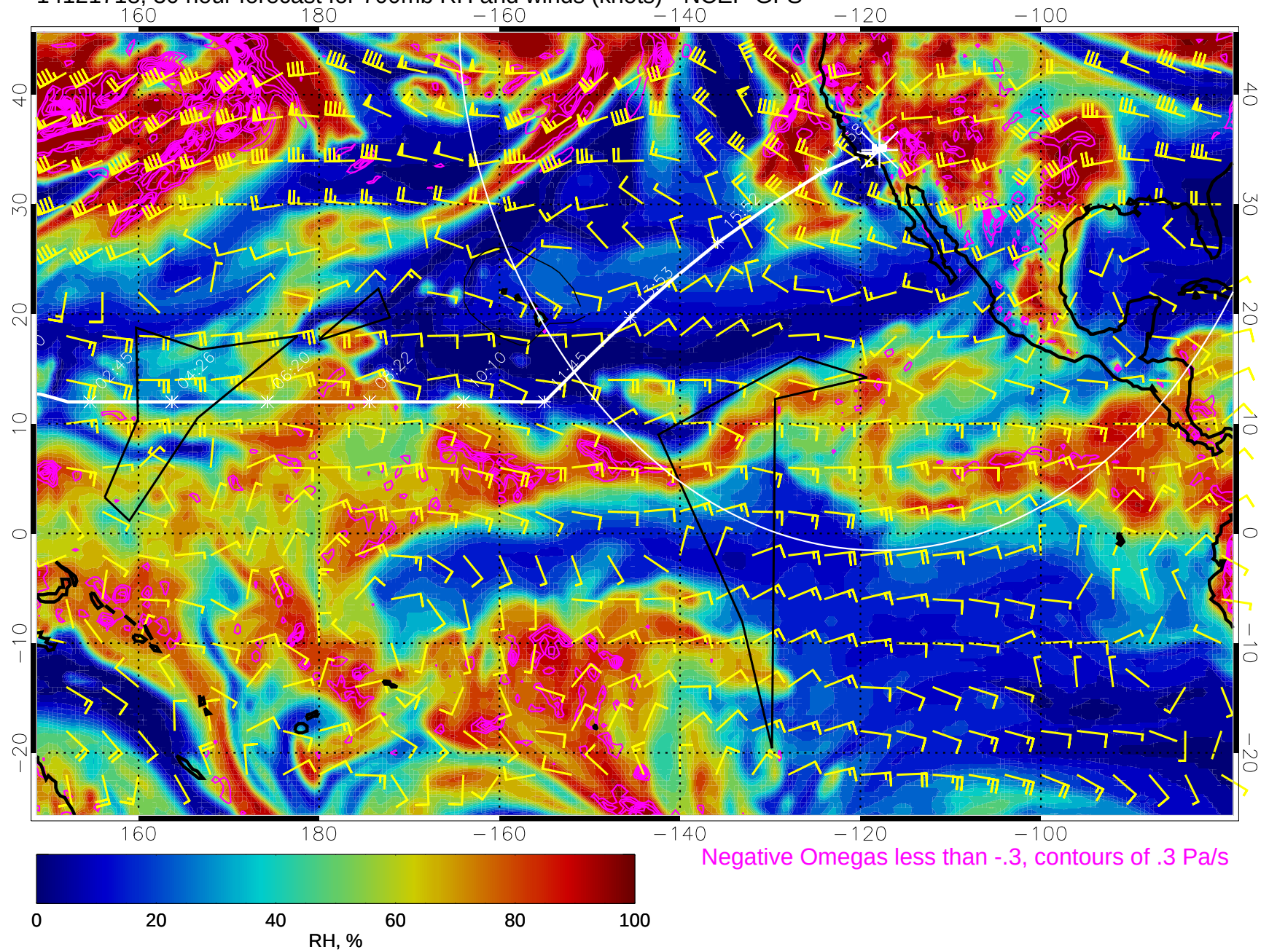
14121718, 30 hour forecast for 700mb RH and winds (knots) - NCEP GFS
