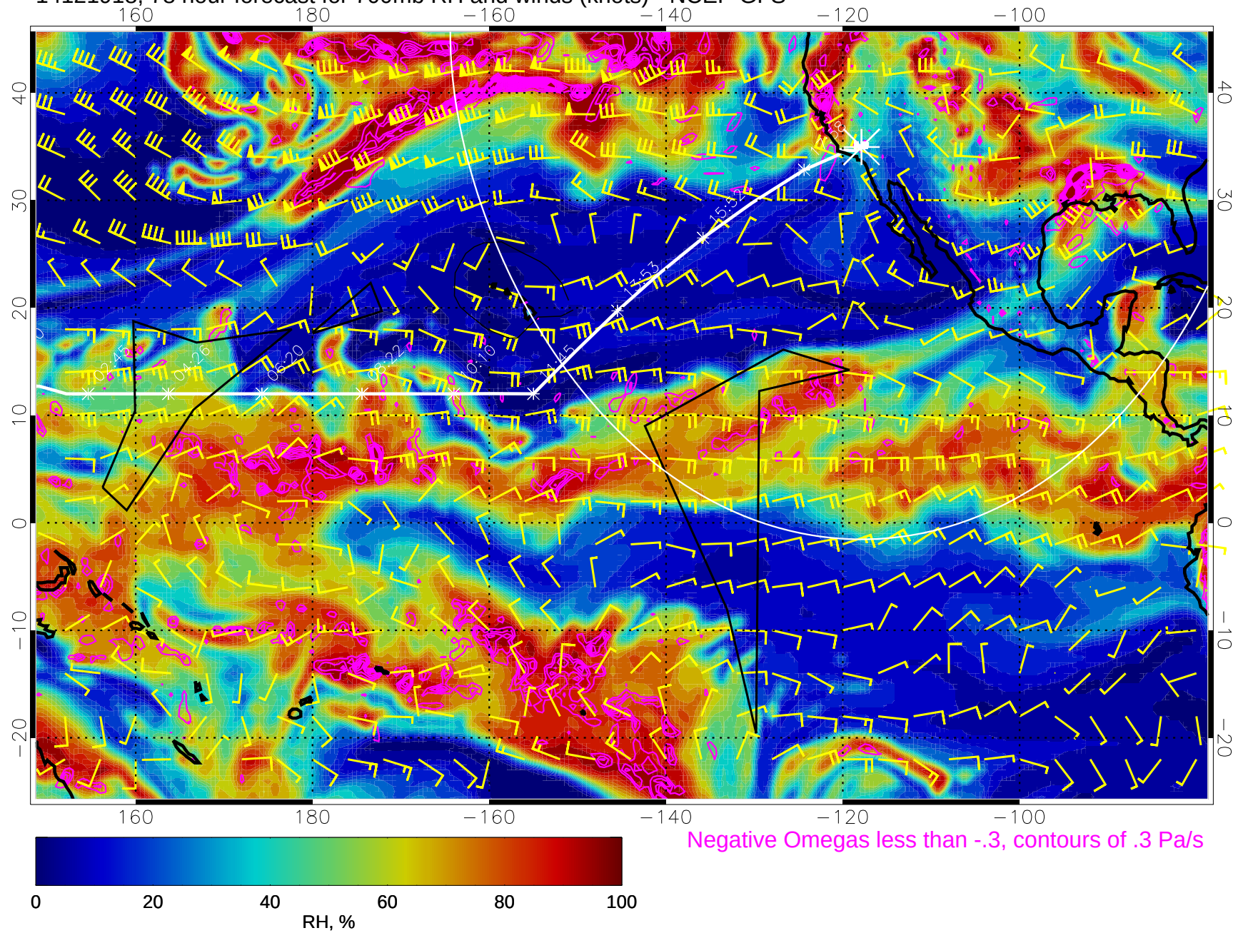
14121918, 78 hour forecast for 700mb RH and winds (knots) - NCEP GFS
