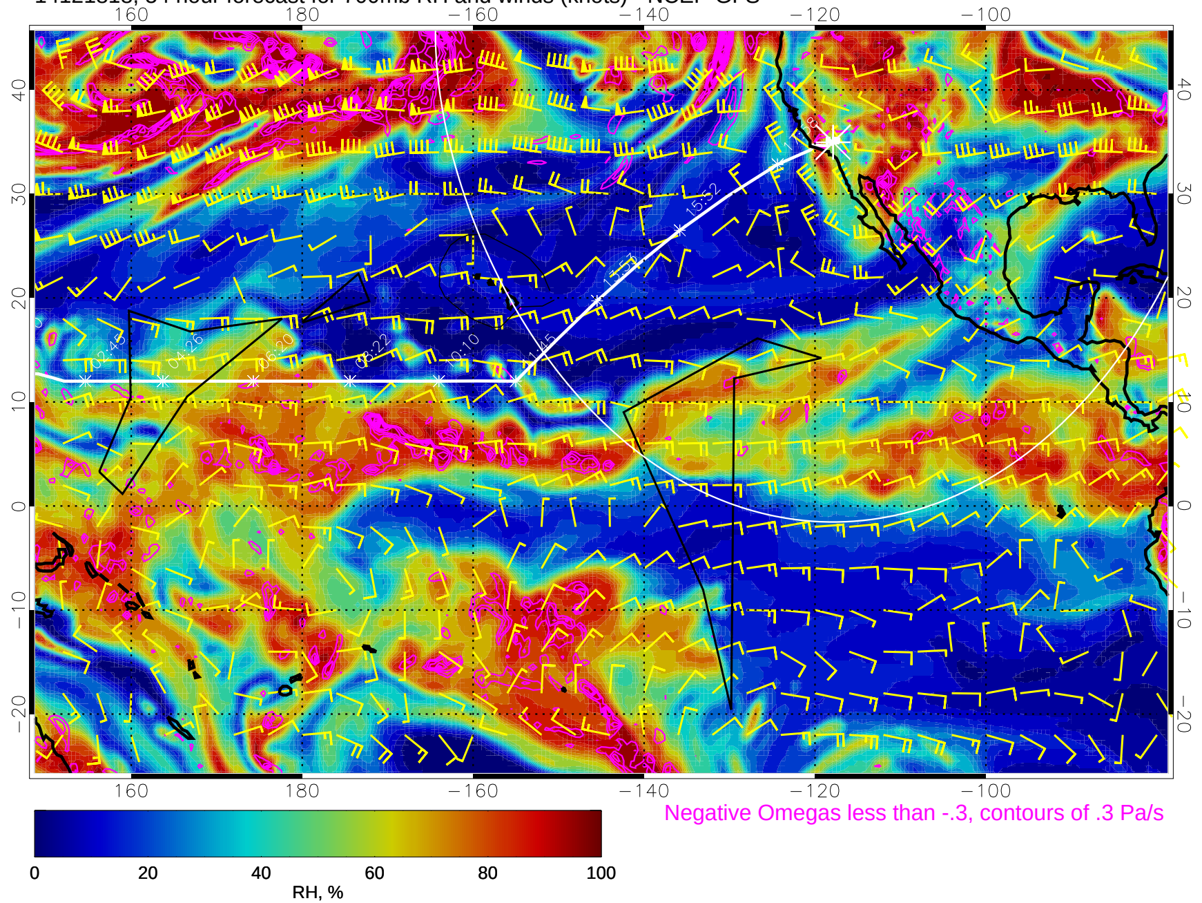
14121818, 54 hour forecast for 700mb RH and winds (knots) - NCEP GFS
