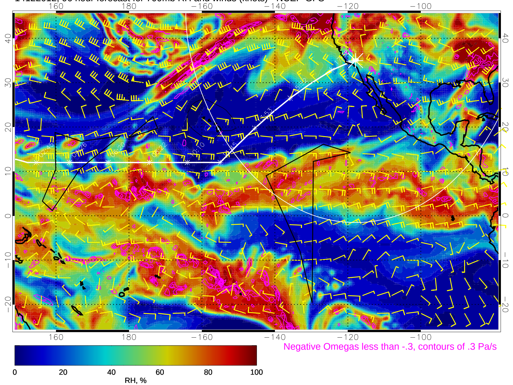
14122012, 96 hour forecast for 700mb RH and winds (knots) - NCEP GFS
