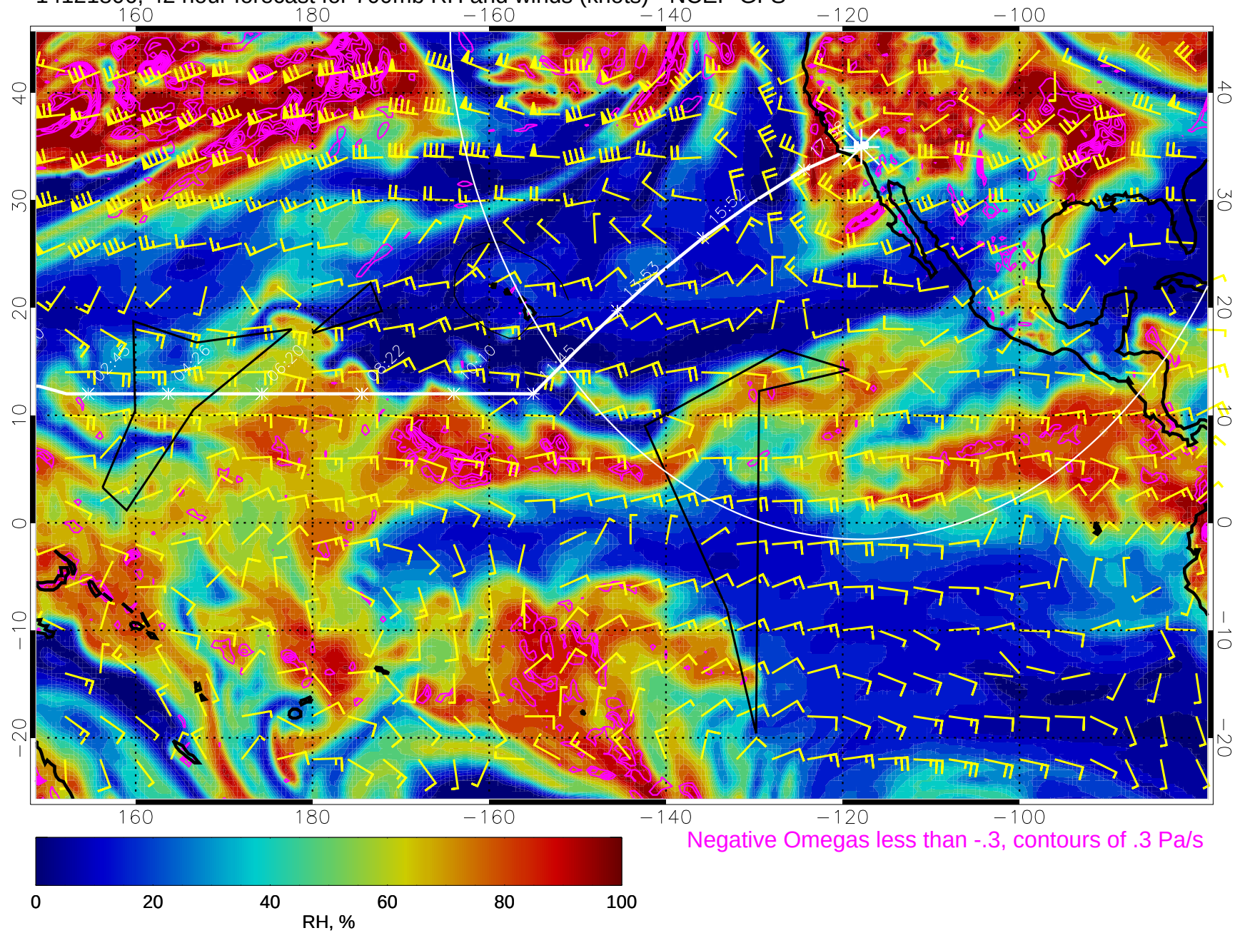
14121806, 42 hour forecast for 700mb RH and winds (knots) - NCEP GFS
