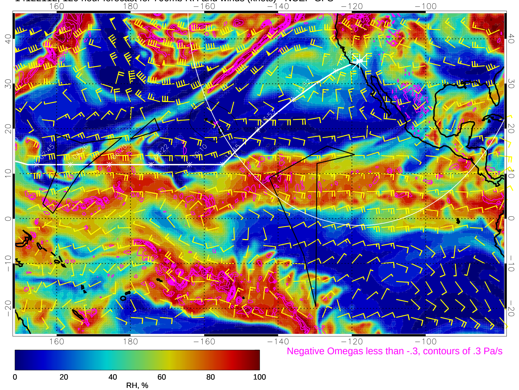
14122112, 120 hour forecast for 700mb RH and winds (knots) - NCEP GFS
