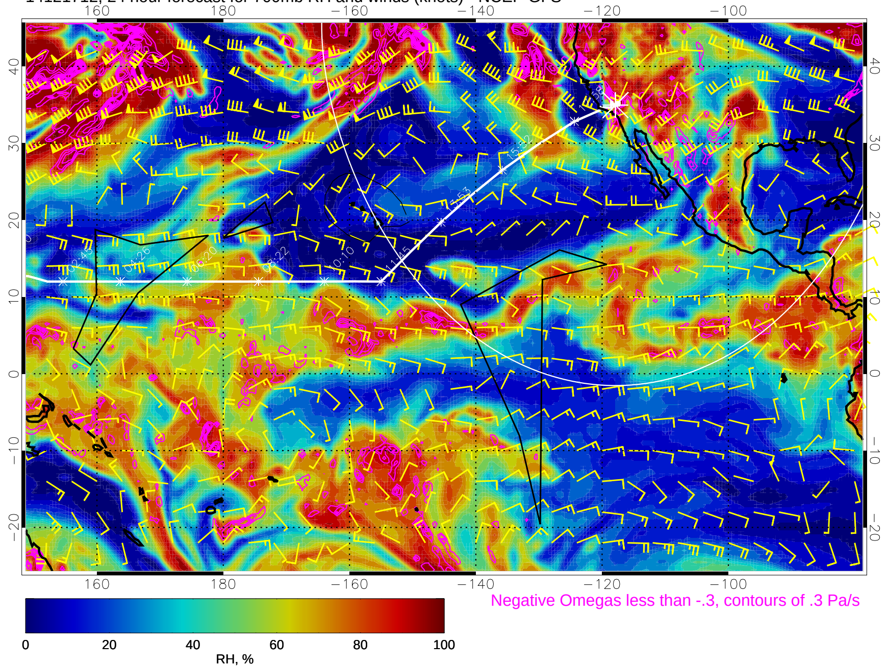
14121712, 24 hour forecast for 700mb RH and winds (knots) - NCEP GFS
