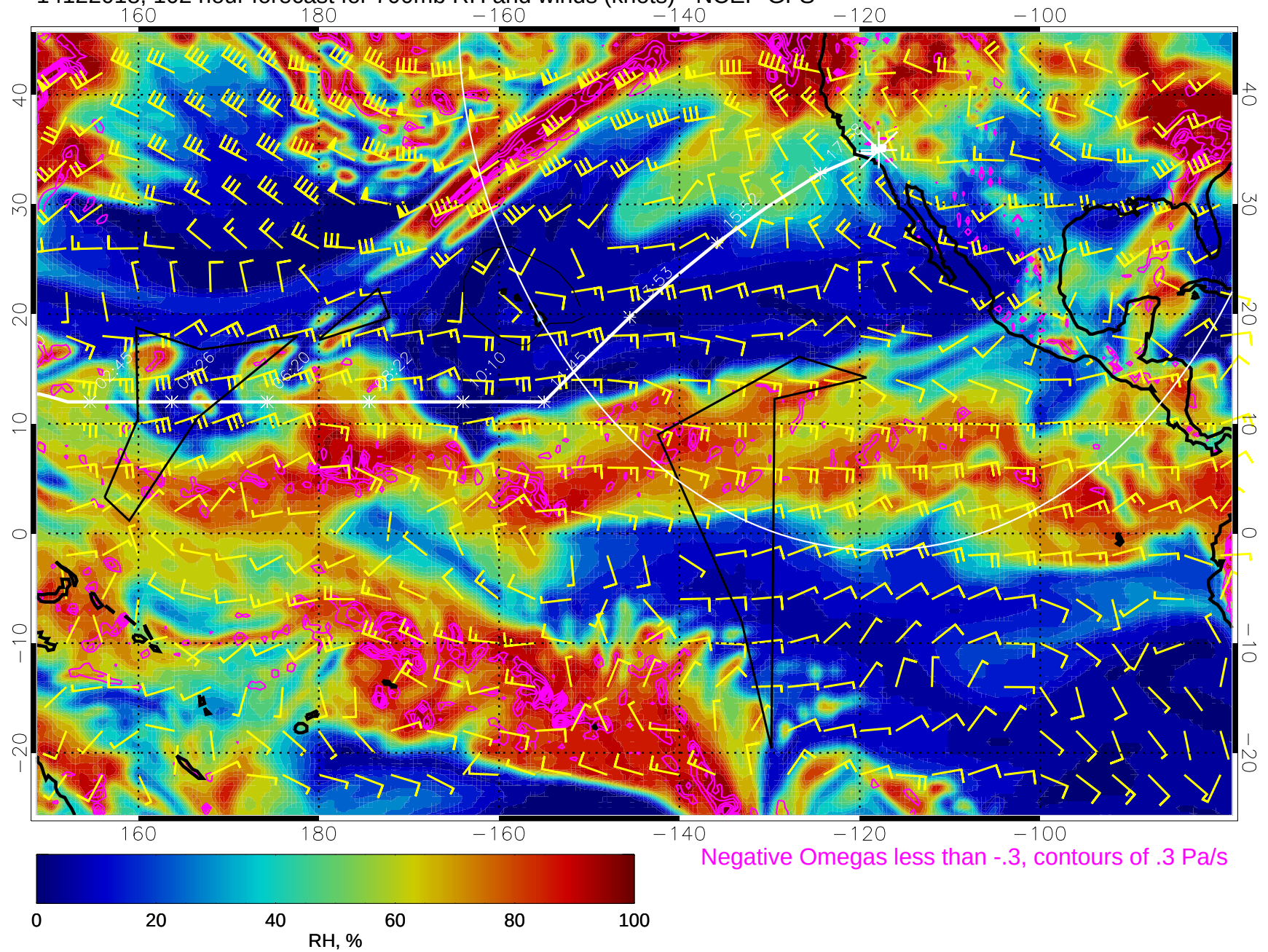
14122018, 102 hour forecast for 700mb RH and winds (knots) - NCEP GFS
