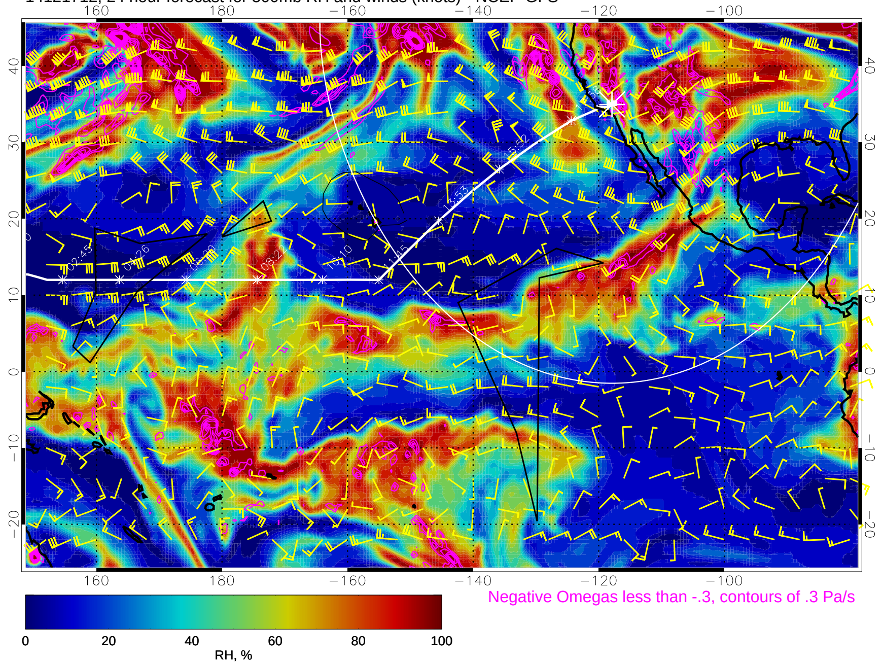
14121712, 24 hour forecast for 500mb RH and winds (knots) - NCEP GFS
