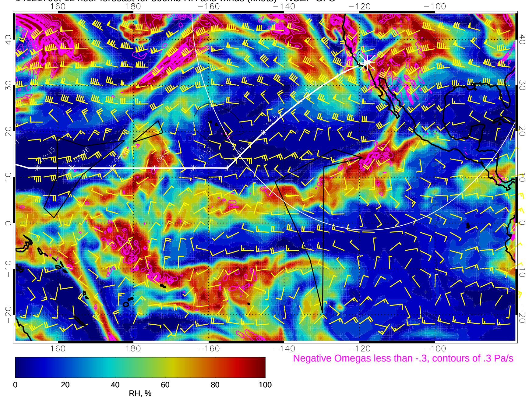
14121700, 12 hour forecast for 500mb RH and winds (knots) - NCEP GFS
