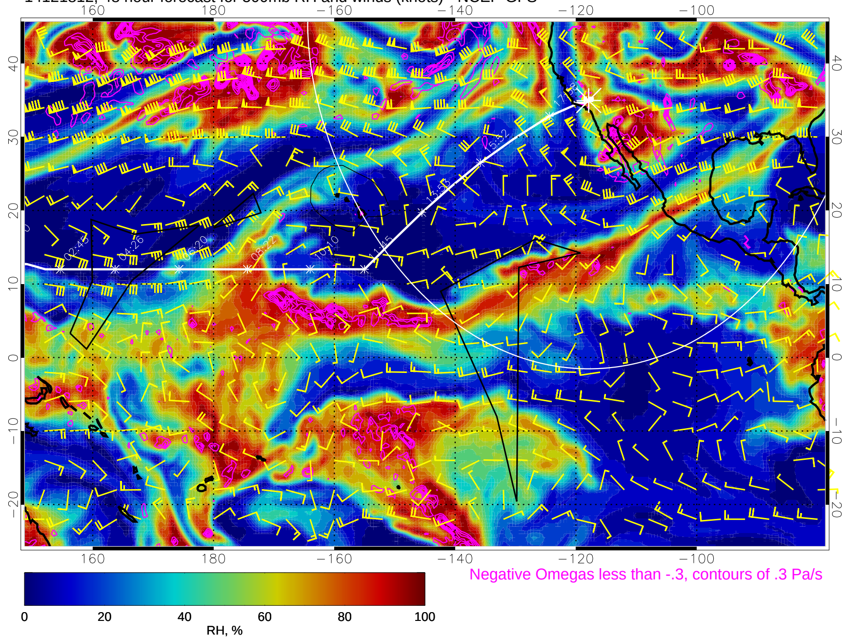
14121812, 48 hour forecast for 500mb RH and winds (knots) - NCEP GFS
