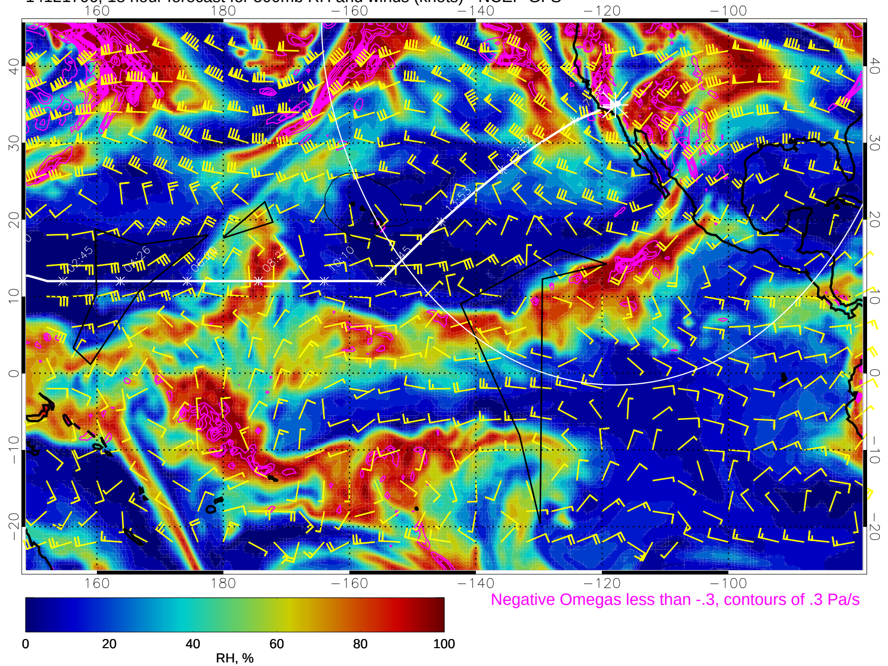
14121706, 18 hour forecast for 500mb RH and winds (knots) - NCEP GFS
