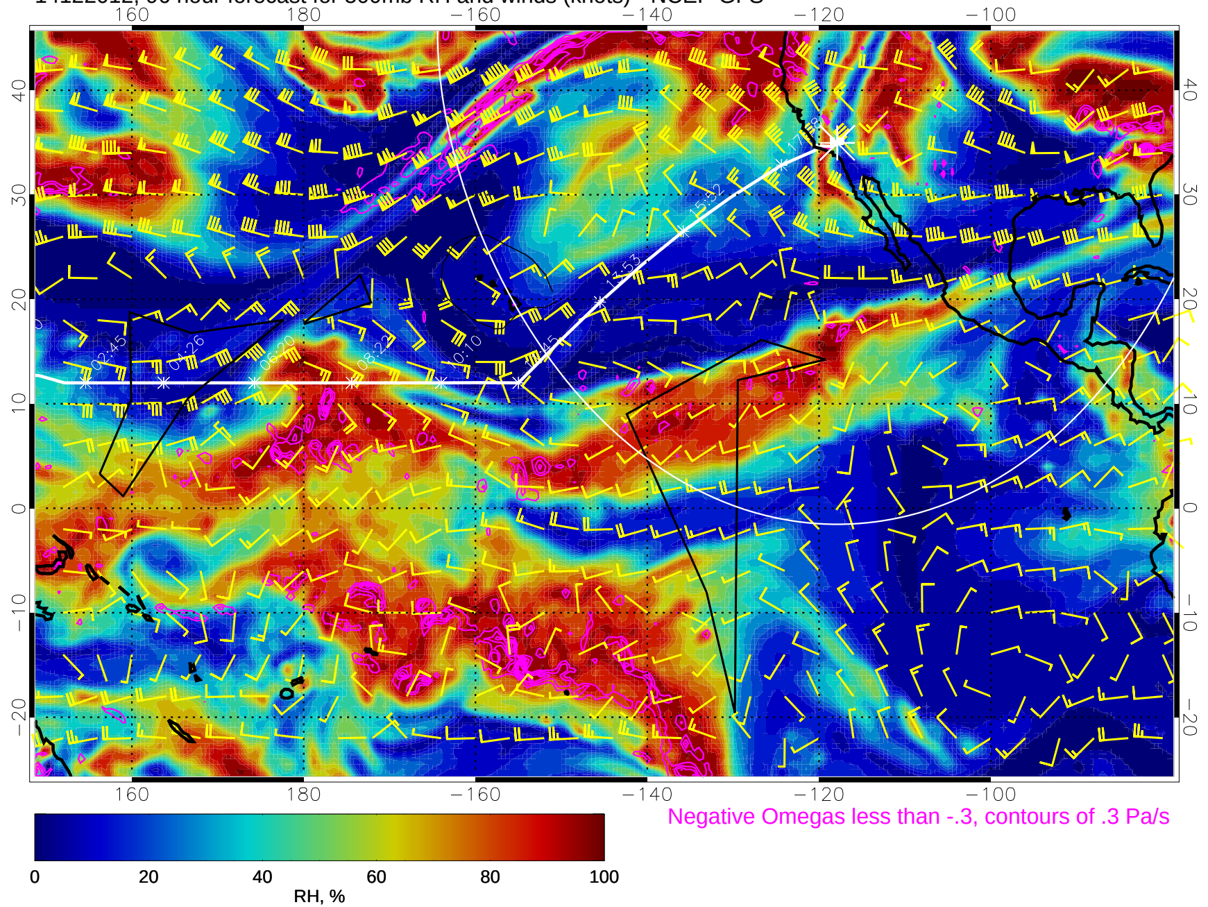
14122012, 96 hour forecast for 500mb RH and winds (knots) - NCEP GFS
