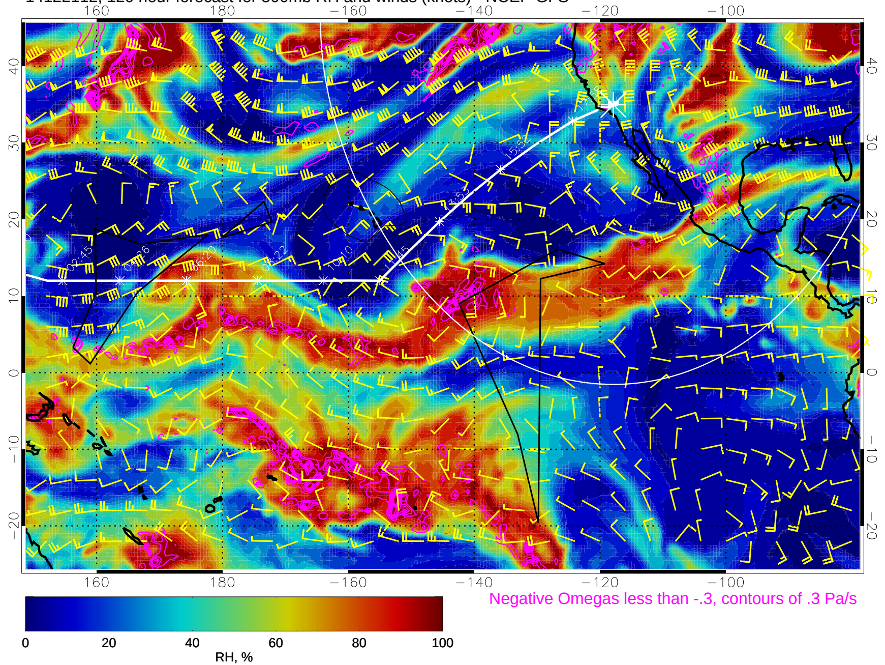
14122112, 120 hour forecast for 500mb RH and winds (knots) - NCEP GFS
