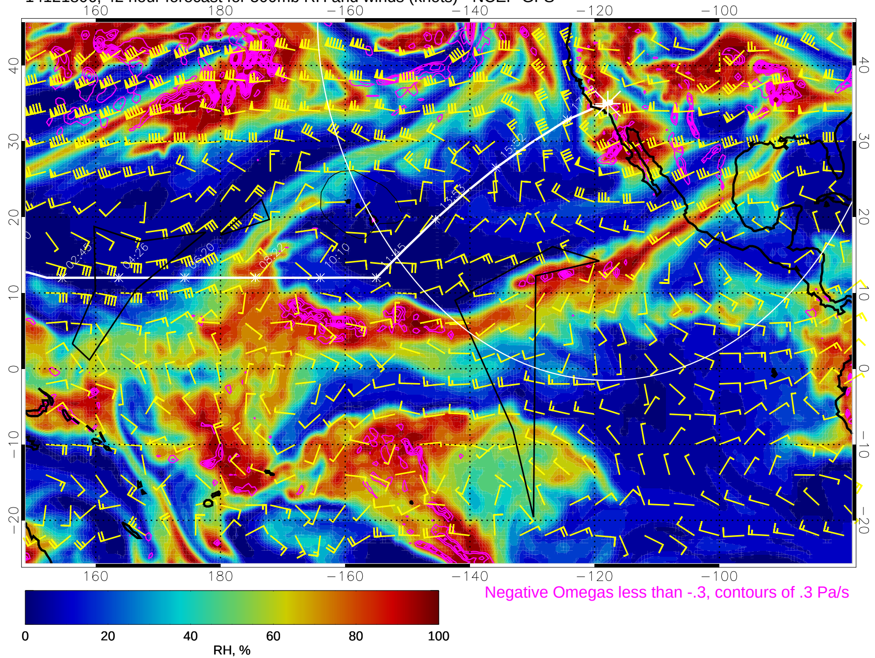
14121806, 42 hour forecast for 500mb RH and winds (knots) - NCEP GFS
