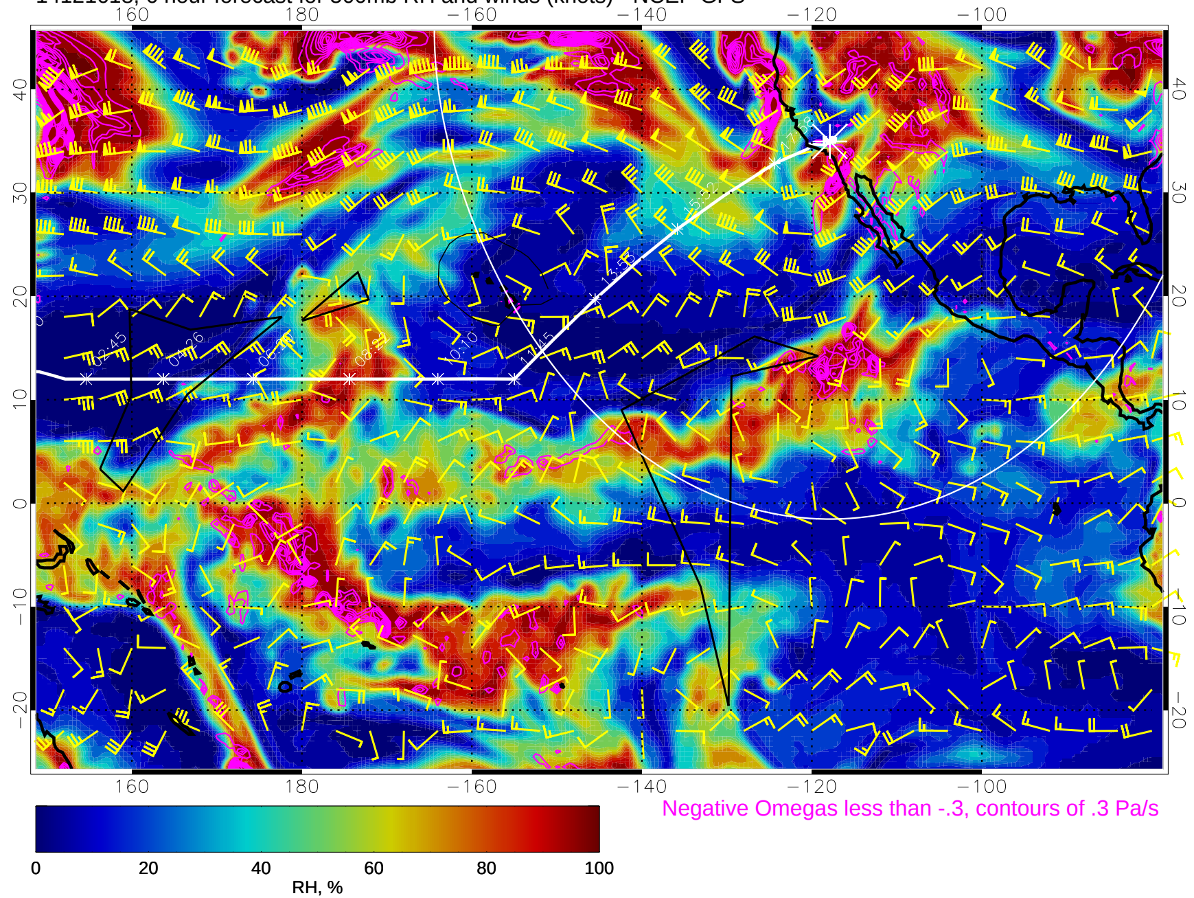
14121618, 6 hour forecast for 500mb RH and winds (knots) - NCEP GFS
