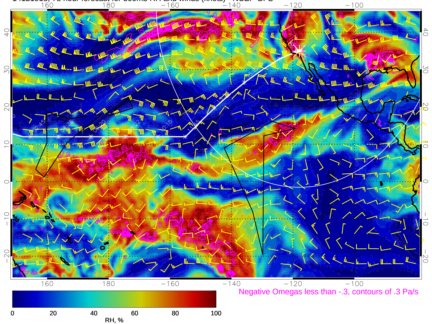
14121918, 78 hour forecast for 500mb RH and winds (knots) - NCEP GFS
